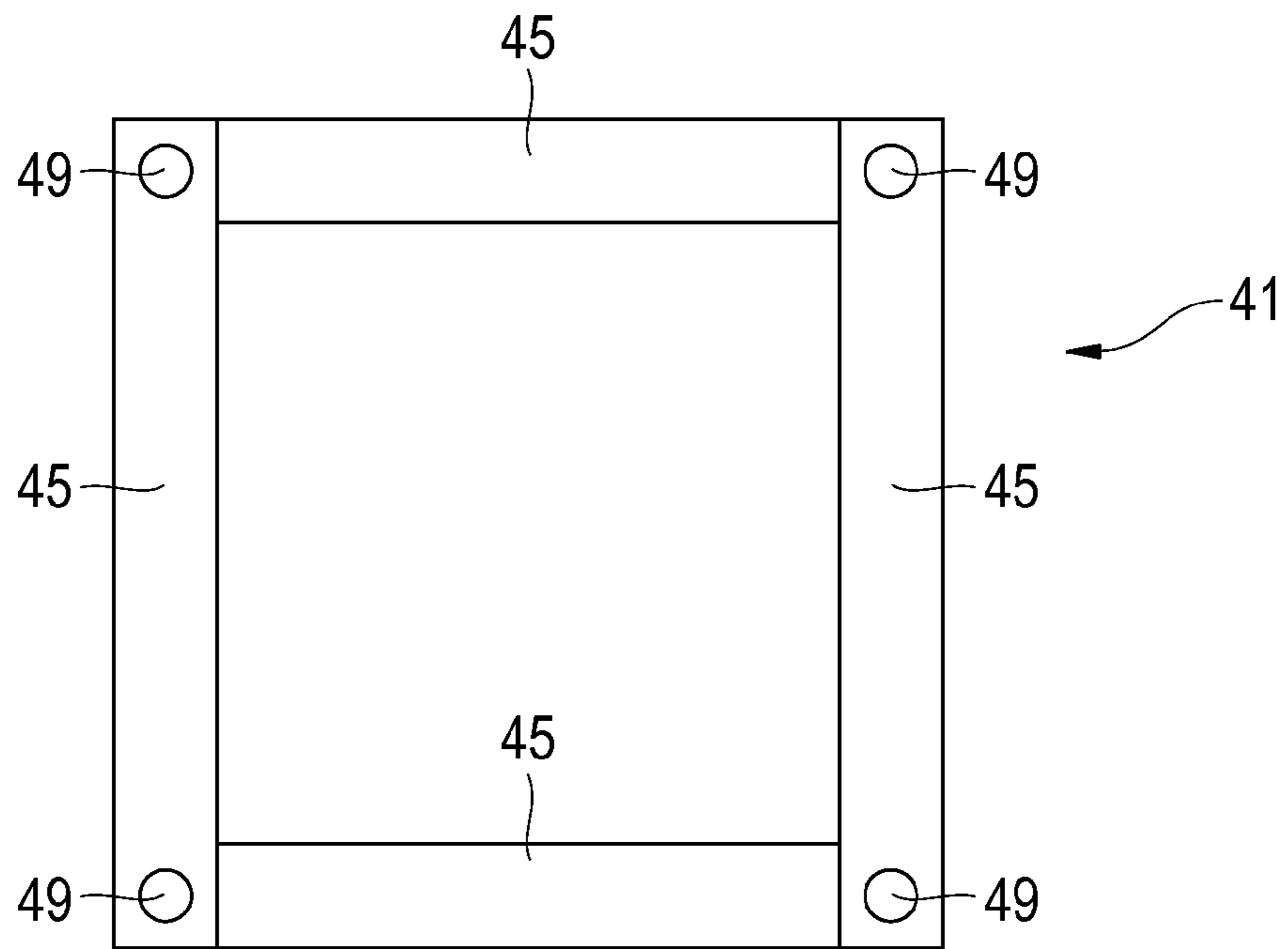
FIG. 2 (Bottom View)
