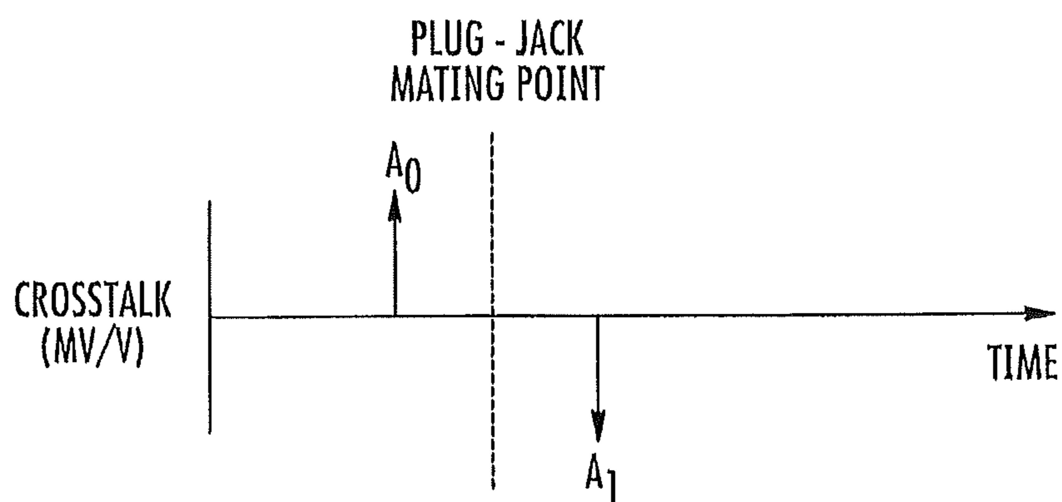
FIG. 4 (PRIOR ART)
