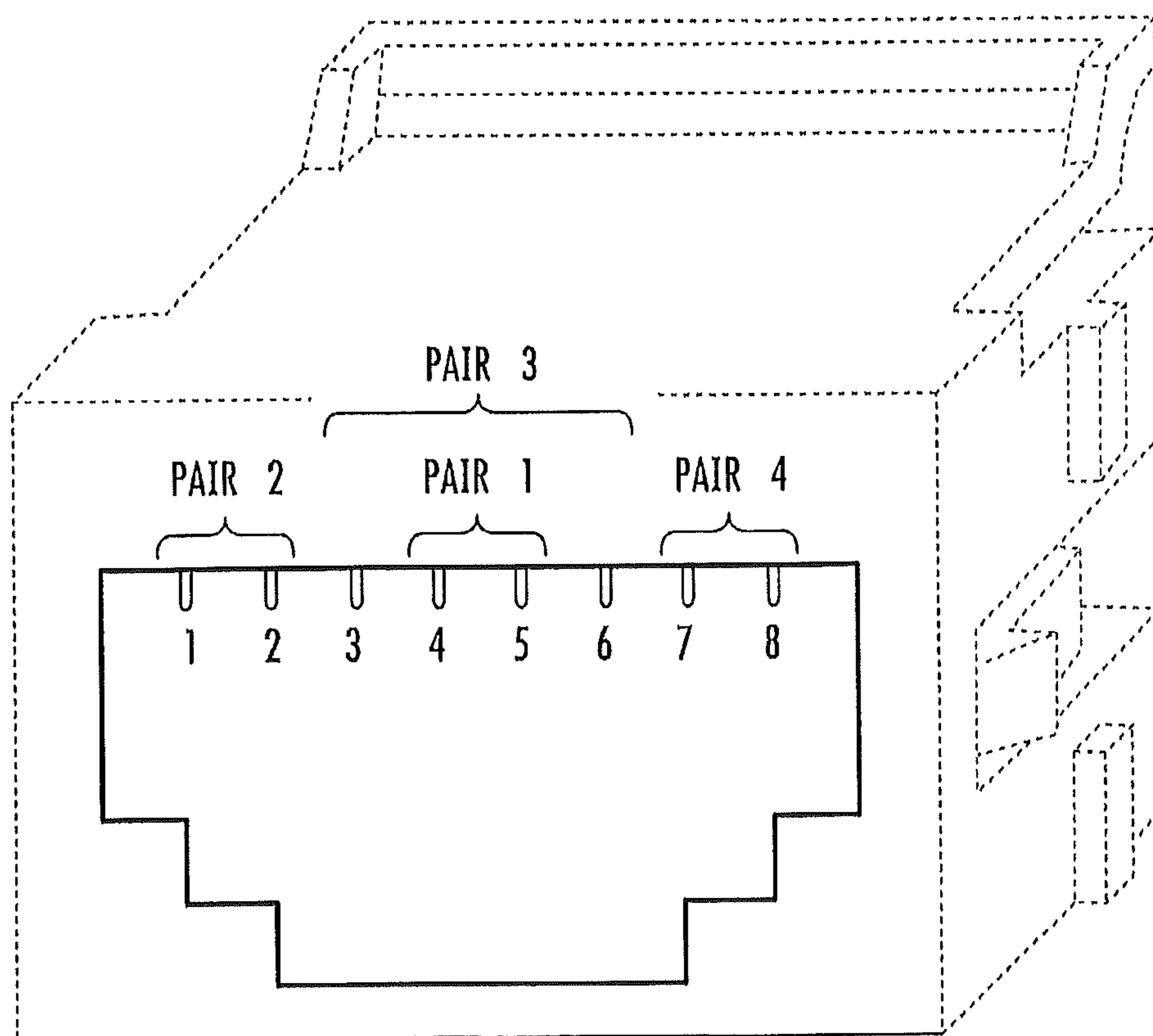
FIG. 2 (PRIOR ART)
