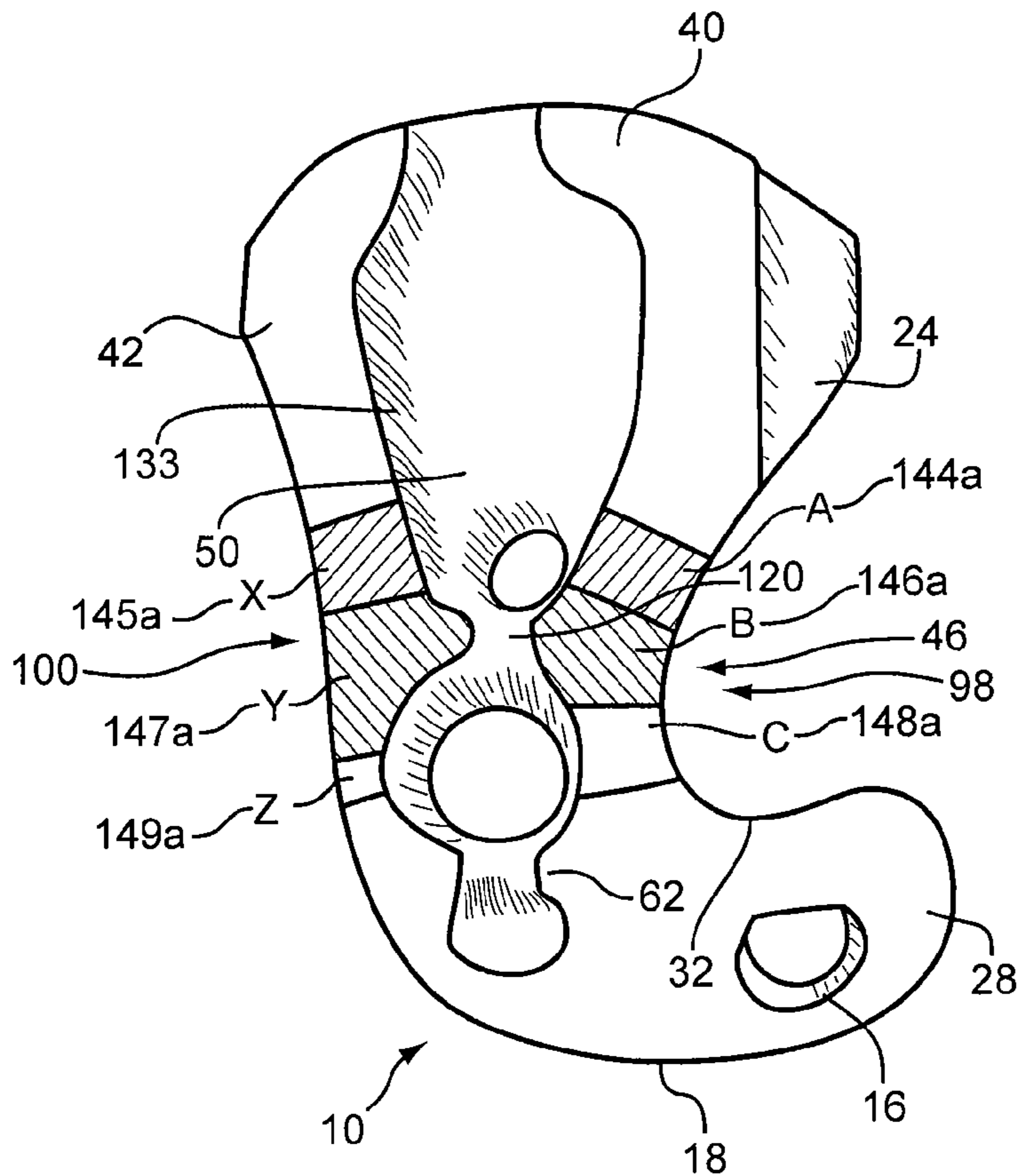
FIG. 16 PRIOR ART
