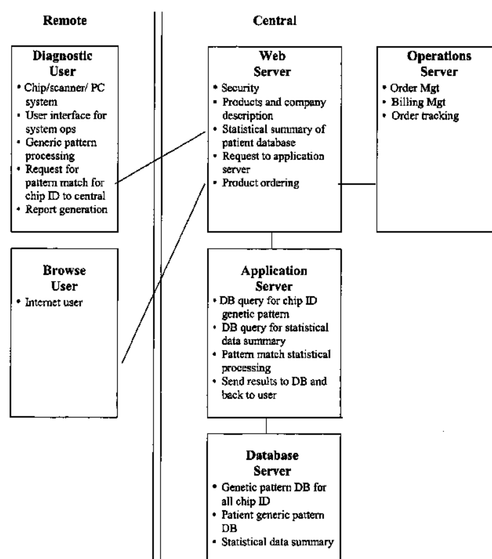
System Architecture
