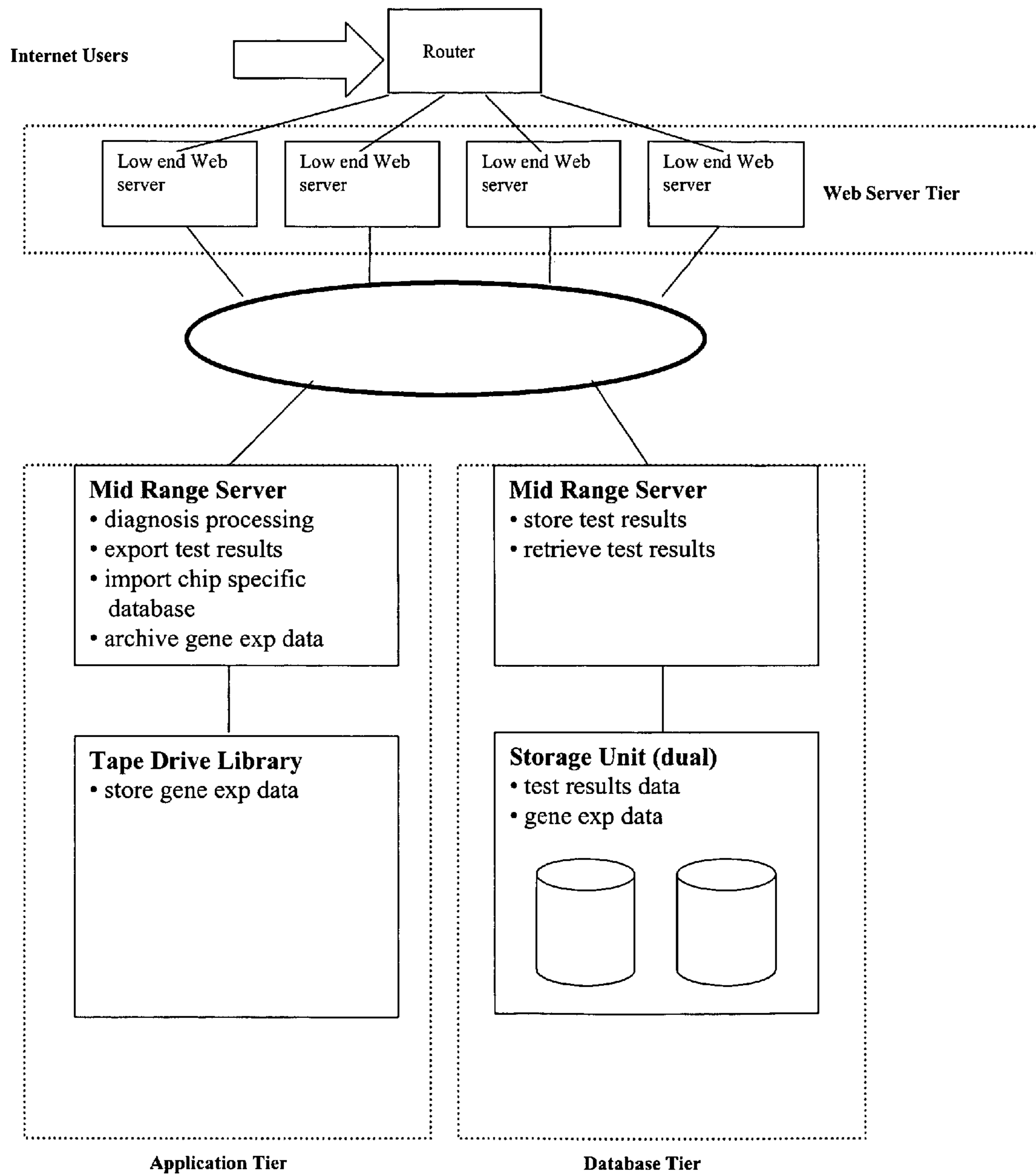
Figure 2: System Design
