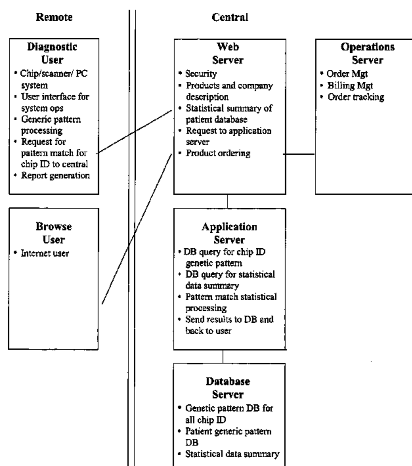
System Architecture
