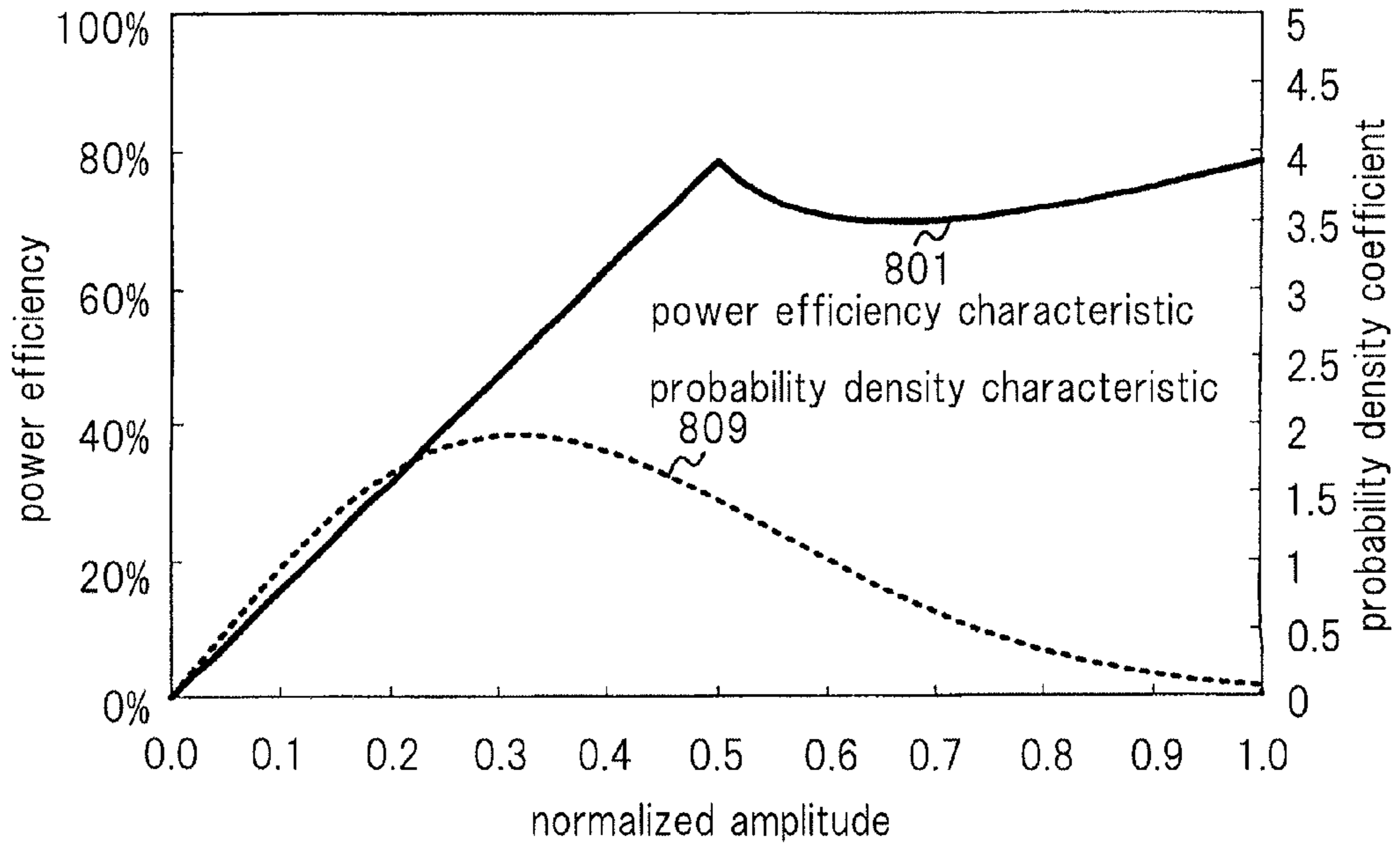
Fig.3 (Related Art)
