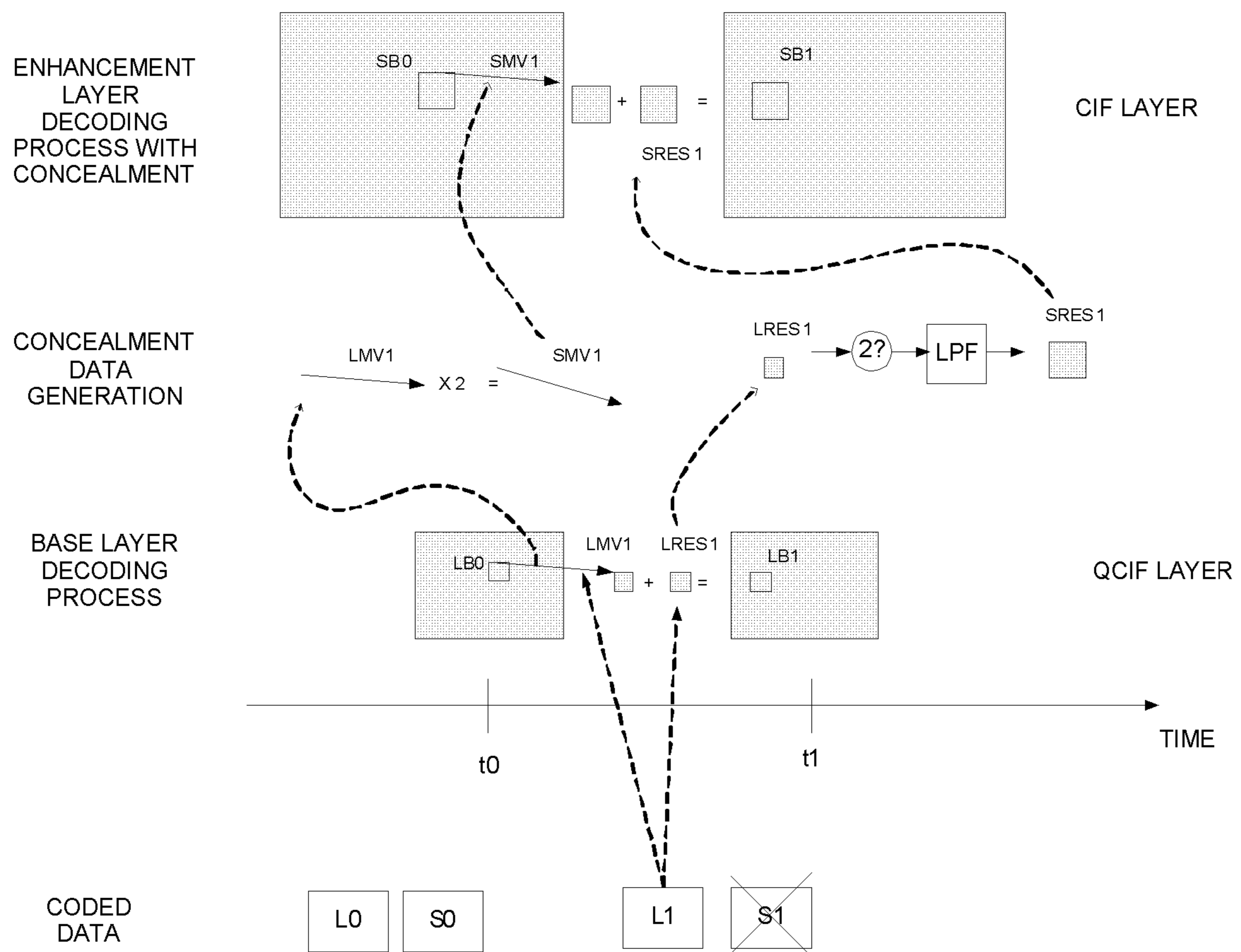
FIG. 8: CONCEALMENT PROCESS
