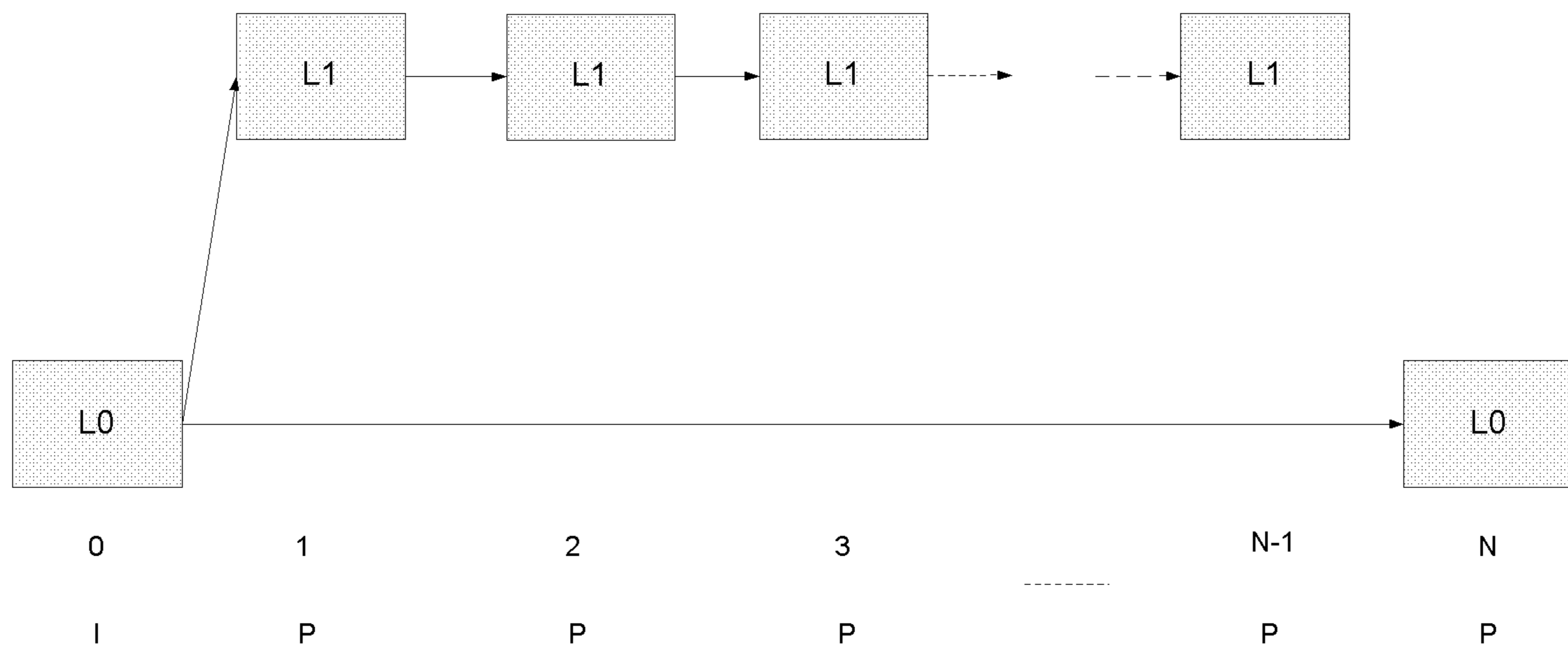
FIG. 5: ALTERNATIVE PICTURE CODING STRUCTURE EXAMPLE
