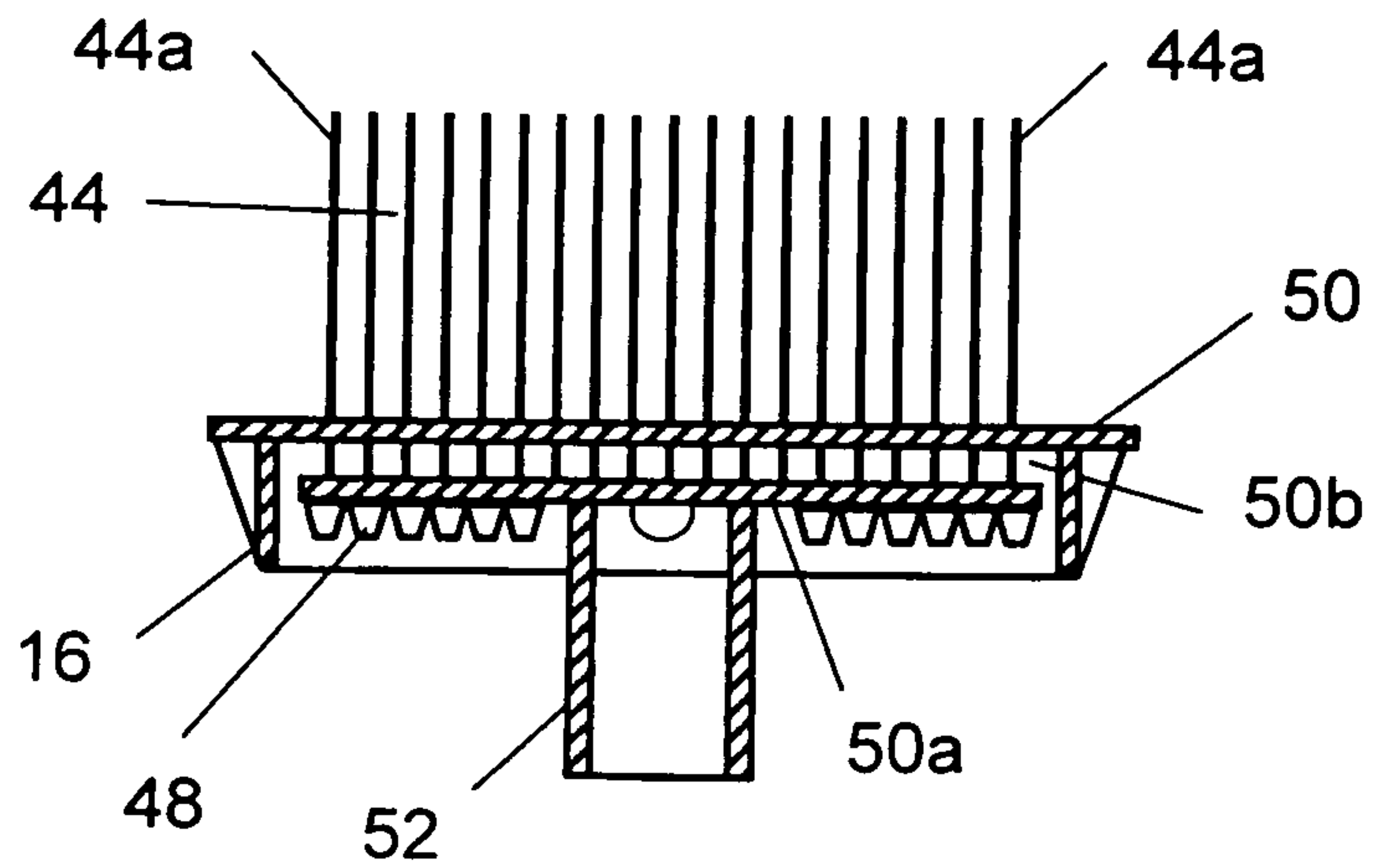
SEC B-B
