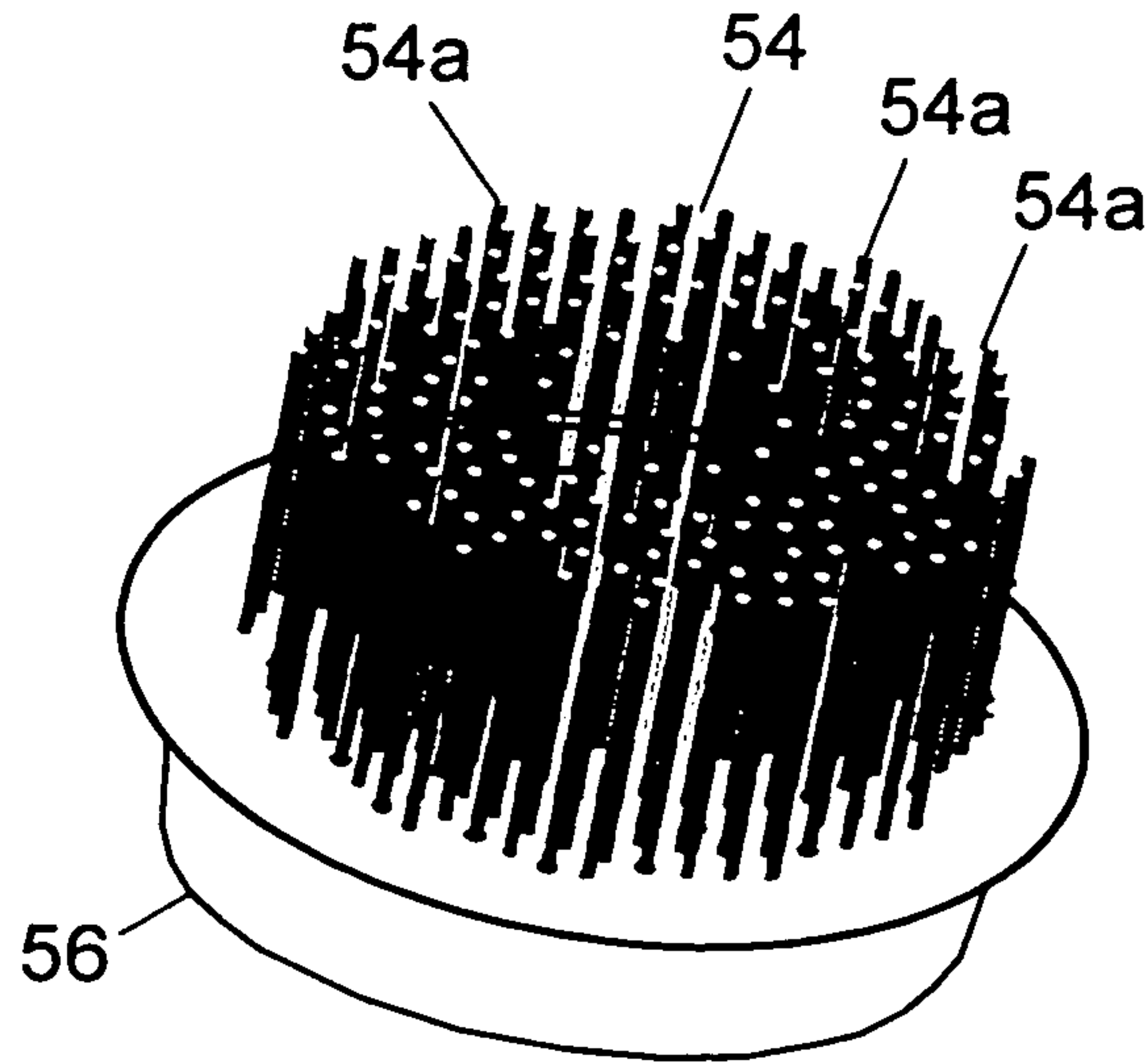
FIGURE 3A (PRIOR ART)
