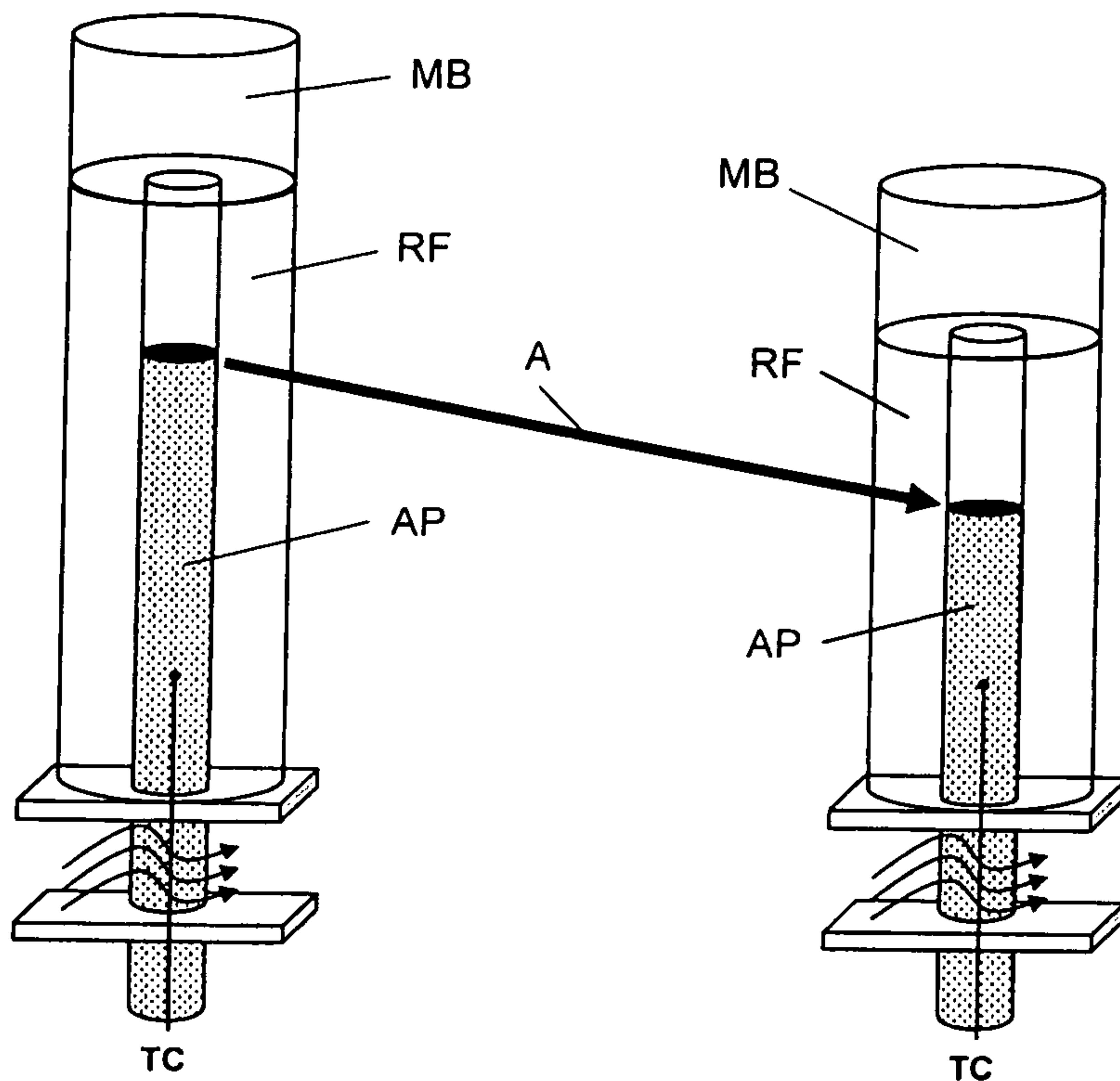
FIGURE 5A (PRIOR ART)
