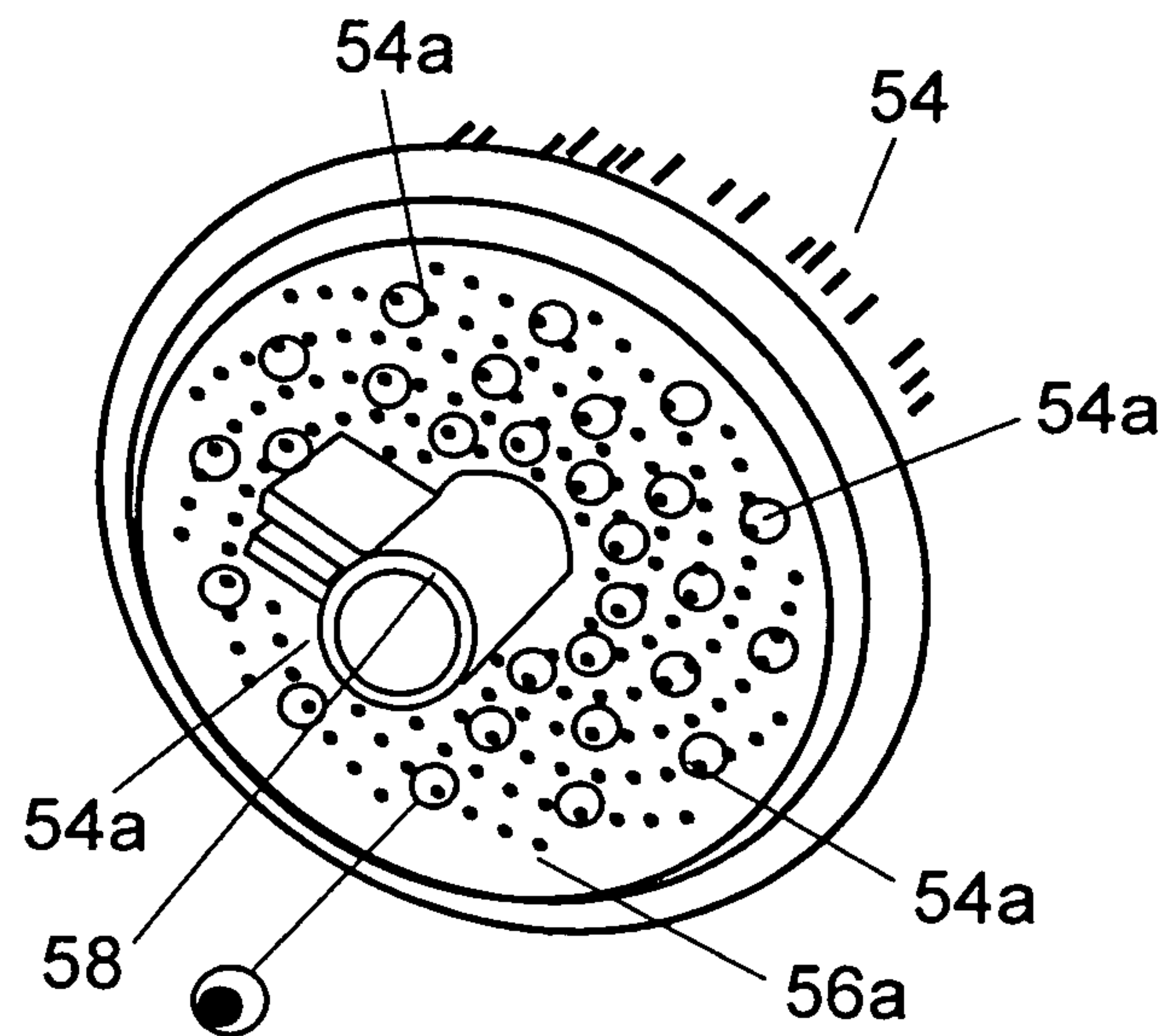
FIGURE 3B (PRIOR ART)
