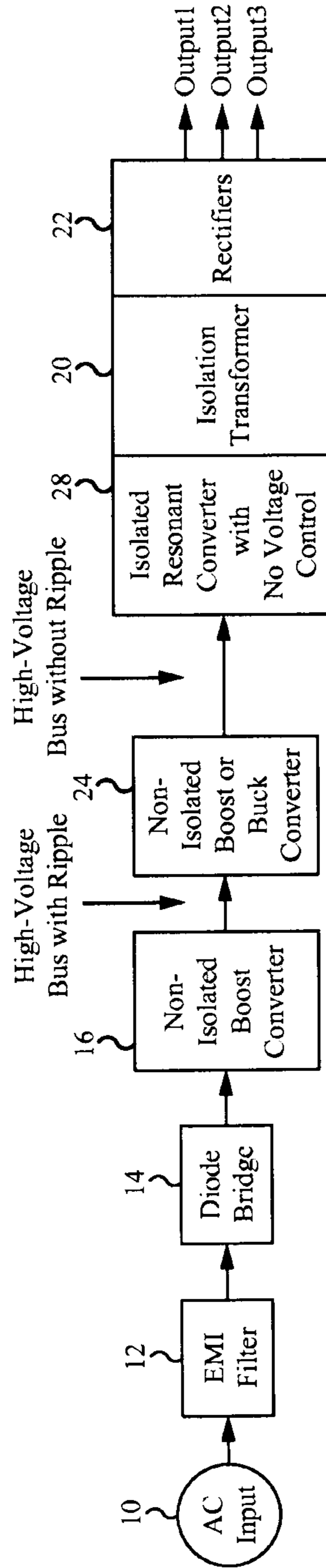
Fig. 2 (Prior Art)
