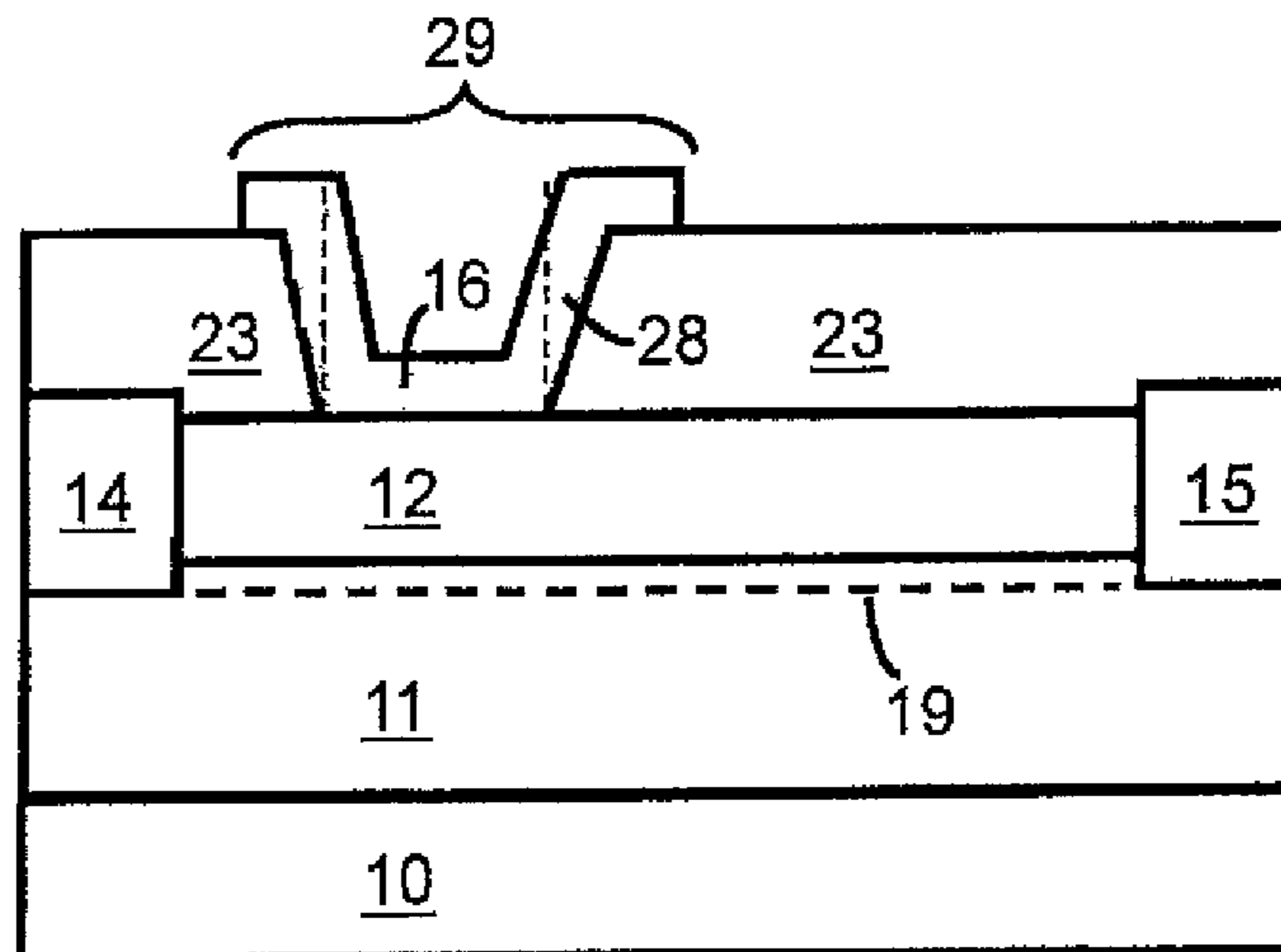
Figure 3 (prior art)
