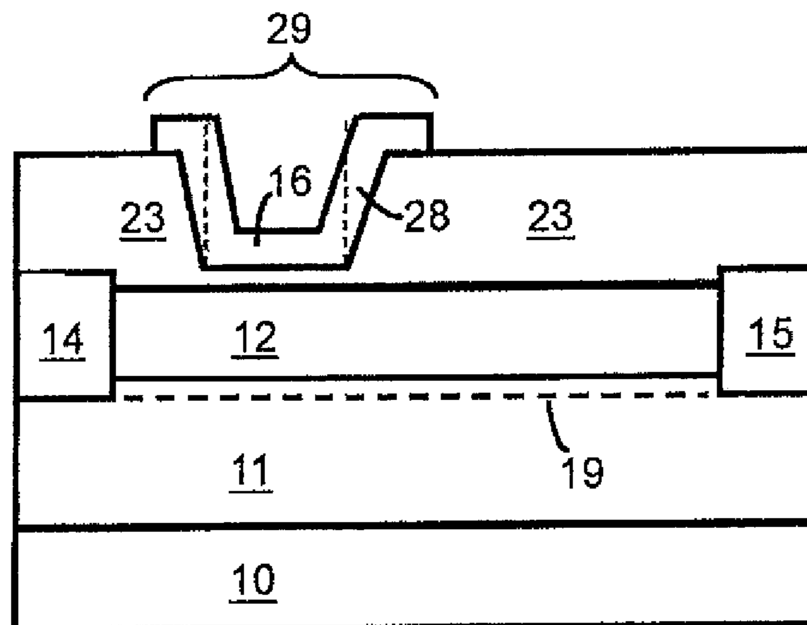
Figure 4 (prior art)
