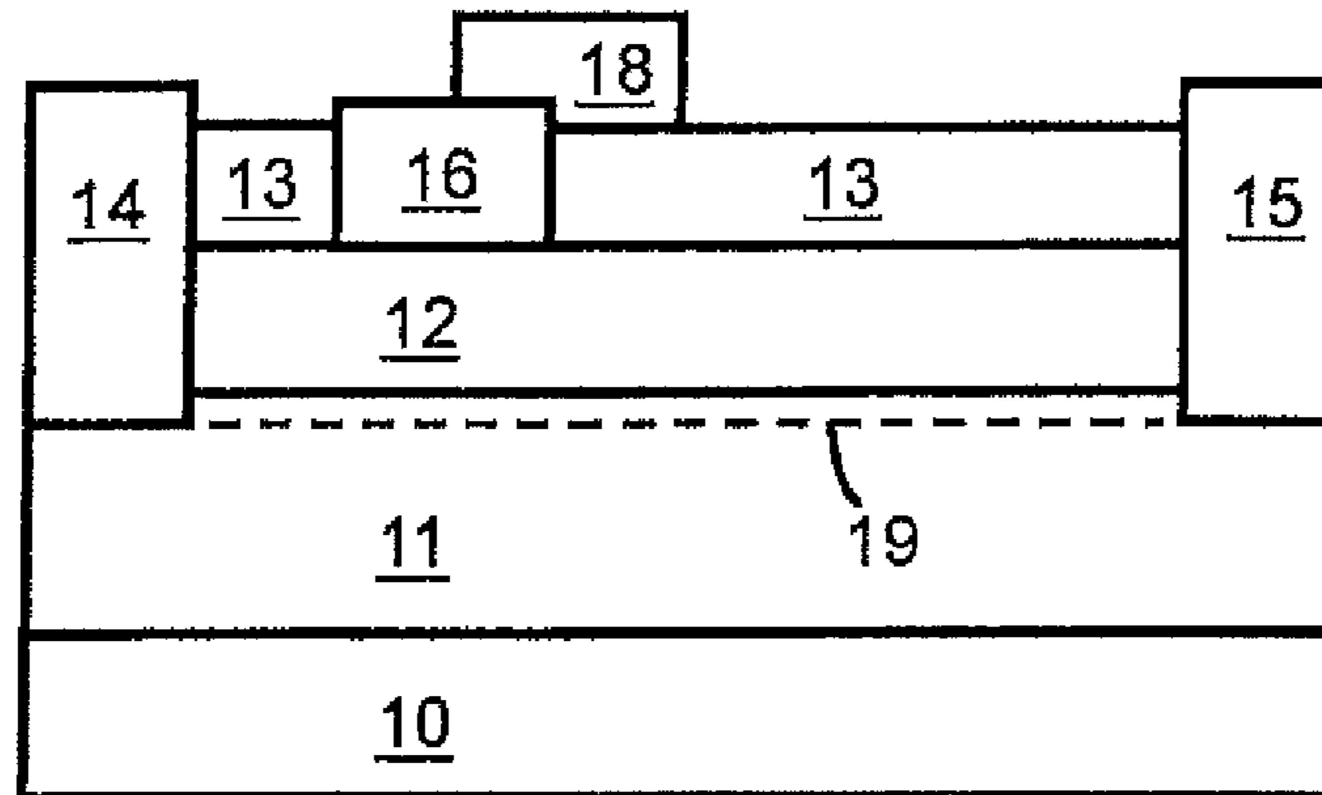
Figure 2 (prior art)
