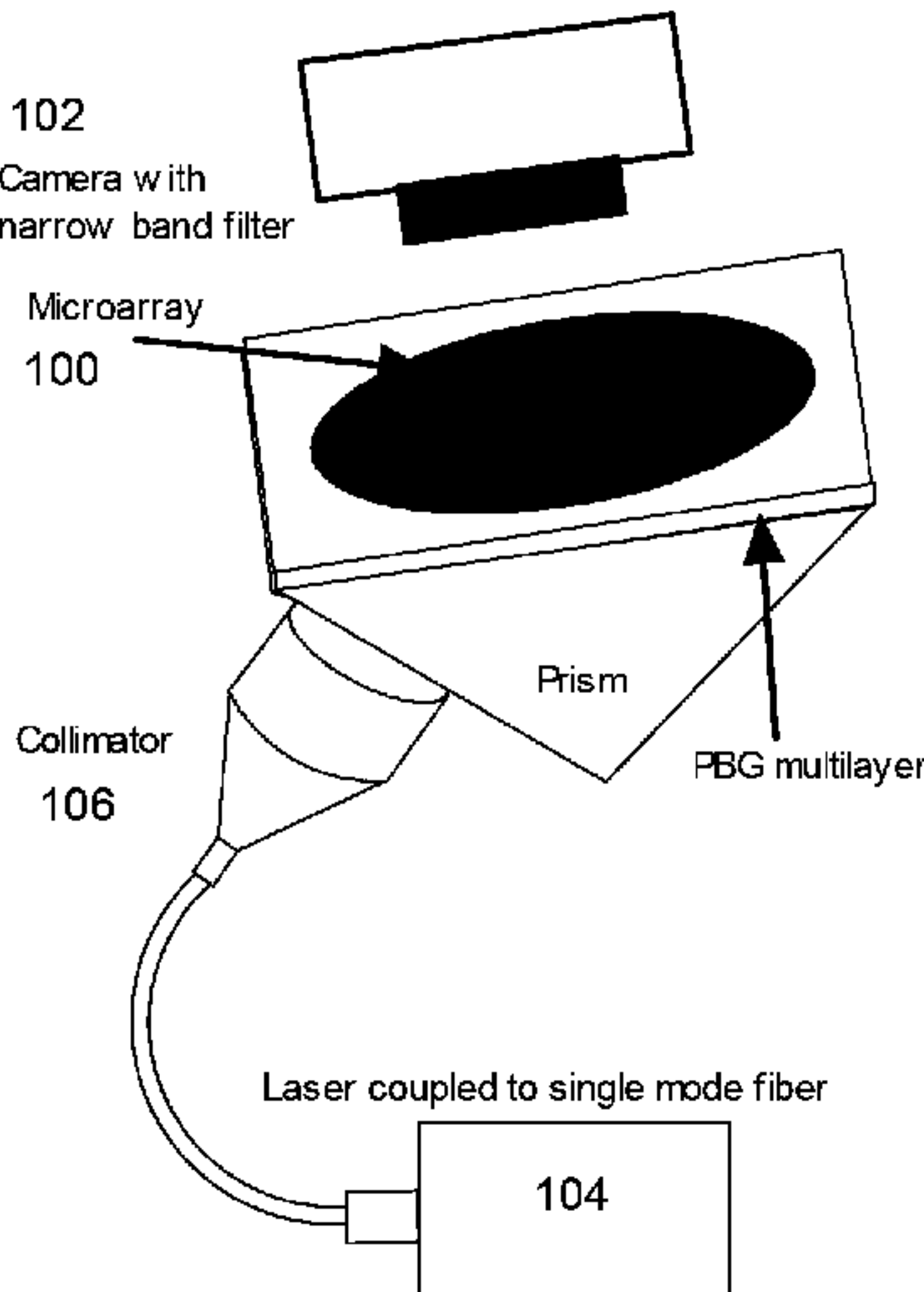
Enhanced fluorescent detection from microarrays utilizing prism coupled illumination to generate SEWs and imaging of the resulting fluorescence from the array elements.
