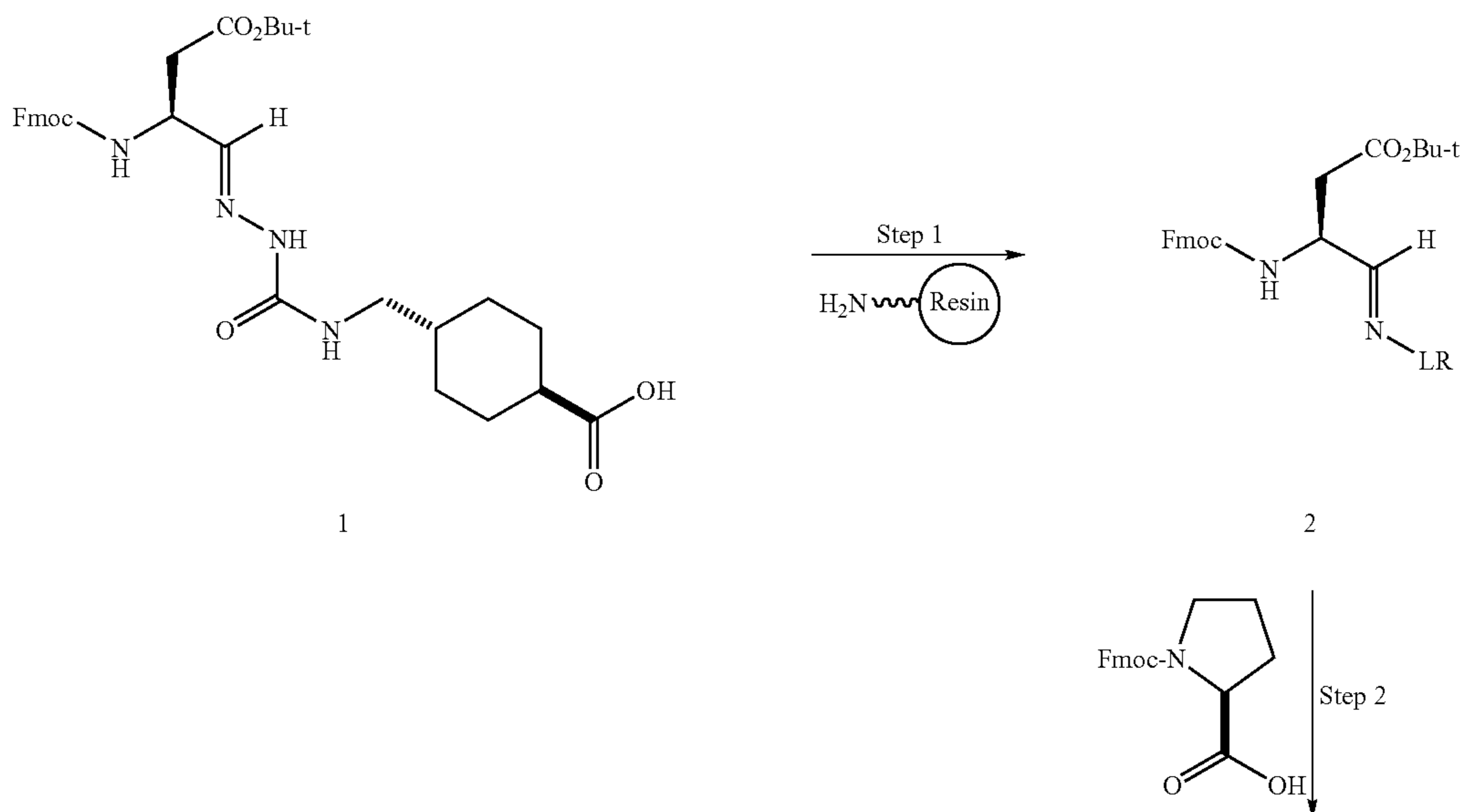
Scheme I
