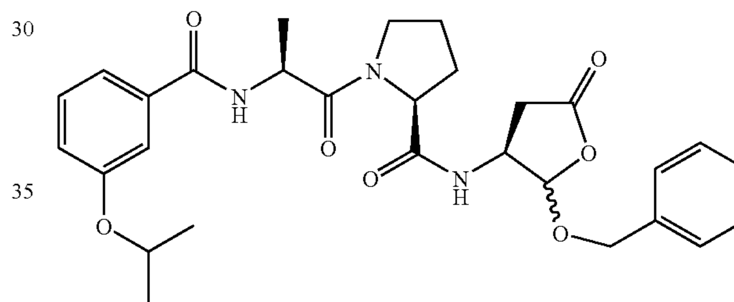
1-[2-(3-Isopropoxy-benzoylamino)-propionyl]-pyrrolidine-2-carboxylic acid (2-benzyloxy-5-oxo-tetrahydro-furan-3-yl)-amide (79)
