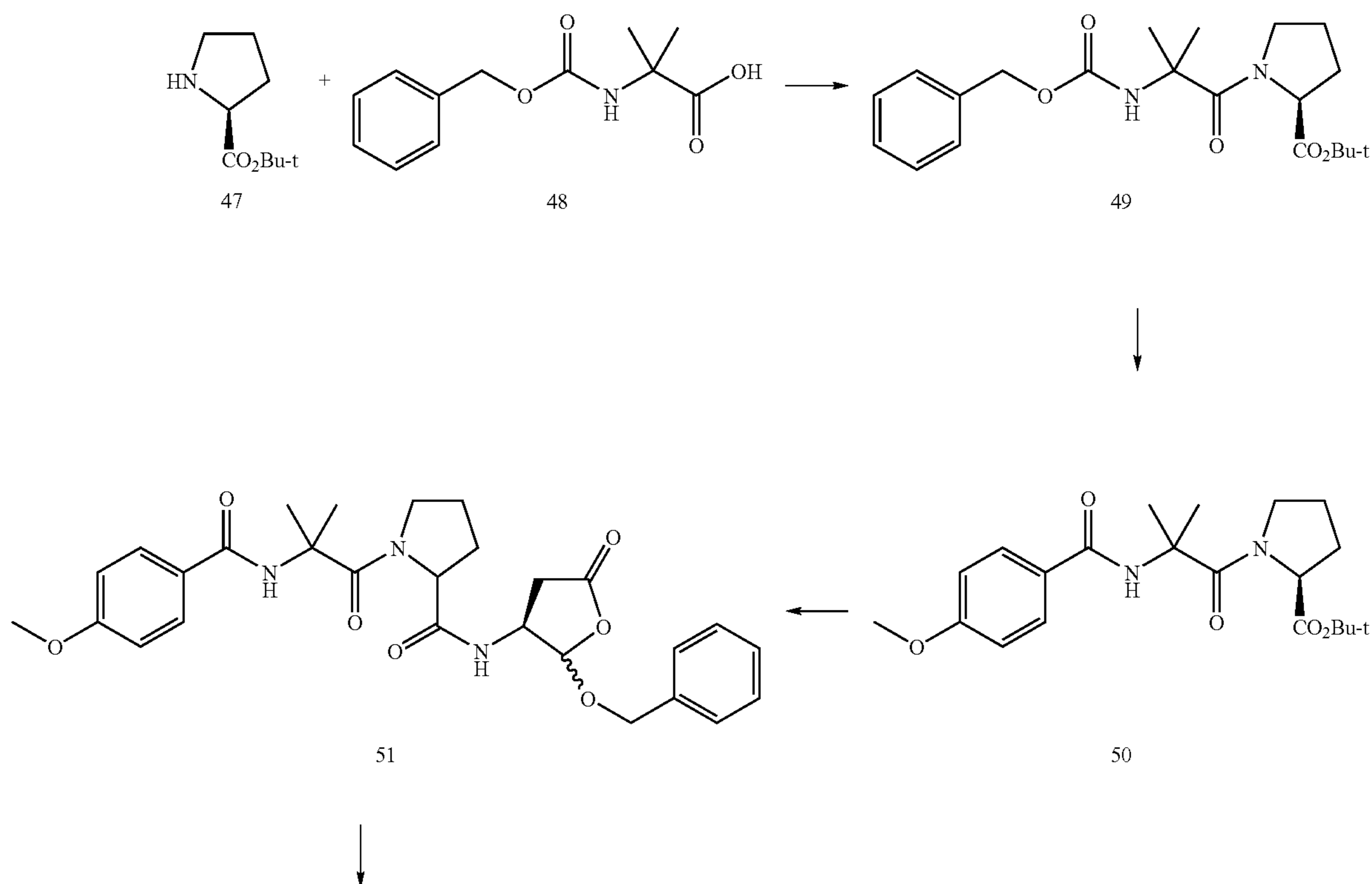
Scheme XI
