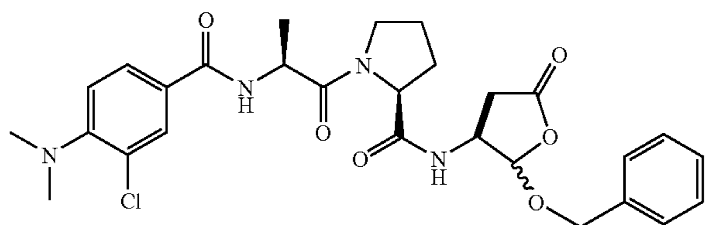
1-[2-(3-chloro-4-dimethylamino-benzoylamino)-propionyl]-pyrrolidine-2-carboxylic acid (2-benzyloxy-5-oxo-tetrahydro-furan-3-yl)-amide (98x)
