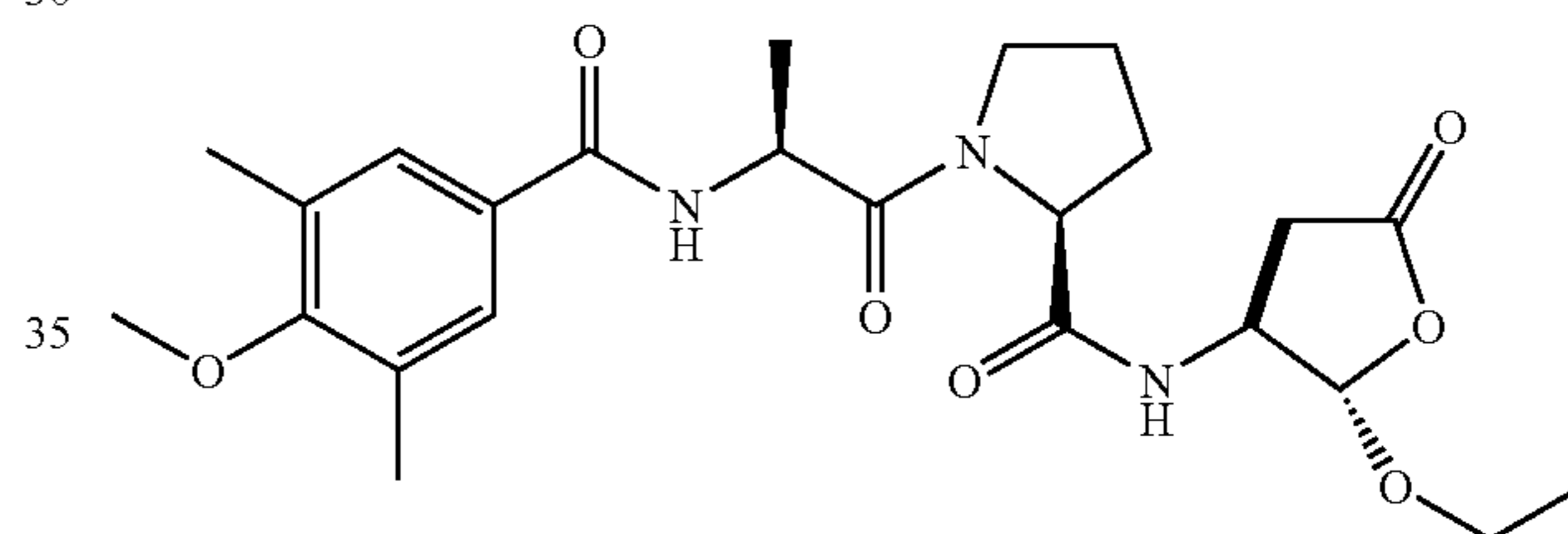
1-[2-(4-Methoxy-3,5-dimethyl-benzoylamino)-propionyl]-pyrrolidine-2-carboxylic acid (2-ethoxy-5-oxo-tetrahydro-furan-3-yl)-amide (98af)
