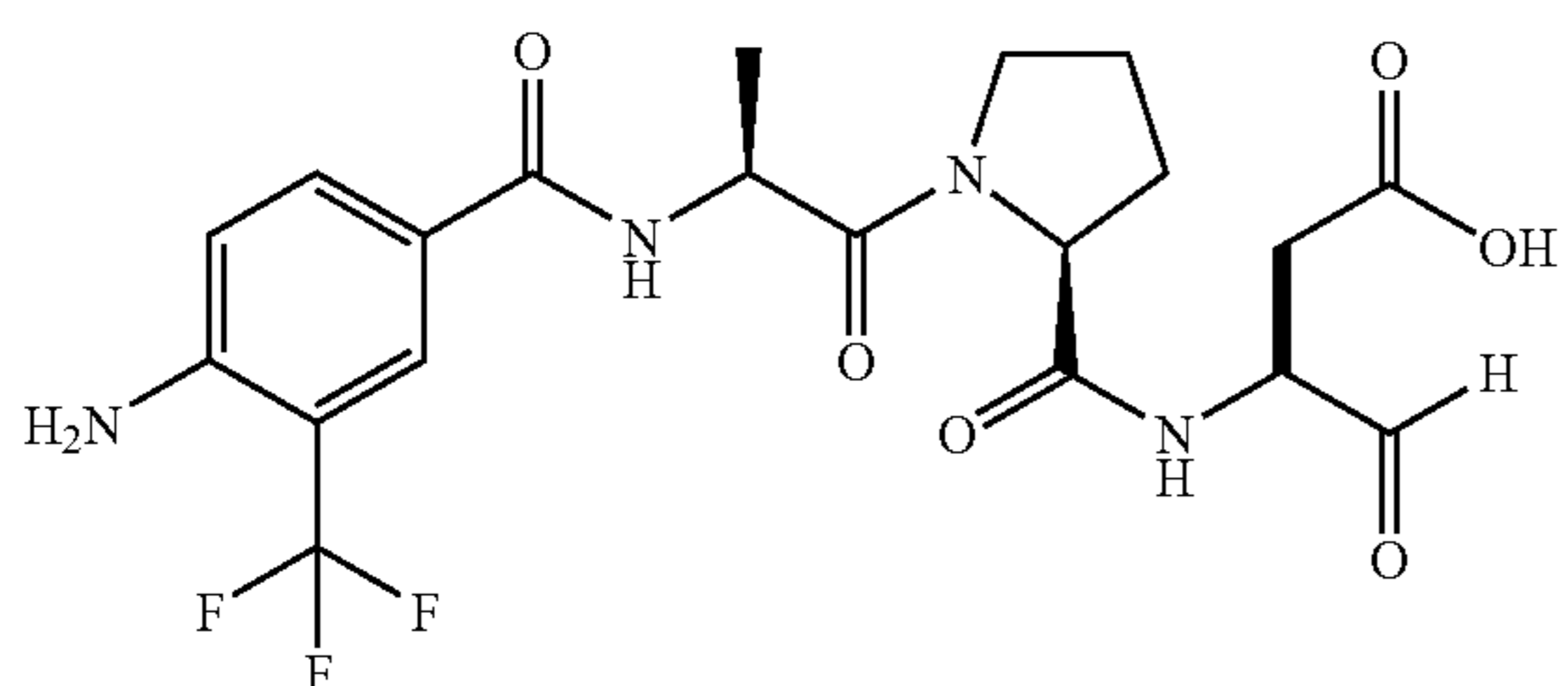
3-({1-[2-(4-Amino-3-trifluoromethyl-benzoylamino)-propionyl]-pyrrolidine-2-carbonyl}-amino)-4-oxo-butyric acid (1221)
