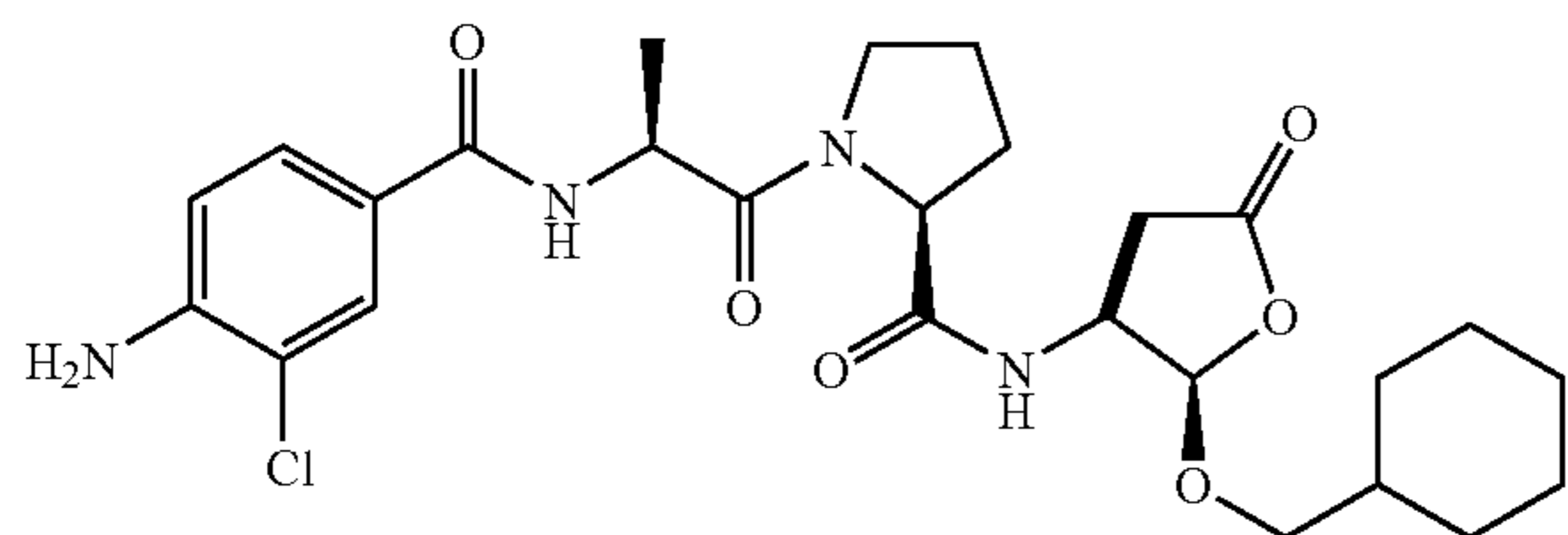
1-[2-(4-Amino-3-chloro-benzoylamino)-propionyl]-pyrrolidine-2-carboxylic acid (2-cyclohexylmethoxy-5-oxo-tetrahydro-furan-3-yl)-amide (98aq)
