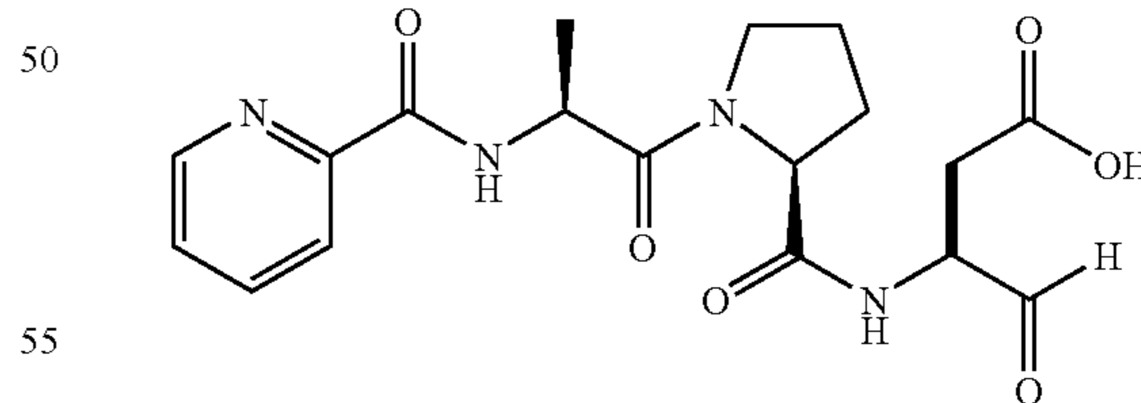
3-({1-[2-(4-Amino-3-chloro-benzoylamino)-propionyl]-pyrrolidine-2-carbonyl}-amino)-4-oxo-butyrac acid (122b)
