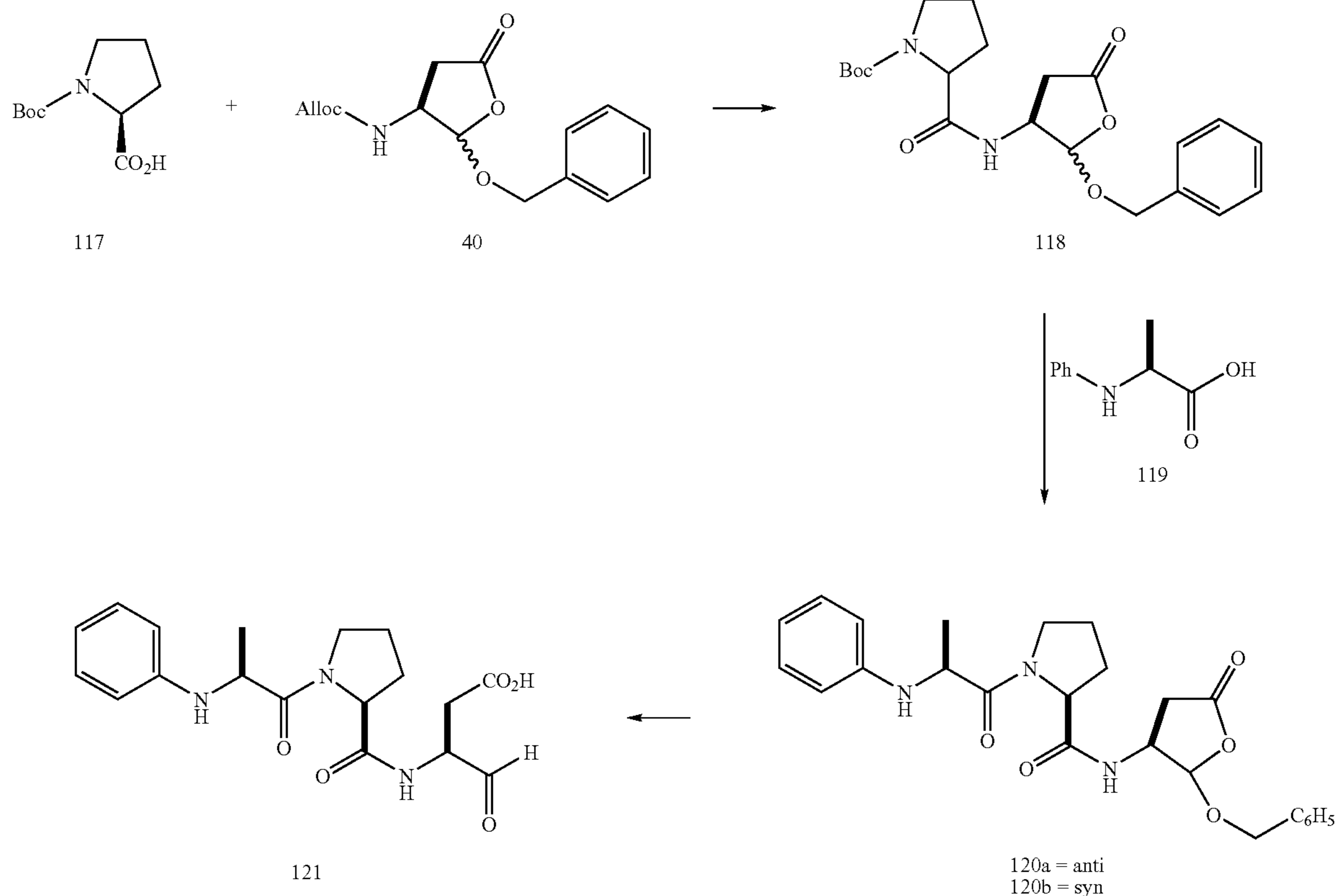
Scheme XXII
