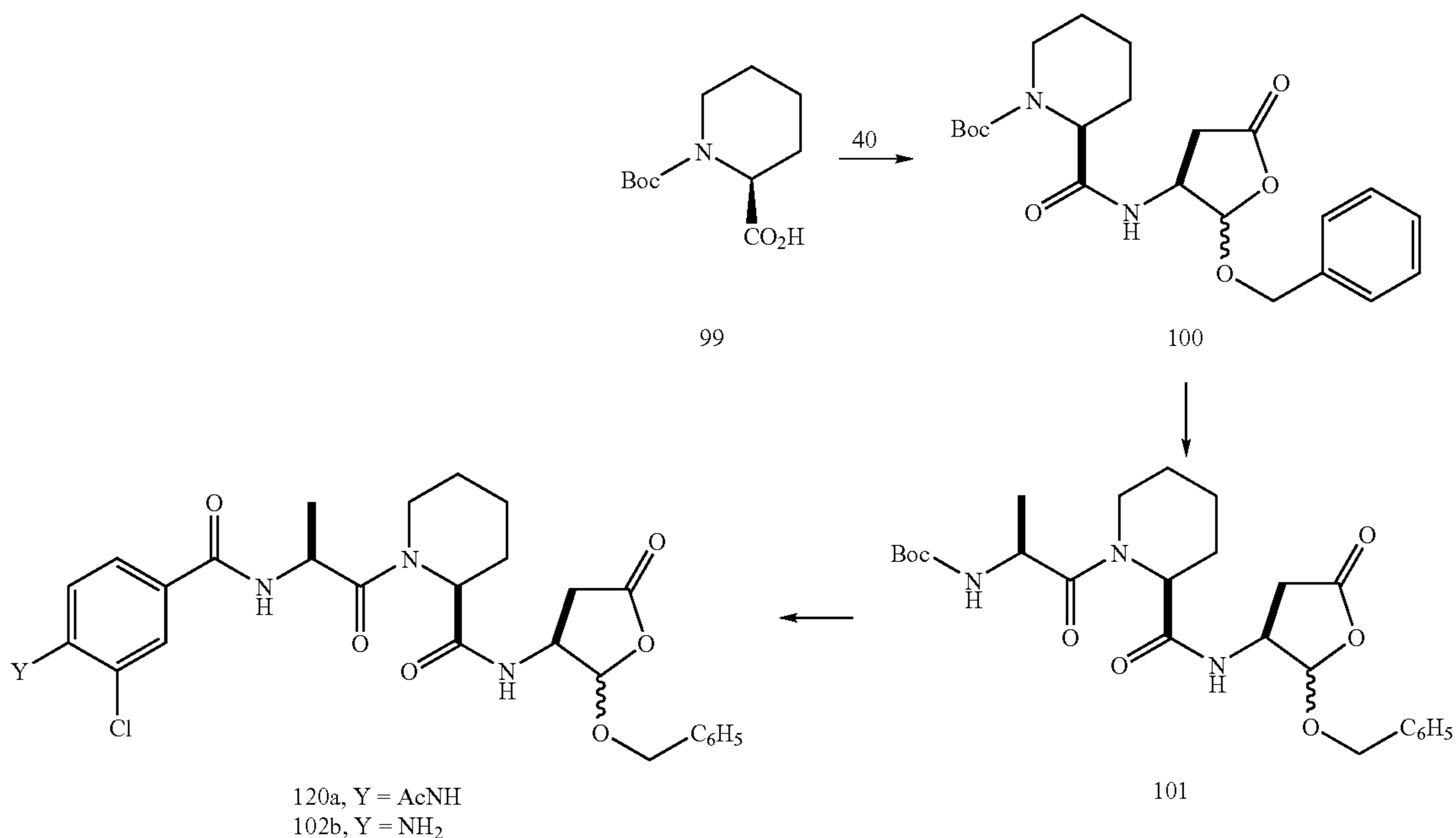
Scheme XVIII
