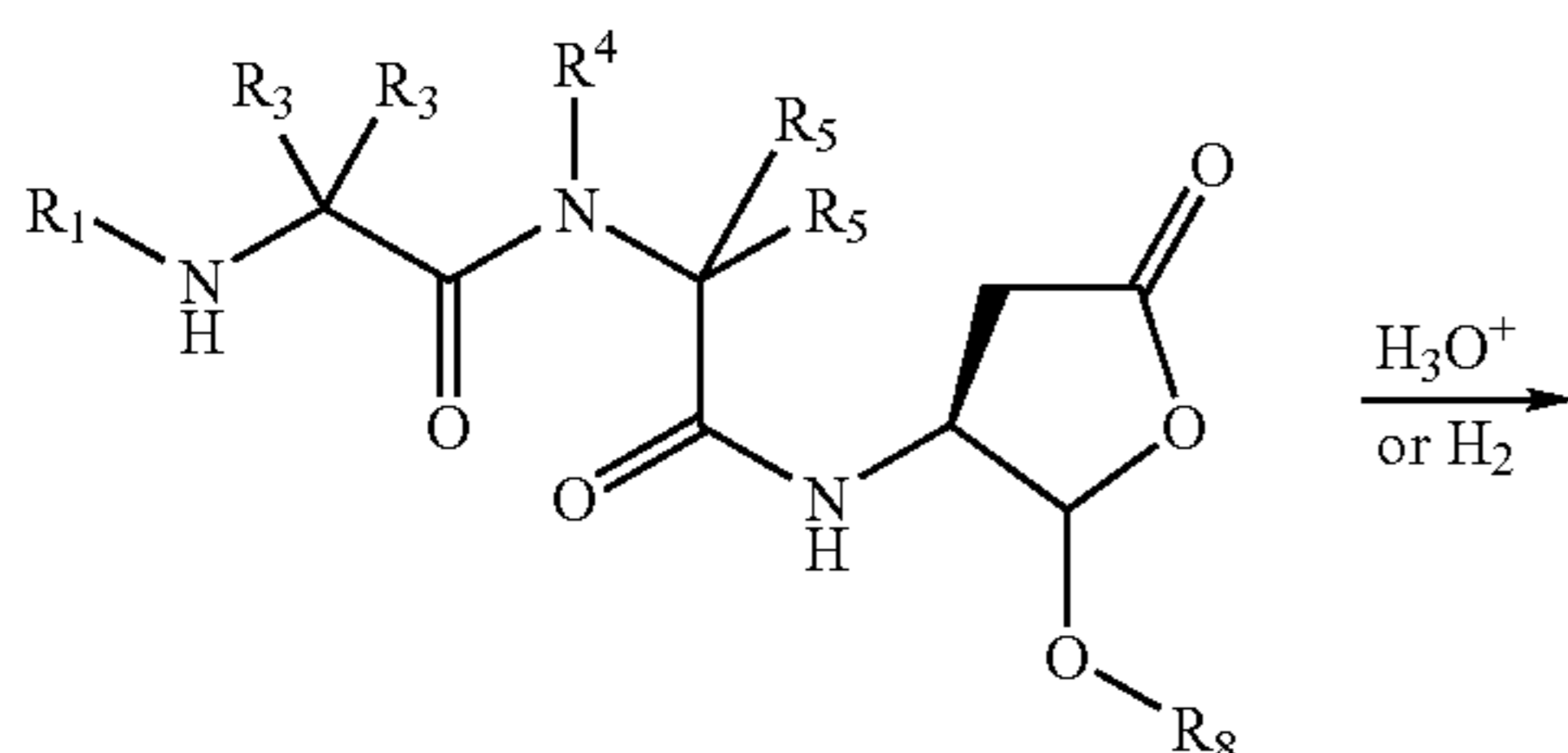
Scheme XXIII
