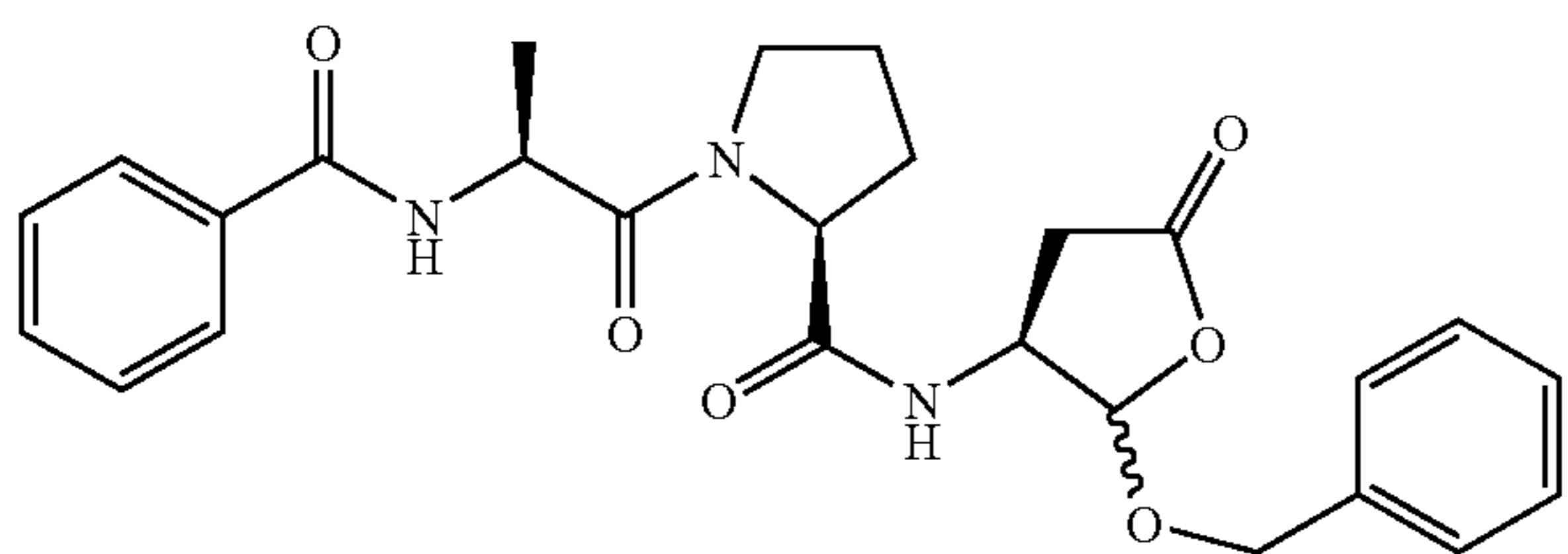
1-(2-Benzoylamino-propionyl)-pyrrolidine-2-carboxylic acid (2-benzyloxy-5-oxo-tetrahydro-furan-3-yl)-amide (84)
