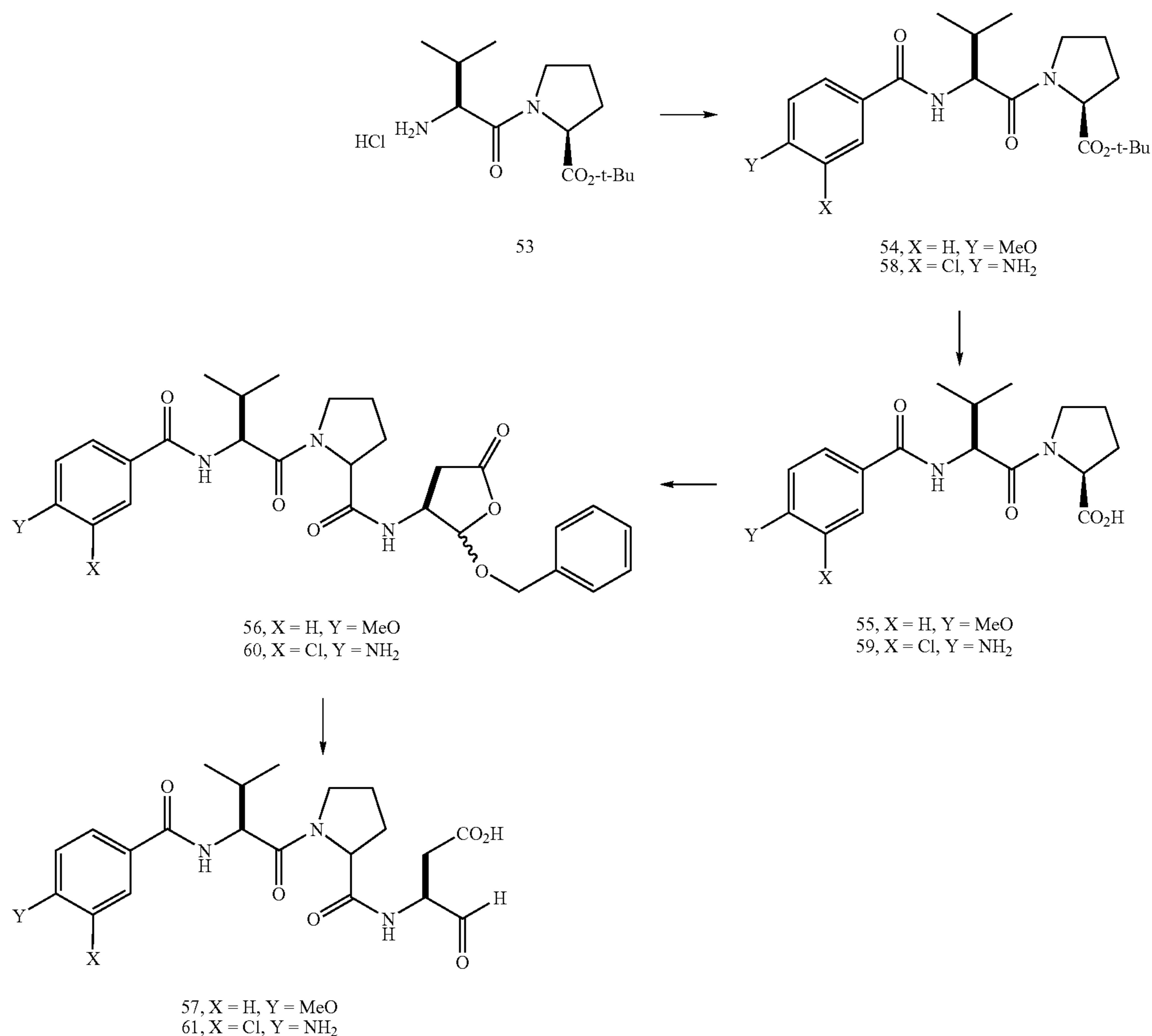
Scheme XII
