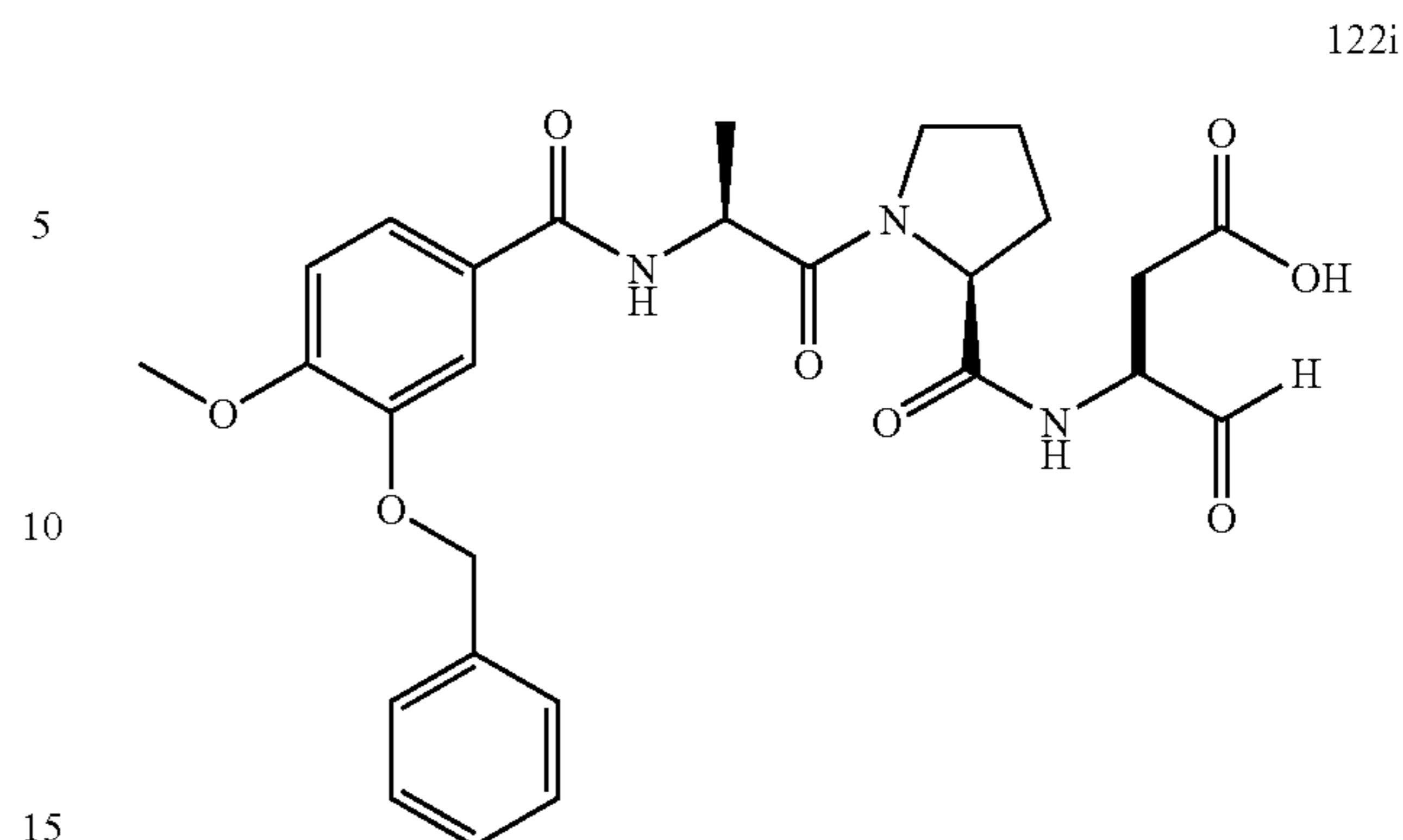
3-({1-[2-(3-benzyloxy-4-methoxy-benzoylamino)-propionyl]-pyrrolidine-2-carbonyl}-amino)-4-oxo-butyrinic acid (122i)
