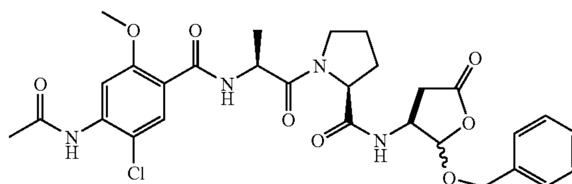
1-[2-(4-Acetylamino-5-chloro-2-methoxy-benzoylamino)-propionyl]-pyrrolidine-2-carboxylic acid (2-benzyloxy-5-oxo-tetrahydro-furan-3-yl)-amide (87)
