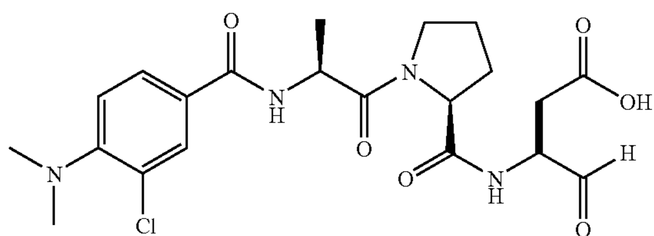
3-({1-[2-(3-Chloro-4-dimethylamino-benzoylamino)-propionyl]-pyrrolidine-2-carbonyl}-amino)-4-oxo-butyric acid (122m)
