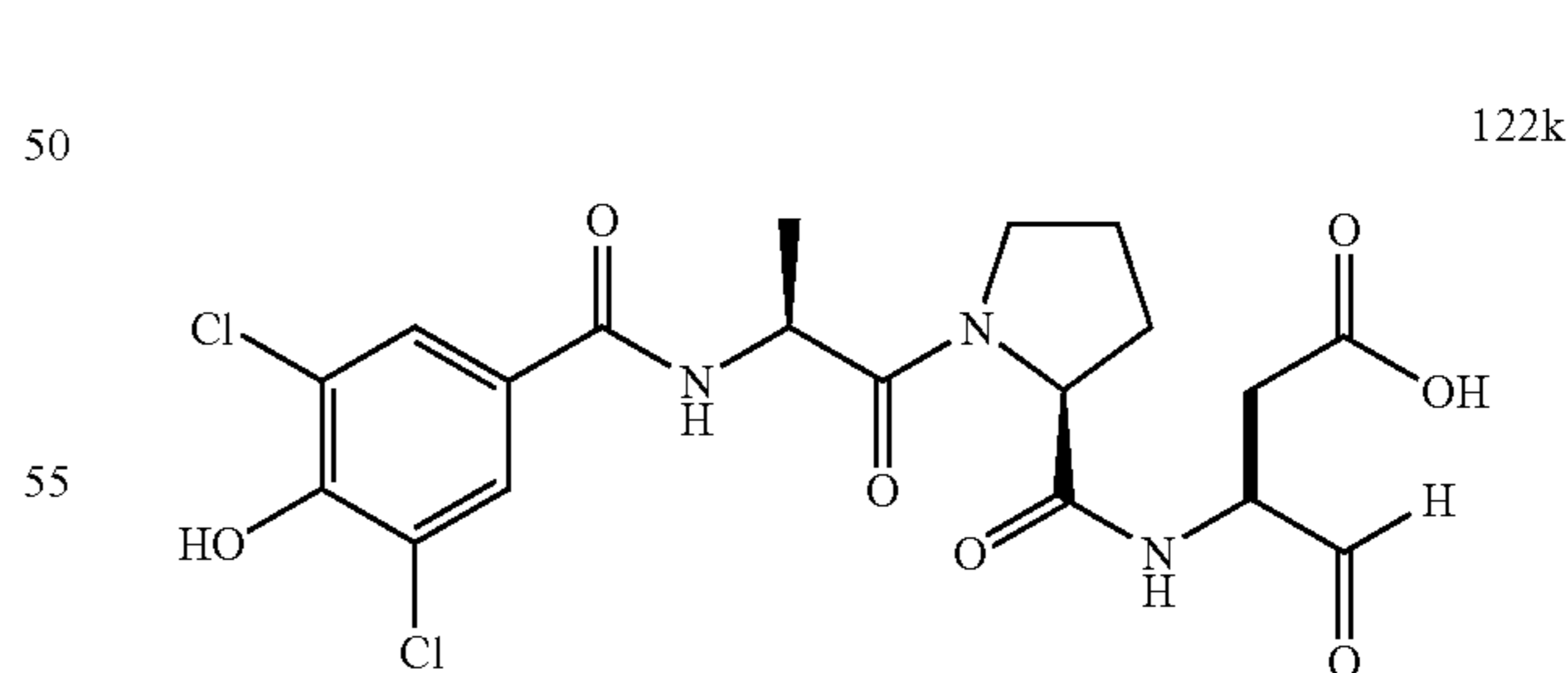
3-({1-[2-(3,5-Dichloro-4-hydroxy-benzoylamino)-propionyl]-pyrrolidine-2-carbonyl}-amino)-4-oxo-butyrinic acid (122k)
