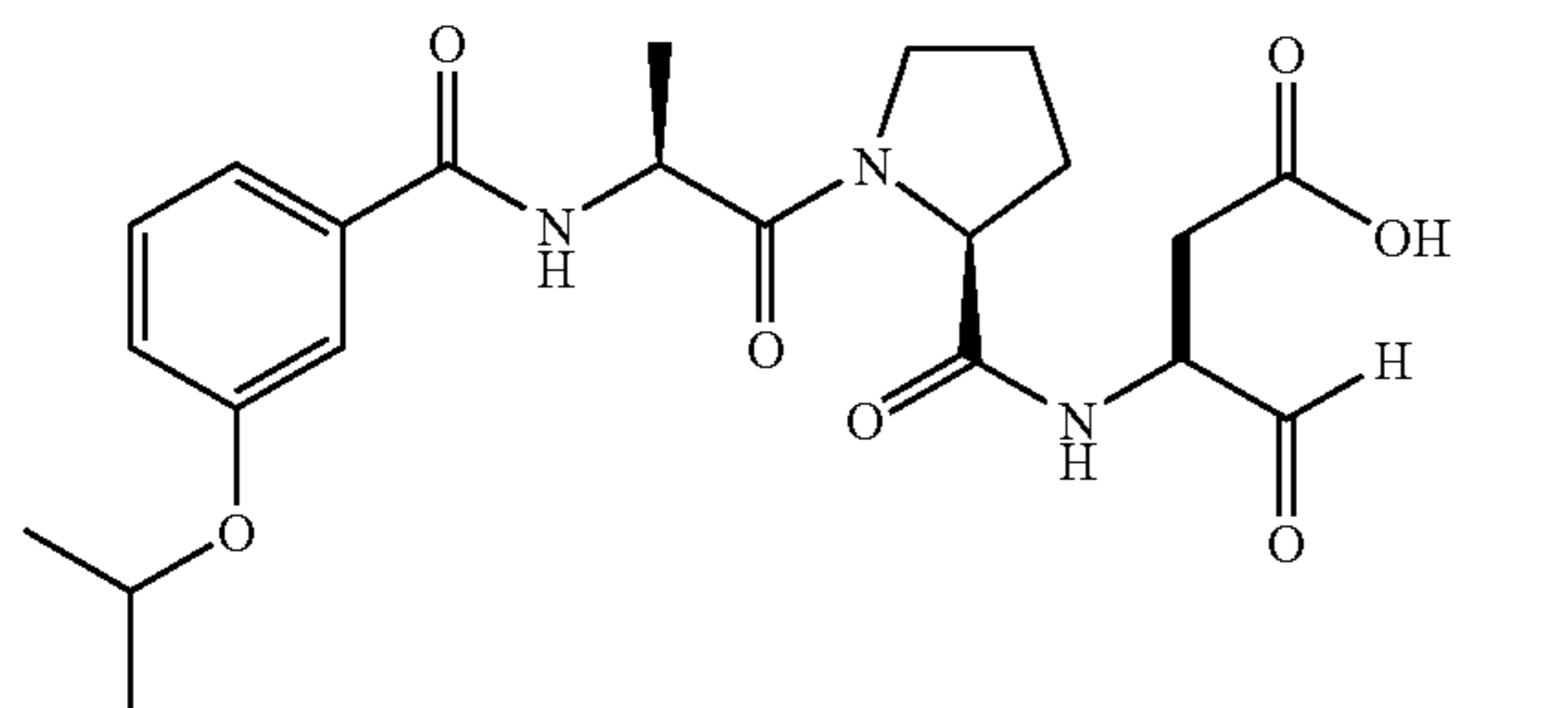
3-({1-[2-(3-Isopropoxy-benzoylamino)-propionyl]-pyrrolidine-2-carbonyl}-amino)-4-oxo-butyrinic acid (122h)
