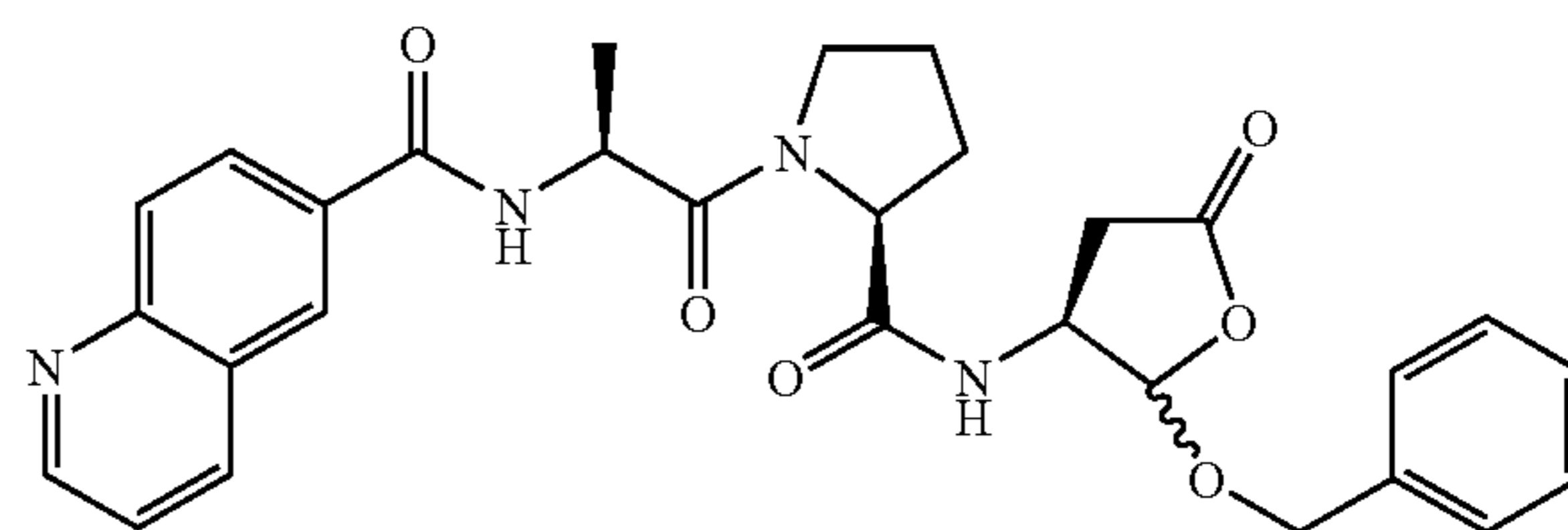
Quinoline-6-carboxylic acid {2-(2-benzyloxy-5-oxo-tetrahydro-furan-3-ylcarbamoyl)-pyrrolidin-1-yl}-1-methyl-2-oxo-ethyl}-amide (93)
