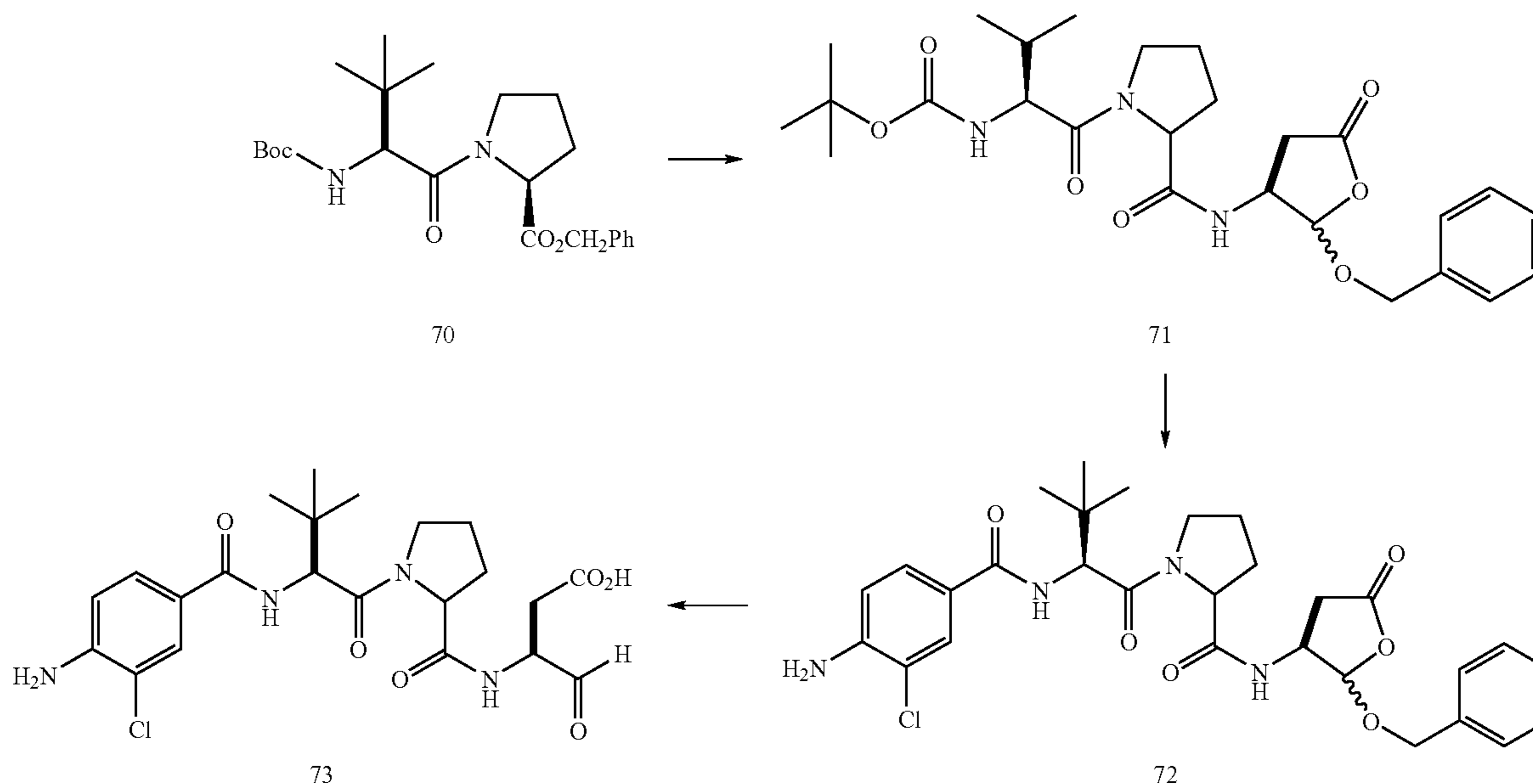
Scheme XV
