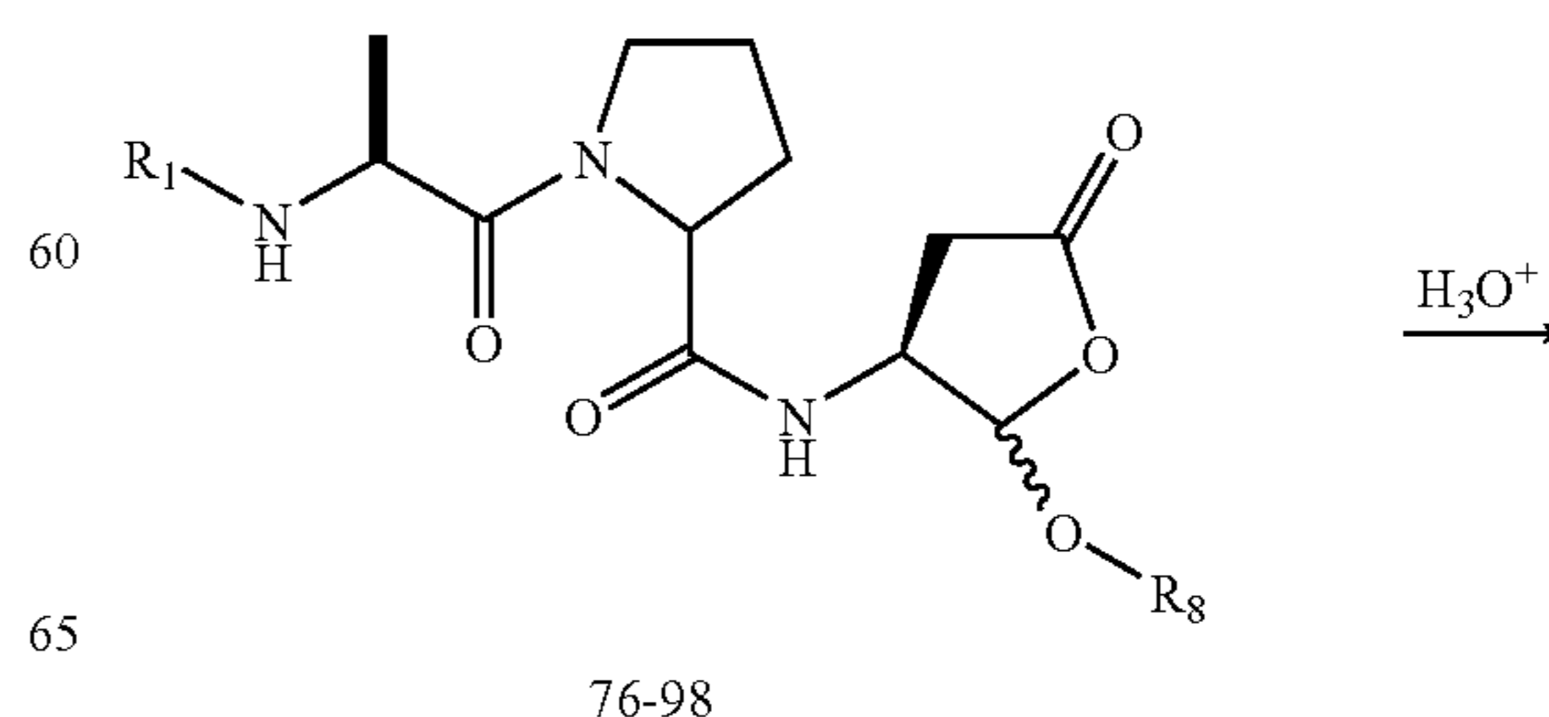
Scheme XXIV
