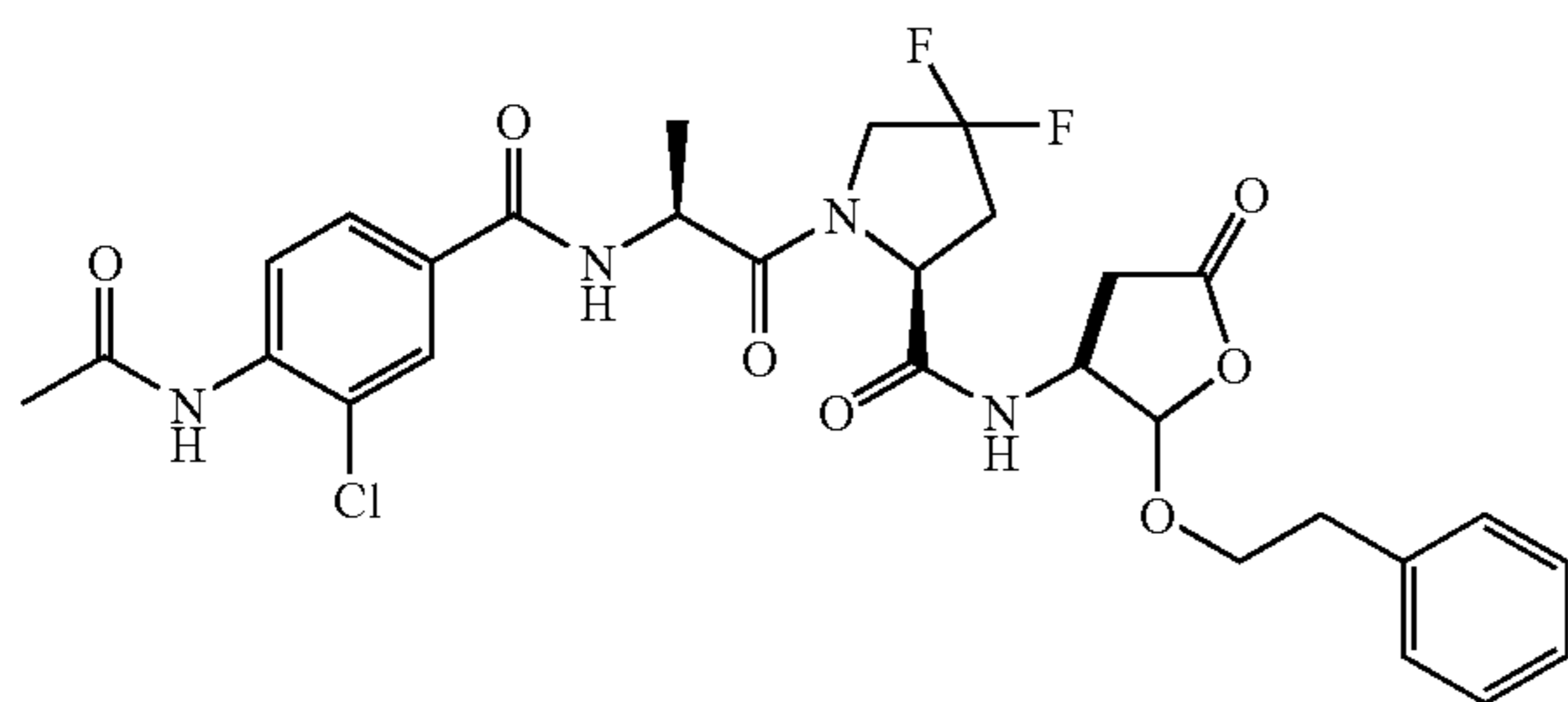
1-[2-(4-Acetylamino-3-chloro-benzoylamino)-propionyl]-4,4-difluoro-pyrrolidine-2-carboxylic acid (2-phenylethoxy-5-oxo-tetrahydro-furan-3-yl)-amide (116h)
