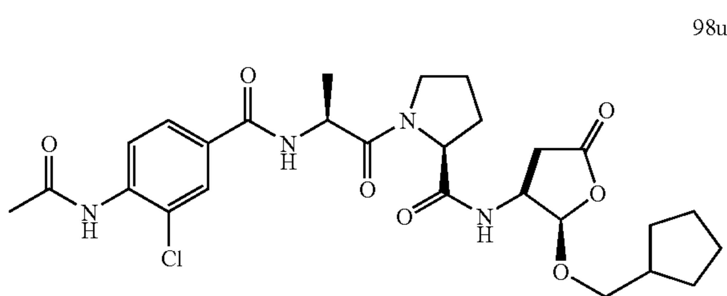
Synthesis of 1-[2-(4-acetylamino-3-chloro-benzoylamino)-propionyl]-pyrrolidine-2-carboxylic acid (2-cyclopentylmethoxy-5-oxo-tetrahydro-furan-3-yl)-amide (98u)
