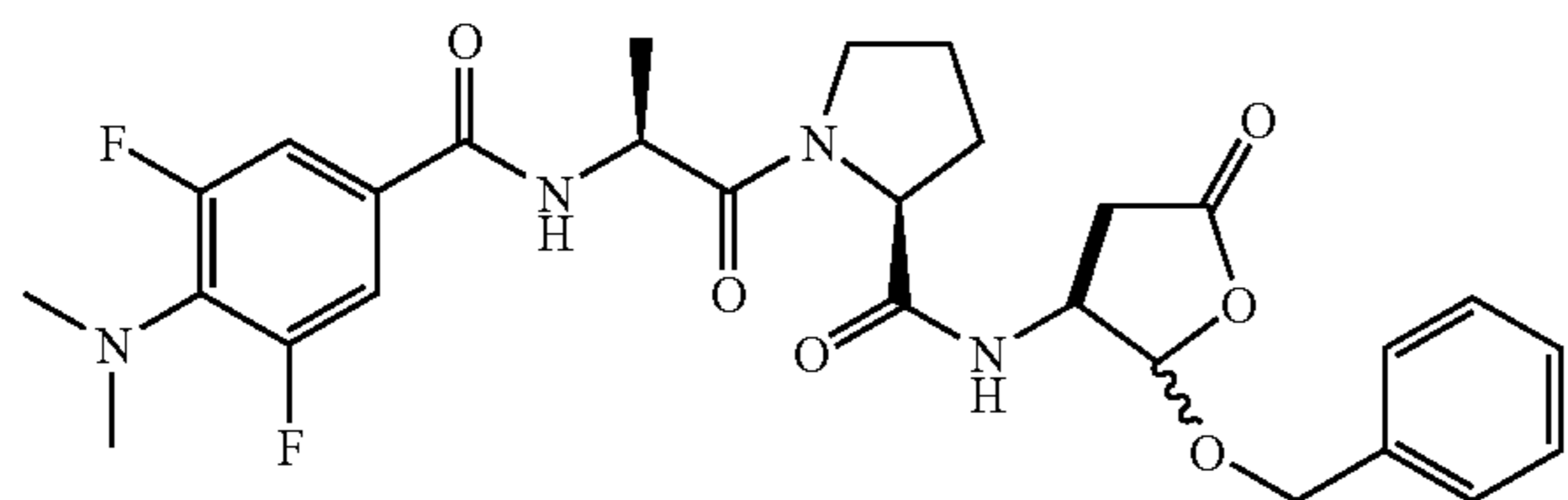
1-[2-(4-dimethylamino-3,5-difluoro-benzoylamino)-propionyl]-pyrrolidine-2-carboxylic acid (2-benzyloxy-5-oxo-tetrahydro-furan-3-yl)-amide (98y)
