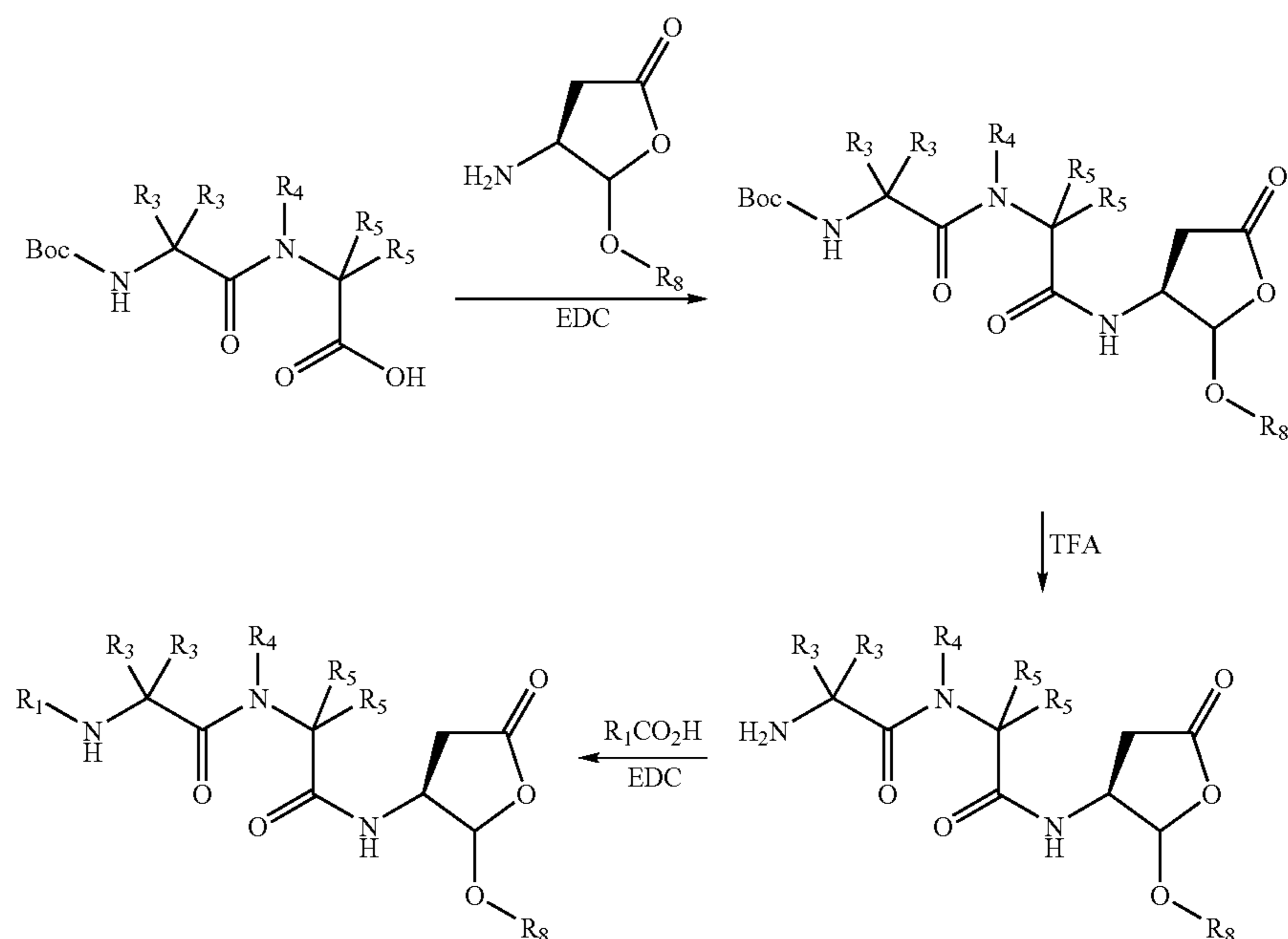
Scheme IX
