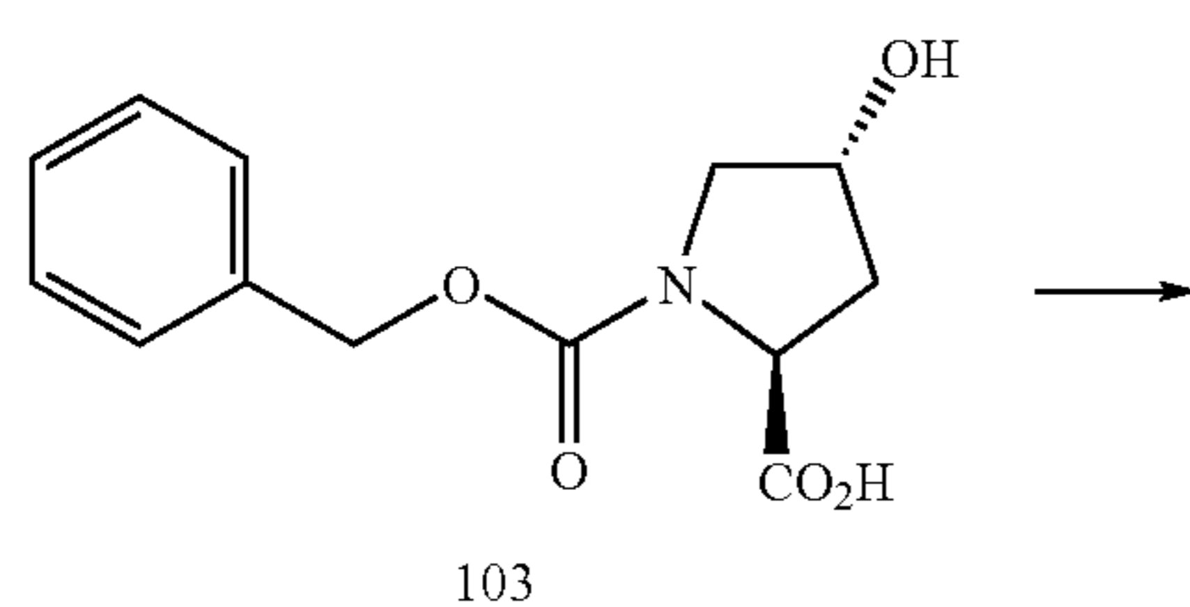
Scheme XIX
