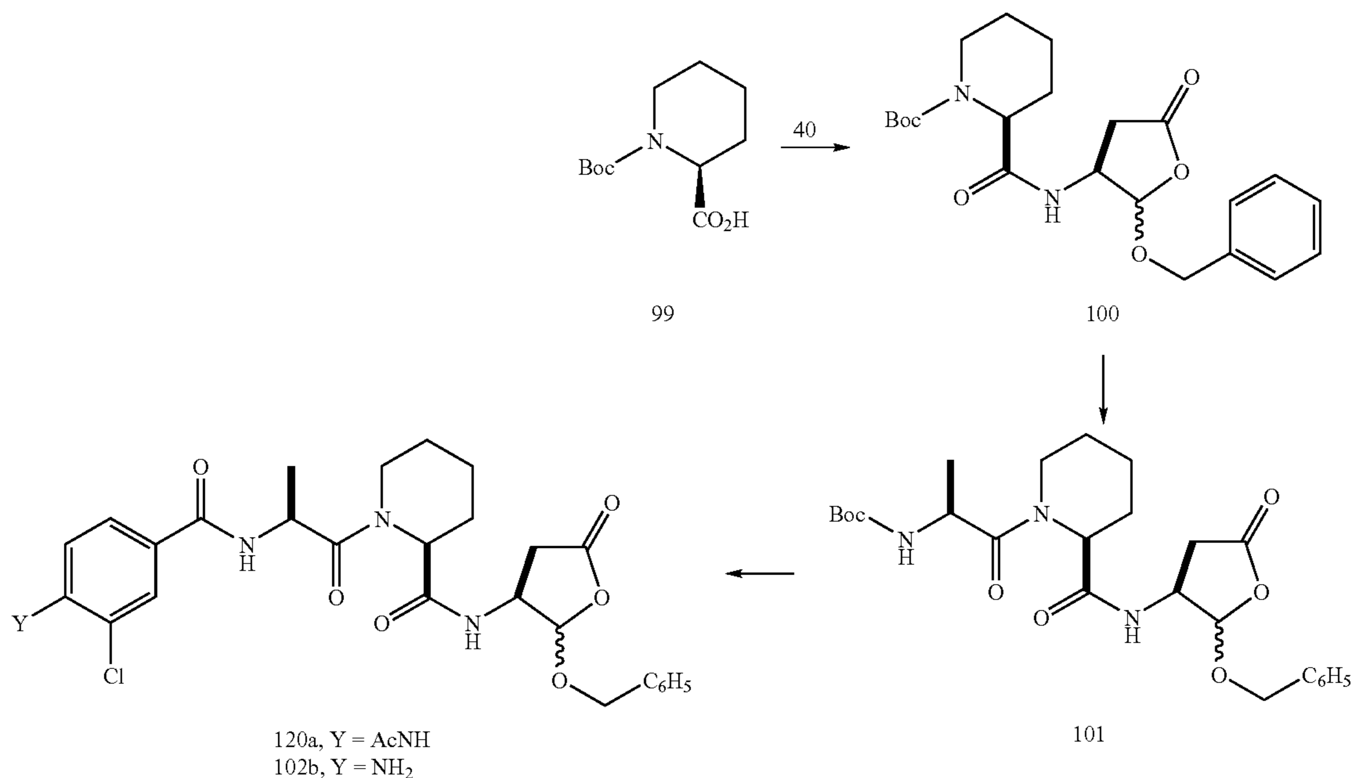
Scheme XVIII
