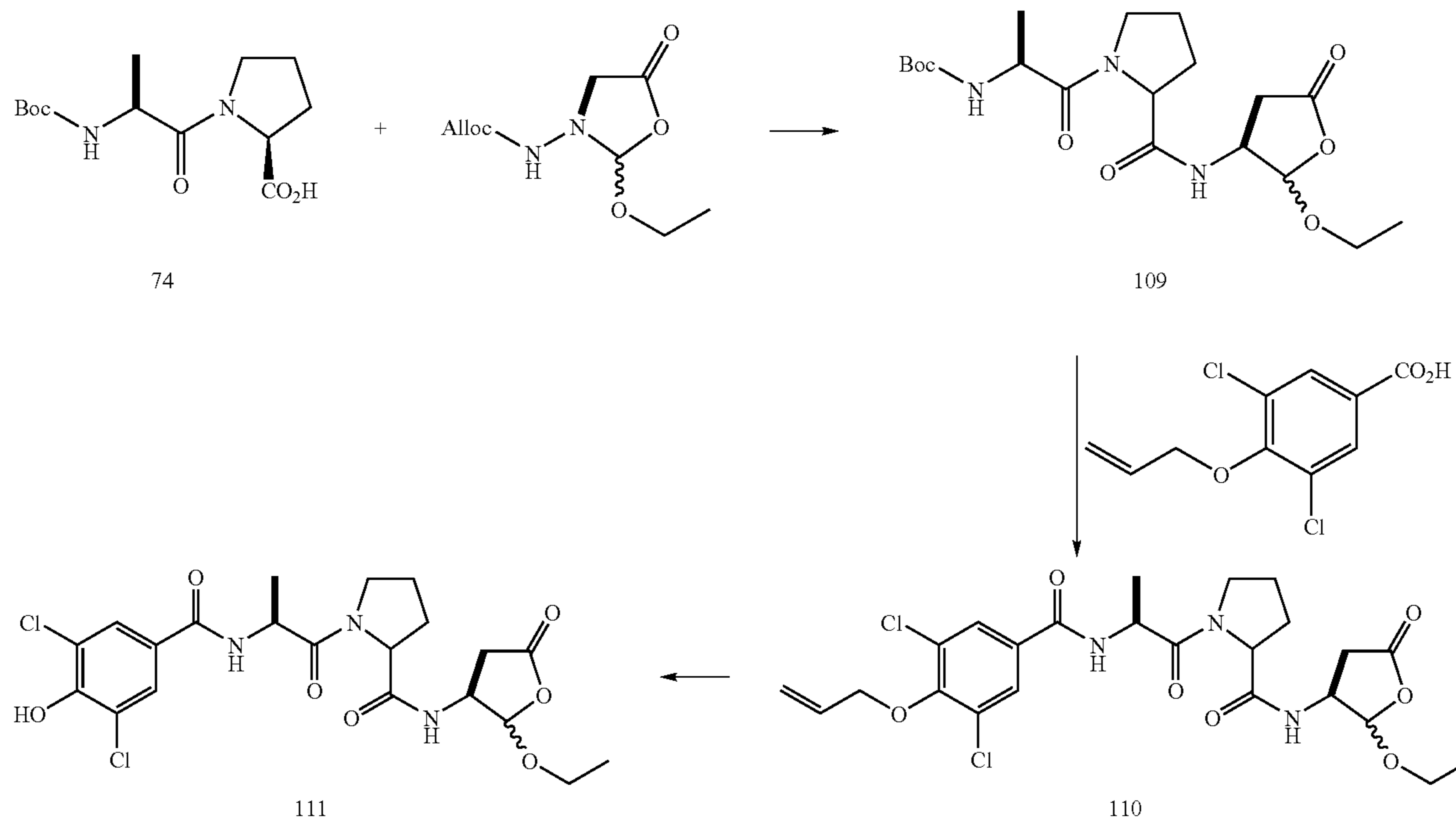
Scheme XX
