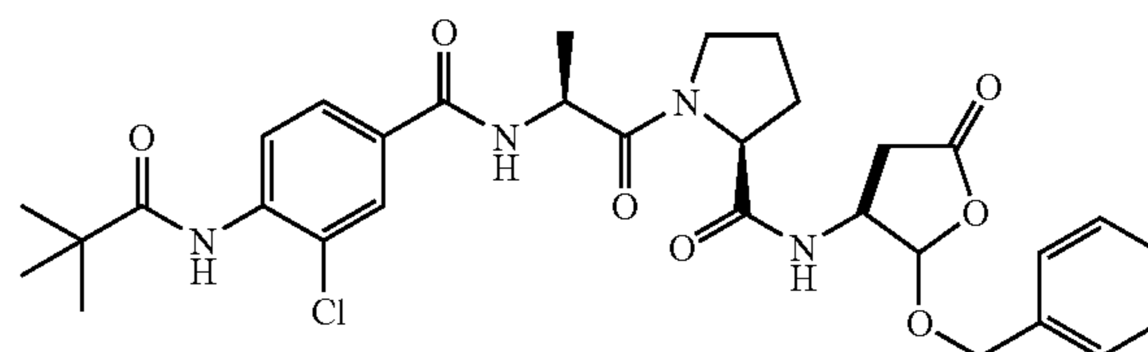
1-{2-[3-chloro-4-(2,2-dimethylpropionylamino)-benzoylamino]-propionyl}-pyrrolidine-2-carboxylic acid (2-benzyloxy-5-oxo-tetrahydro-furan-3-yl)-amide (98aa)
