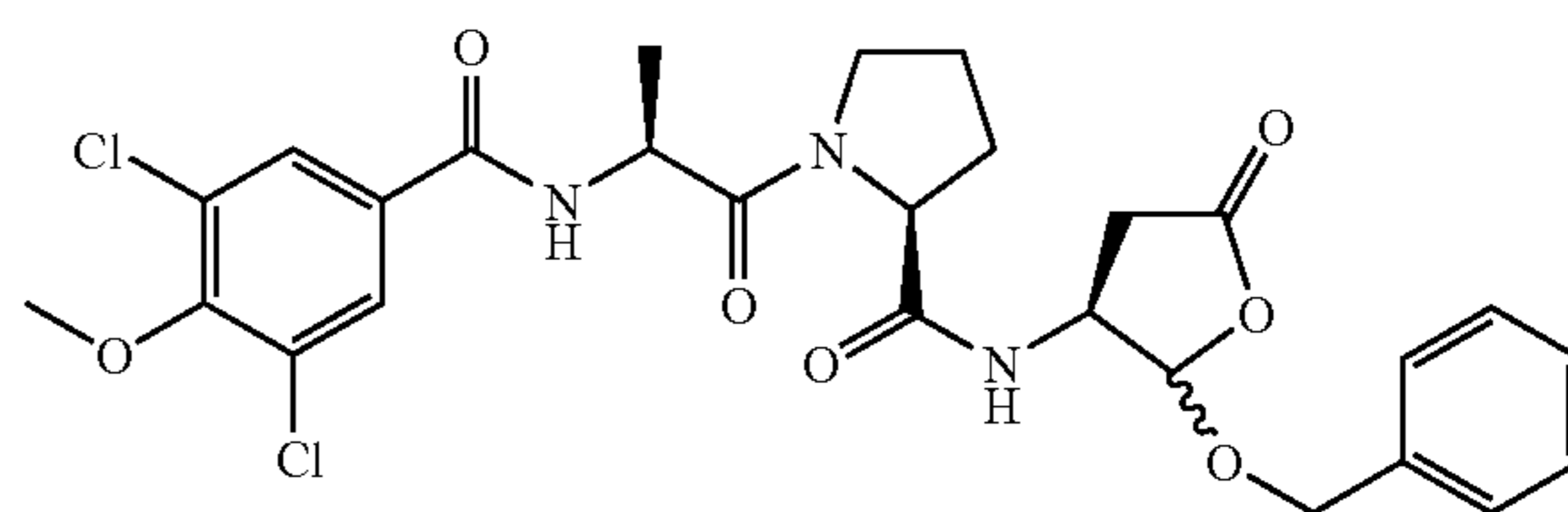
1-[2-(3,5-Dichloro-4-methoxy-benzoylamino)-propionyl]-pyrrolidine-2-carboxylic acid (2-benzyloxy-5-oxo-tetrahydro-furan-3-yl)-amide (92)
