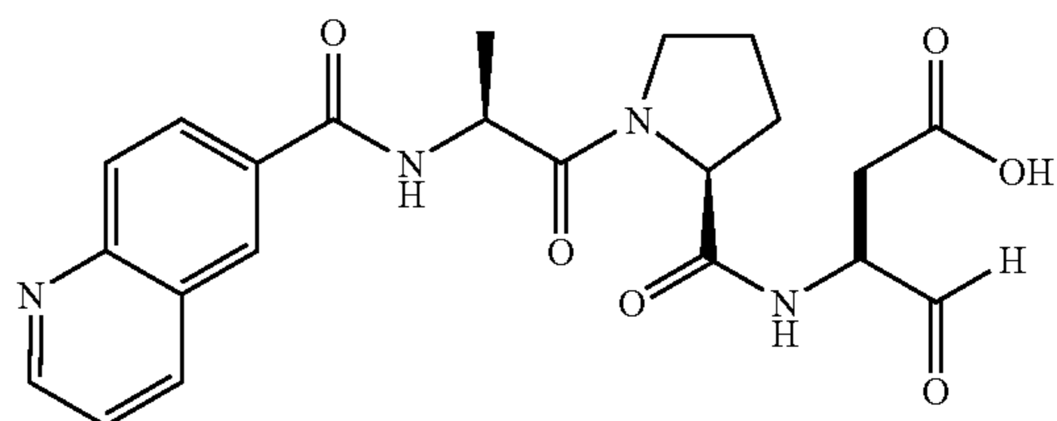
4-Oxo-3-[(1-{2-[(quinoline-6-carbonyl)-amino]-propionyl}-pyrrolidine-2-carbonyl)-amino]-butyric acid (122q)
