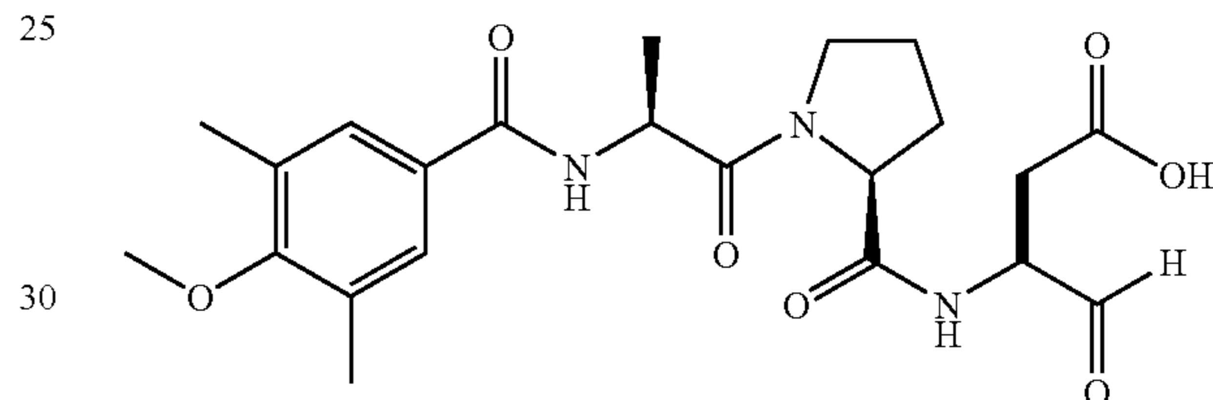
4-Oxo-3-[(1-{2-[9-oxo-9H-fluorene-4-carbonyl]-amino]-propionyl}-pyrrolidine-2-carbonyl)-amino]-butyrac acid (122a)
