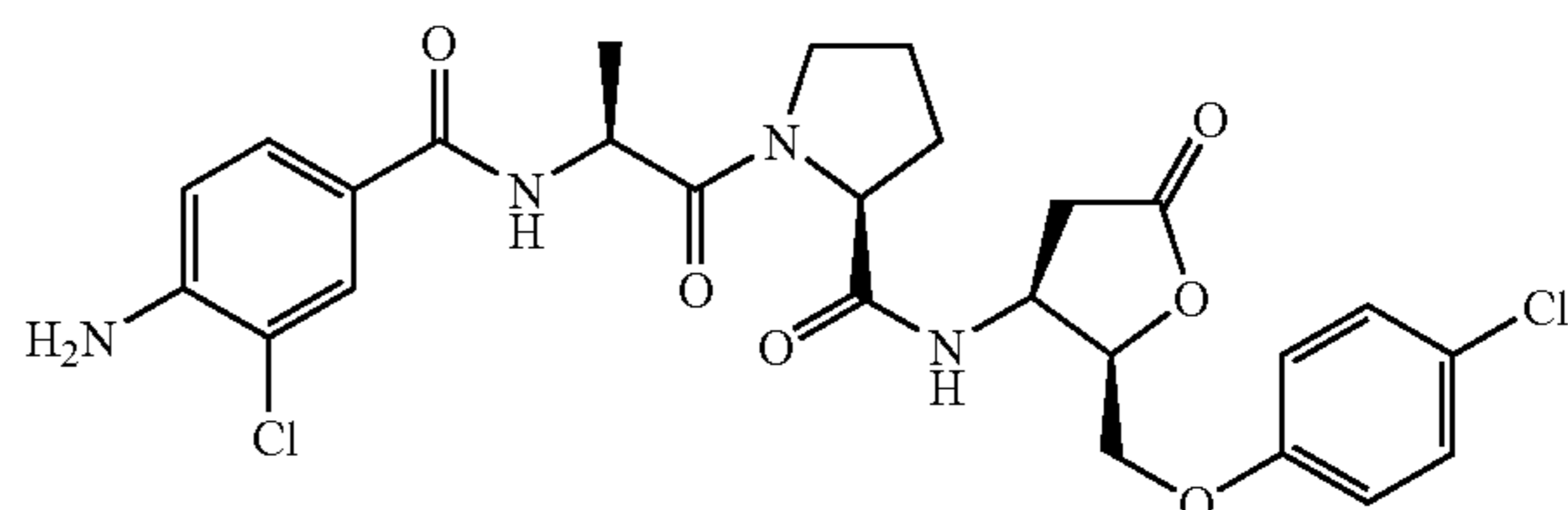
[2-(4-Chloro-benzyloxy)-5-oxo-tetrahydro-furan-3-yl]-carbamic acid allyl ester
