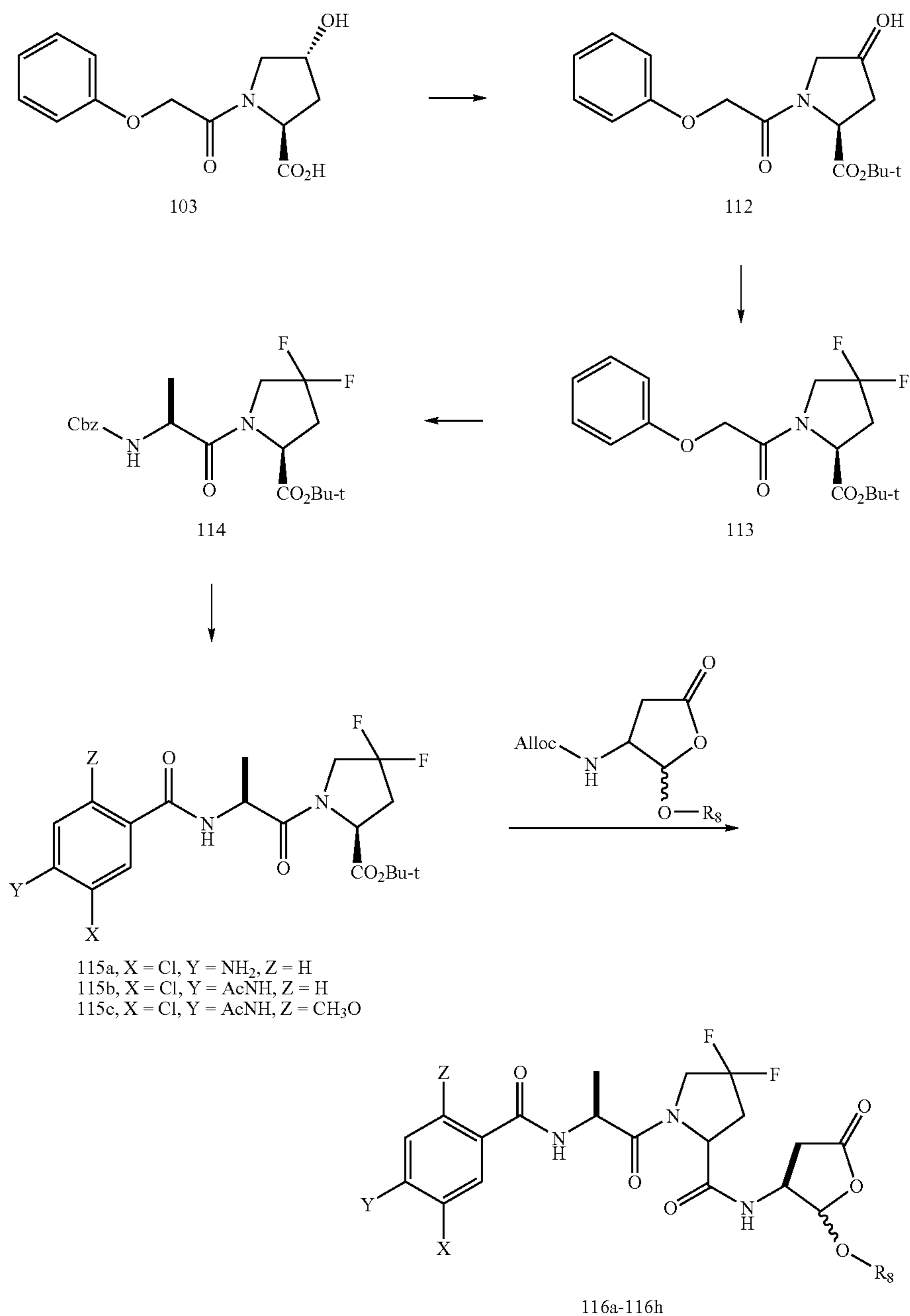
Scheme XXI
