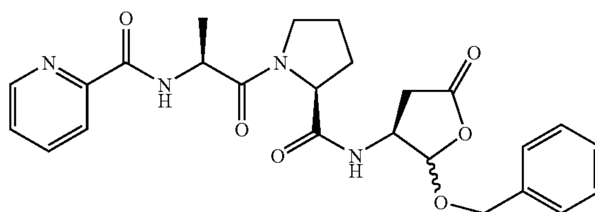
Pyridine-2-carboxylic acid {2-[2-(2-benzyloxy-5-oxo-tetrahydro-furan-3-yl)carbamoyl]-pyrrolidin-1-yl]-1-methyl-2-oxo-ethyl}-amide (88)
