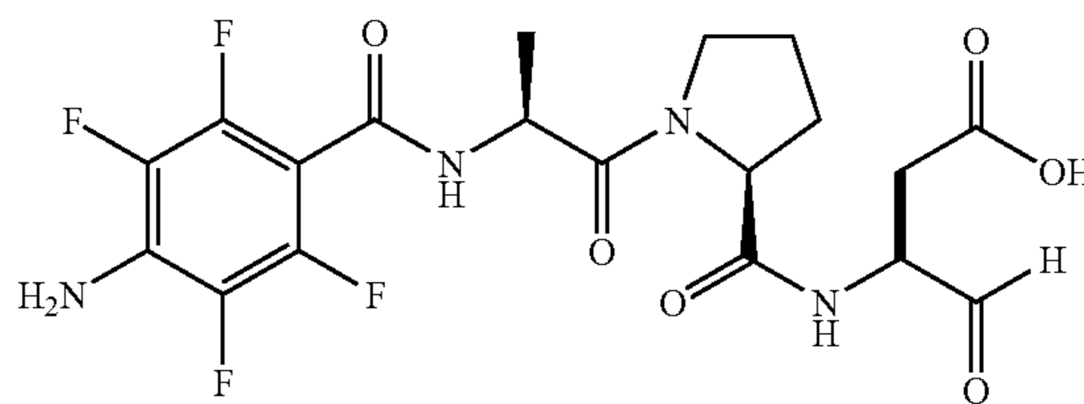
3-({1-[2-(4-Amino-2,3,5,6-tetrafluoro-benzoylamino)-propionyl]-pyrrolidine-2-carbonyl}-amino)-4-oxo-butyric acid (122p)
