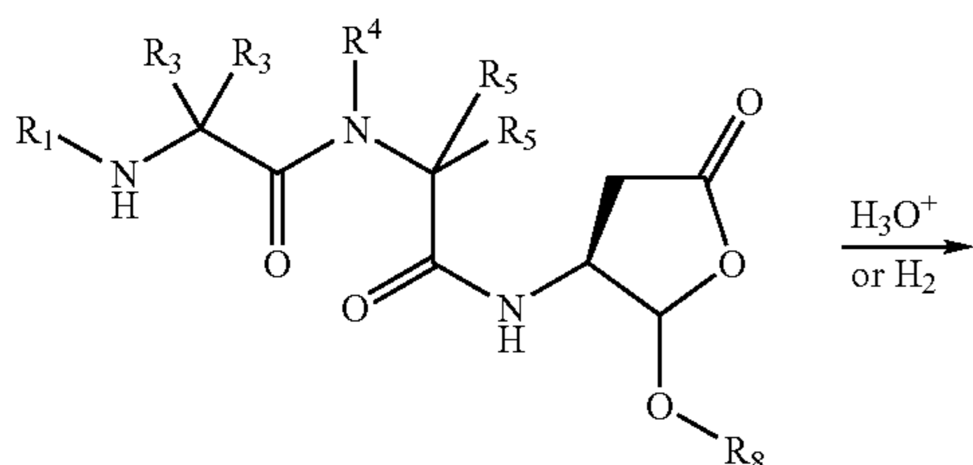
Scheme XXIII
