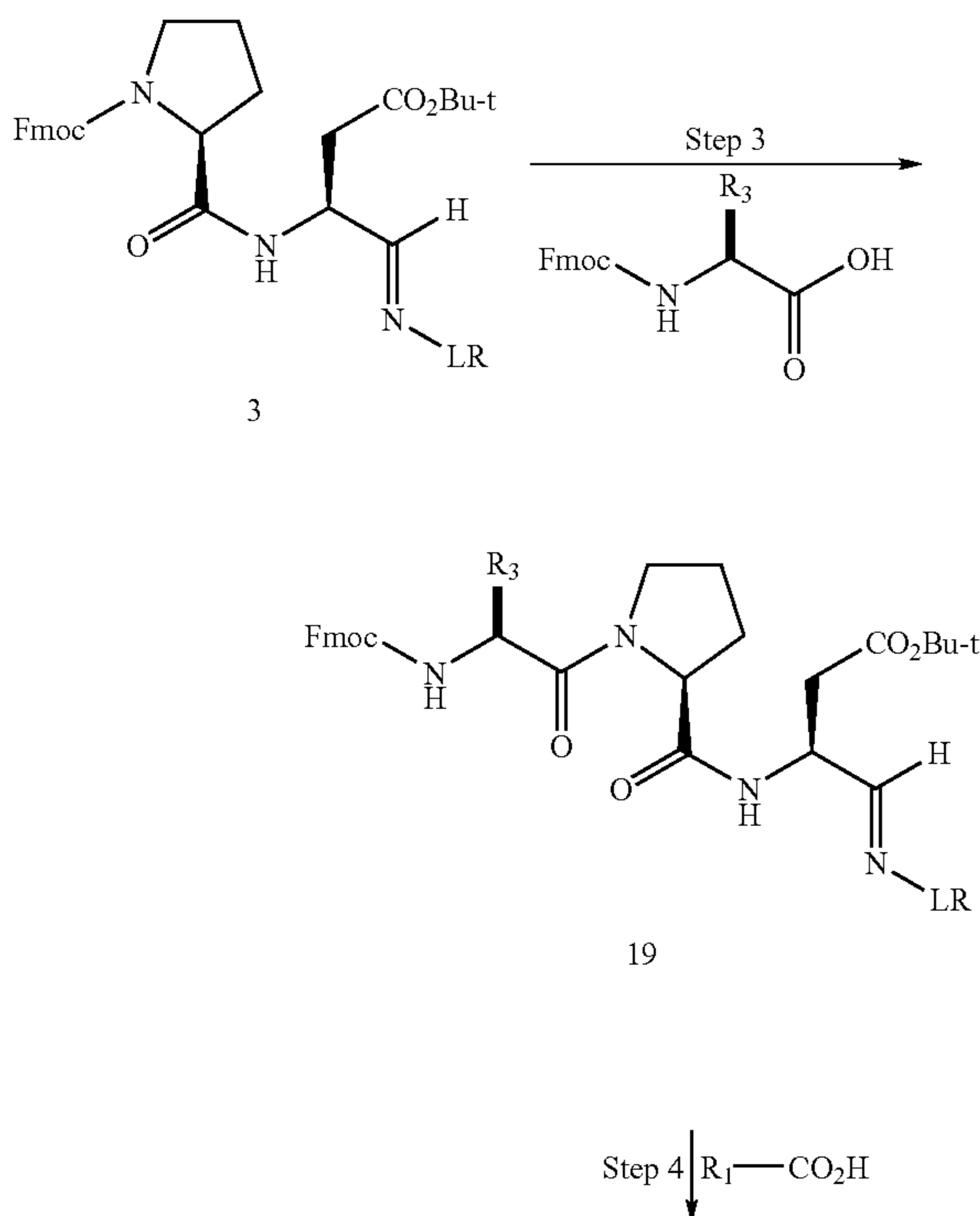
Scheme V
