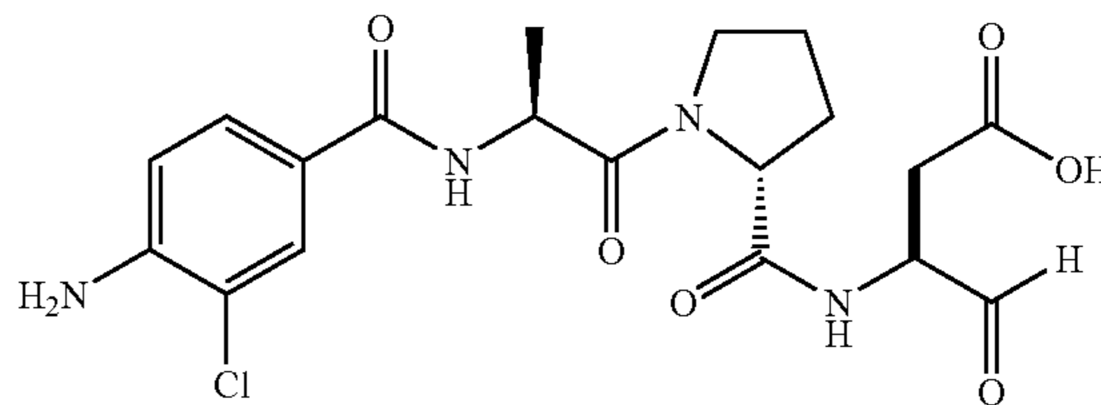
3-({1-[2-(4-Amino-3-chloro-benzoylamino)-propionyl]-pyrrolidine-2-carbonyl}-amino)-4-oxo-butyric acid (122o)
