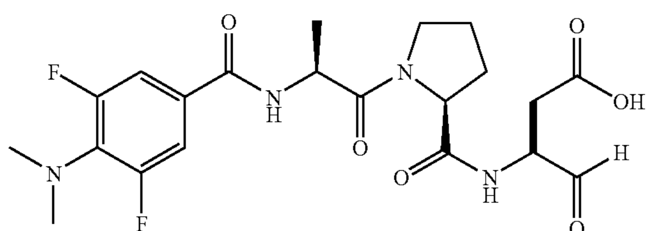
3-({1-[2-(4-Dimethylamino-3,5-difluoro-benzoylamino)-propionyl]-pyrrolidine-2-carbonyl}-amino)-4-oxo-butyric acid (122n)
