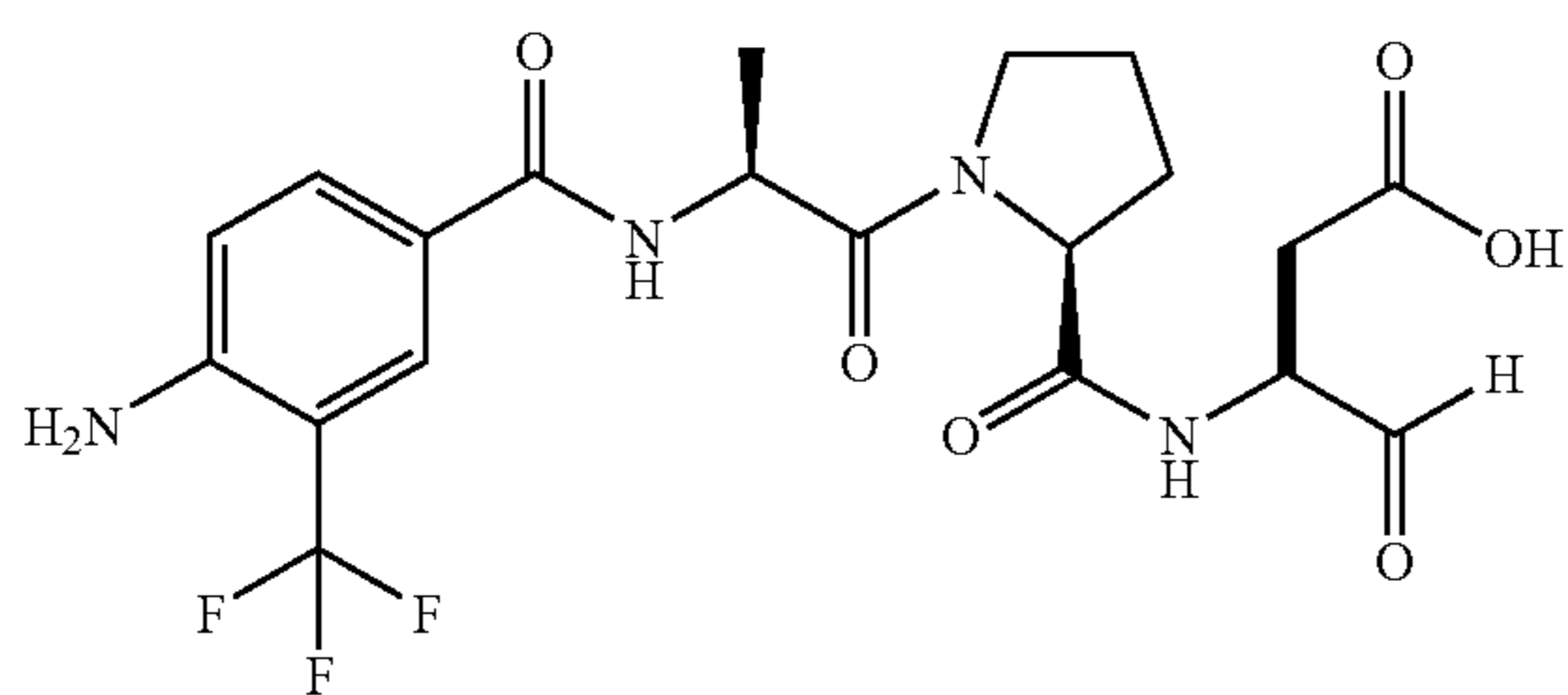
3-({1-[2-(4-Amino-3-trifluoromethyl-benzoylamino)-propionyl]-pyrrolidine-2-carbonyl}-amino)-4-oxo-butyric acid (1221)
