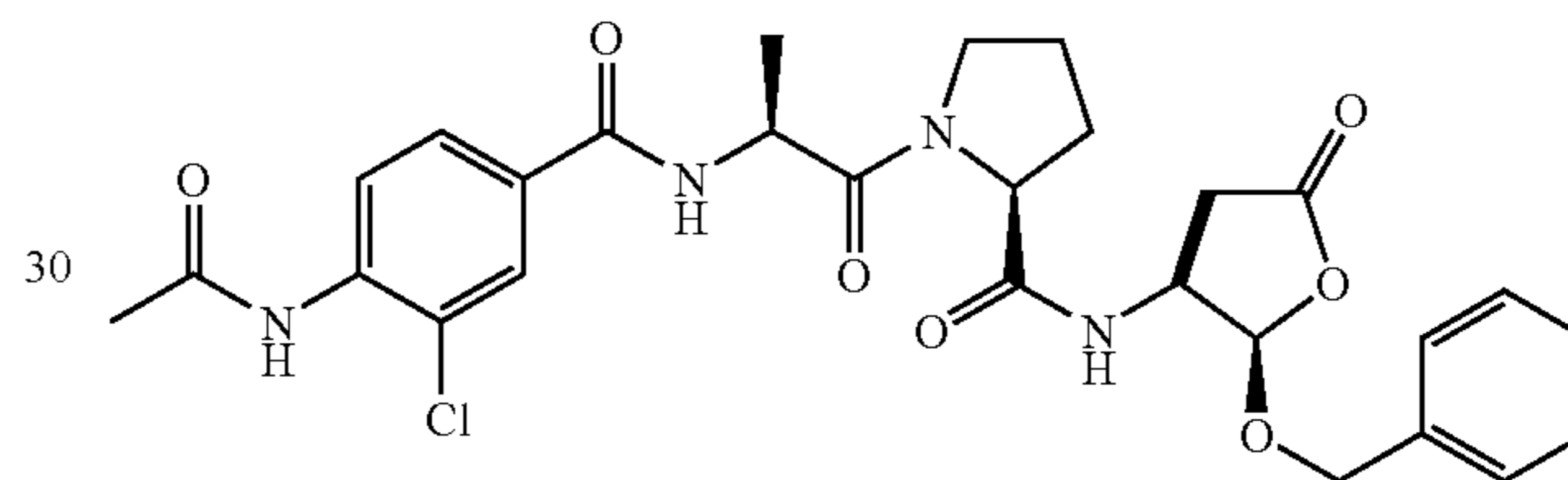
1-[2-(4-acetylamino-3-chloro-benzoylamino)-propionyl]-pyrrolidine-2-carboxylic acid (2-benzyloxy-5-oxo-tetrahydro-furan-3-yl)-amide (98n)
