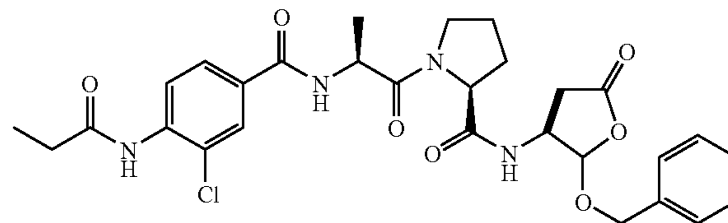
1-[2-(3-chloro-4-propionylamino)-benzoylamino]-propionyl]-pyrrolidine-2-carboxylic acid (2-benzyloxy-5-oxo-tetrahydro-furan-3-yl)-amide (98ab)
