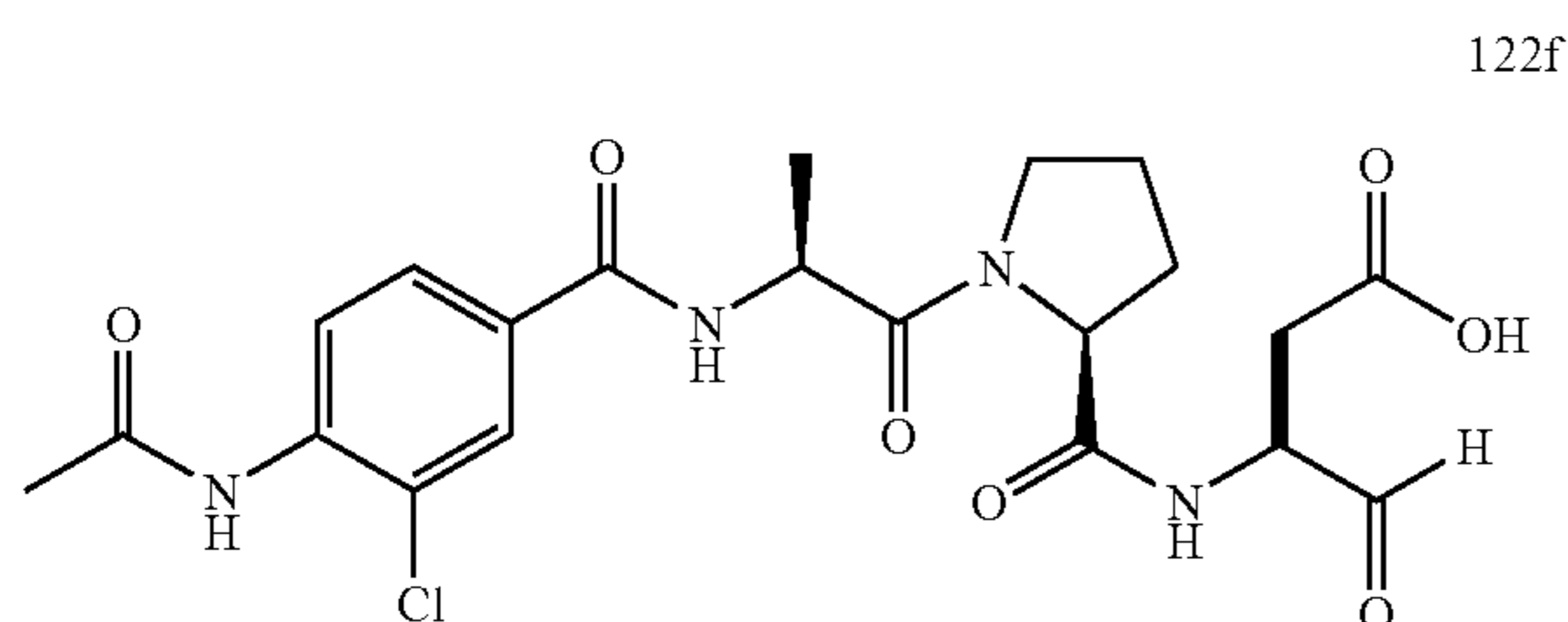
3-({1-[2-(4-Acetylamino-3-chloro-benzoylamino)-propionyl]-pyrrolidine-2-carbonyl}-amino)-4-oxo-butyrinic acid (122f)
