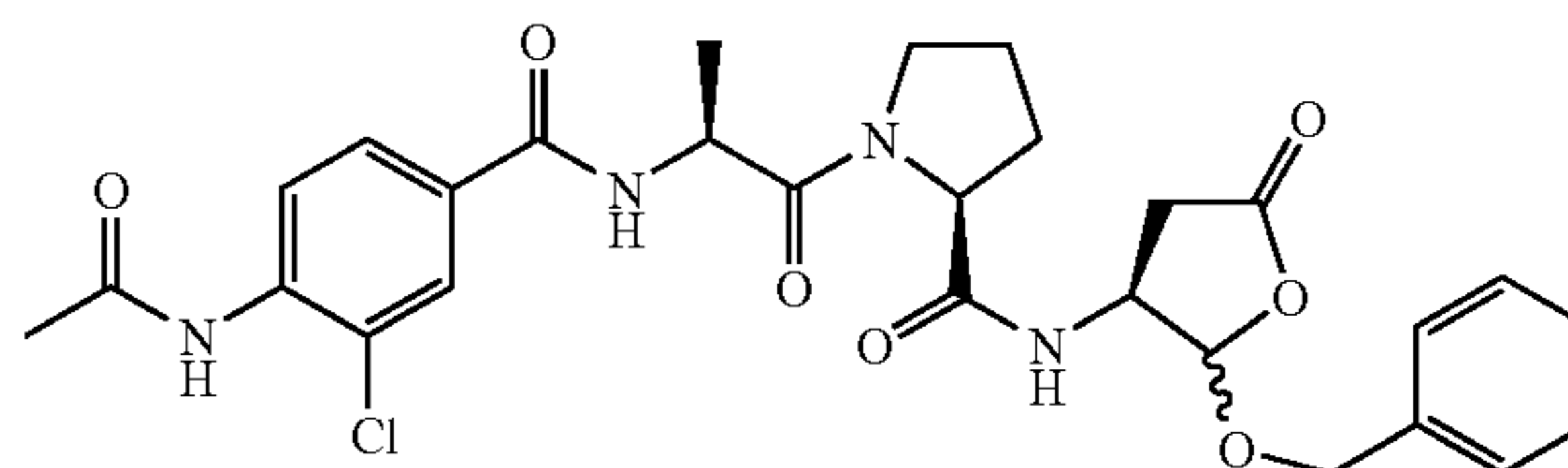
1-[2-(4-Acetylamino-3-chloro-benzoylamino)-propionyl]-pyrrolidine-2-carboxylic acid (2-benzyloxy-5-oxo-tetrahydro-furan-3-yl)-amide (78)
