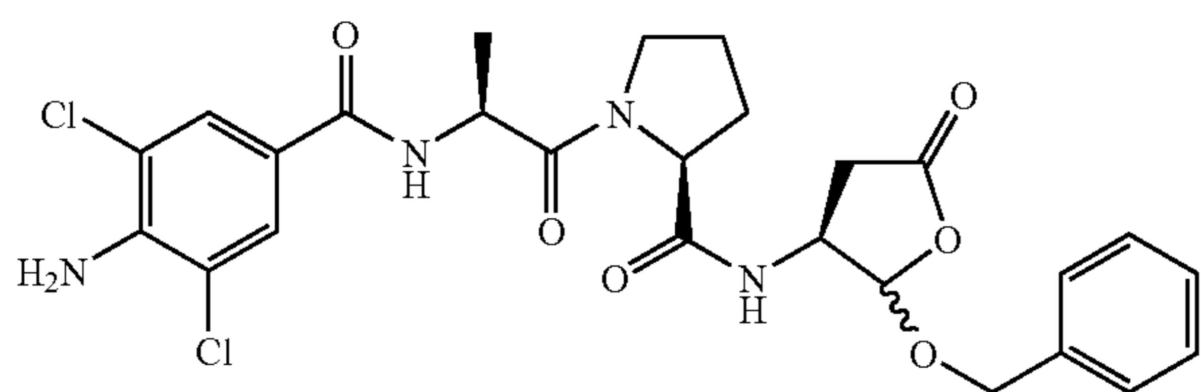
[1-[2-(4-Amino-3,5-dichloro-benzoylamino)-propionyl]-pyrrolidine-2-carboxylic acid (2-benzyloxy-5-oxo-tetrahydro-furan-3-yl)-amide] (89)
