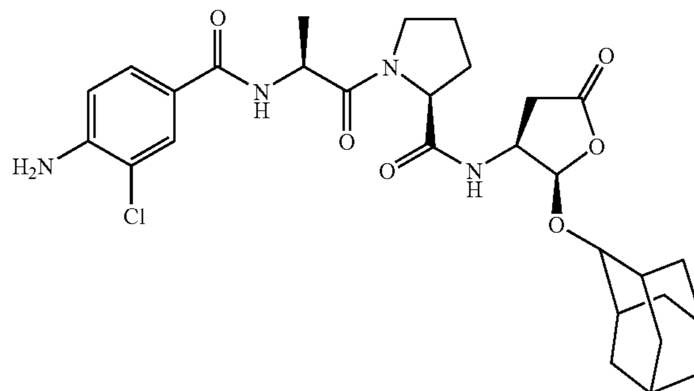
[5-Oxo-2-(tricyclo[3.3.1.1 o,o ]dec-2-yloxy)-tetrahydro-furan-3-yl]-carbamic acid allyl ester
