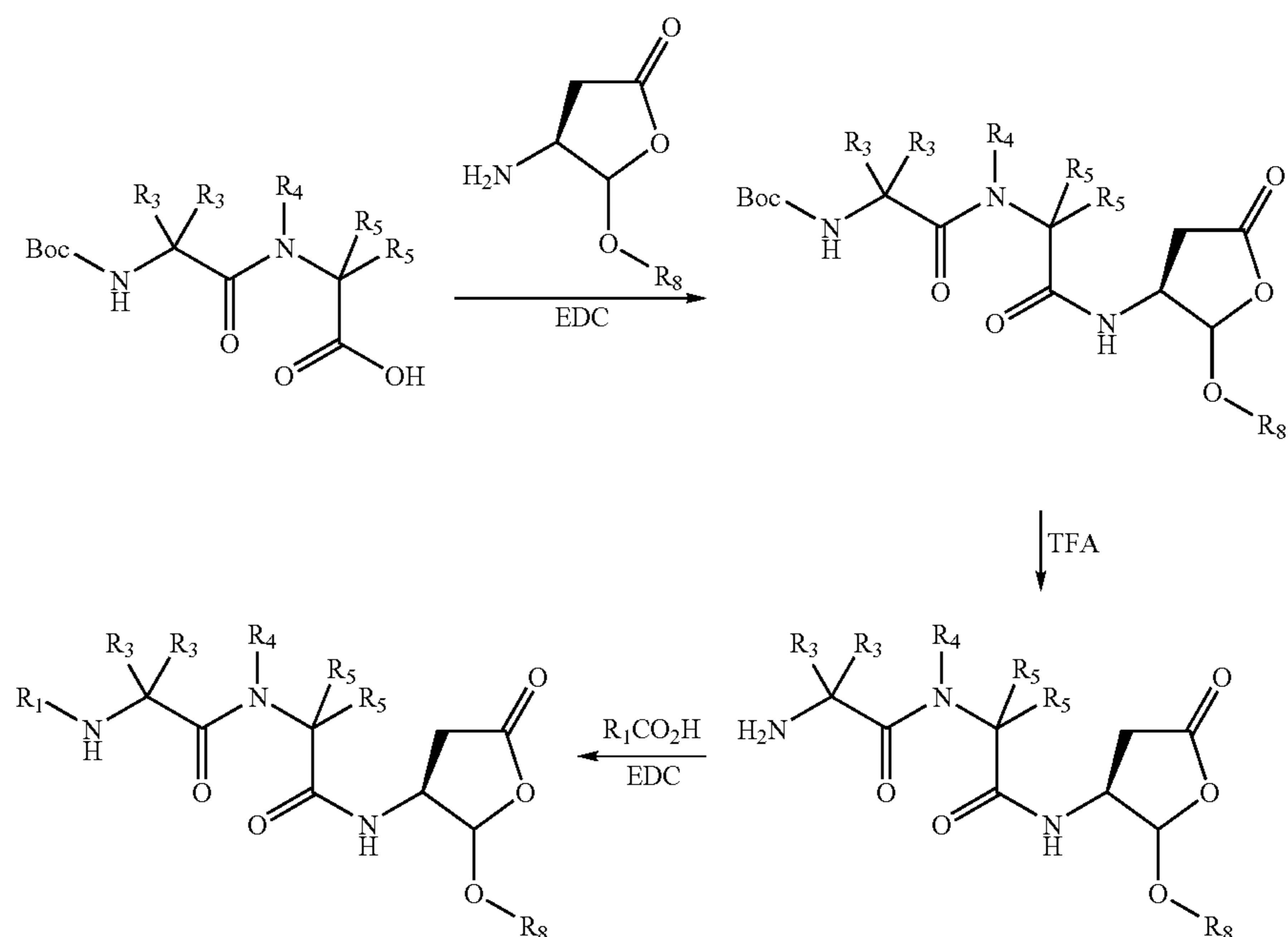
Scheme IX
