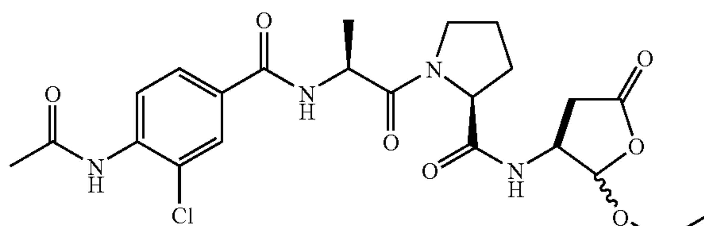
1-[2-(4-Acetylamino-3-chloro-benzoylamino)-propionyl]-pyrrolidine-2-carboxylic acid (2-ethoxy-5-oxo-tetrahydro-furan-3-yl)-amide (98ay)
