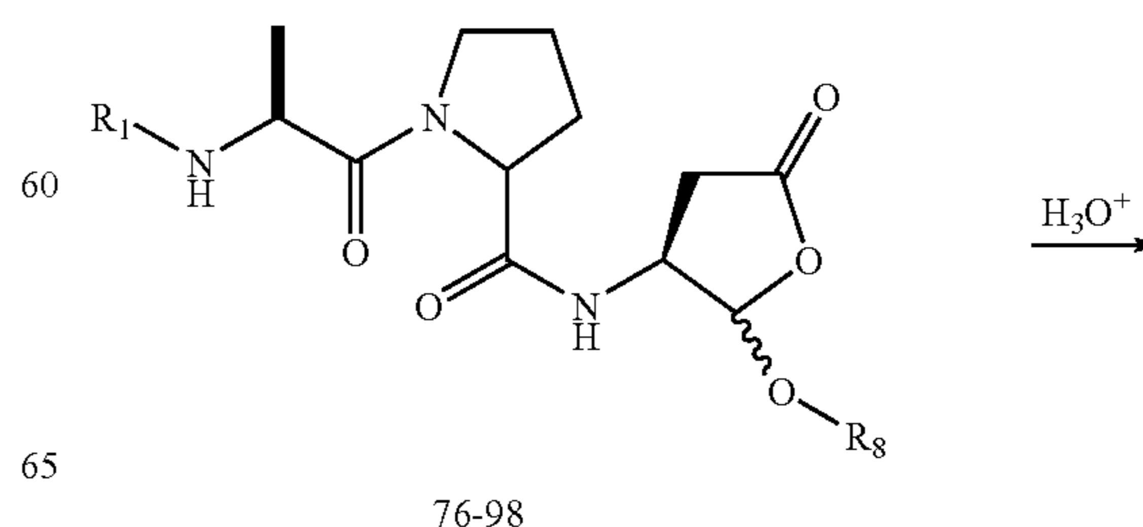
Scheme XXIV
