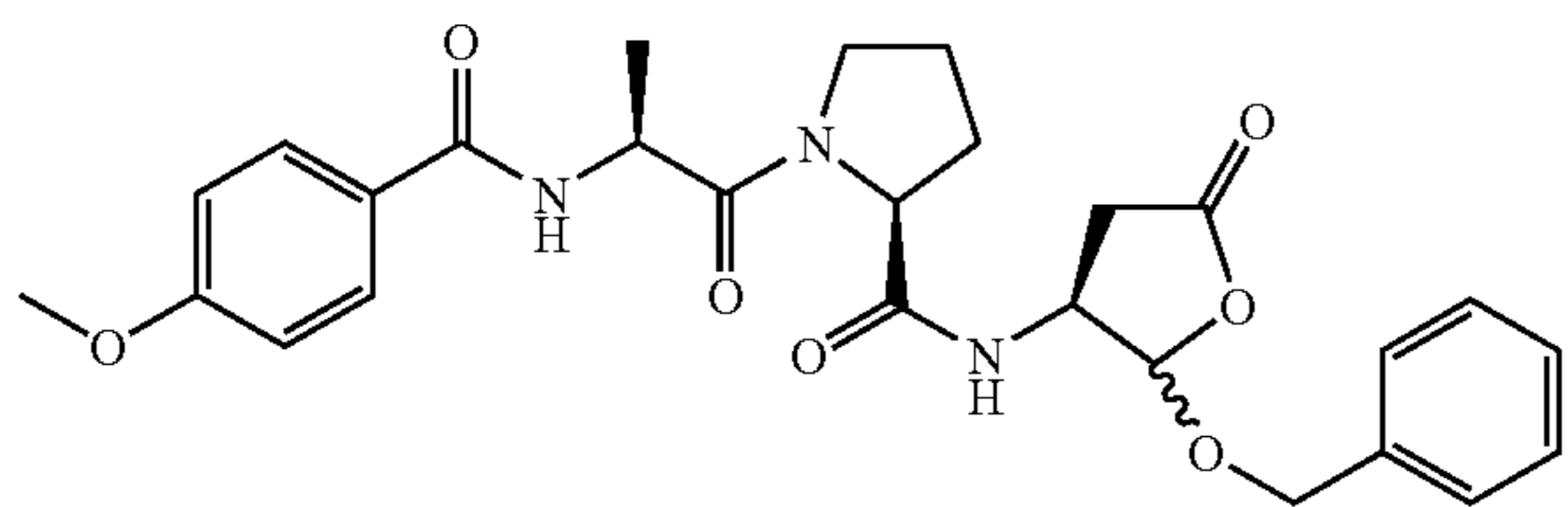
1-[2-(4-Methoxy-benzoylamino)-propionyl]-pyrrolidine-2-carboxylic acid (2-benzyloxy-5-oxo-tetrahydro-furan-3-yl)-amide (90)
