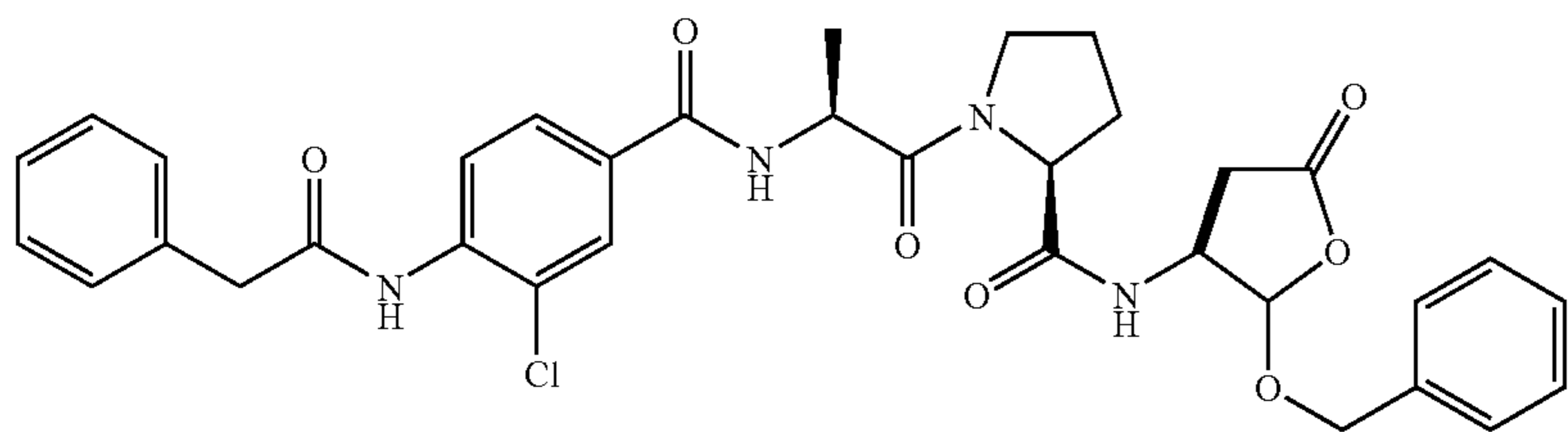
1-[2-(3-chloro-4-phenylacetyl-amino)-benzoylamino]-propionyl]-pyrrolidine-2-carboxylic acid (2-benzyloxy-5-oxo-tetrahydro-furan-3-yl)-amide (98ac)
