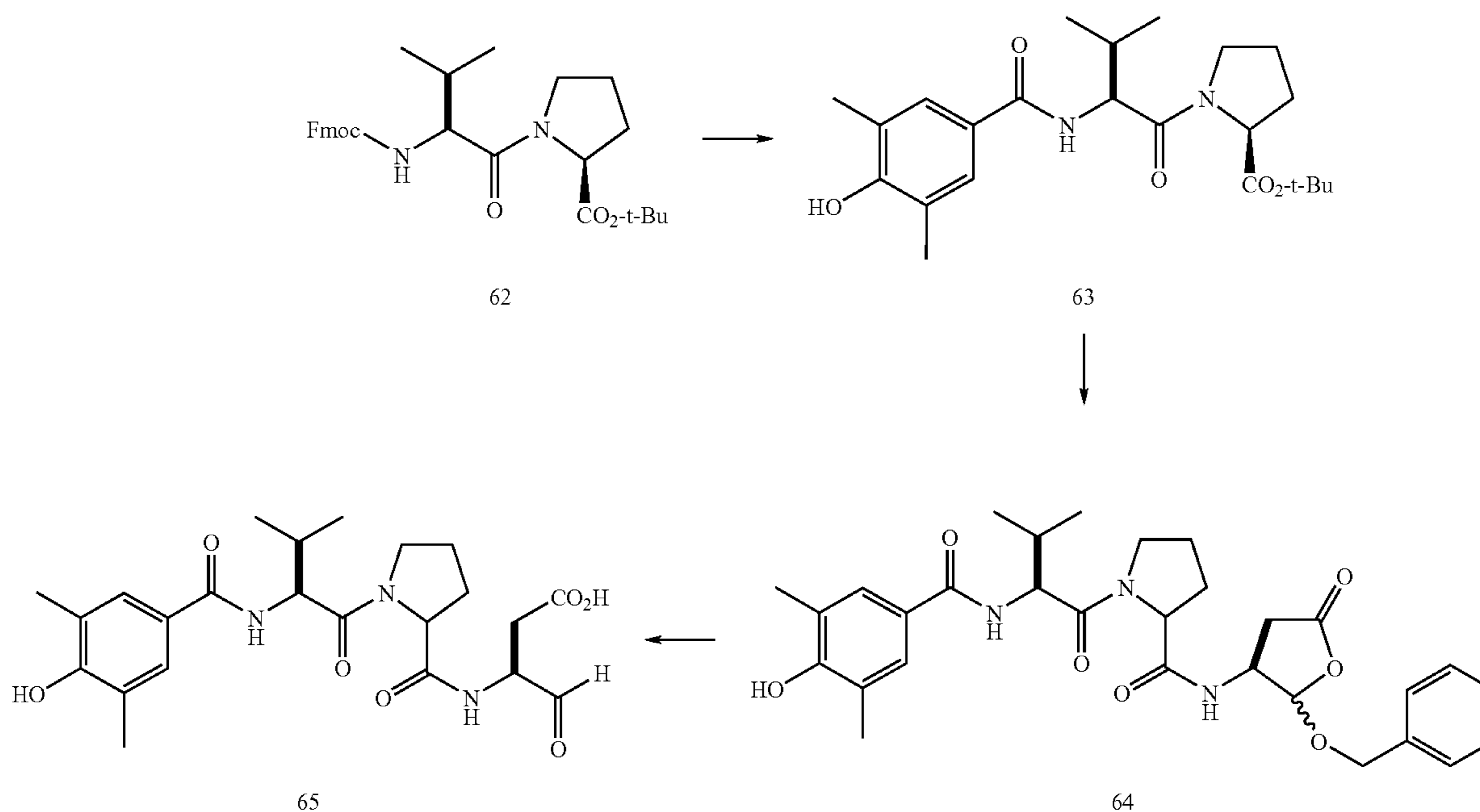
Scheme XIII
