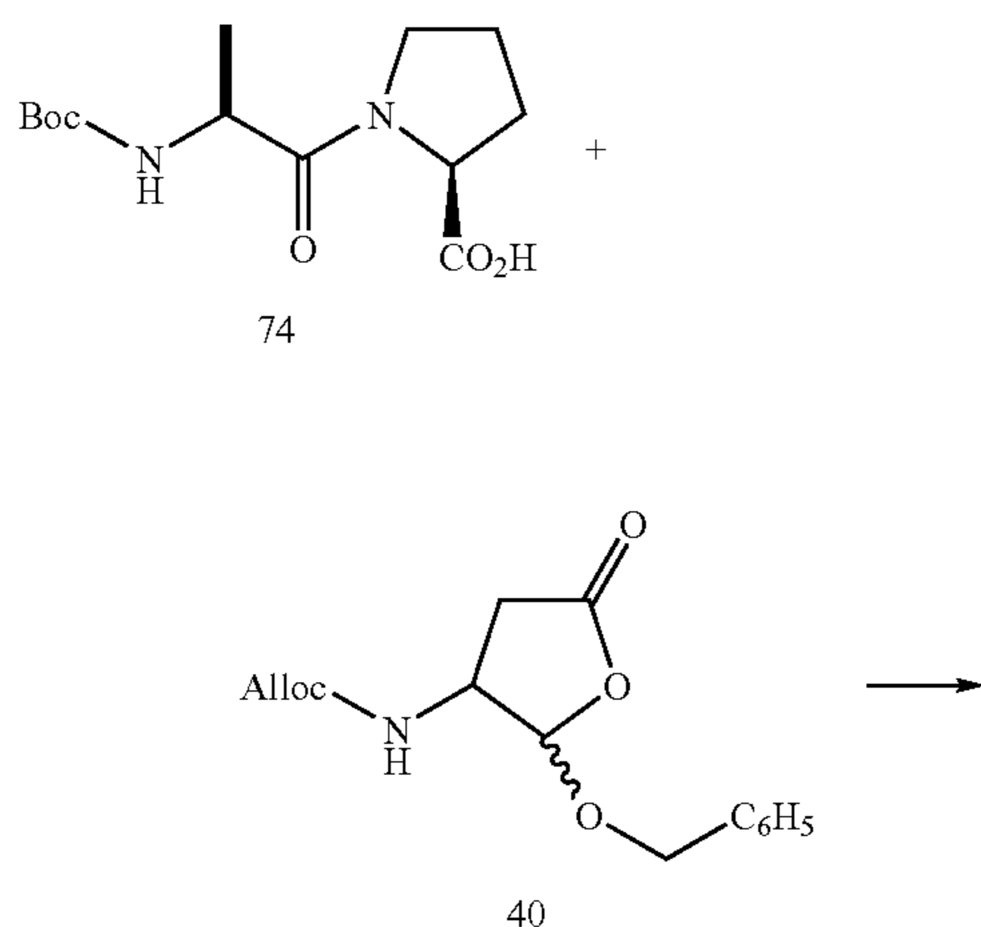
Scheme XVI
