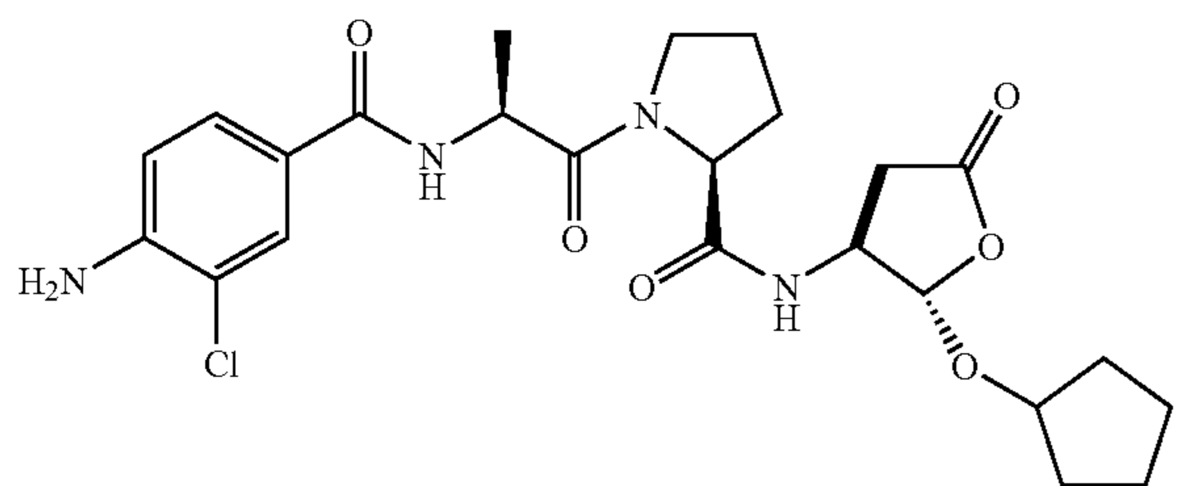
1-[2-(4-Amino-3-chloro-benzoylamino)-propionyl]-pyrrolidine-2-carboxylic acid (2-cyclopentyloxy-5-oxo-tetrahydro-furan-3-yl)-amide (98ax)
