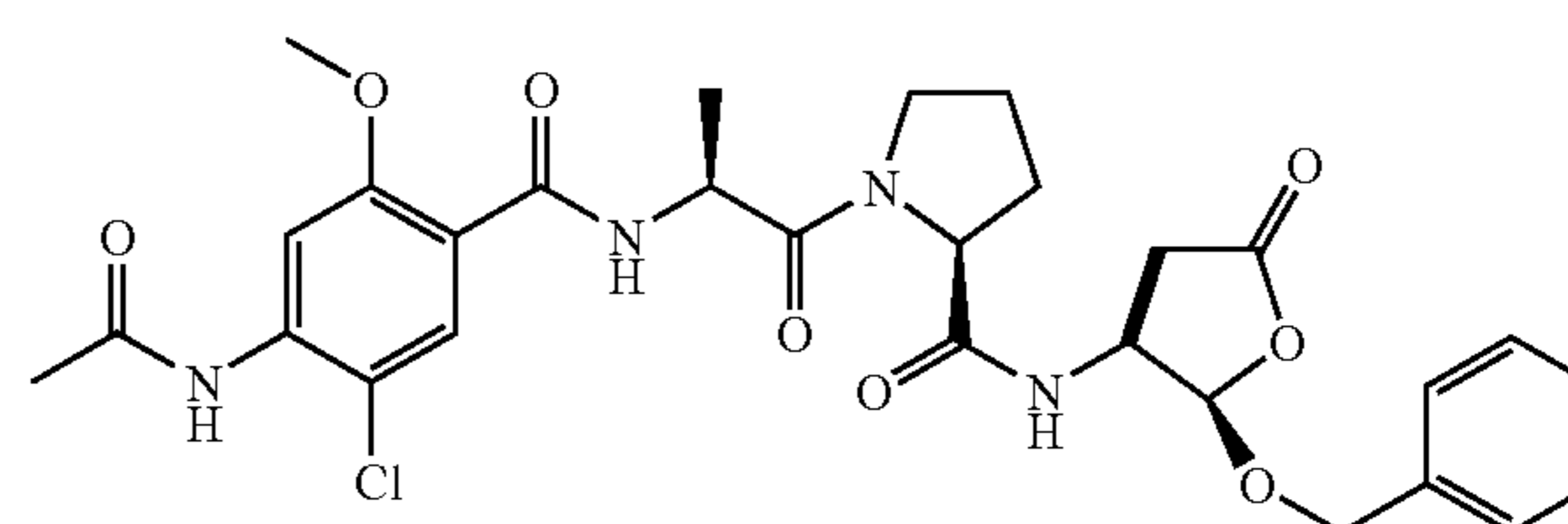
1-[2-(4-Acetylamino-5-chloro-2-methoxy-benzoylamino)-propionyl]-pyrrolidine-2-carboxylic acid (2-benzyloxy-5-oxo-tetrahydro-furan-3-yl)-amide (98j)
