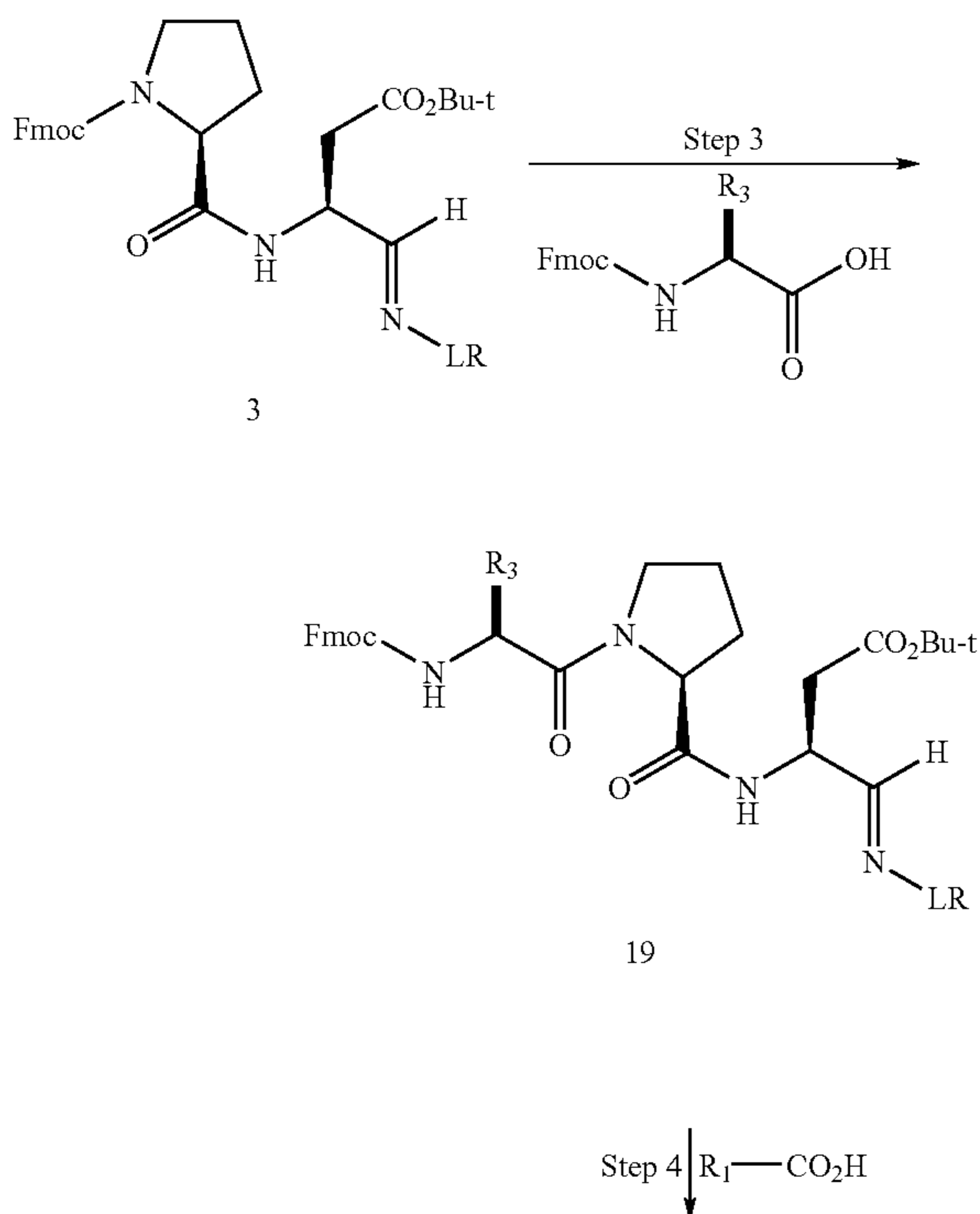
Scheme V
