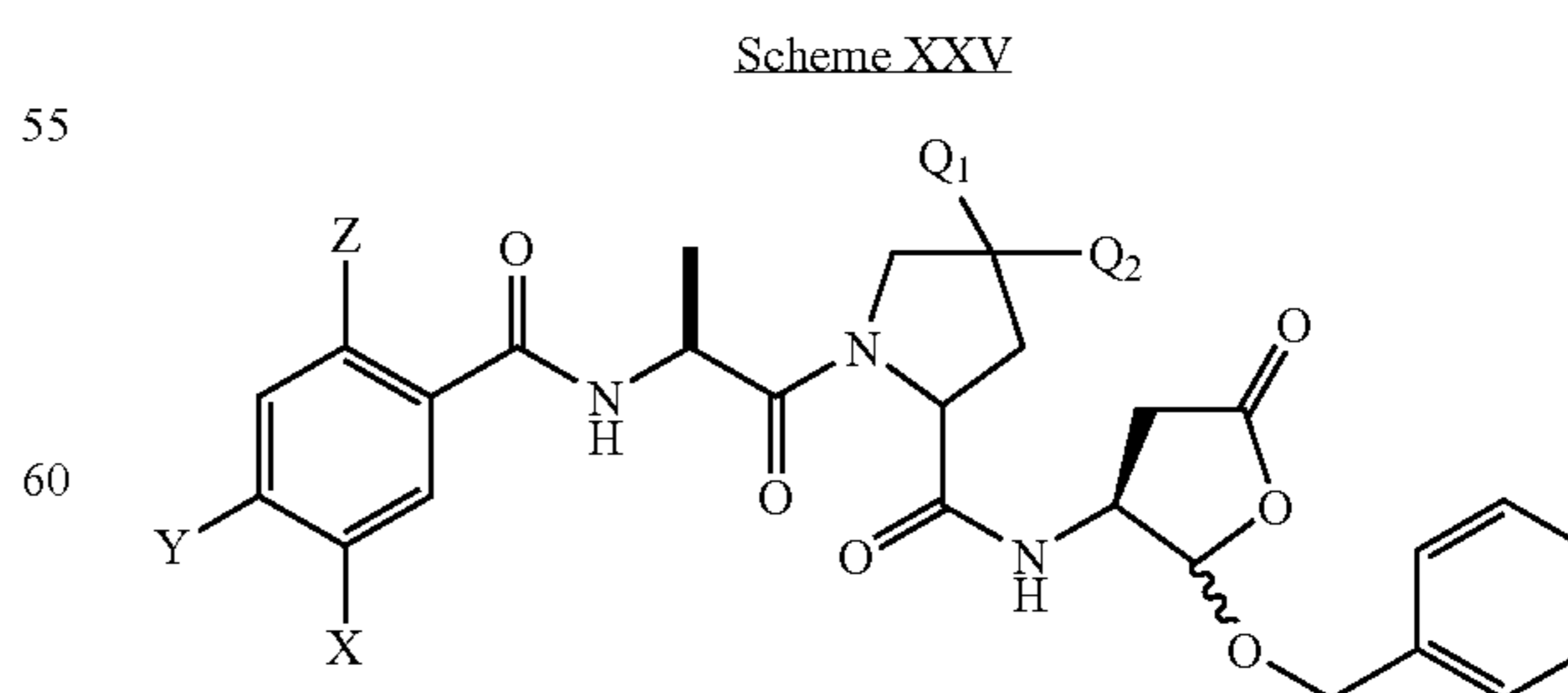
108a, X = Cl, Y = NH 2 , Z = H, Q 1 = F, Q 2 = H 116b, X = Cl, Y = AcNH, Z = H, Q 1 = Q 2 = F 116c, X = Cl, Y = AcNH, Z = CH 3 O, Q 1 = Q 2 = F
