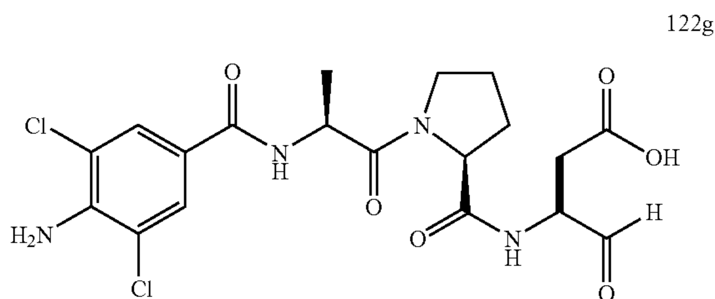
3-({1-[2-(4-Amino-3,5-dichloro-benzoylamino)-propionyl]-pyrrolidine-2-carbonyl}-amino)-4-oxo-butyrinic acid (122g)
