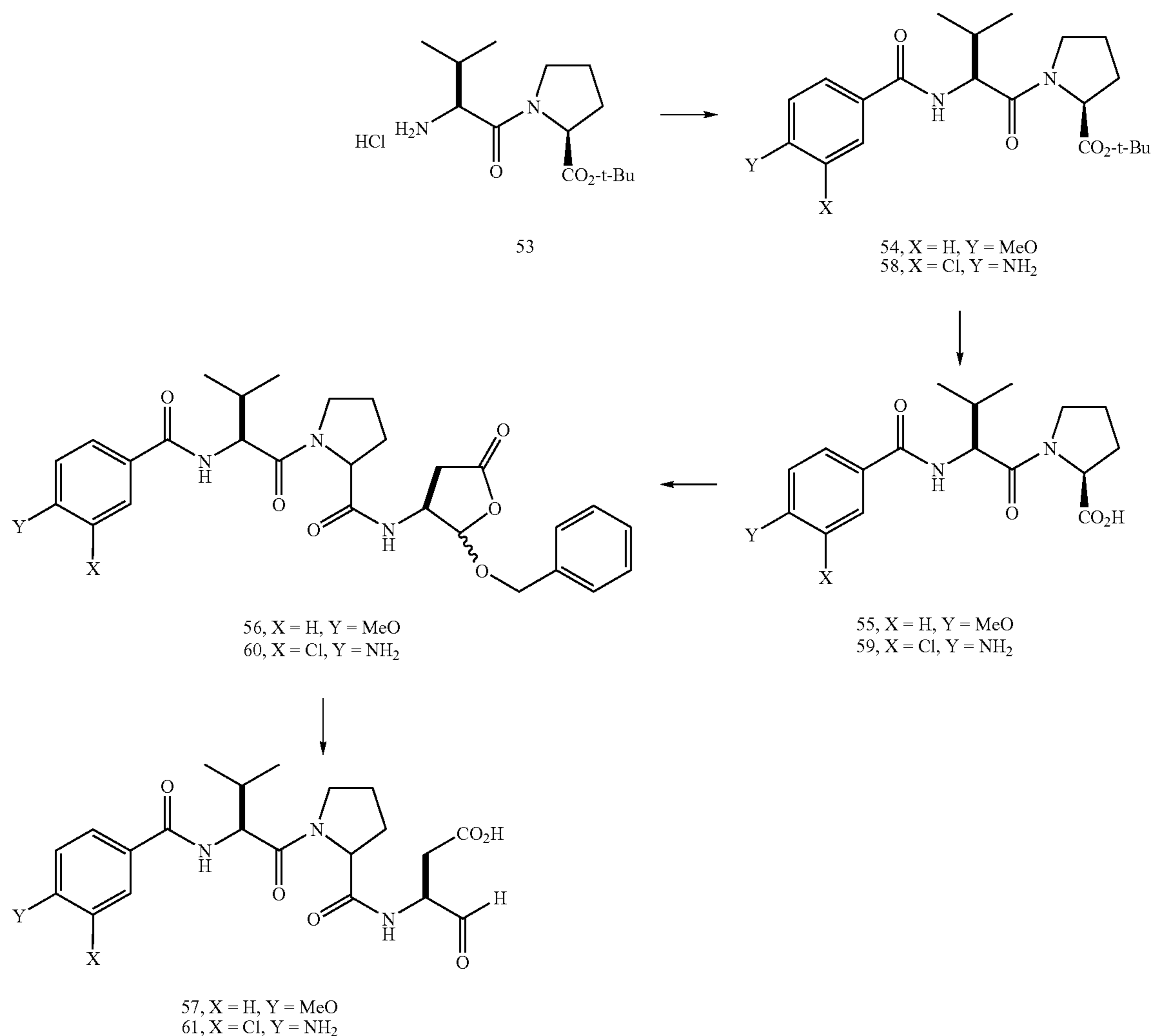
Scheme XII
