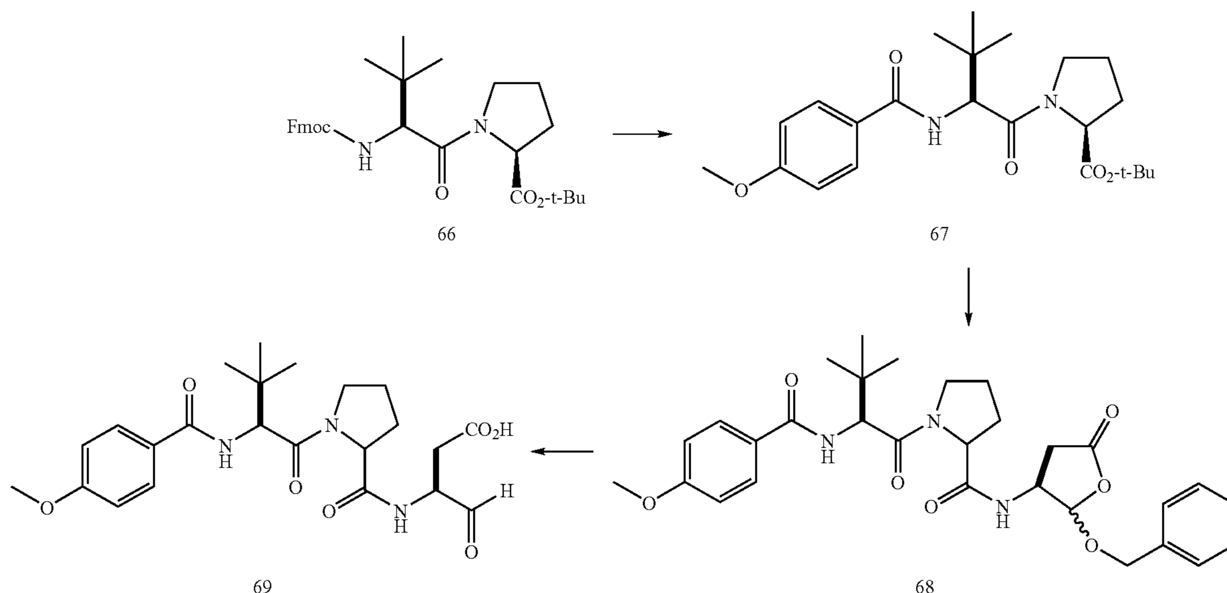
Scheme XIV
