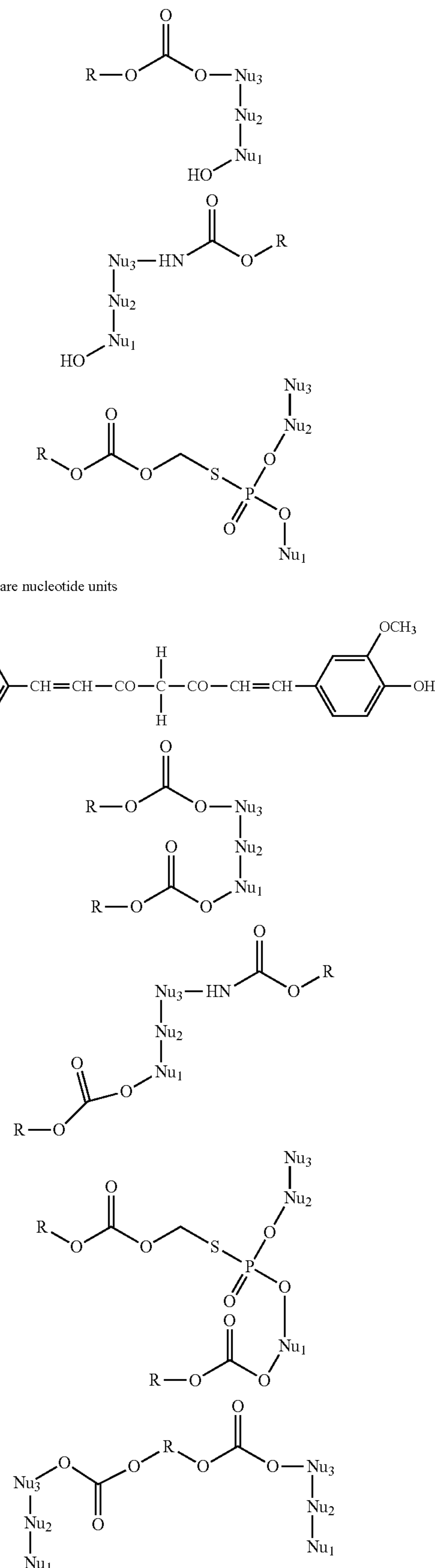
Scheme 2
