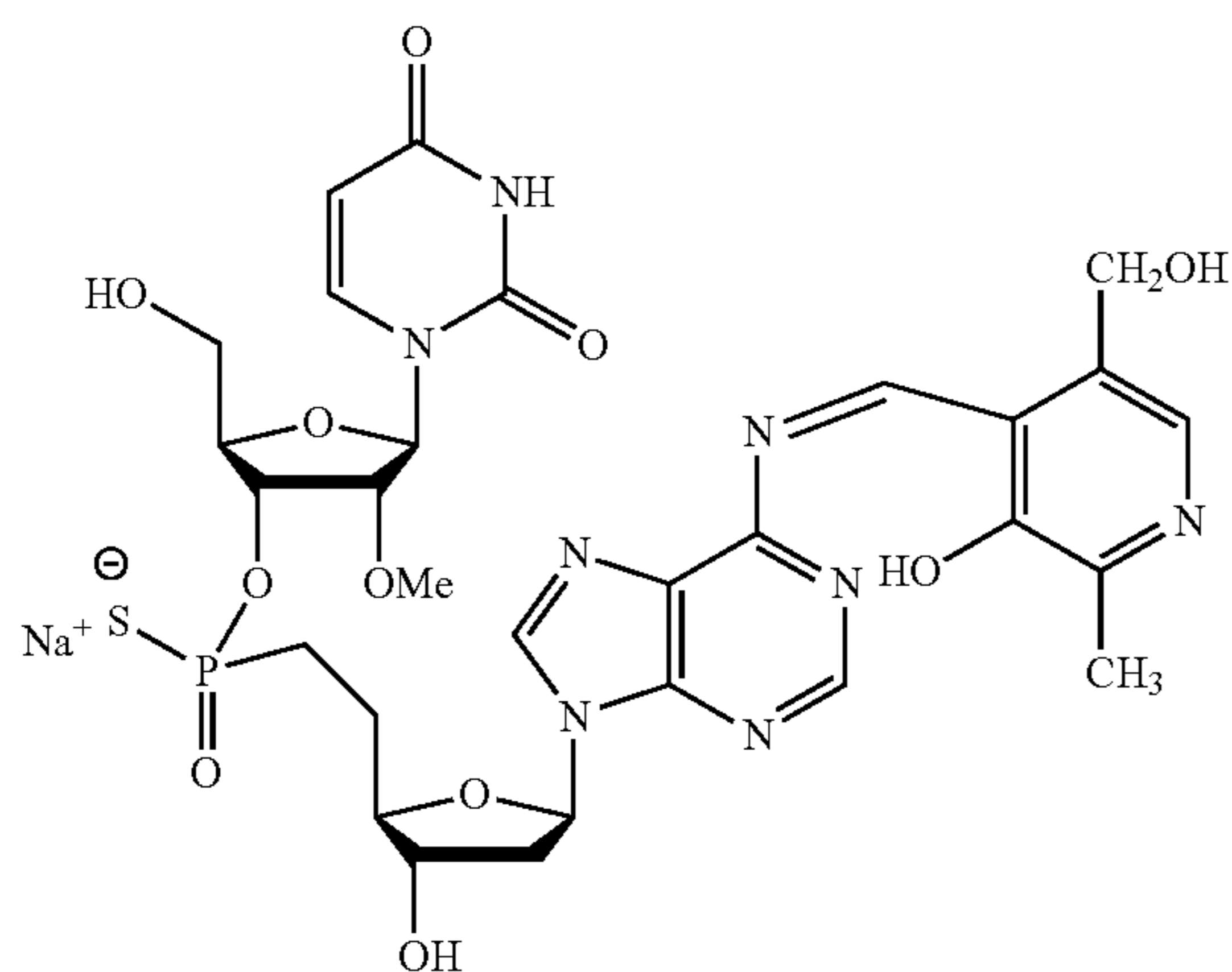
Schiff's base of dinucleotide with pyridoxine
