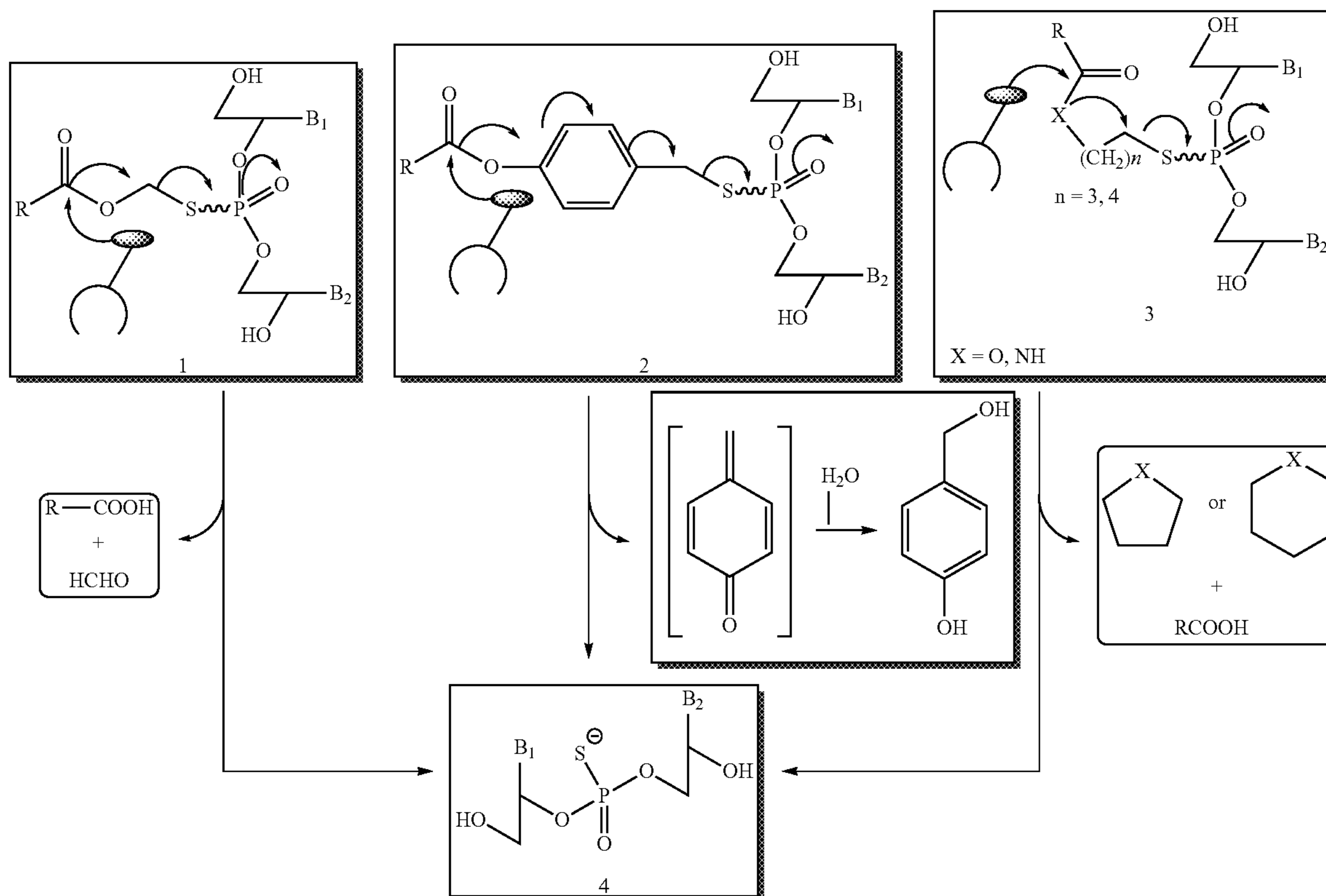
Scheme 1
