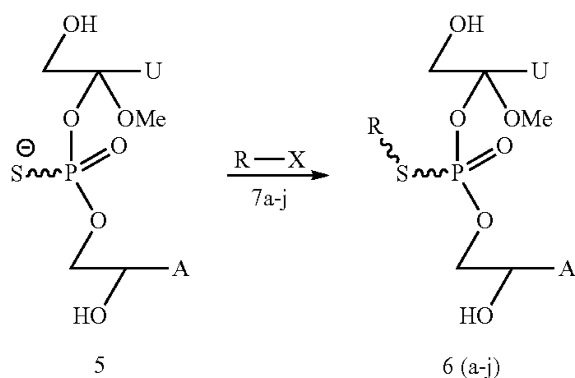
Scheme 4
