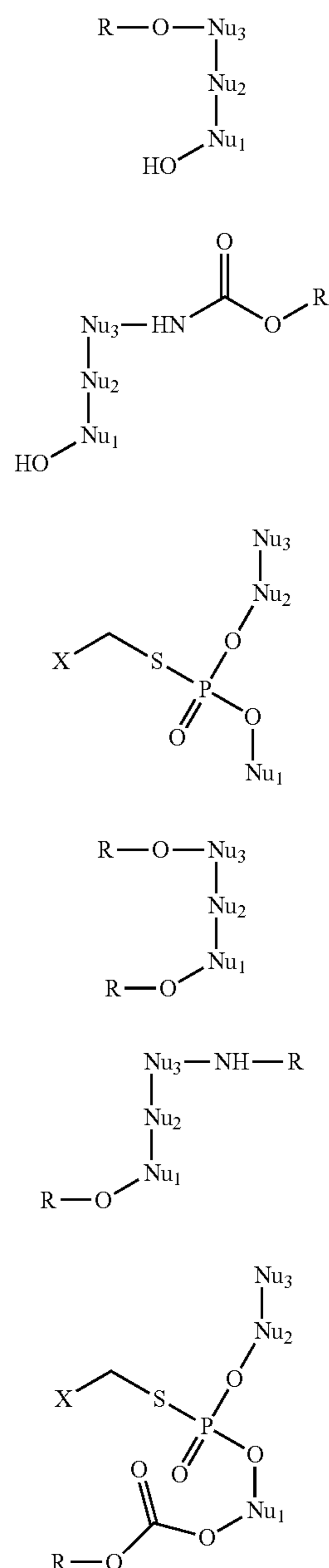
Scheme 3
