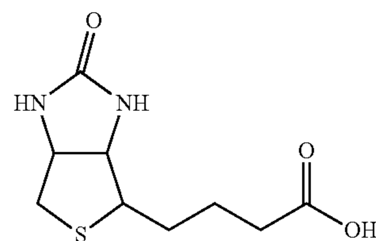
Biotin linked either as alcohol, acid or as derivex compounds
