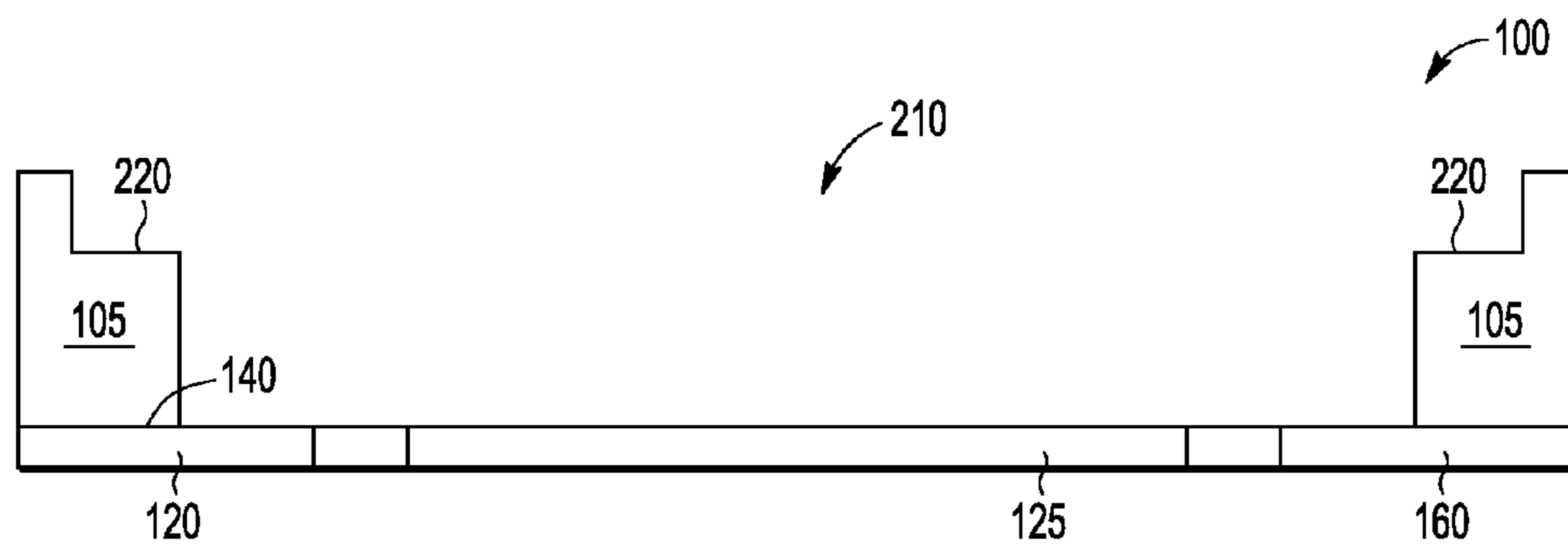
FIG. 2 - PRIOR ART -
