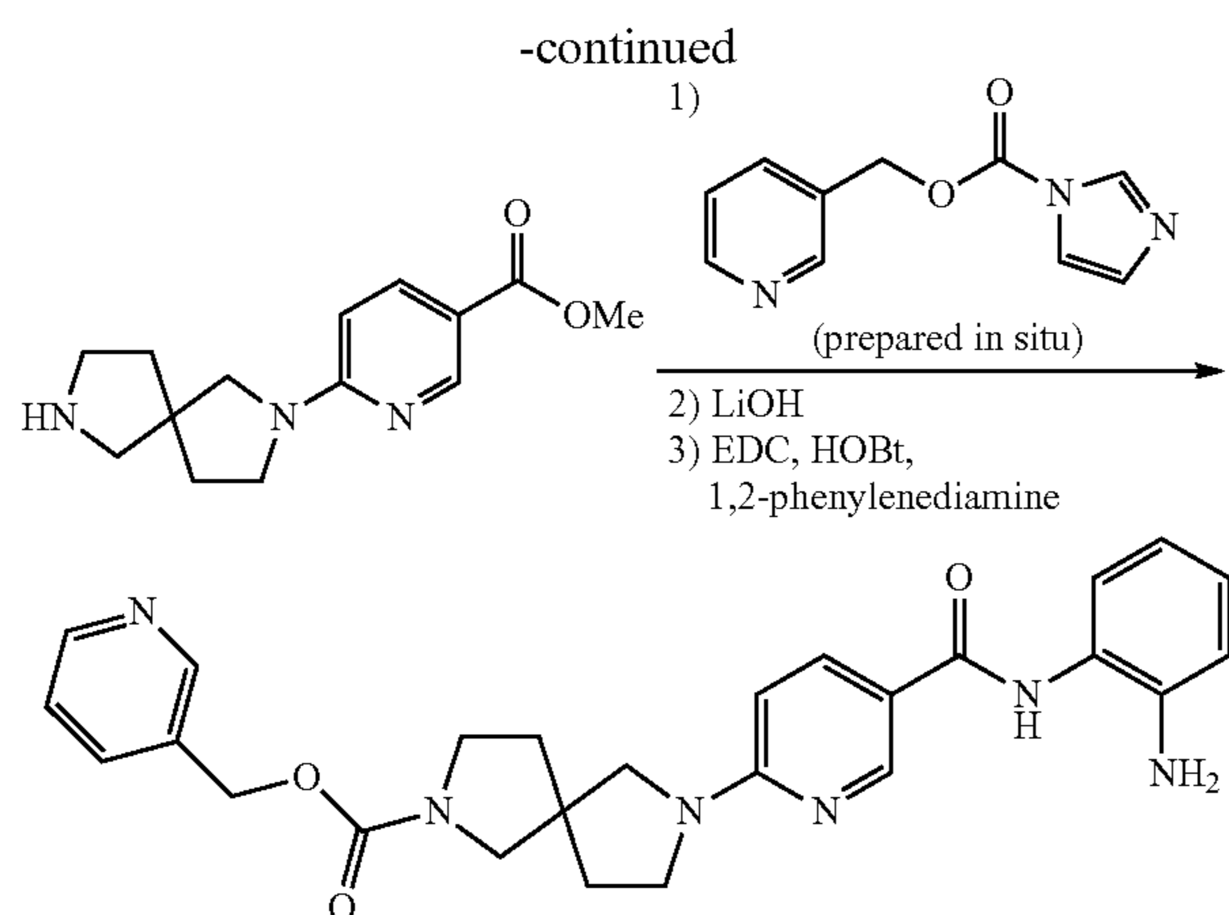
Pyridin-3-ylmethyl 7-(5-[[2-Aminophenyl]amino]carbonyl)pyridin-2-yl)-2,7-diazaspiro[4.4]nonane-2-carboxylate
