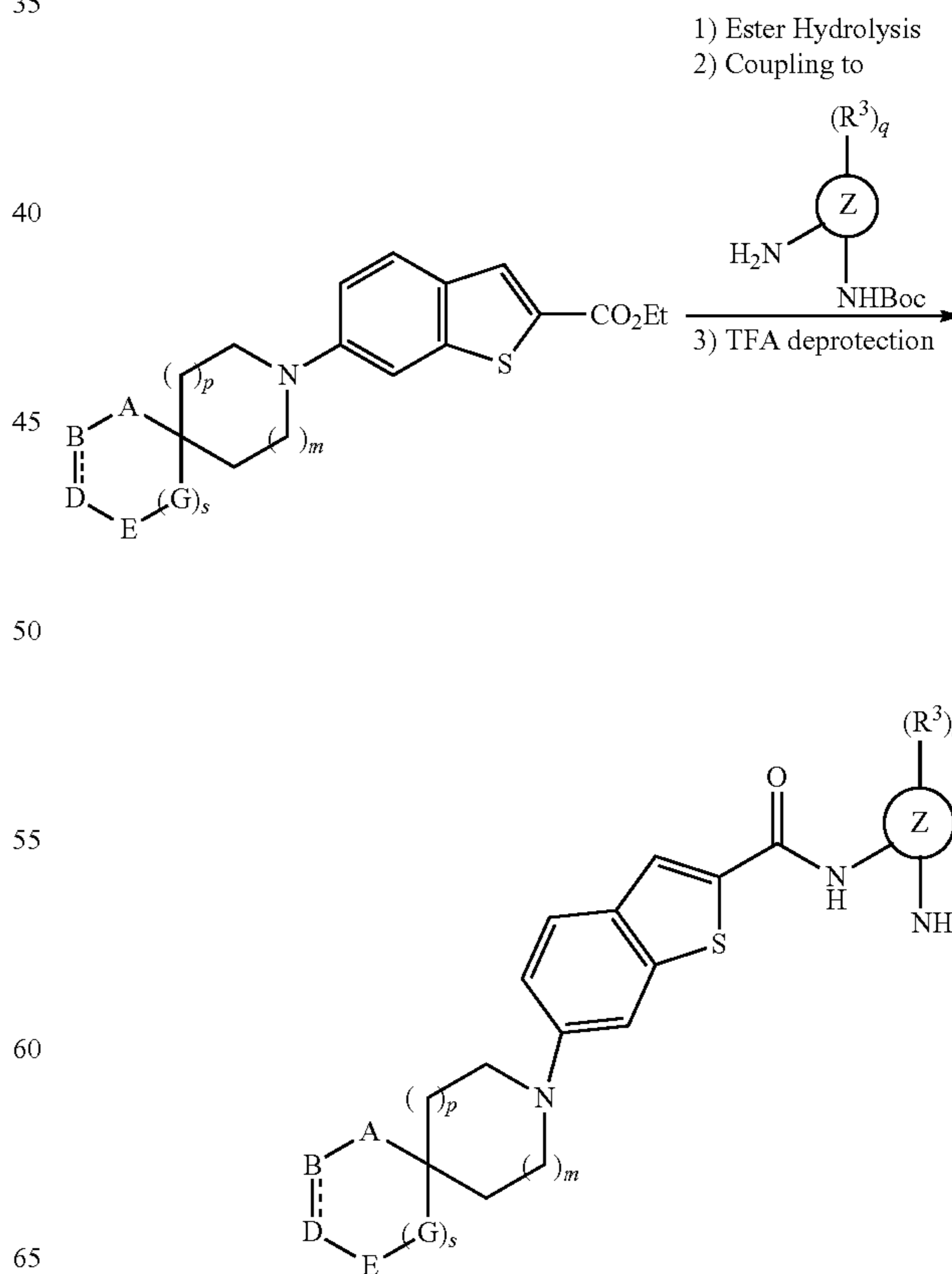
SCHEME 4
