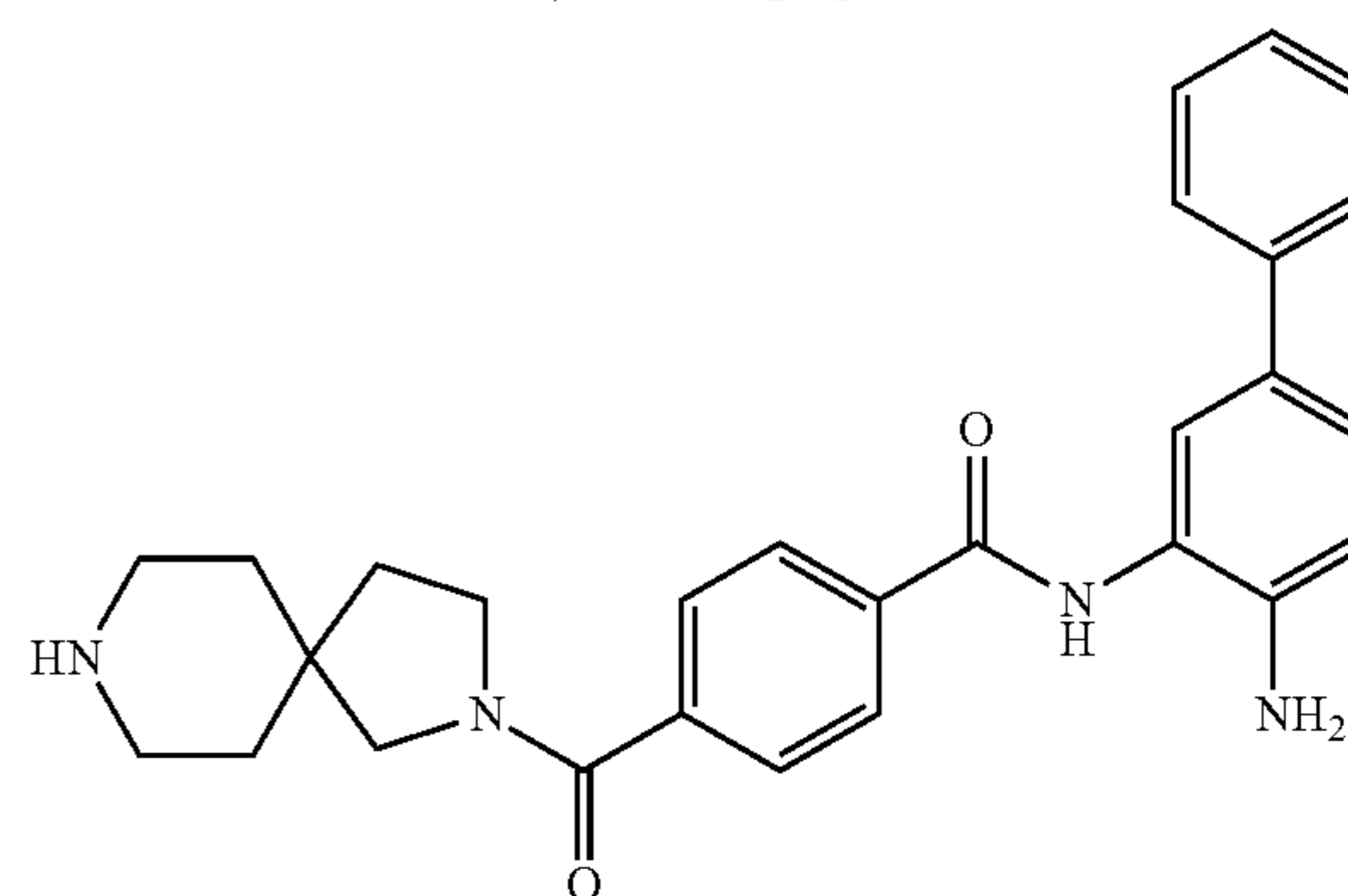
N-(4-Aminobiphenyl-3-yl)-4-(2,8-diazaspiro[4,5]dec-2-ylcarbonyl)benzamide
