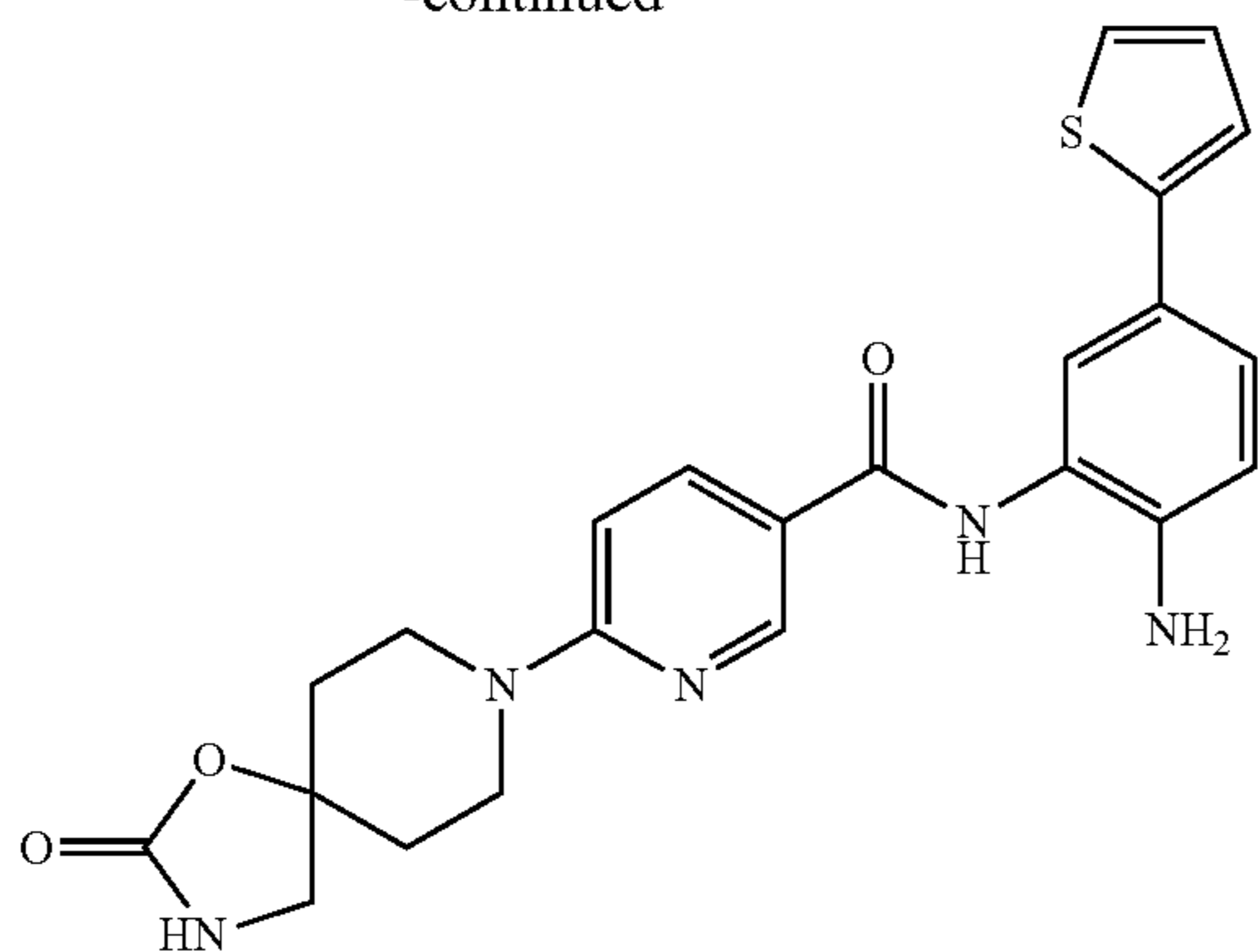
N-[2-Amino-5-(2-thienyl)phenyl]-6-(2-oxo-1-oxa-3,8-diazaspiro[4.5]dec-8-yl)nicotinamide
