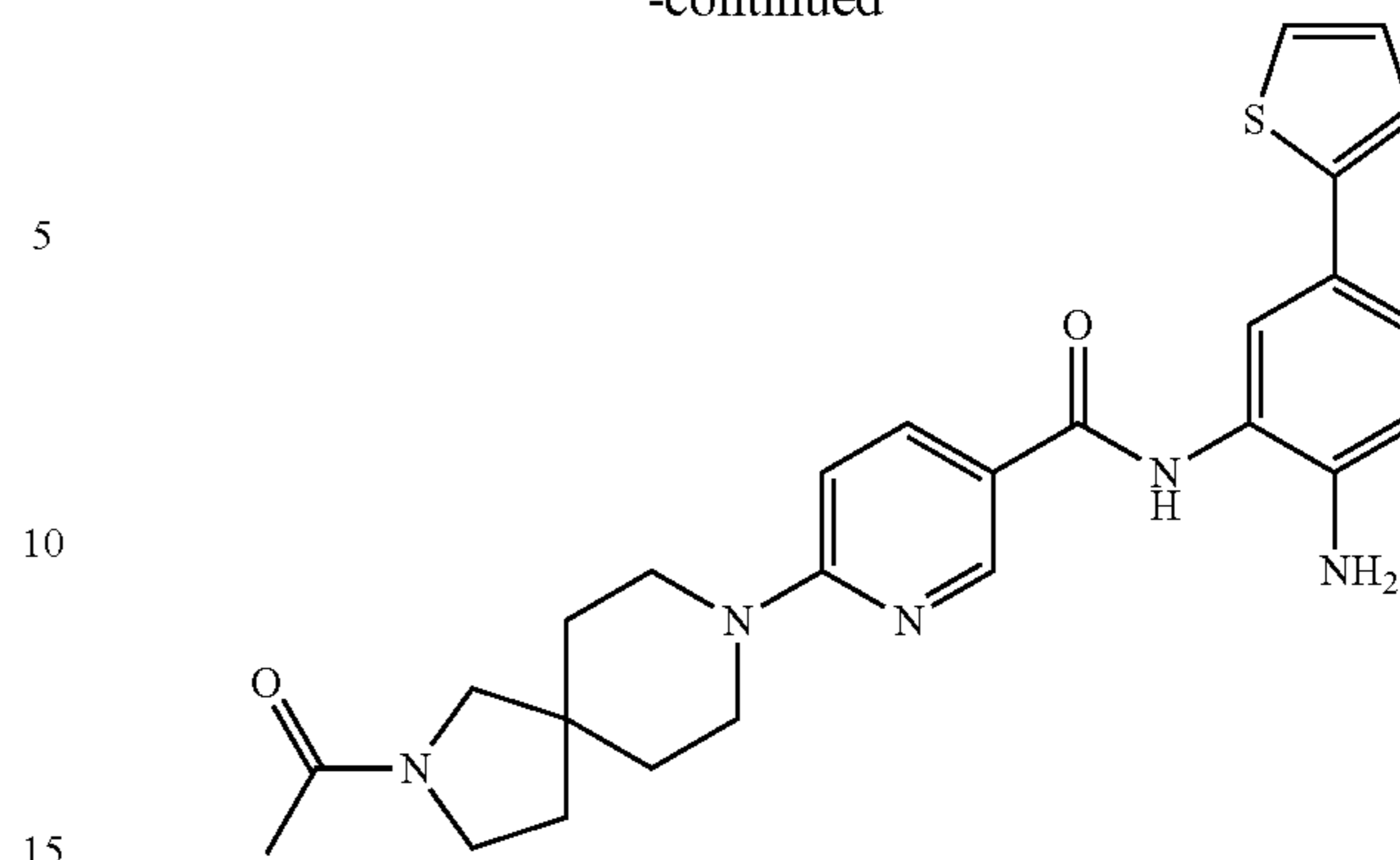
6-(2-acetyl-2,8-diazaspiro[4.5]dec-8-yl)-N-[2-amino-5-(2-thienyl)phenyl]nicotinamide
