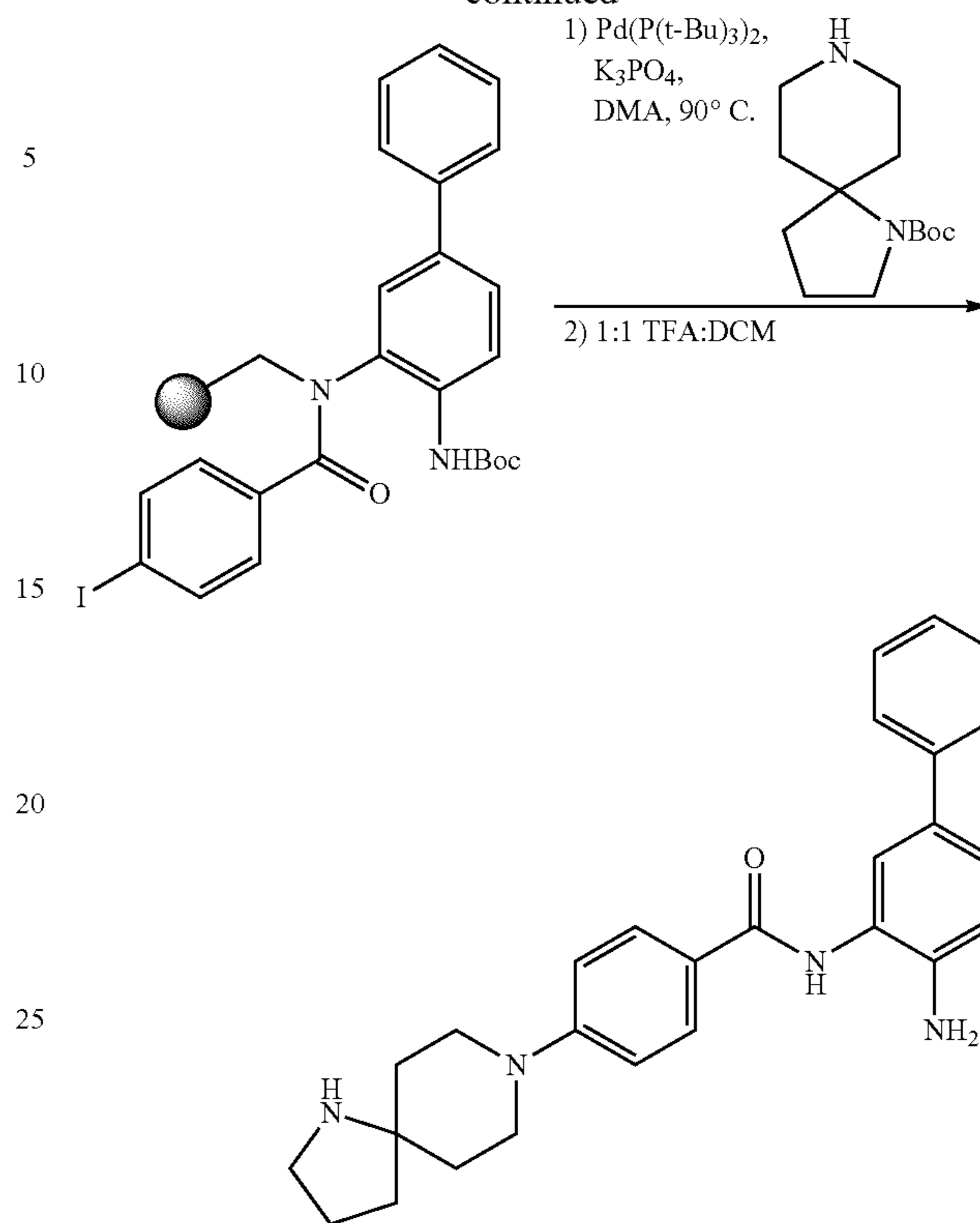
N-(4-Aminobiphenyl-3-yl)-4-(1,8-diazaspiro[4.5]dec-8-yl)benzamide
