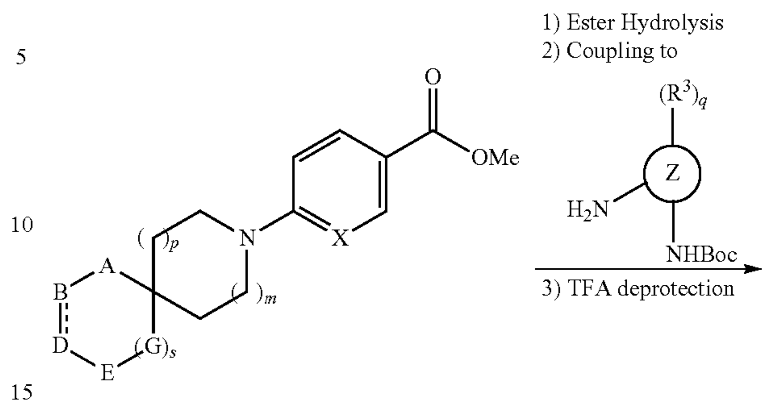
SCHEME 3
