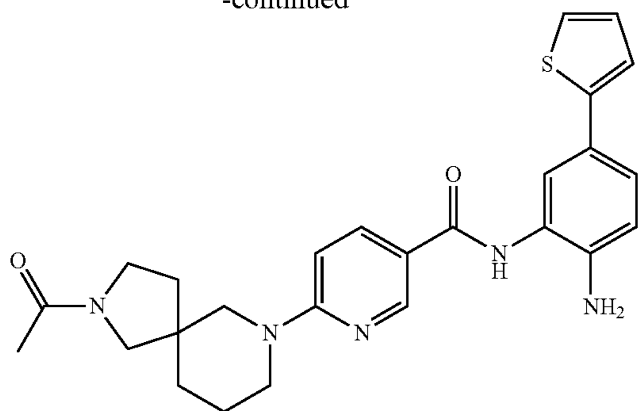
6-(2-Acetyl-2,7-diazaspiro[4.5]dec-7-yl)-N-[2-amino-5-(2-thienyl)phenyl]-nicotinamide
