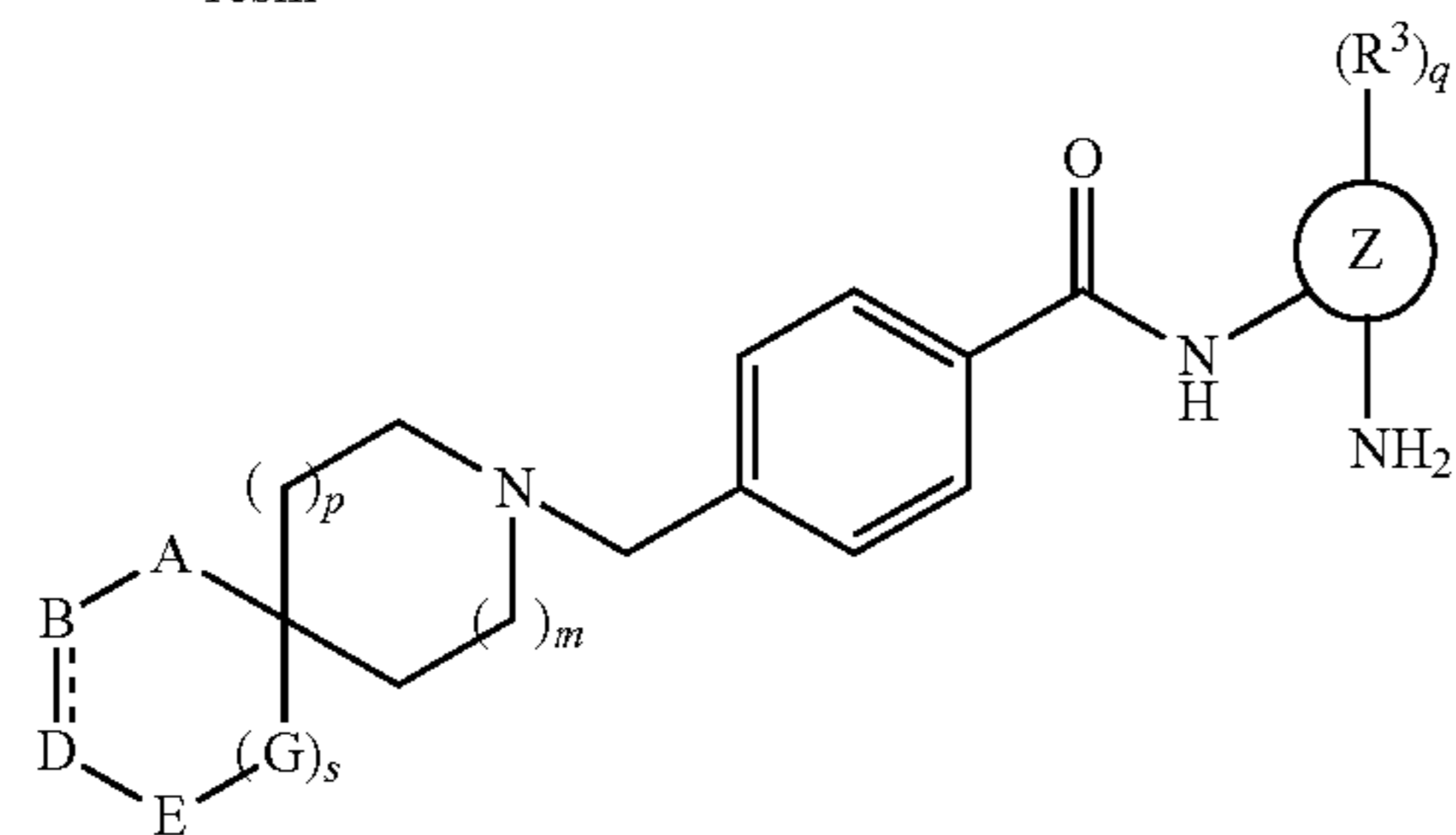
SCHEME 7
