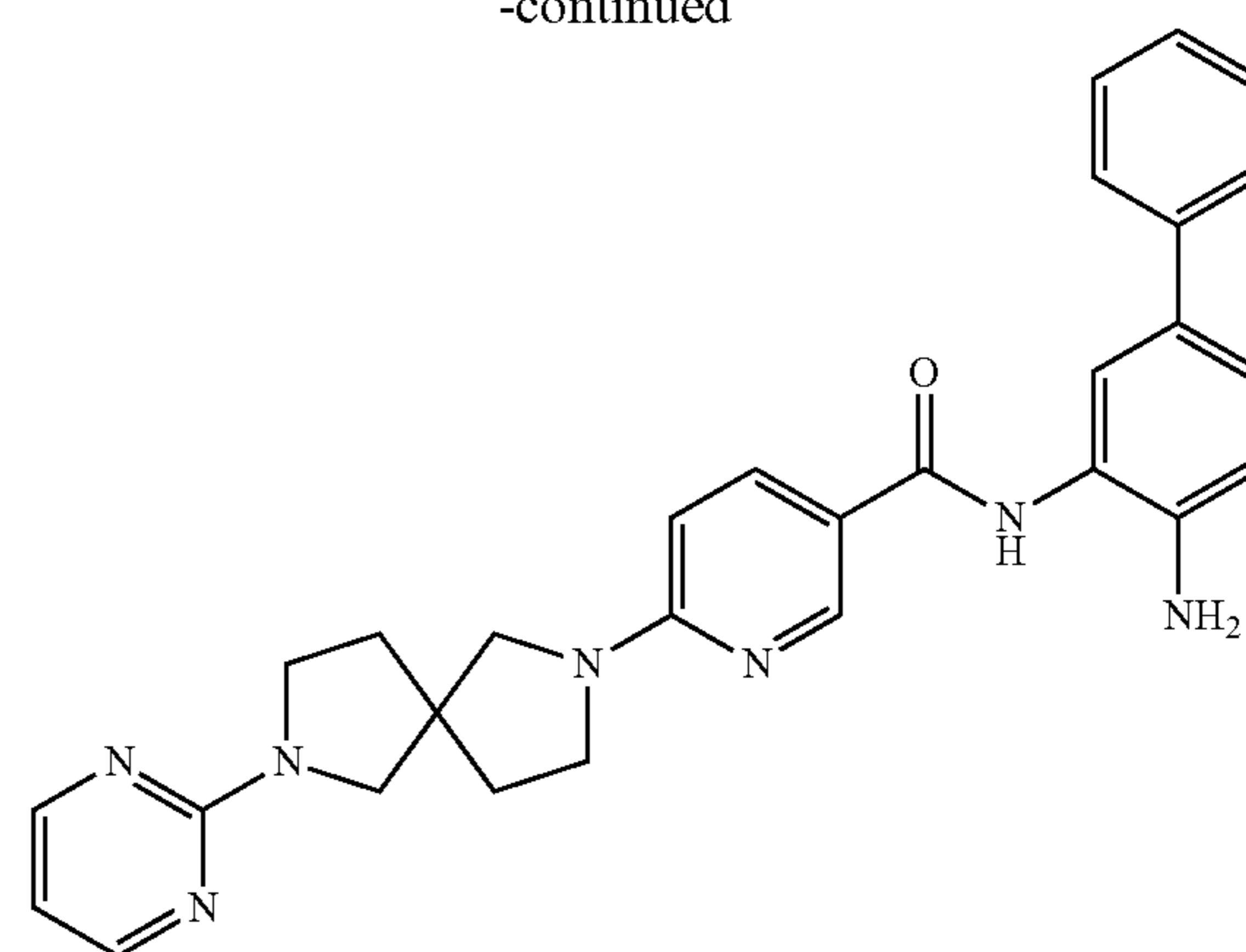
N-(4-Aminobiphenyl-3-yl)-6-(7-pyrimidin-2-yl-2,7-diazaspiro[4.4]non-2-yl)nicotinamide
