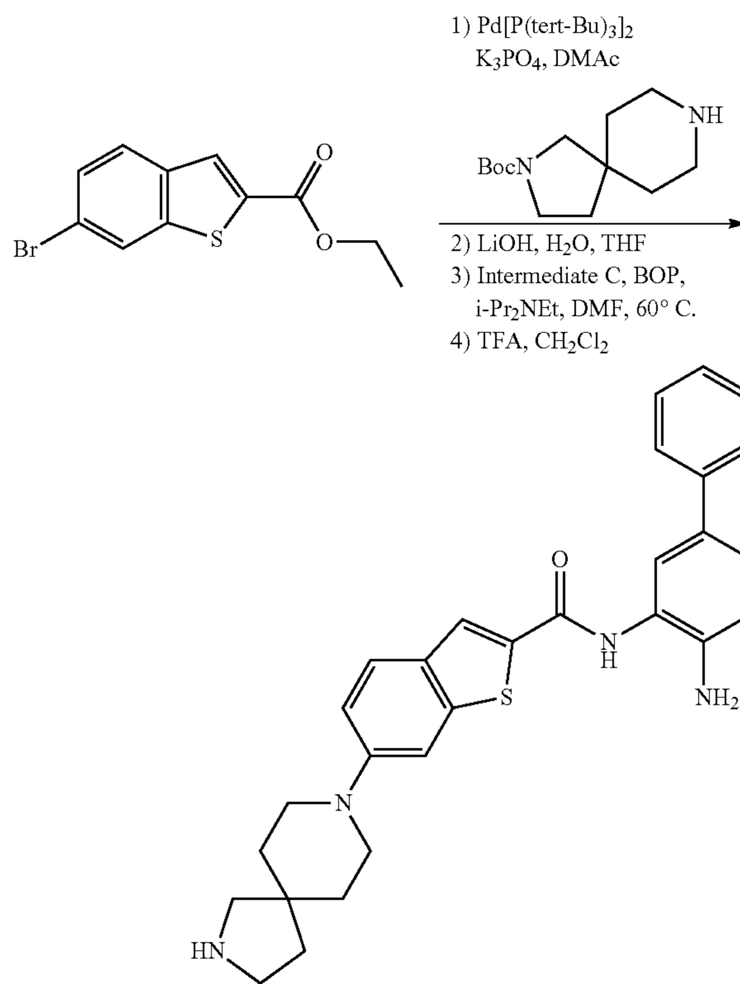
N-(4-Aminobiphenyl-3-yl)-6-(2,8-diazaspiro[4.5]dec-8-yl)-1-benzothiophene-2-carboxamide
