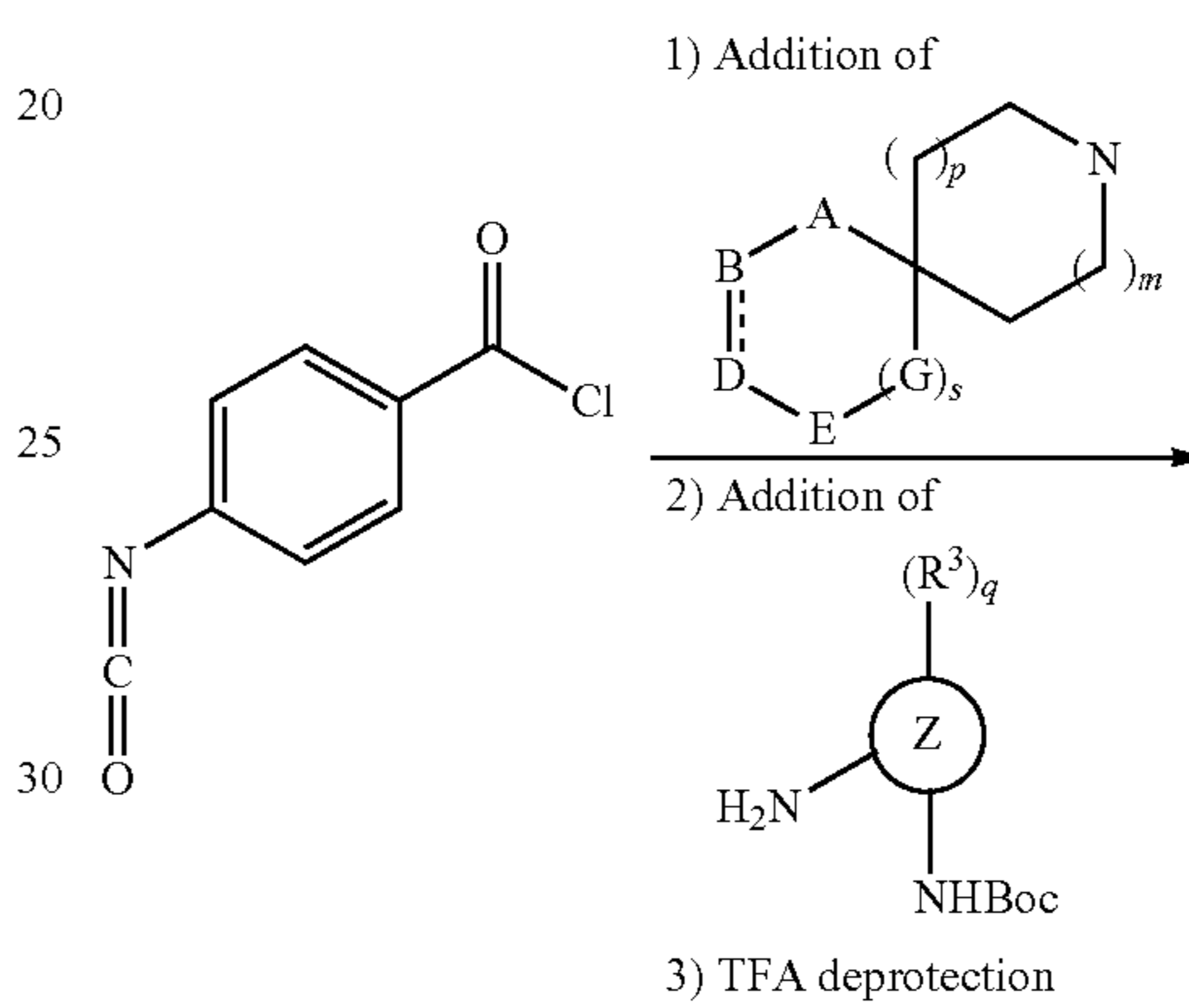
SCHEME 8
