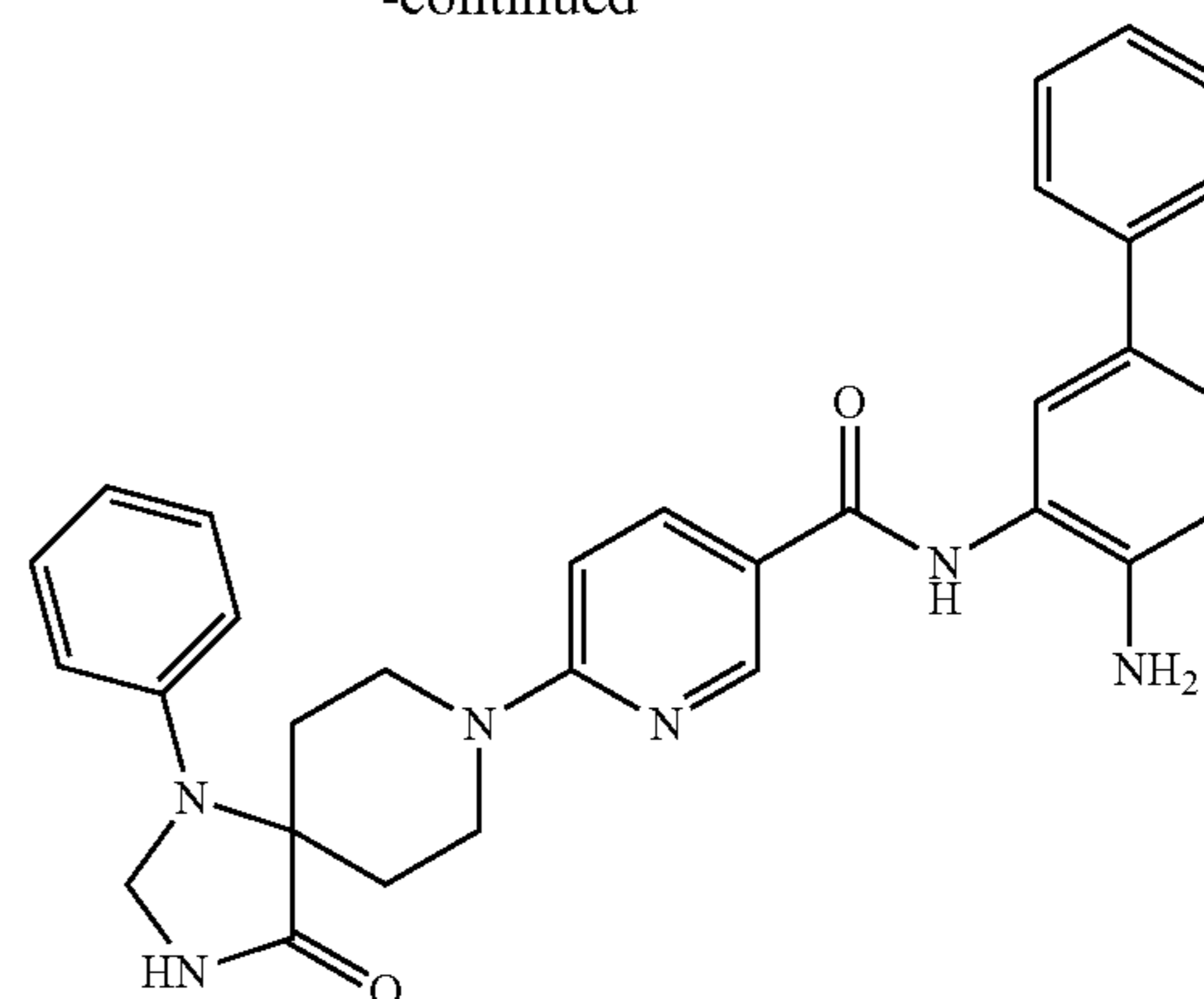
N-(4-Aminobiphenyl-3-yl)-6-(4-oxo-1-phenyl-1,3,8-triazaspiro[4.5]dec-8-yl)nicotinamide
