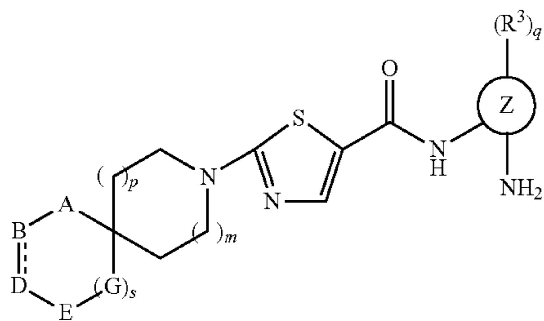
SCHEME 6
