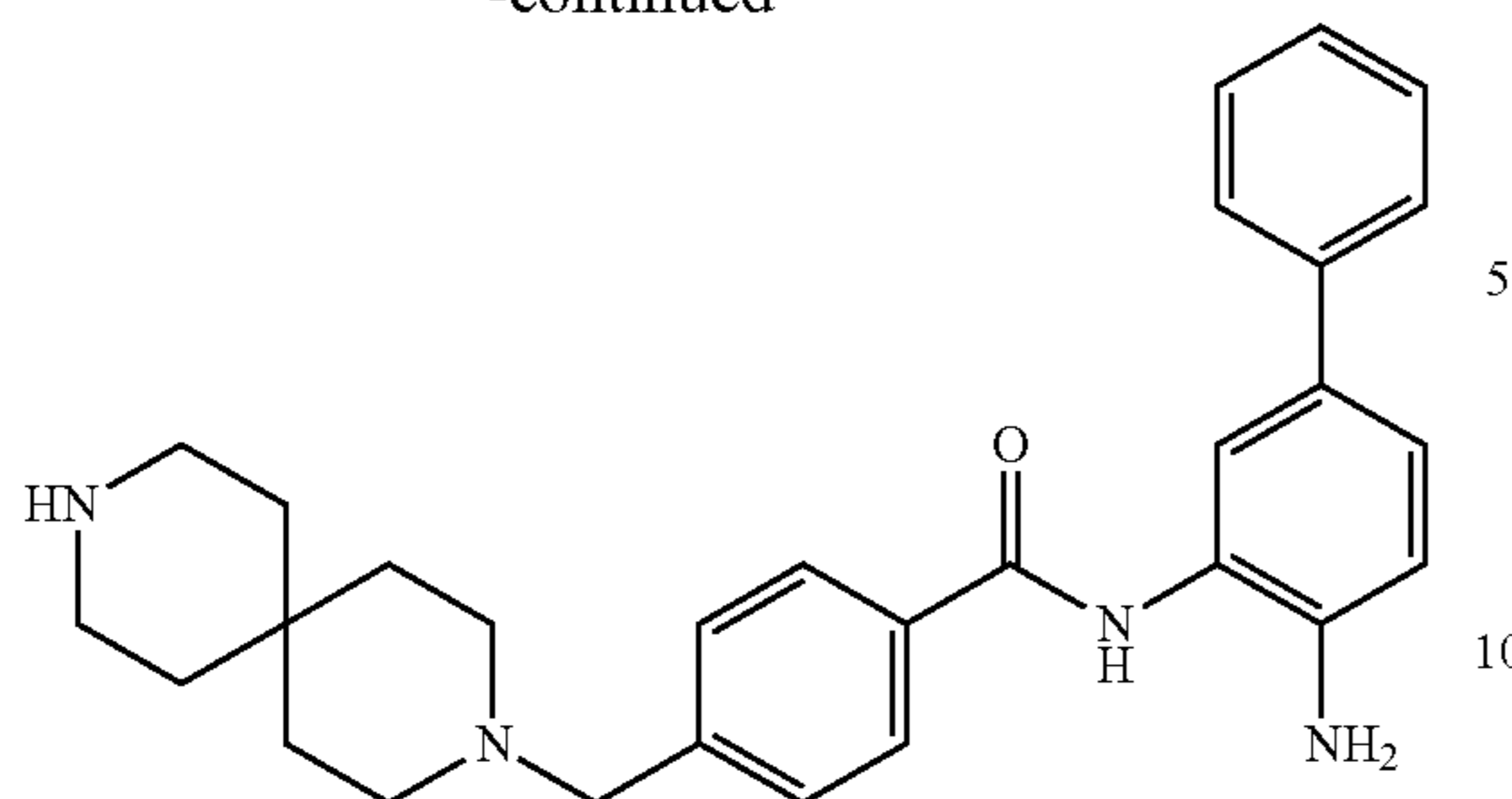
N-(4-aminobiphenyl-3-yl)-4-(3,9-diazaspiro[5.5]undec-3-ylmethyl)benzamide
