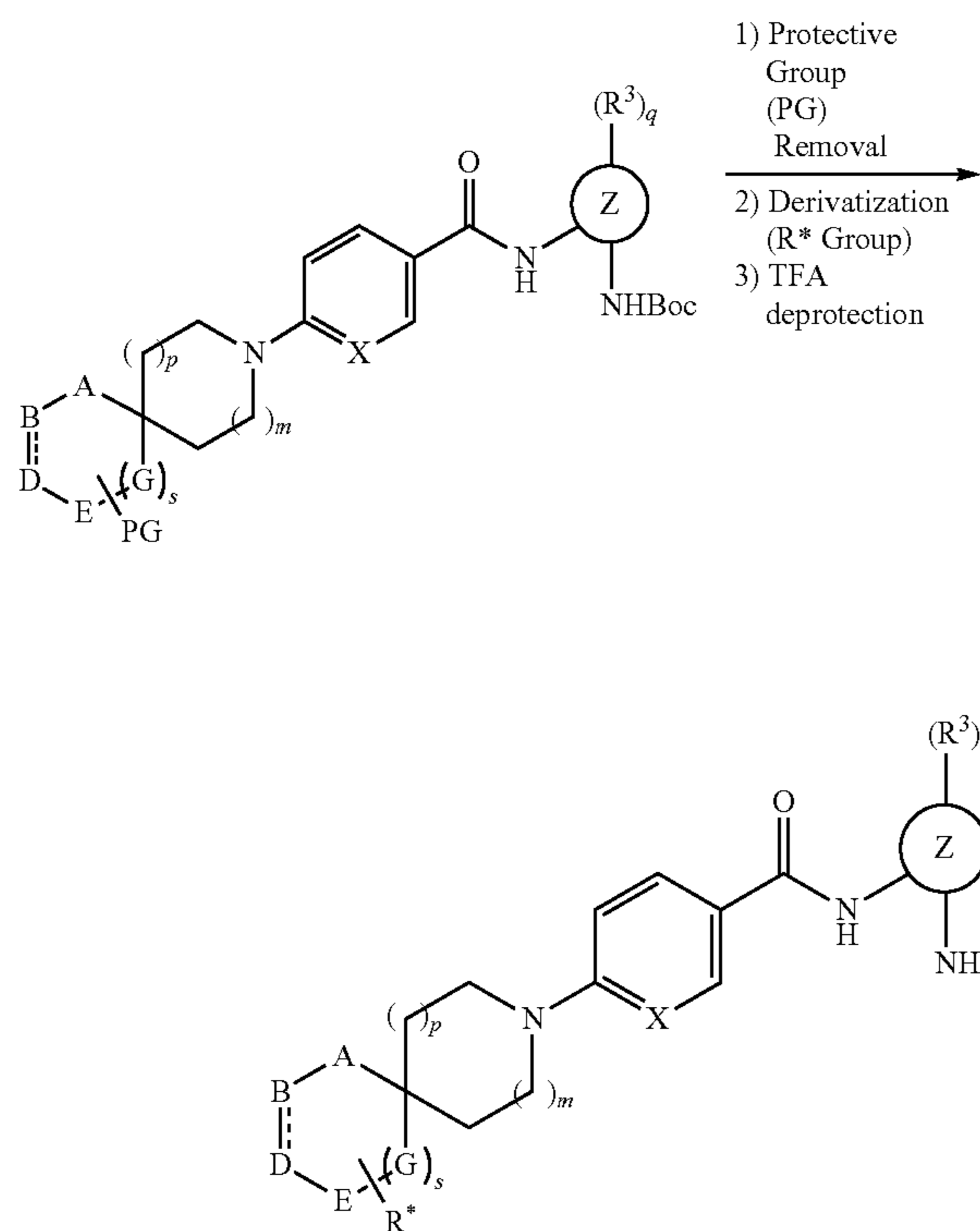
SCHEME 2
