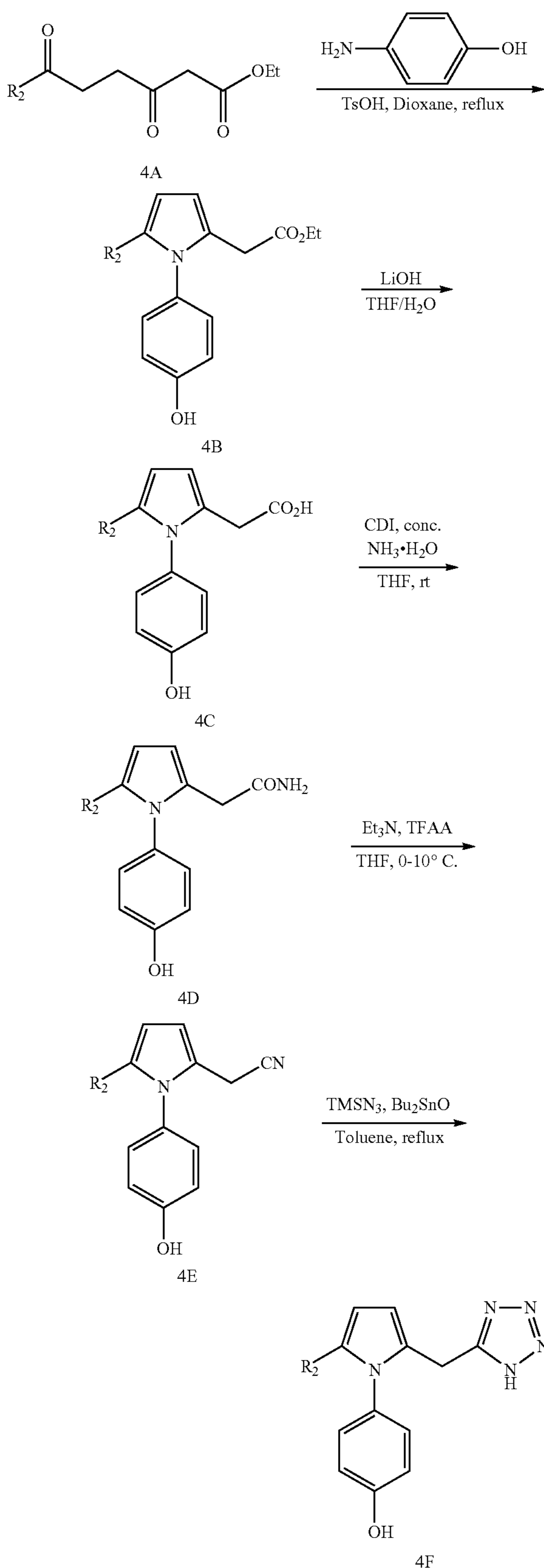
Scheme 4: A general scheme for preparing GSNOR inhibitors with structure 4F
