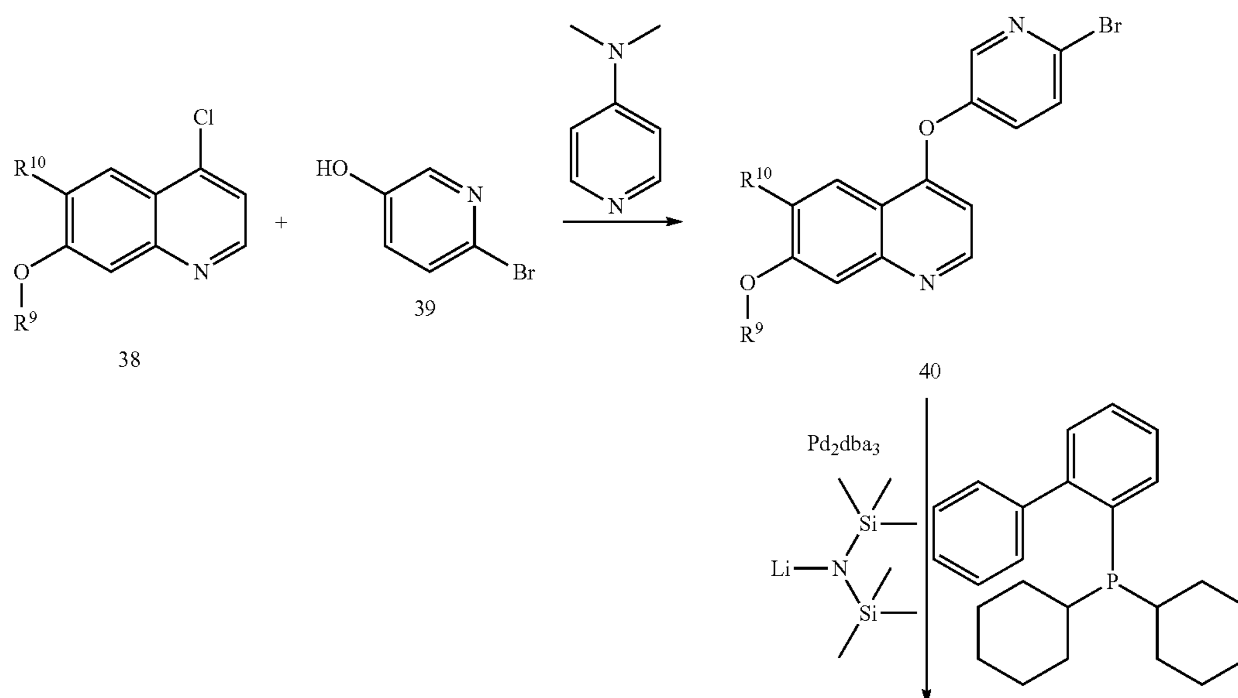
Scheme 10
