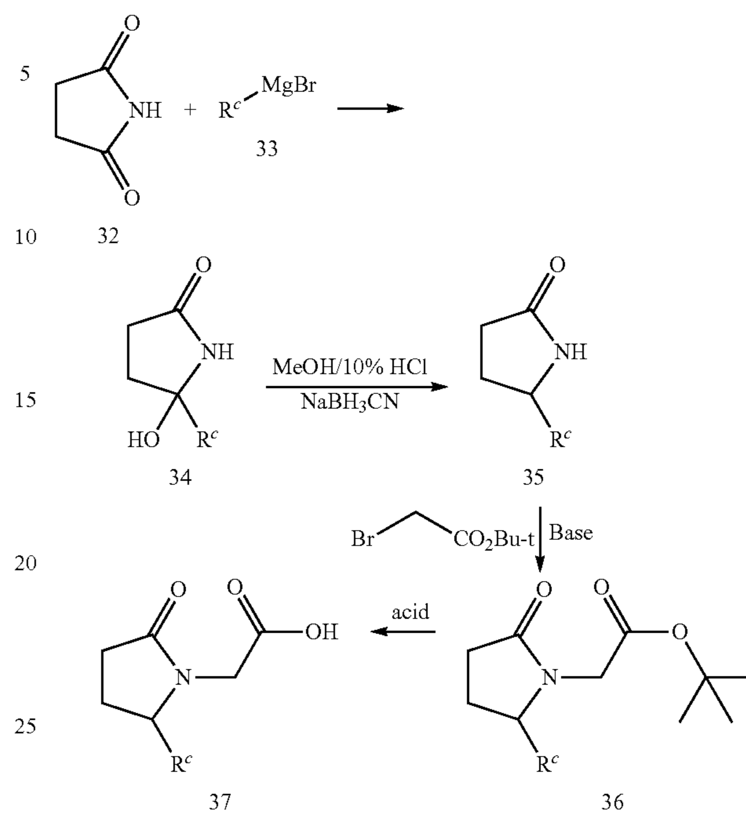
Scheme 9
