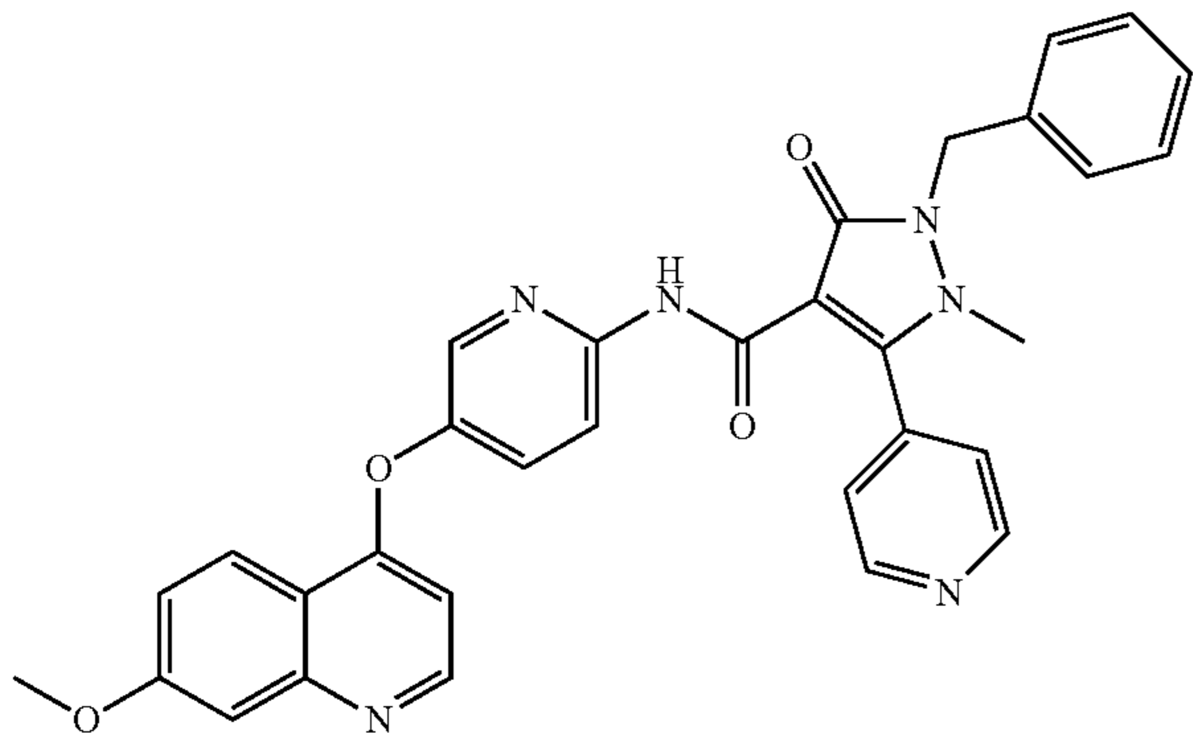
2-benzyl-N-(5-(7-methoxyquinolin-4-yloxy)pyridin-2-yl)-1-methyl-3-oxo-5-(pyridin-4-yl)-2,3-dihydro-1H-pyrazole-4-carboxamide MS (ESI pos. ion) m/z 559 (MH + ). Calc'd exact mass for C 32 H 26 N 6 O 4 558.
