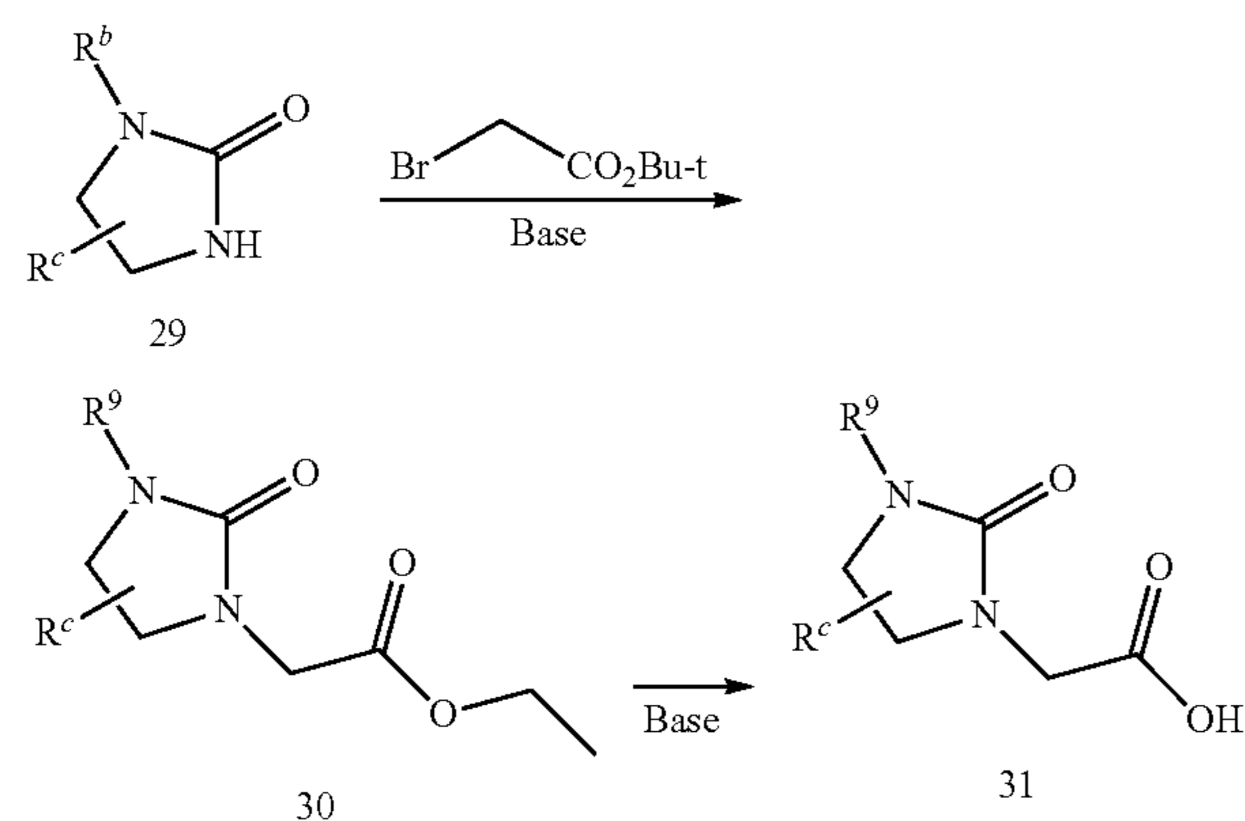
Scheme 8
