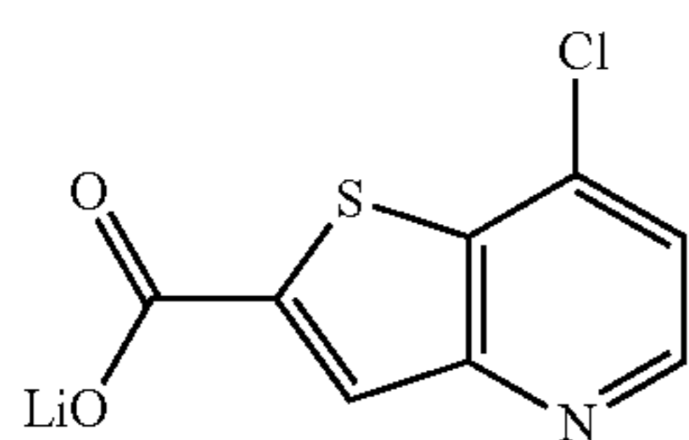
Step 5: lithium 7-chlorothieno[3,2-b]pyridine-2-carboxylate
