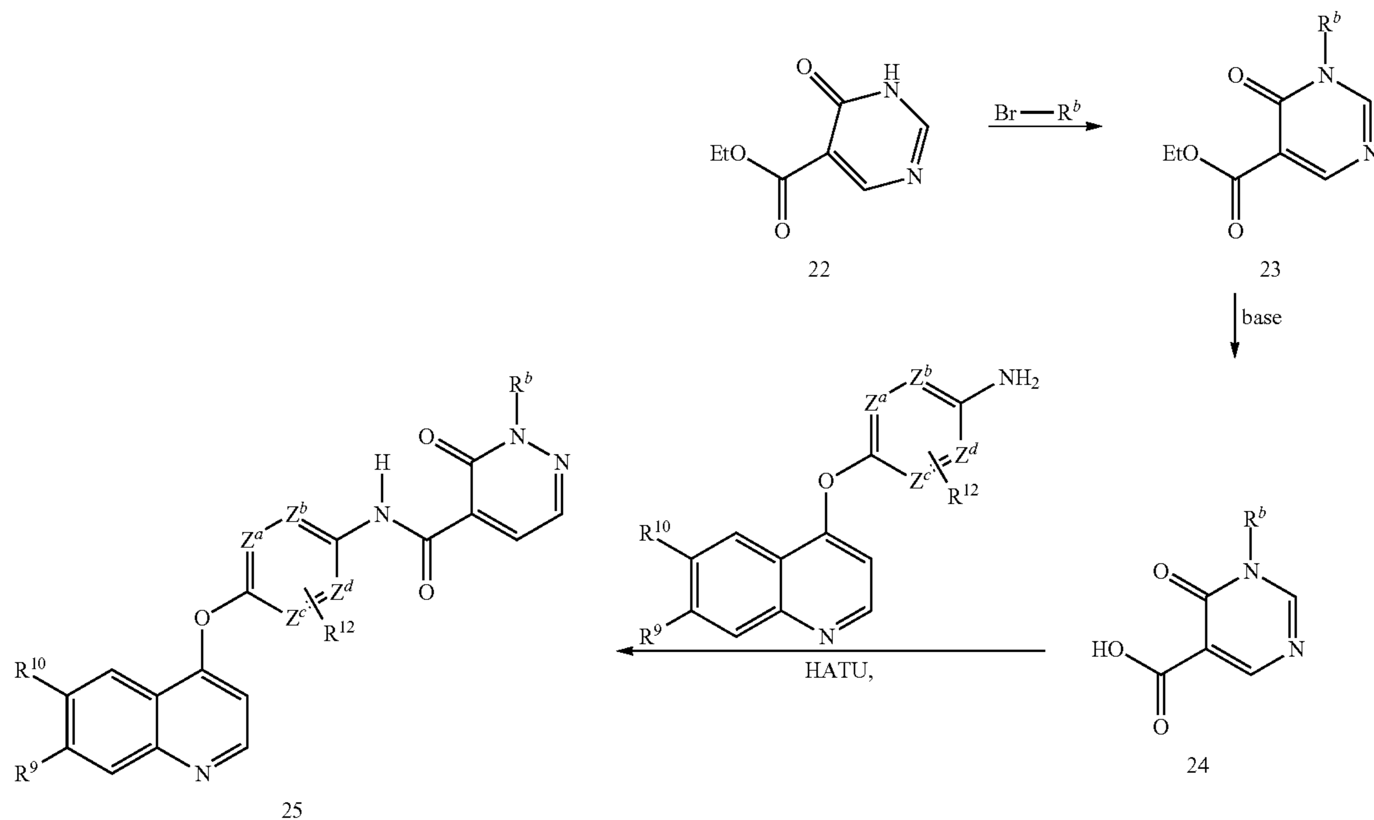
Scheme 6
