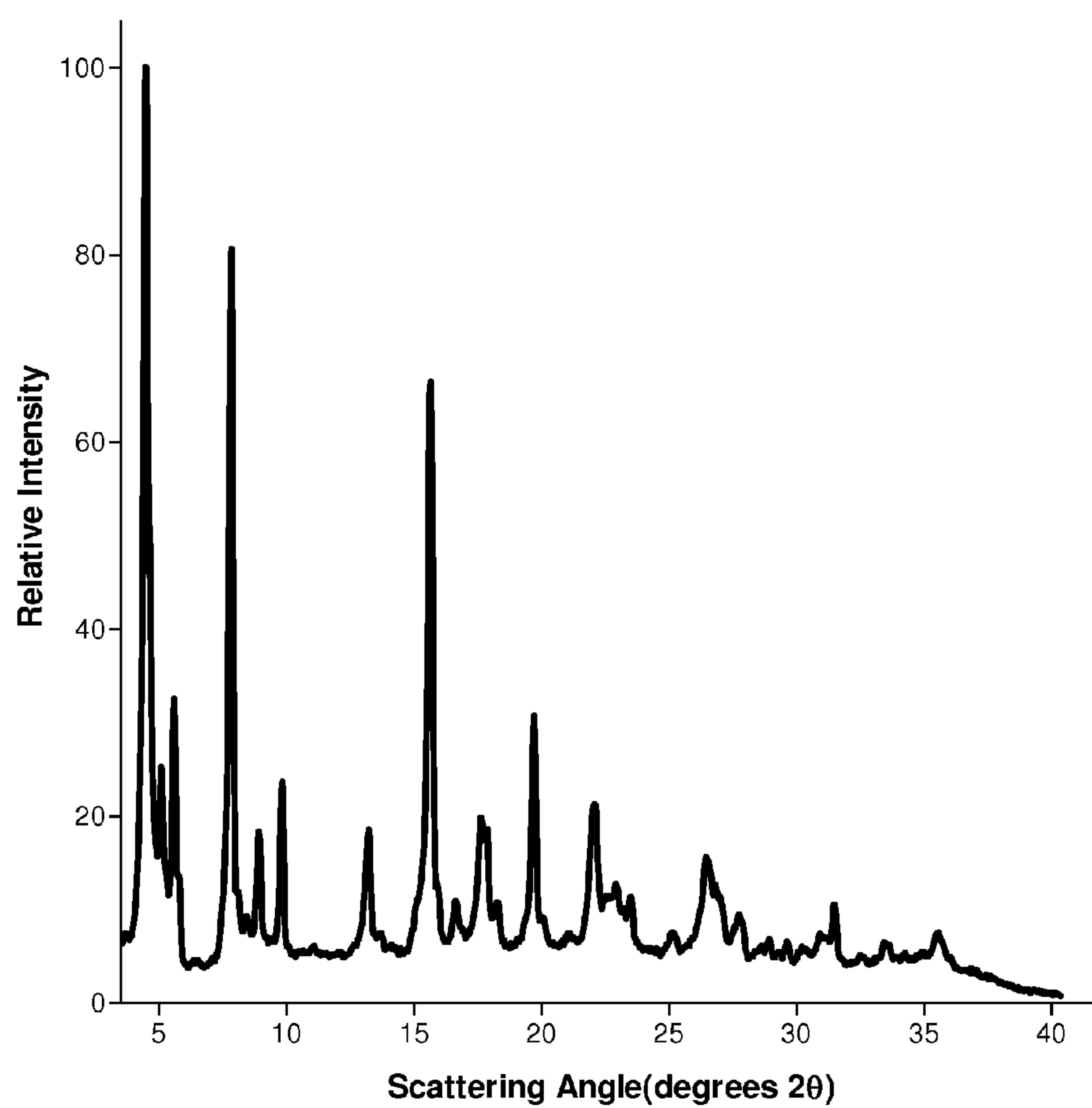
FIG. 3 X-ray powder diffraction pattern of the cocystal product formed by acetylsalicylic acid and L-theanine.
