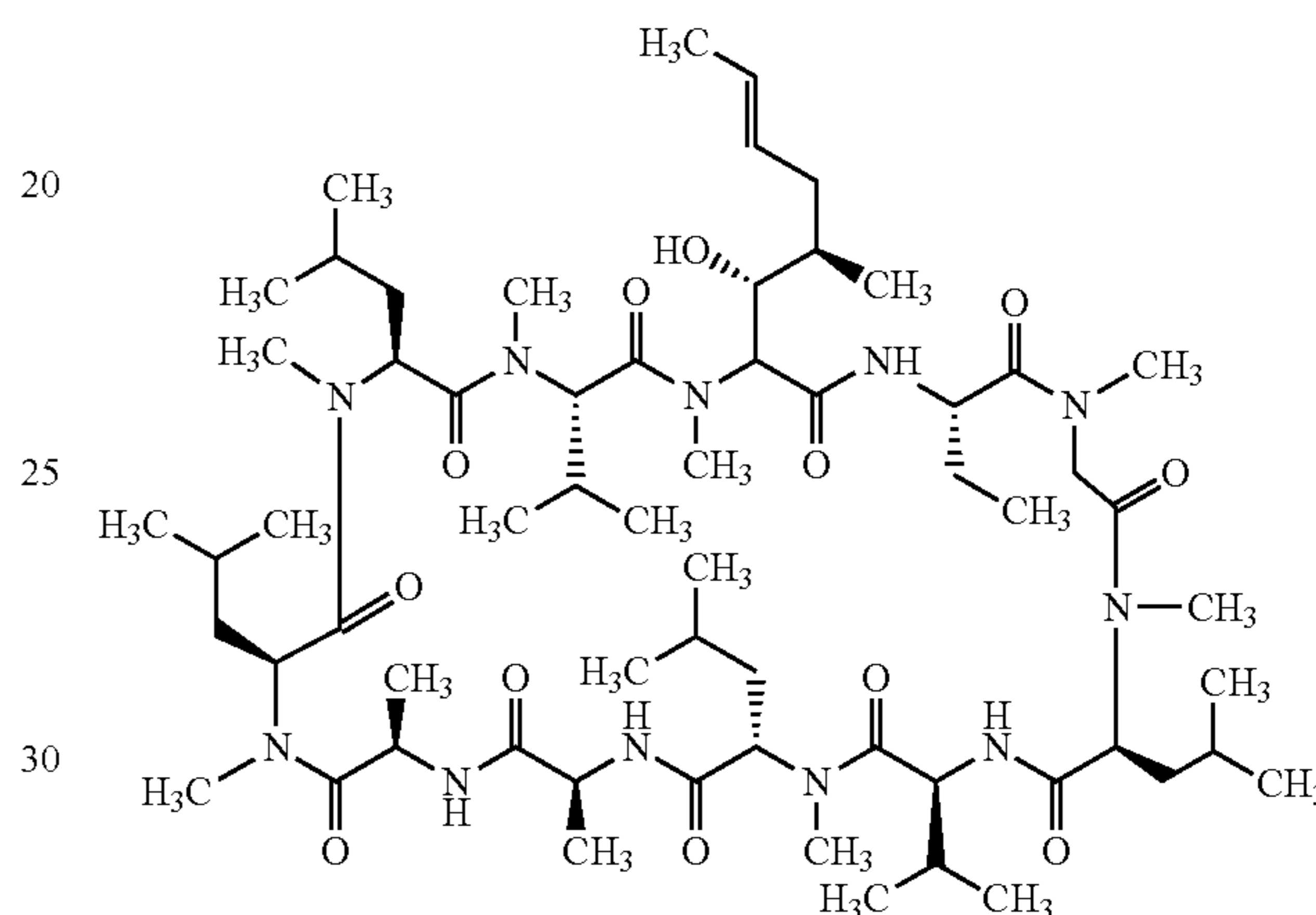
Formula 1
