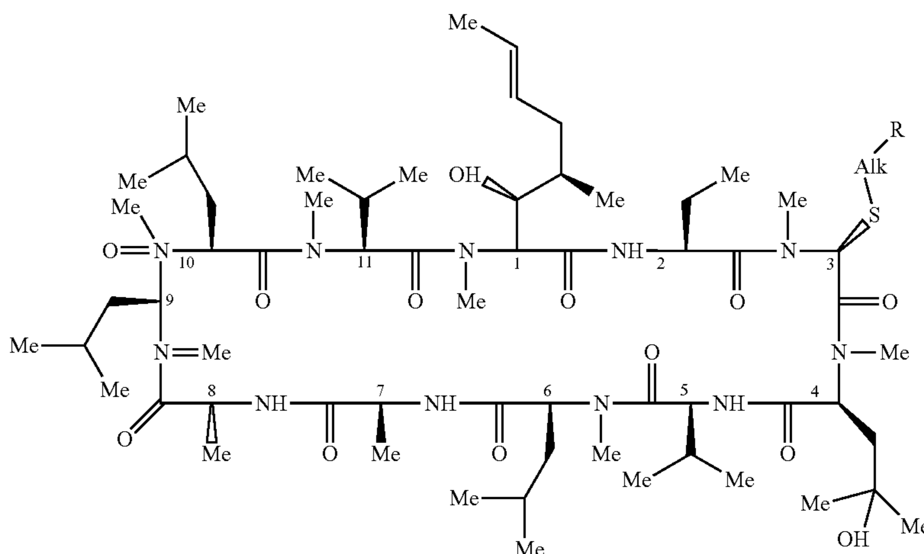
Formula II
