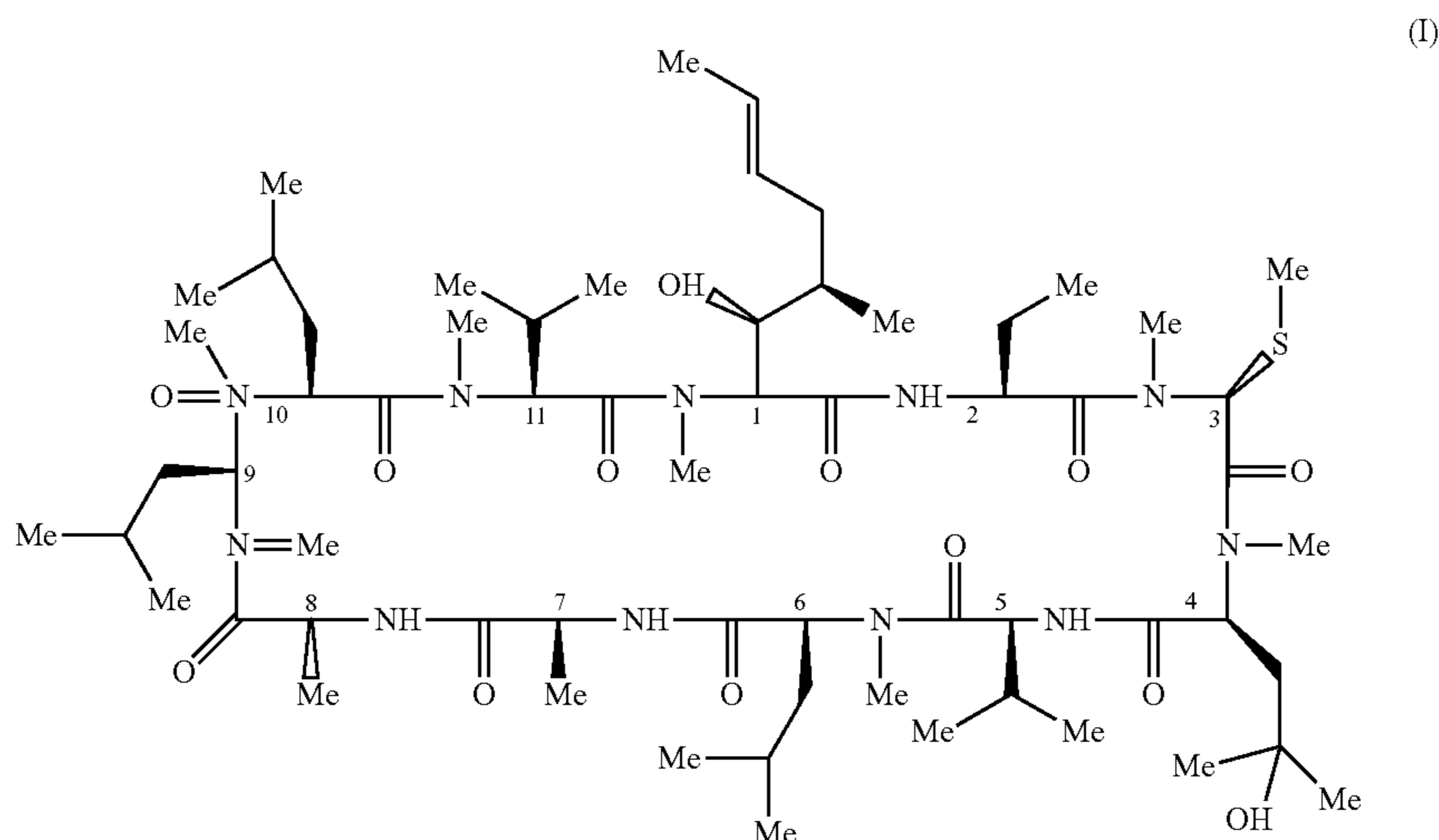
Formula IV
