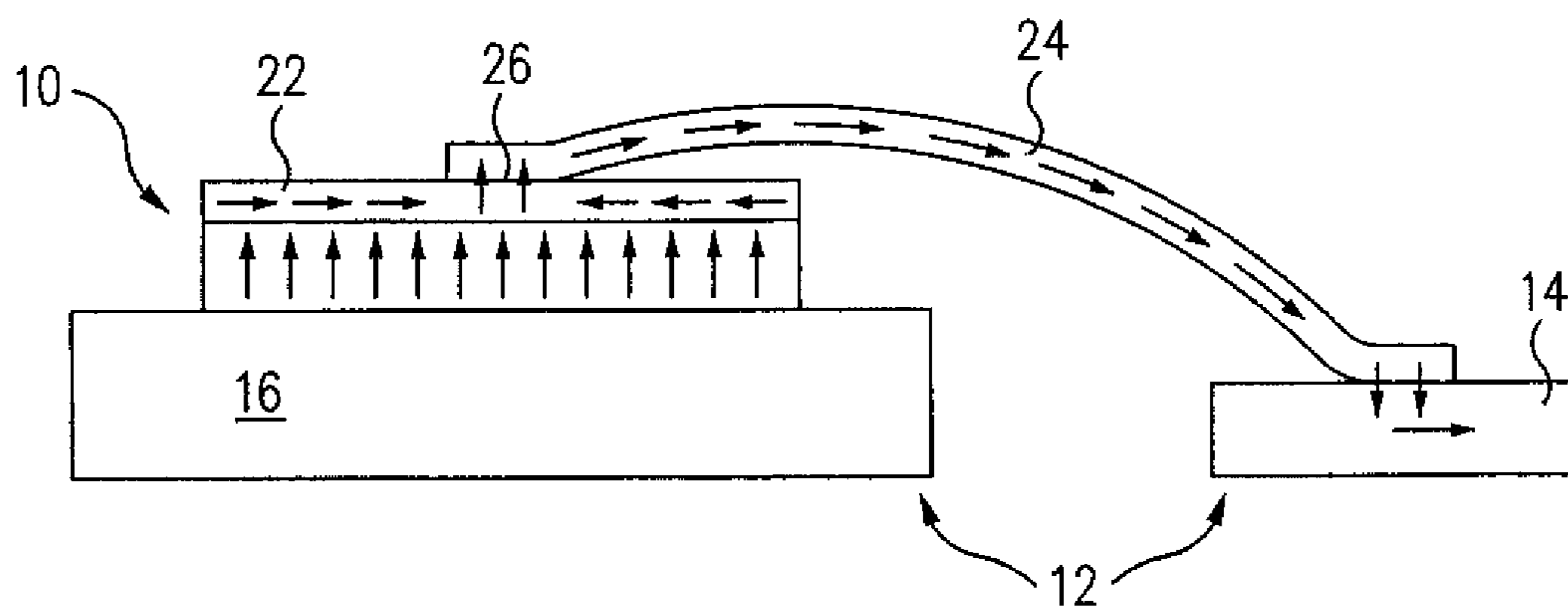
FIG. 1 (PRIOR ART)
