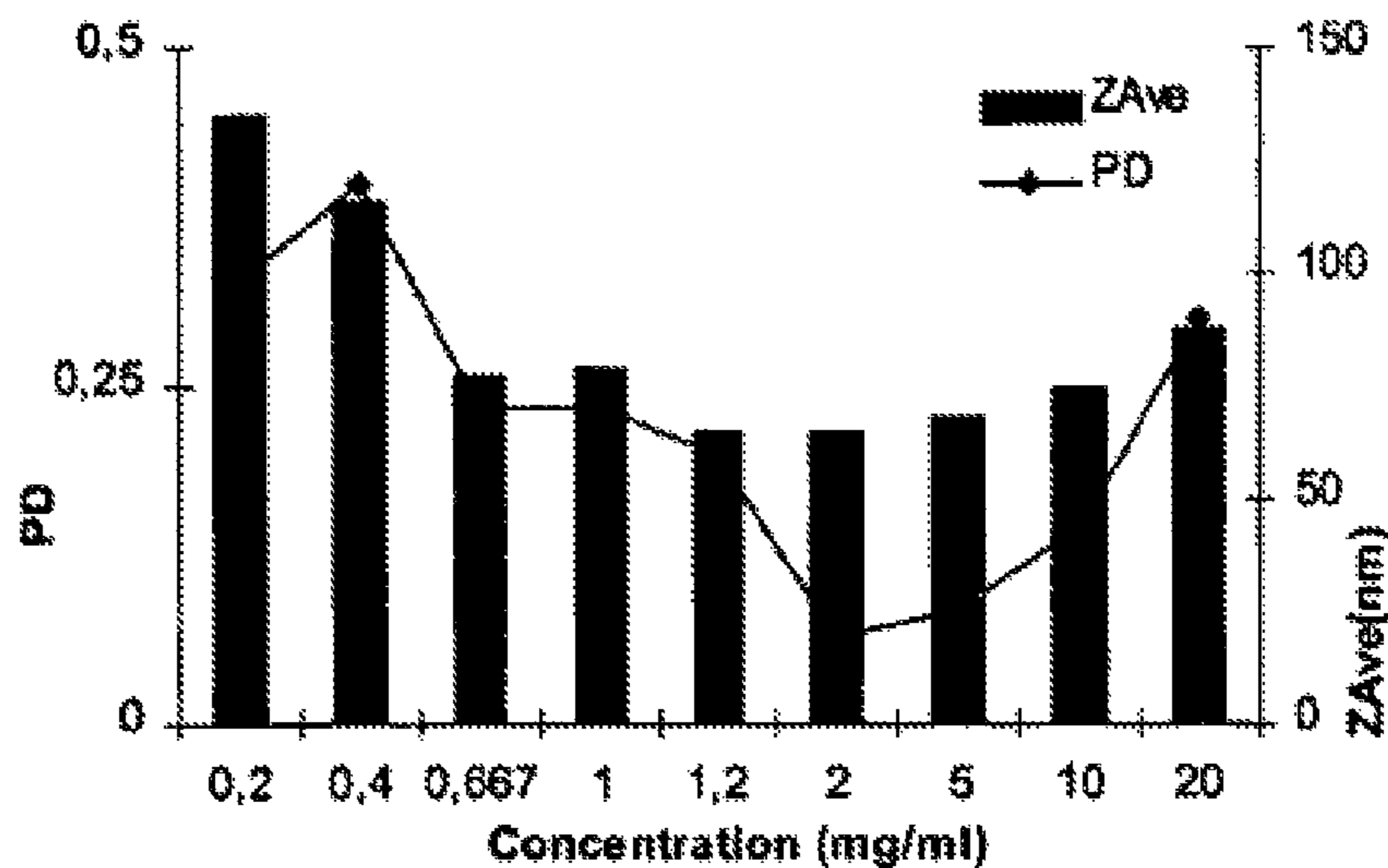
Particle size ( Z_{ave} ) and polydispersity (PD) versus concentration of PEG- b - (80%HEMA-Lac 2 -20%HEMAM-Lac 4 ) solutions.
