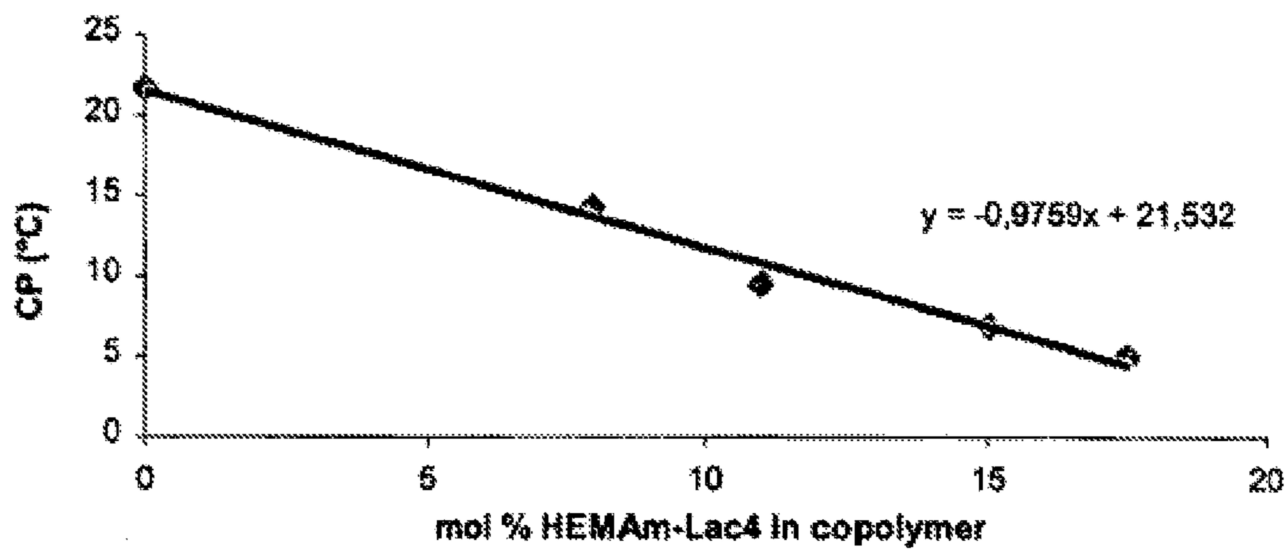
CP (°C) of HEMAm-Lac 2 copolymers as a function of the mole % of HEMAm-Lac 4 in the copolymer.
