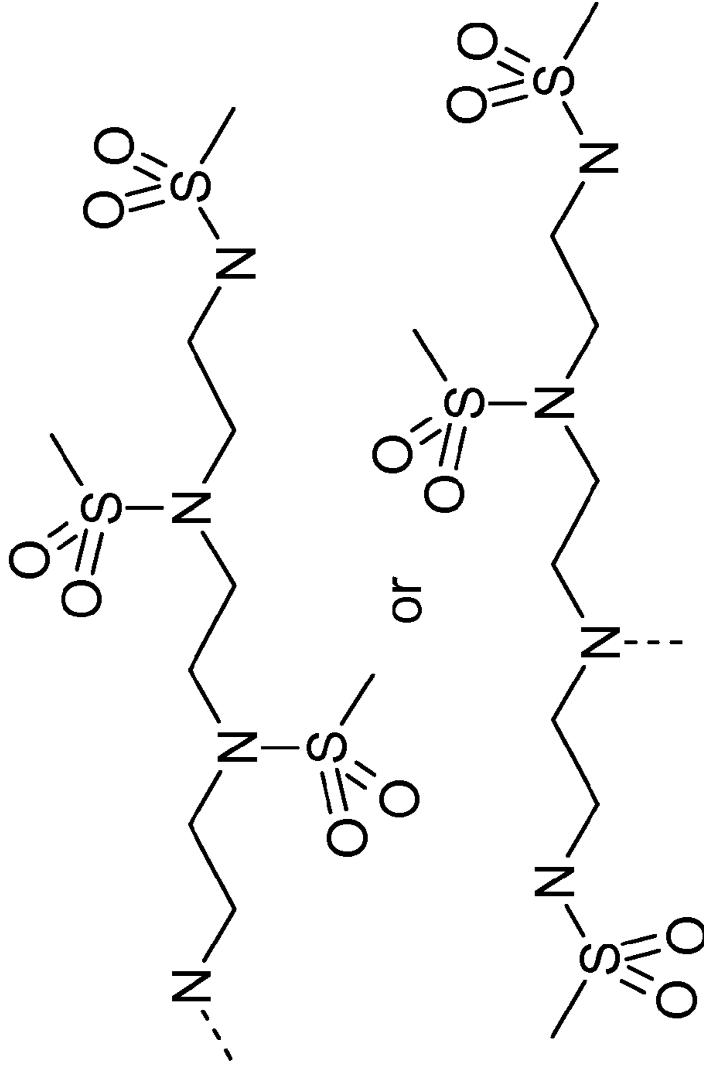
Triethylenetetramine
