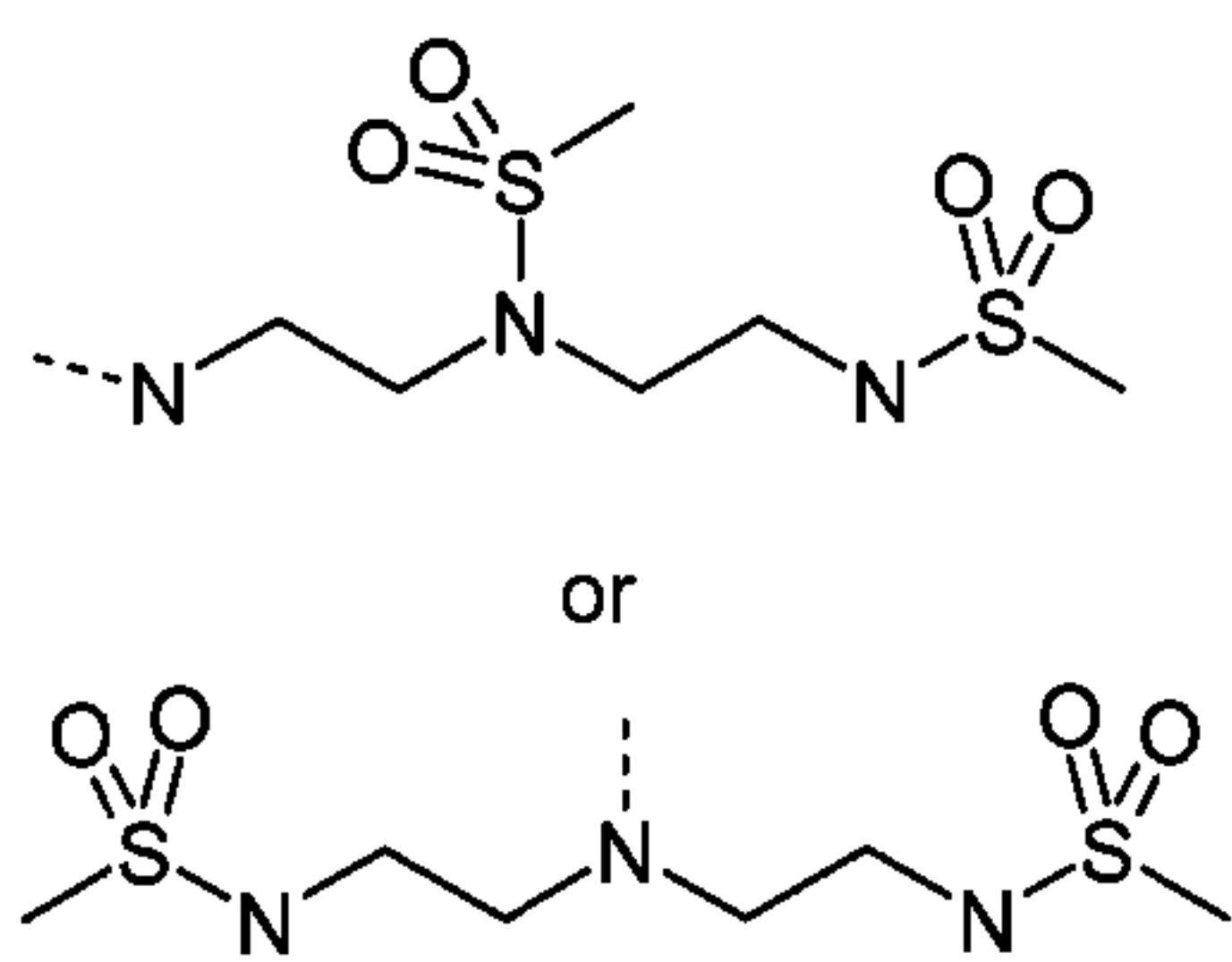
Diethylenetriamine
