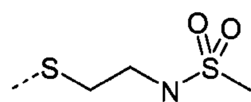
Cysteamine
