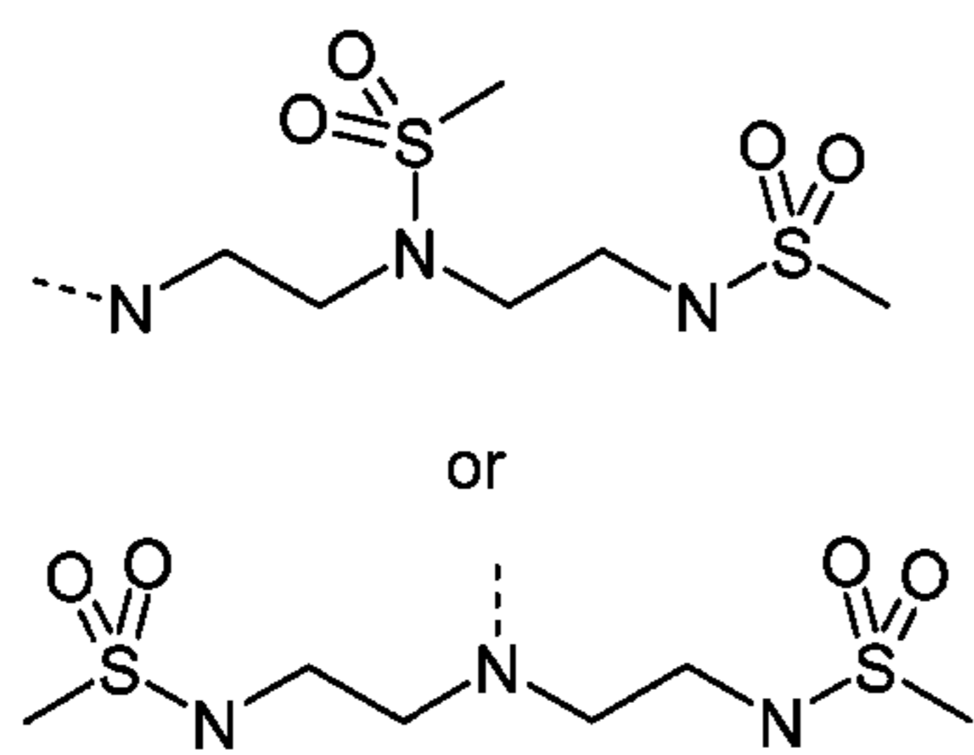
Diethylenetriamine
