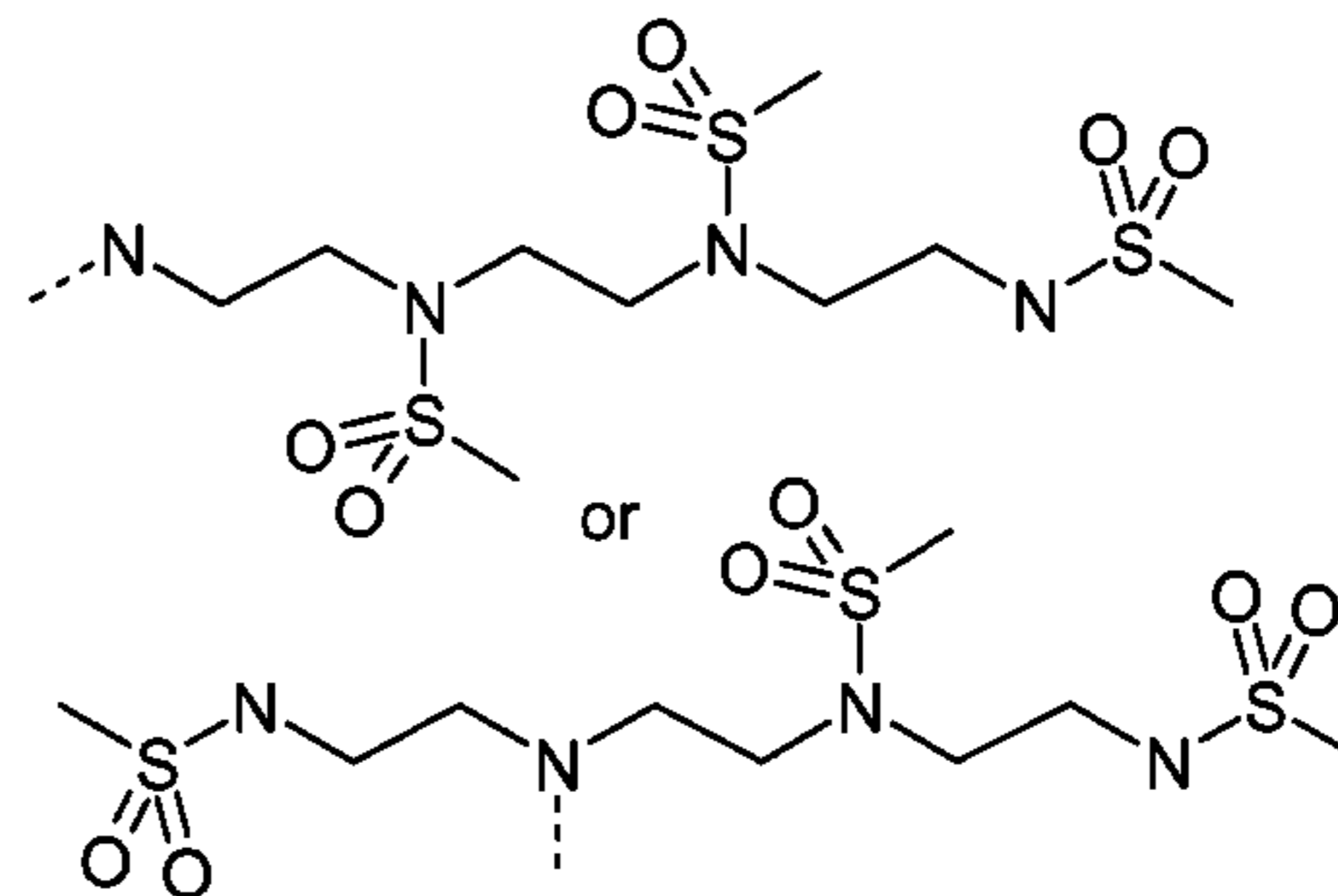
Triethylenetetramine
