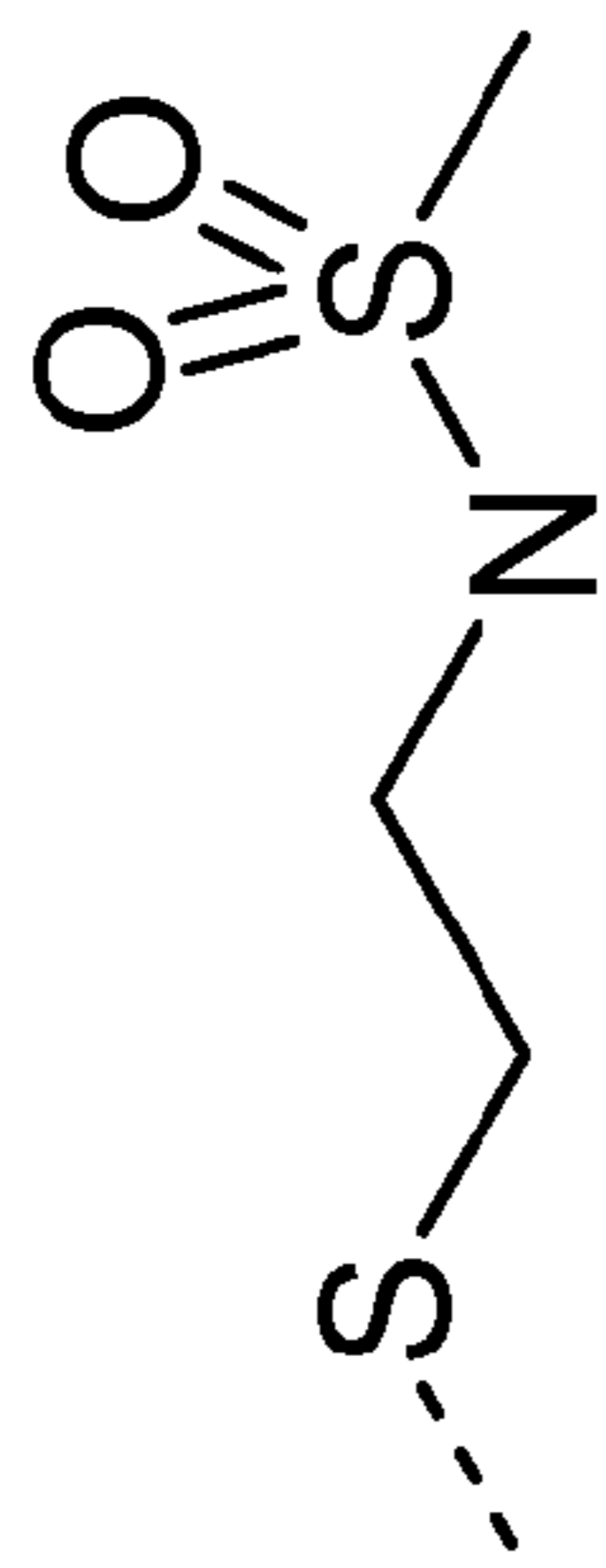
Cysteamine
