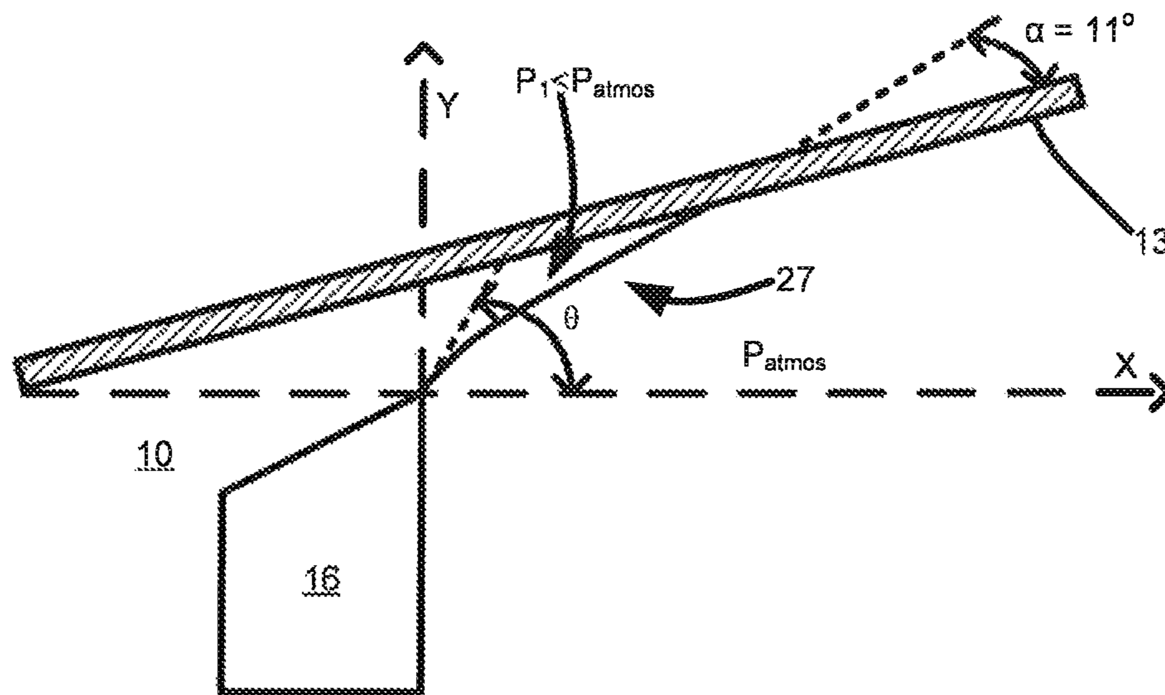
FIG. 3 (Prior Art)
