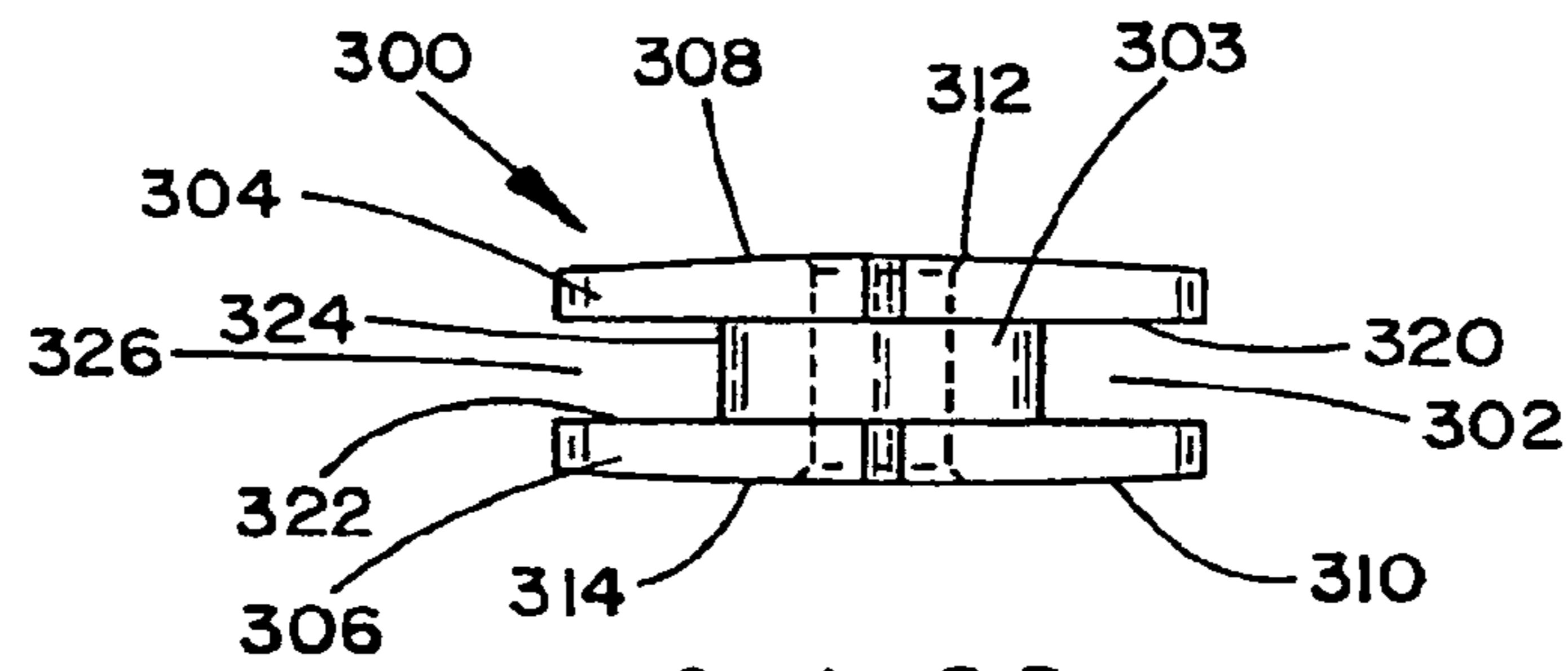
Section B-B
