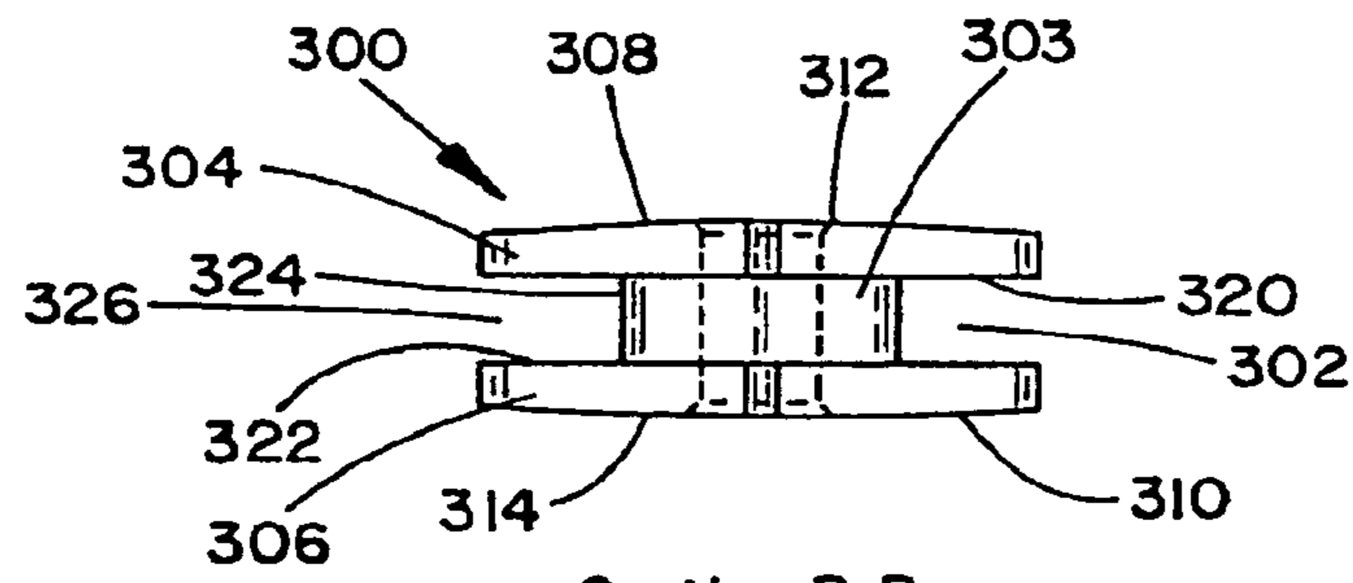
Section B-B
