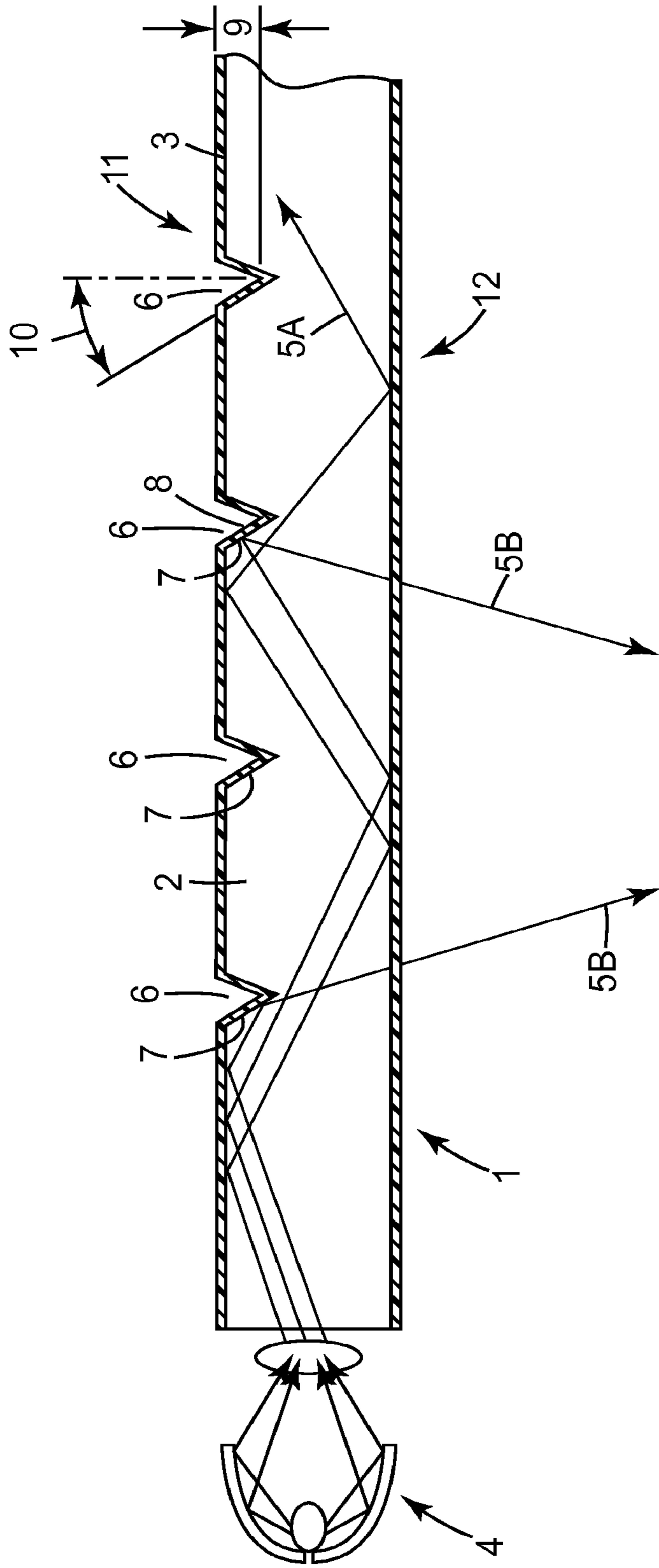
Fig. 1 PRIOR ART
