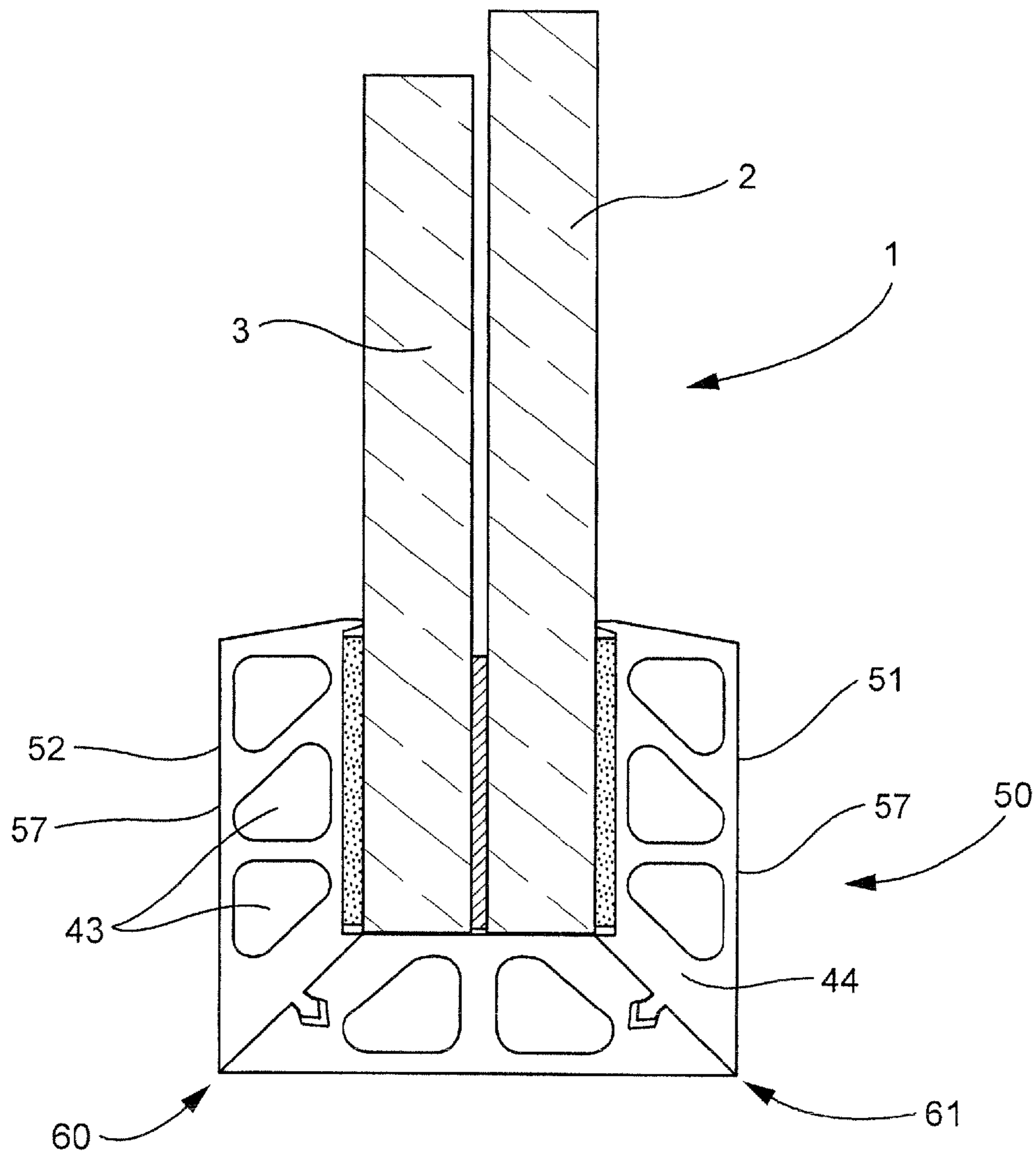
Completed Assy with sides snapped in place and VHB adhesive secured to VIG
