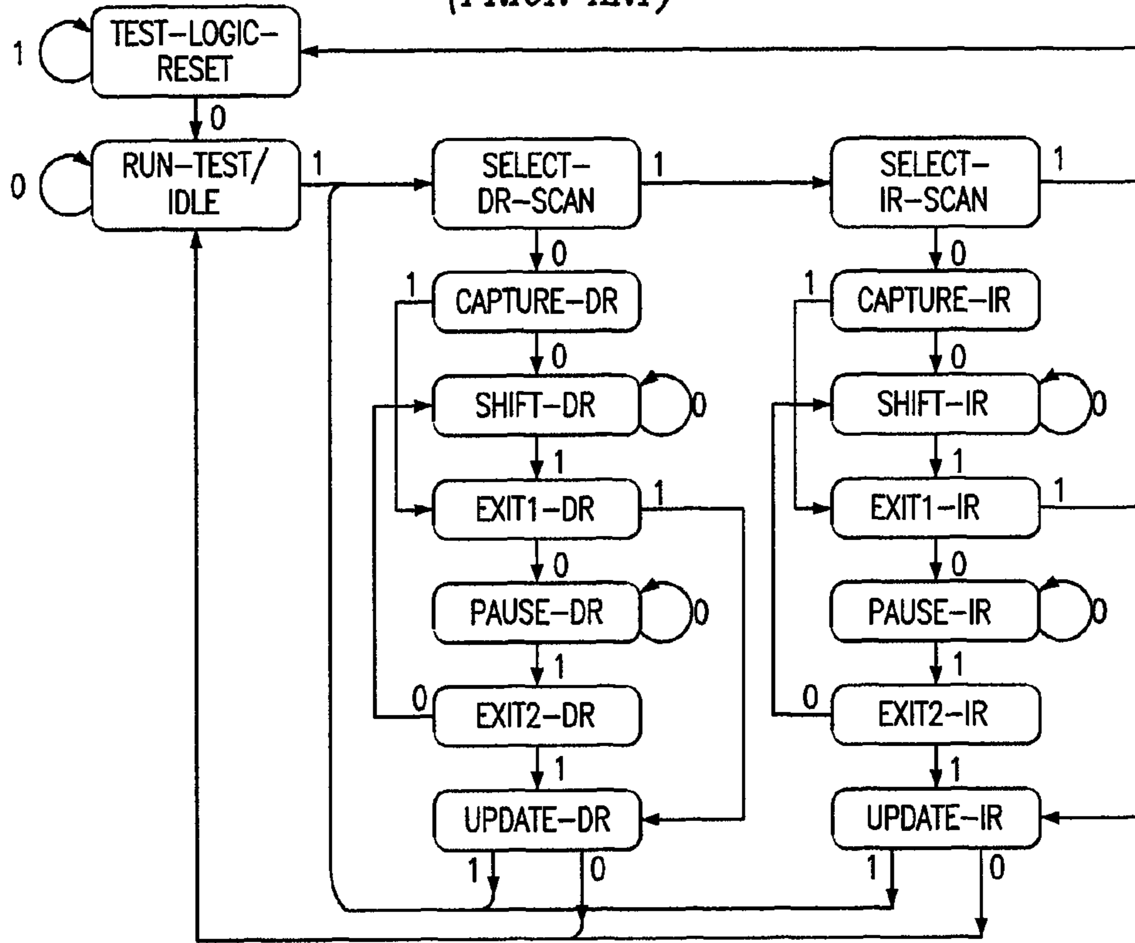
FIG. 14 (PRIOR ART)
