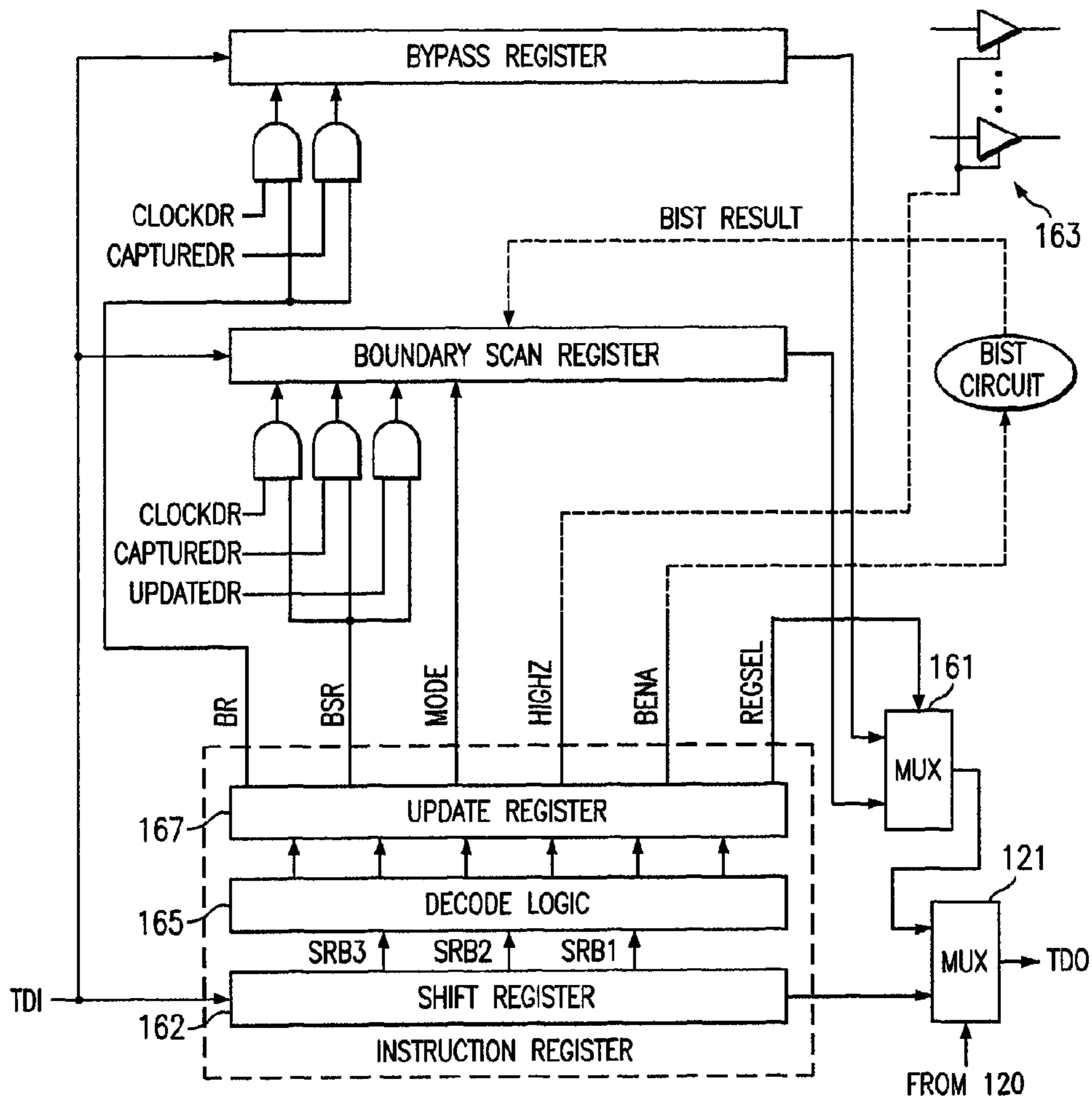
FIG. 16 (PRIOR ART)
