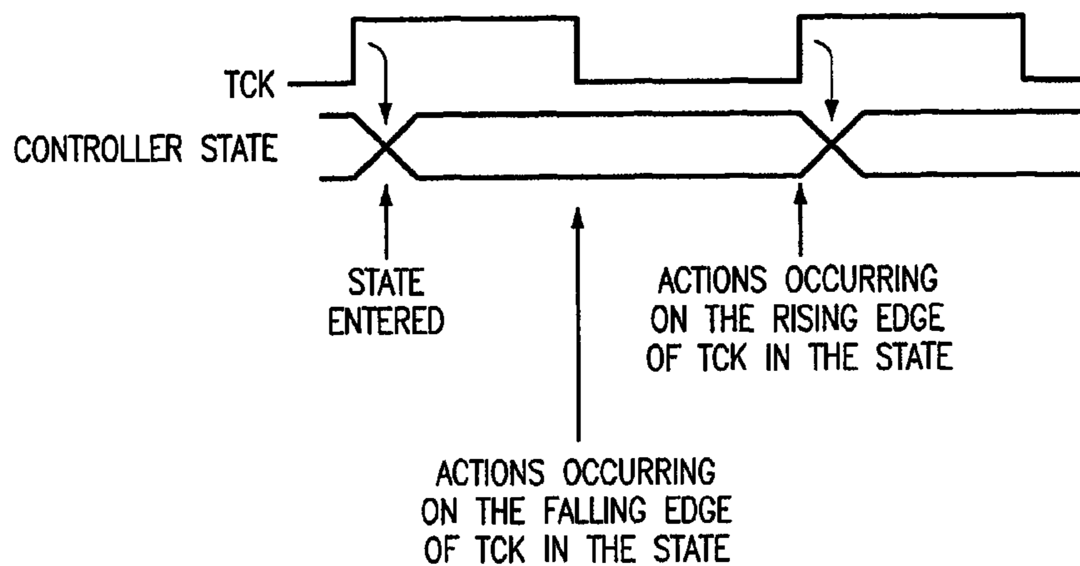
FIG. 15 (PRIOR ART)
