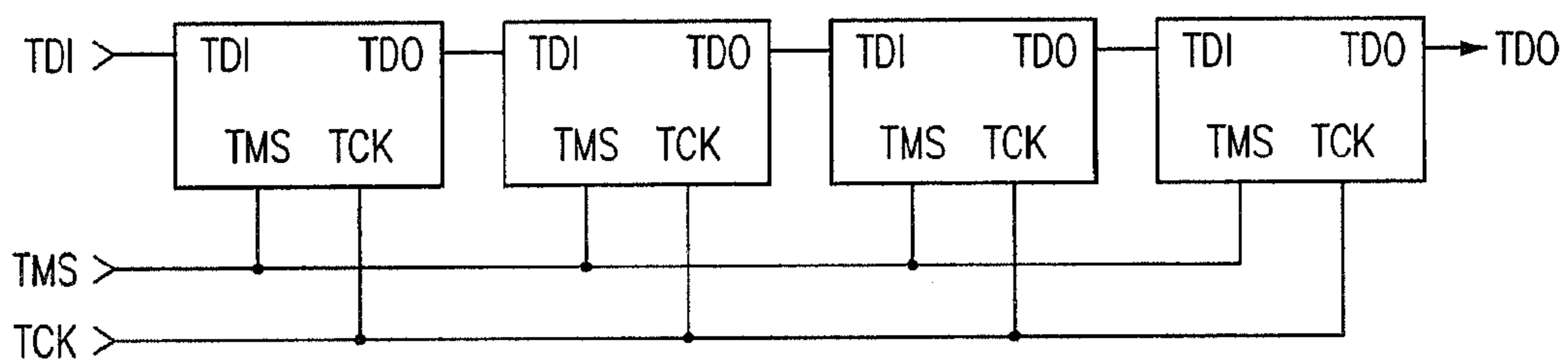
FIG. 13 (PRIOR ART)
