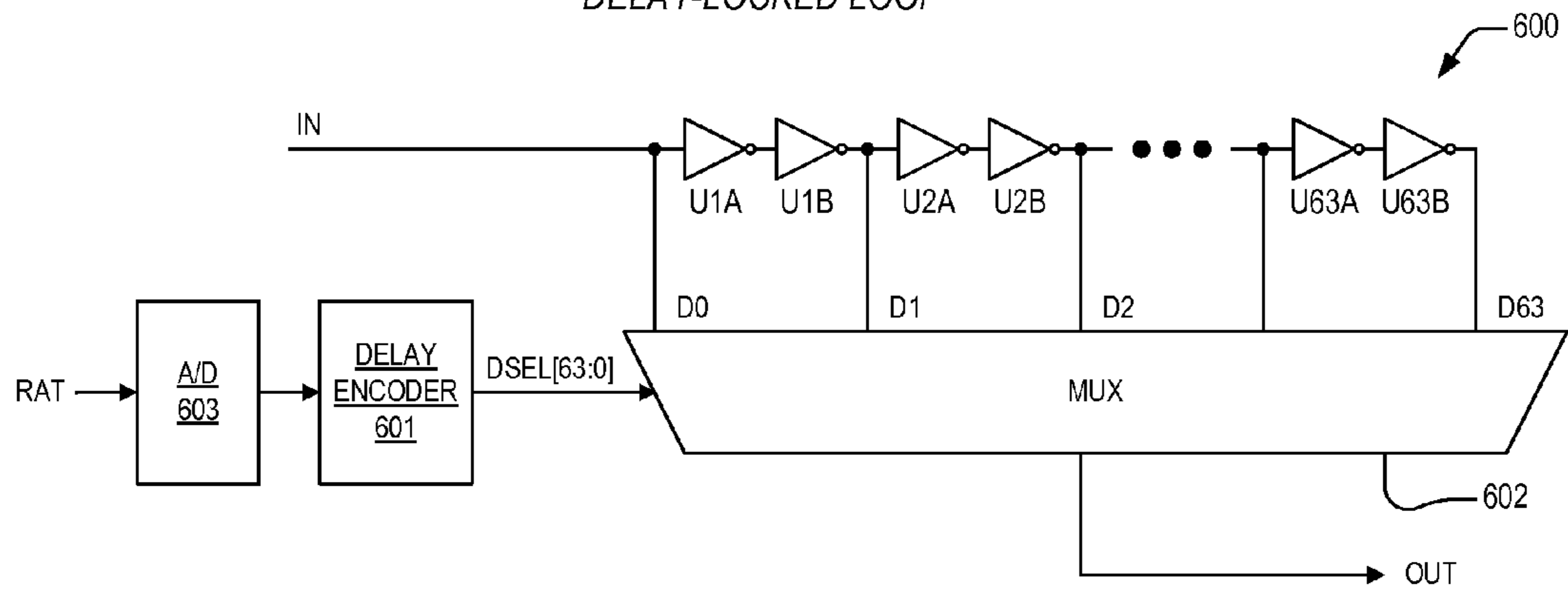
DELAY-LOCKED LOOP
