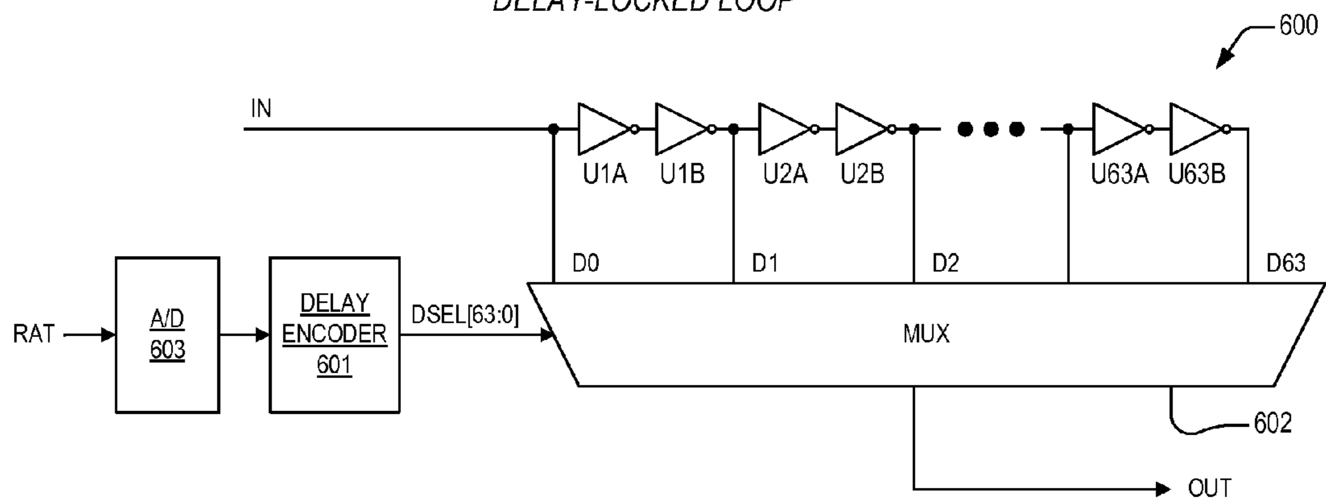
DELAY-LOCKED LOOP
