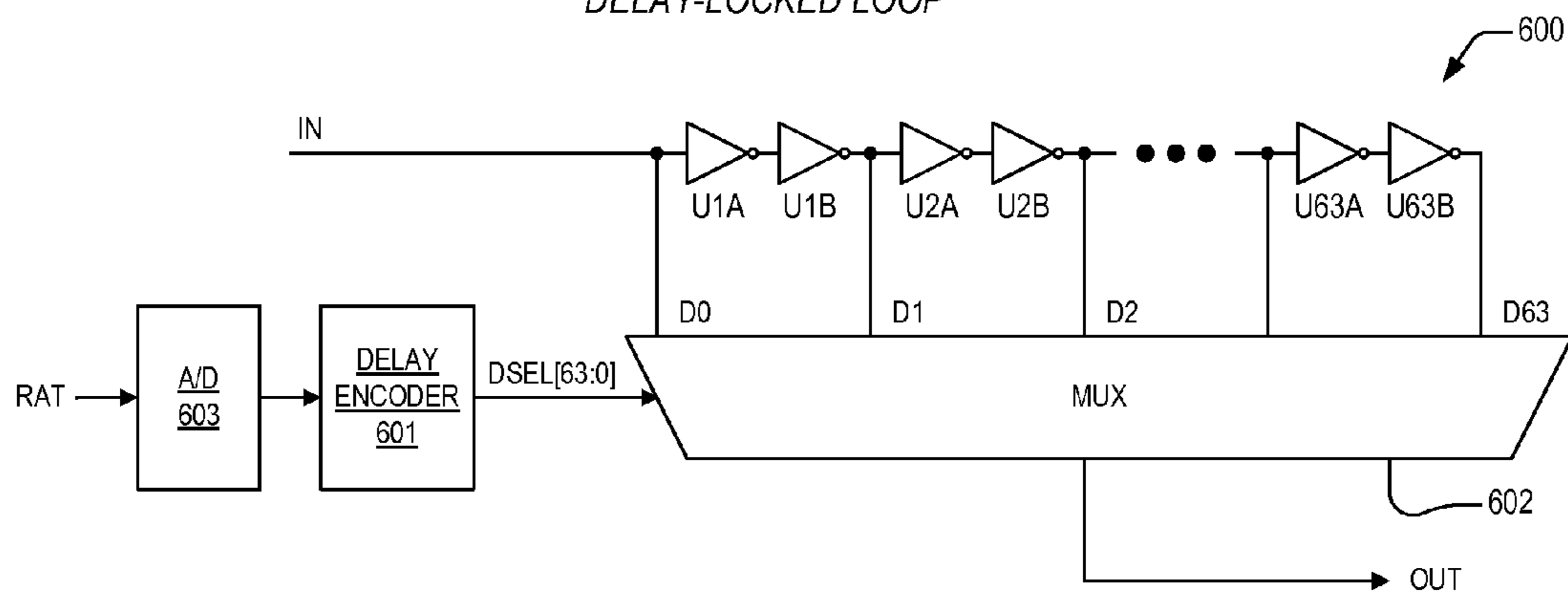
DELAY-LOCKED LOOP
