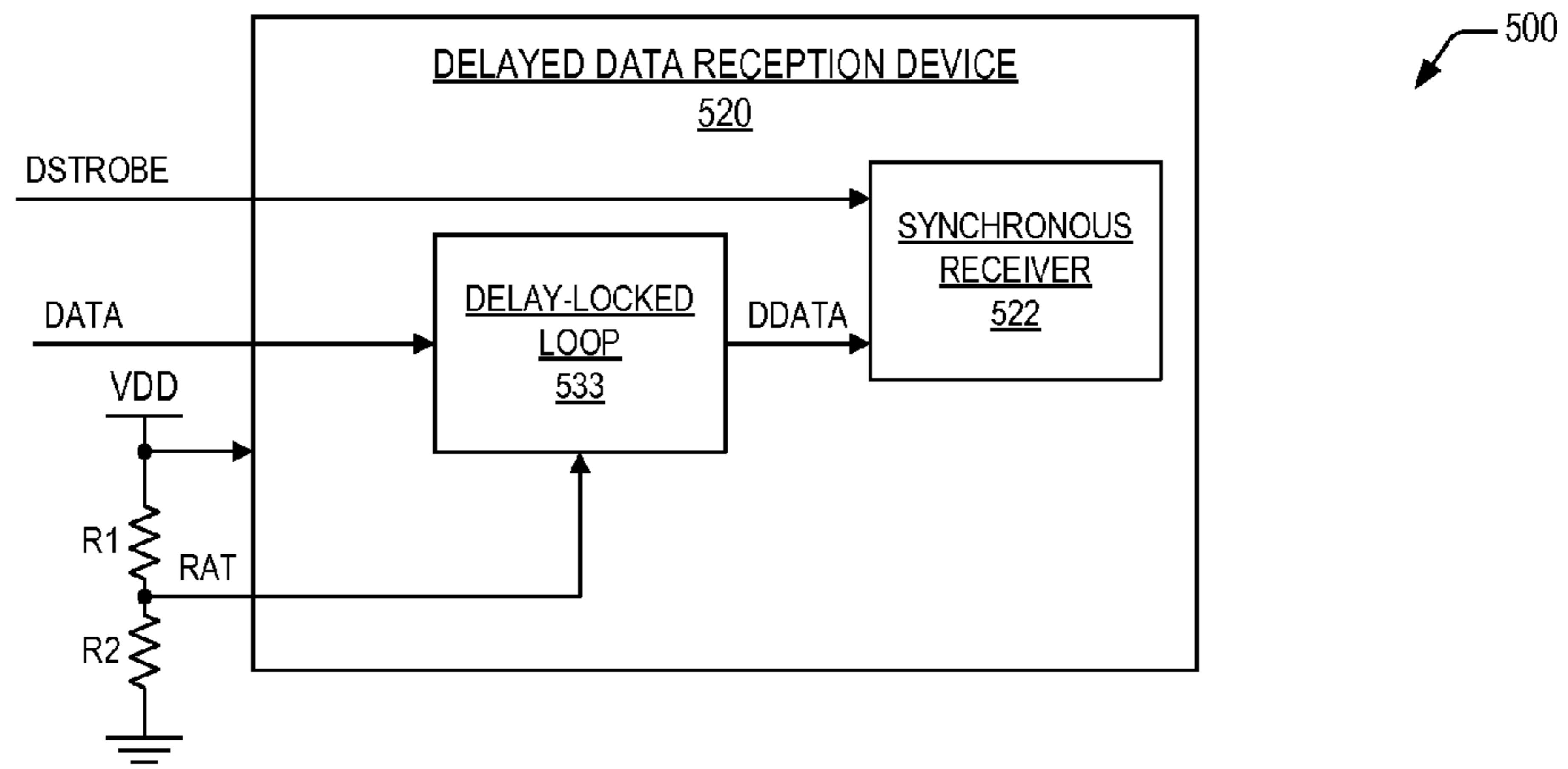
APPARATUS FOR DELAYED SYNCHRONOUS DATA RECEPTION
