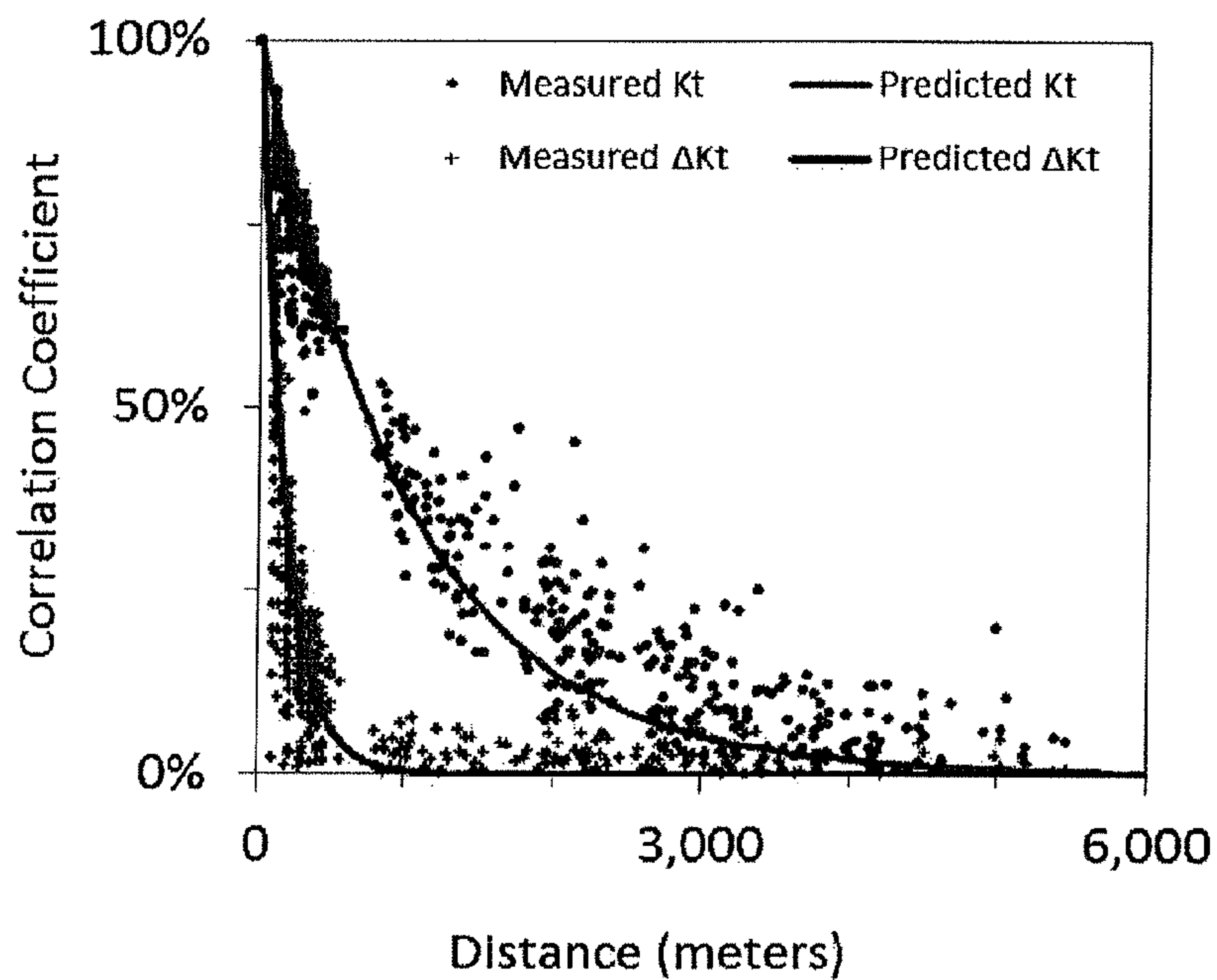
Correlation vs. Distance ( \Delta t=10 )
