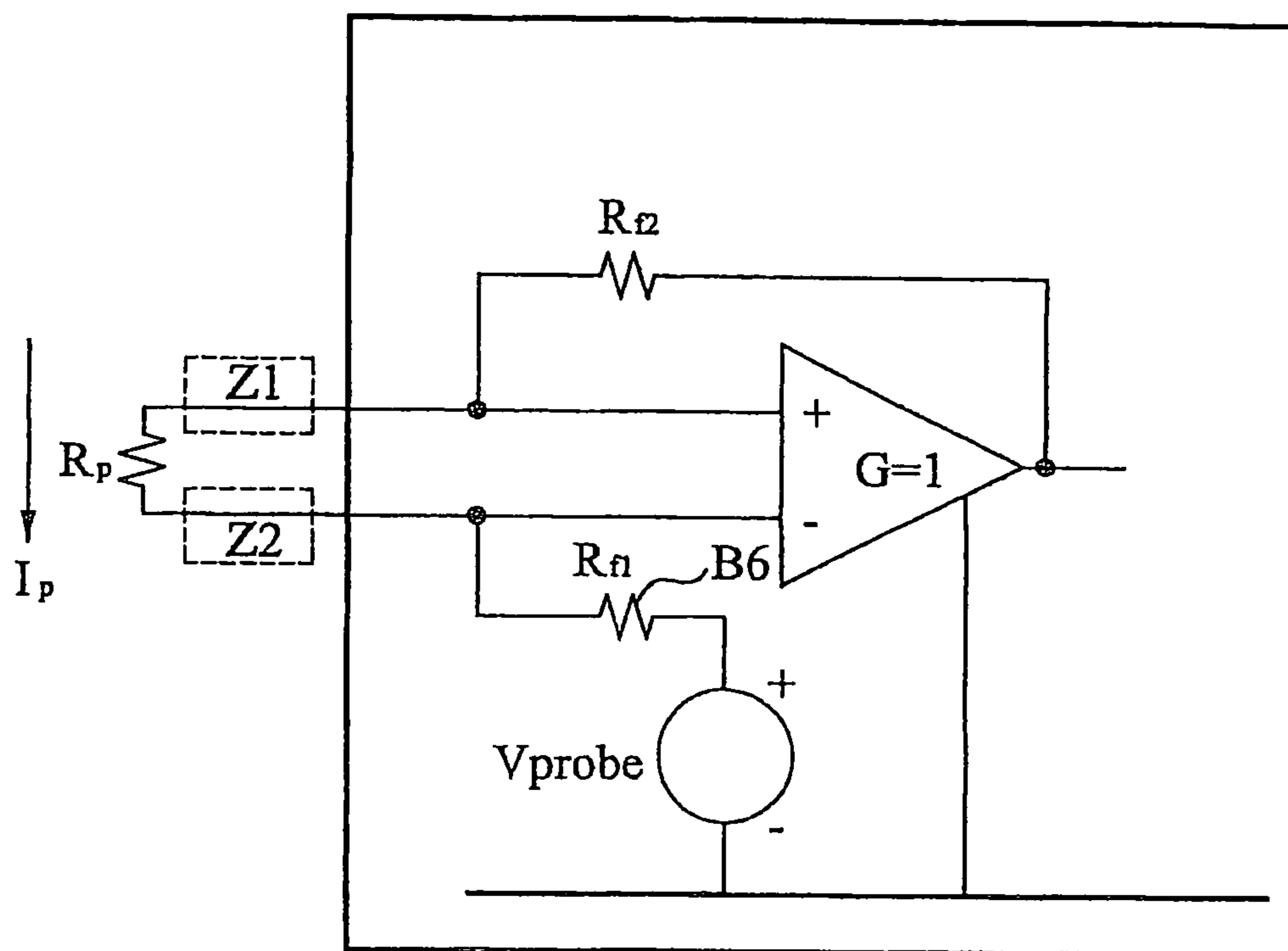
FIG. 1 (CONVENTIONAL ART)
