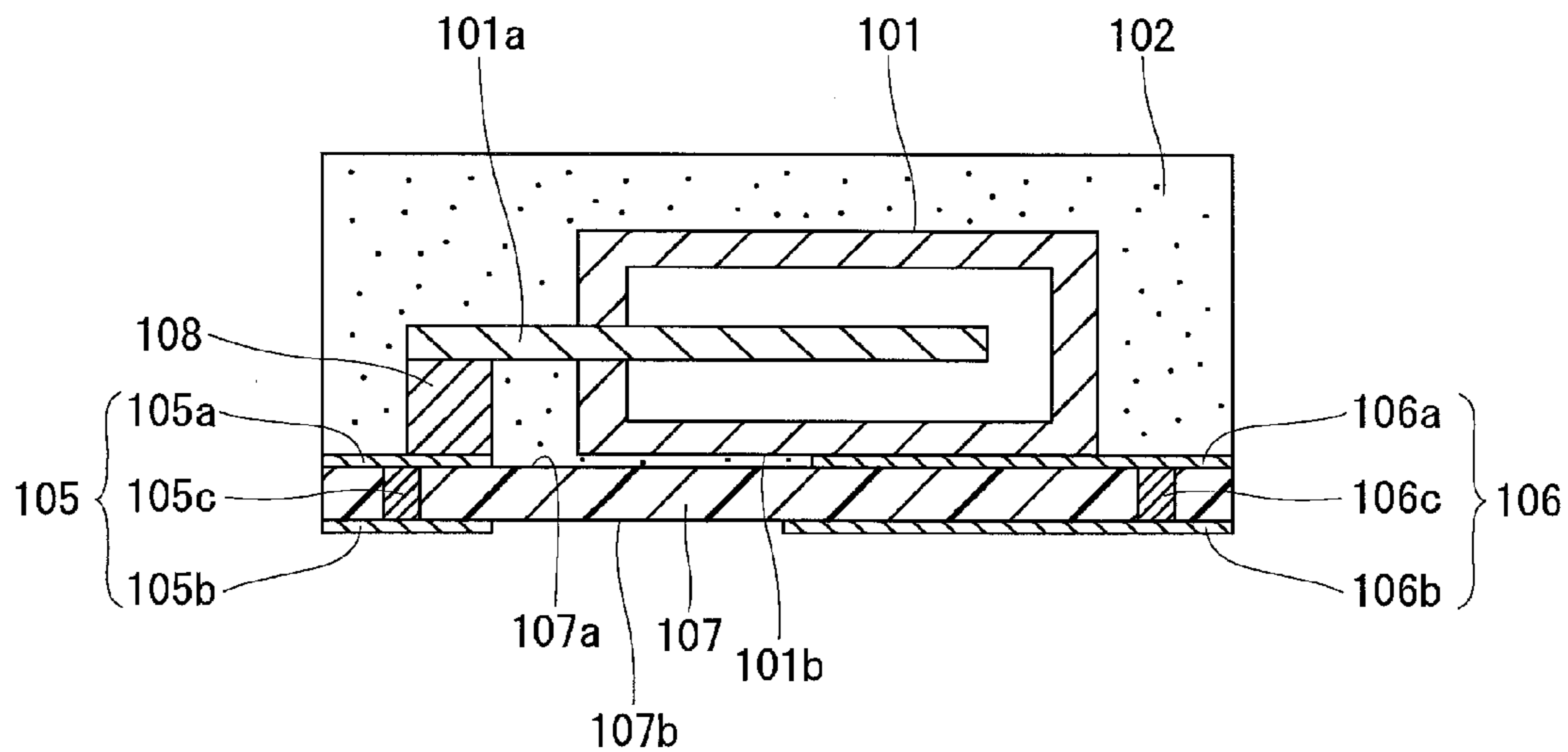
FIG. 13 PRIOR ART
