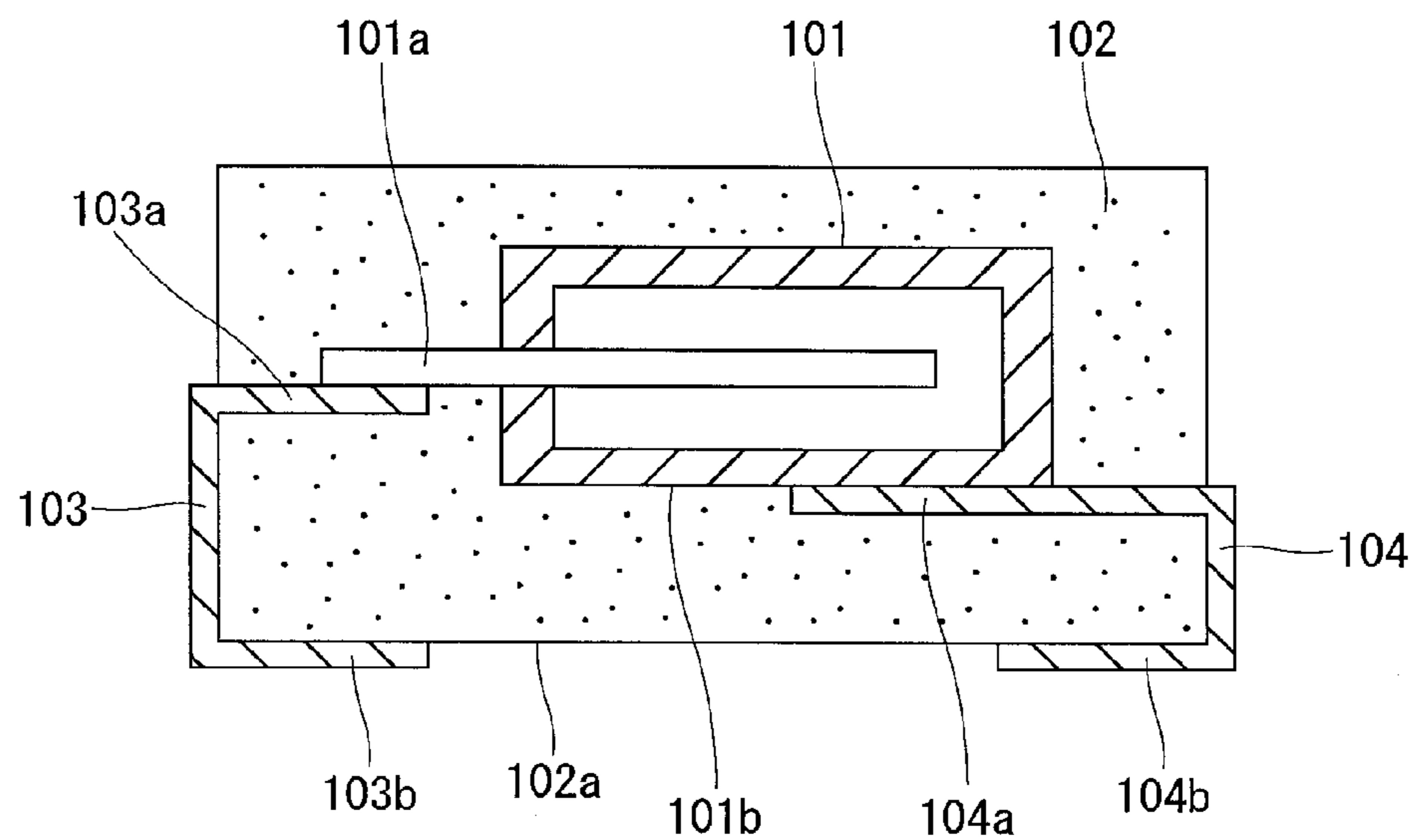
FIG. 12 PRIOR ART
