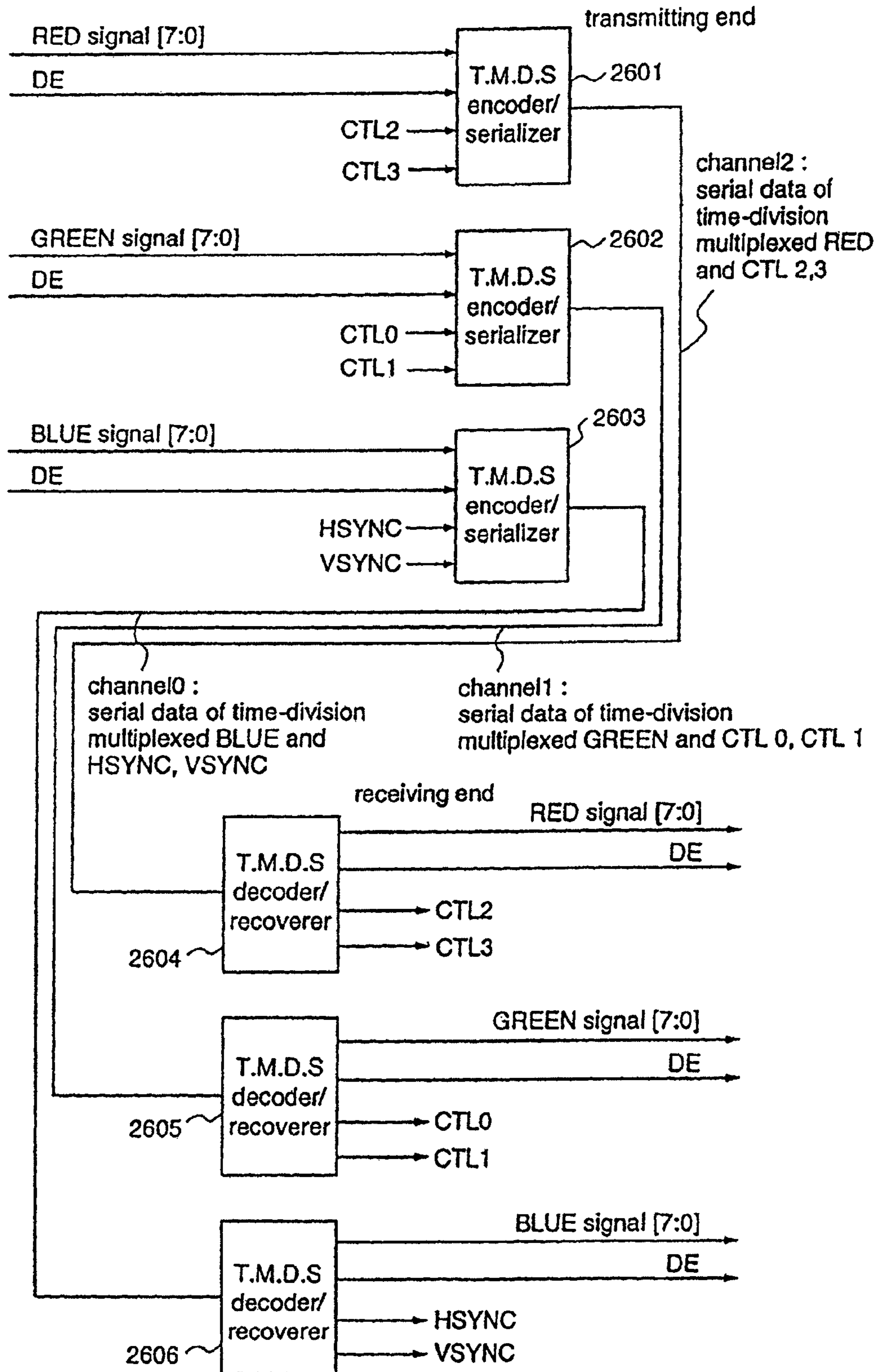
Fig.26 PRIOR ART
