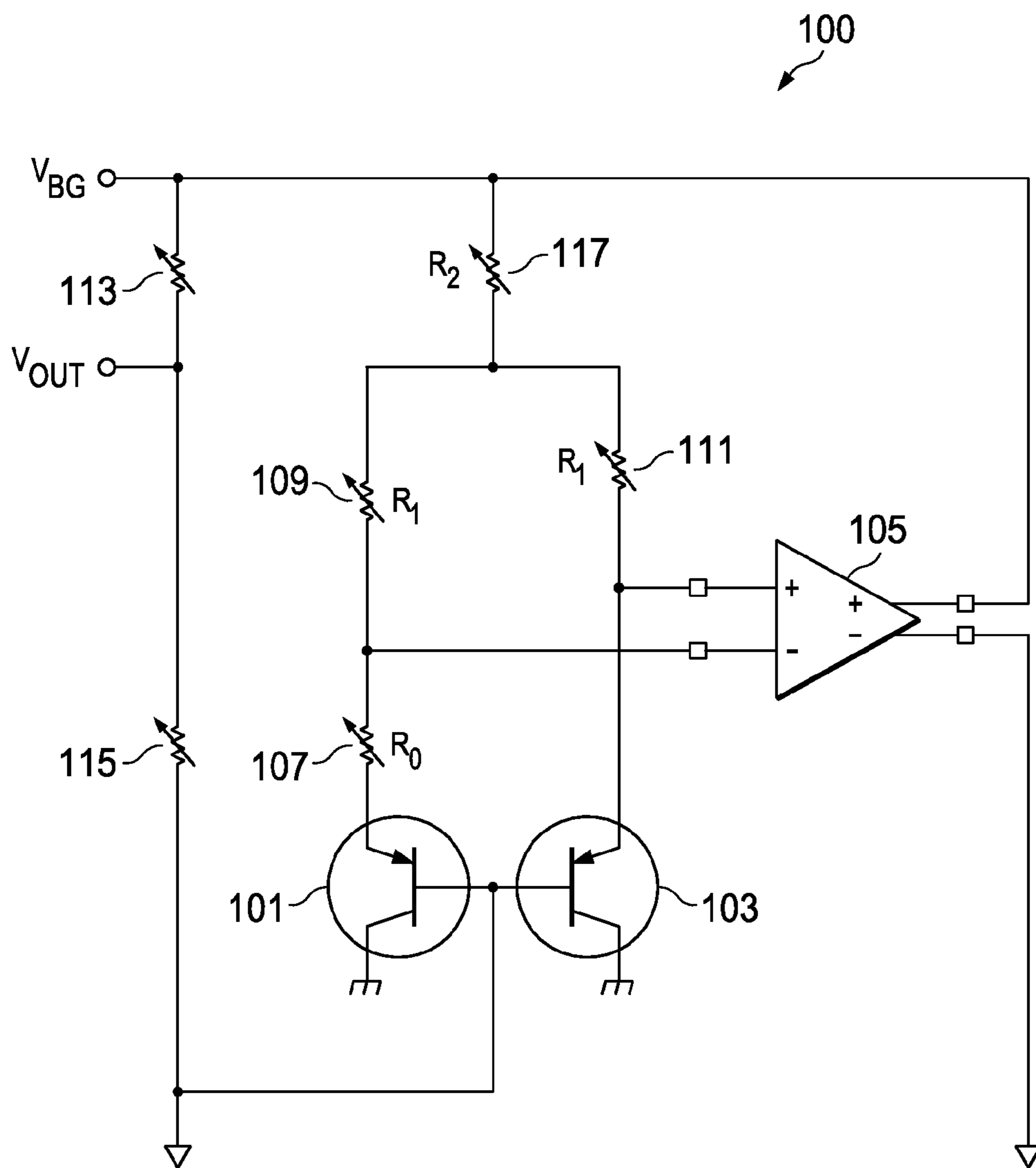
FIG. 1 (PRIOR ART)
