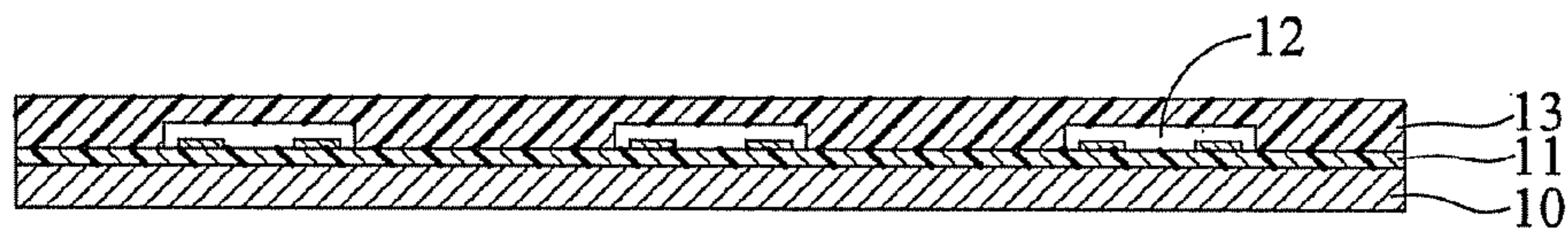
FIG. 1C (PRIOR ART)
