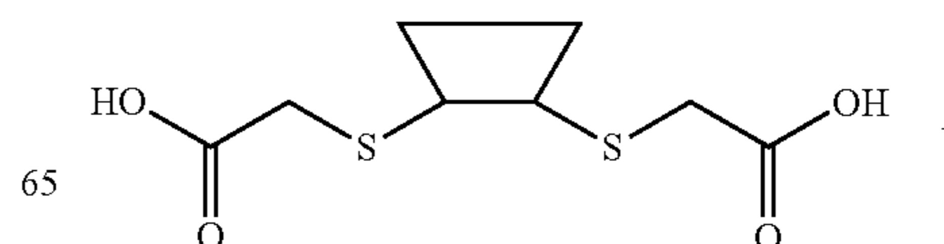
Scheme XXXII
