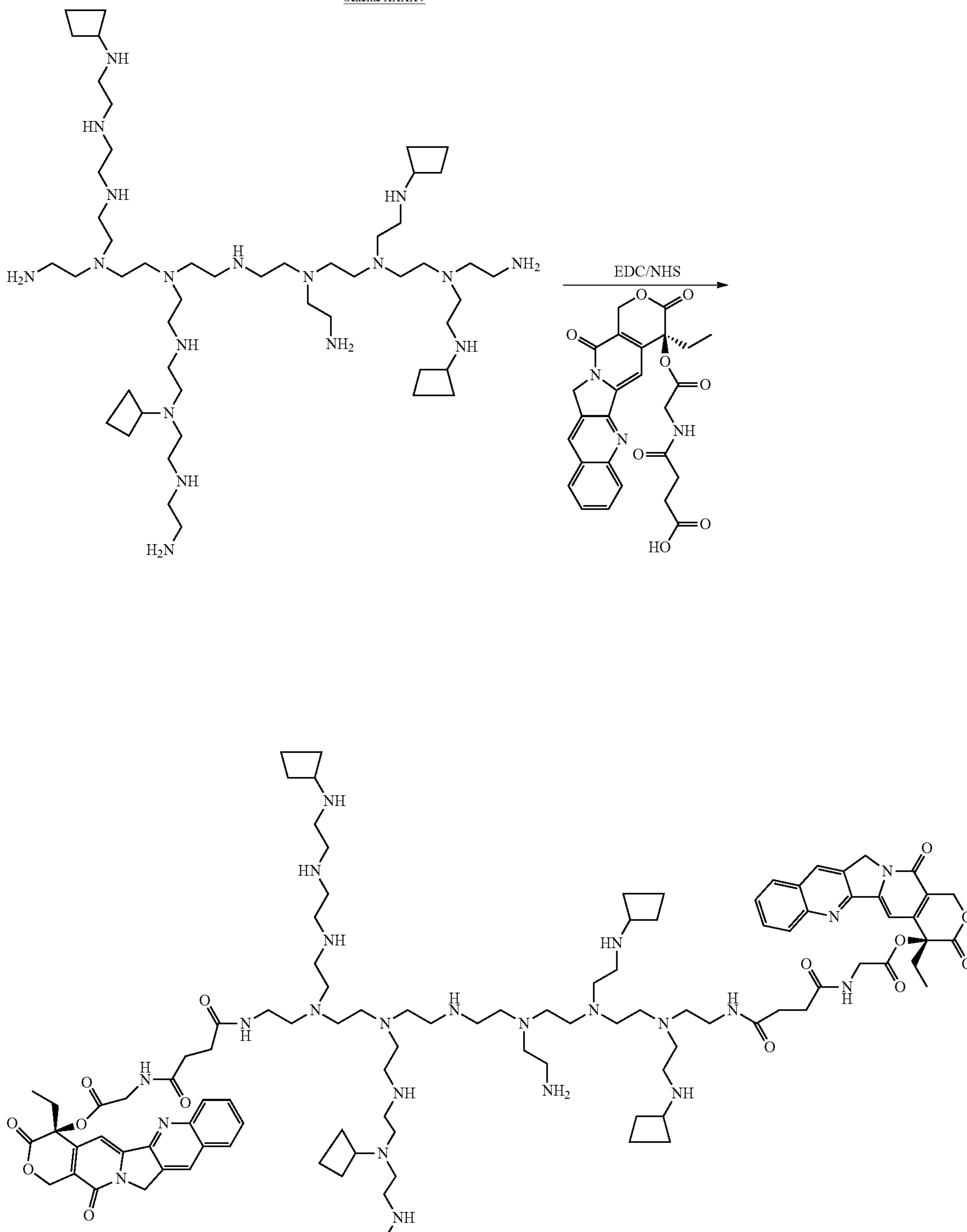
Scheme XXXXV
