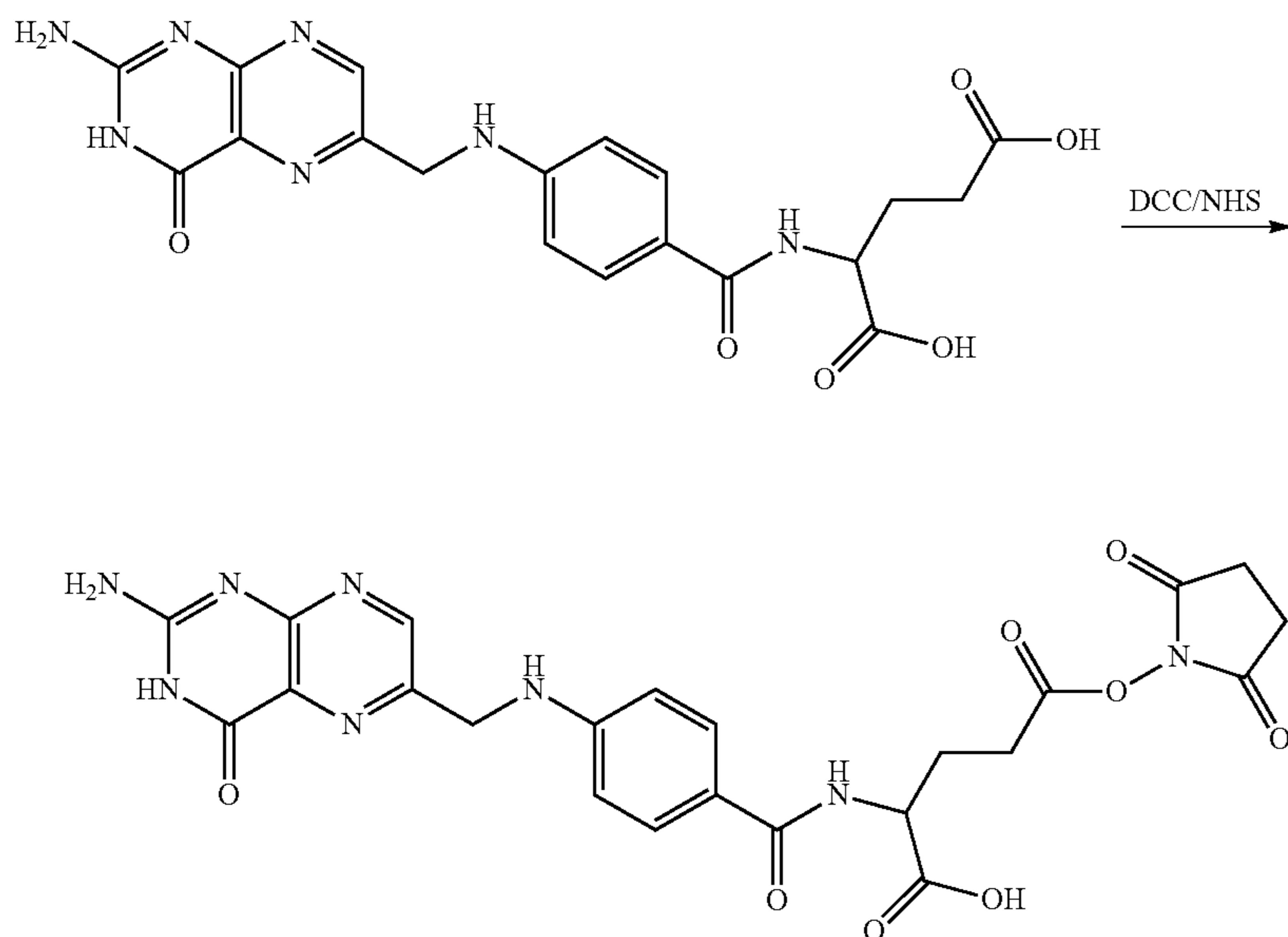
Scheme XXXXIX
