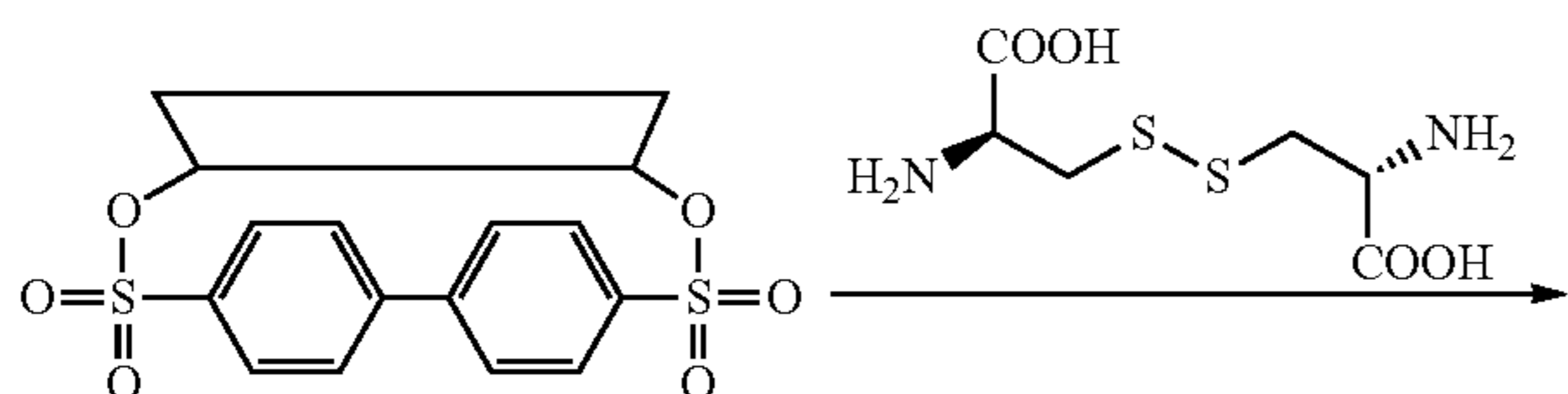
Scheme XXX
