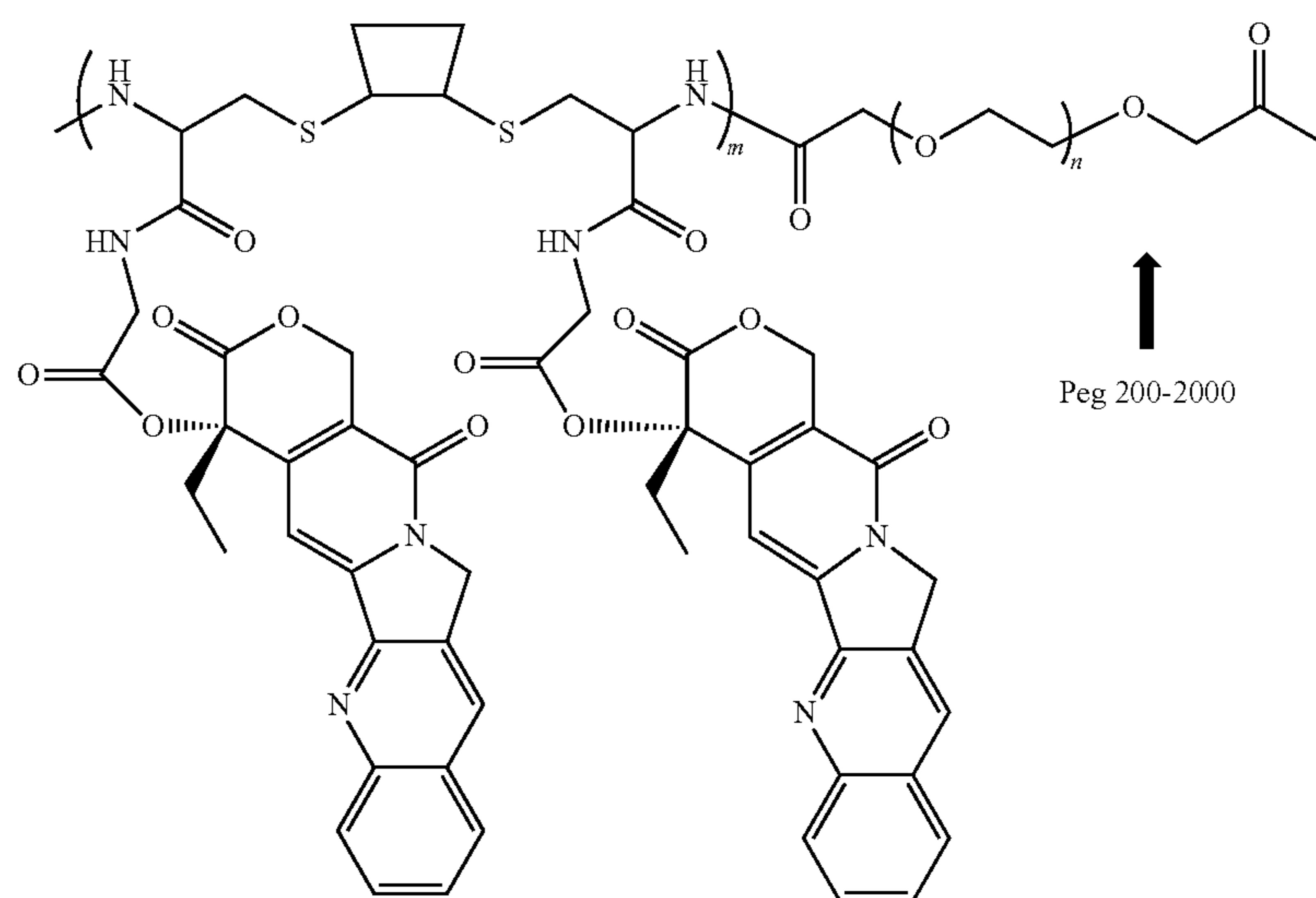
Scheme XXXXII
