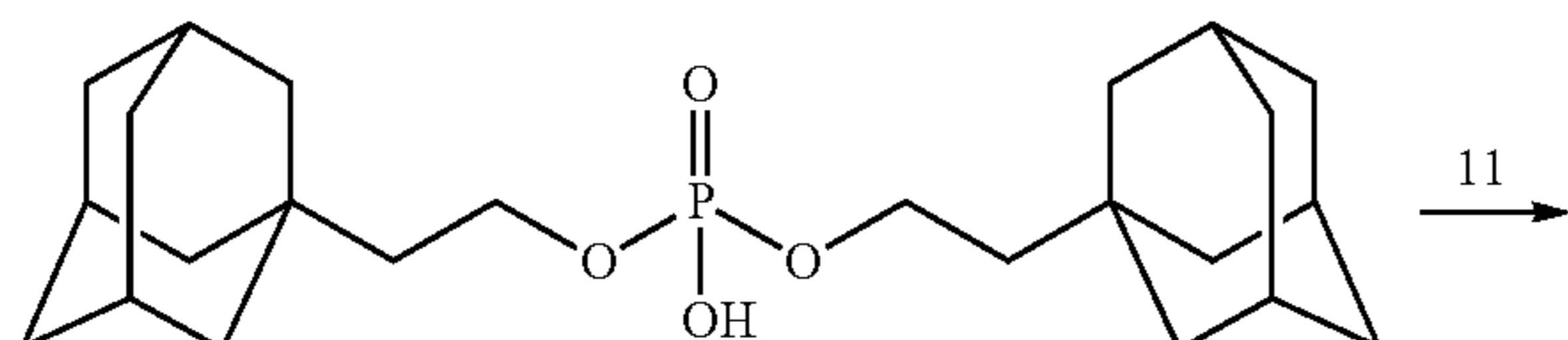
Scheme XXXXVIII
