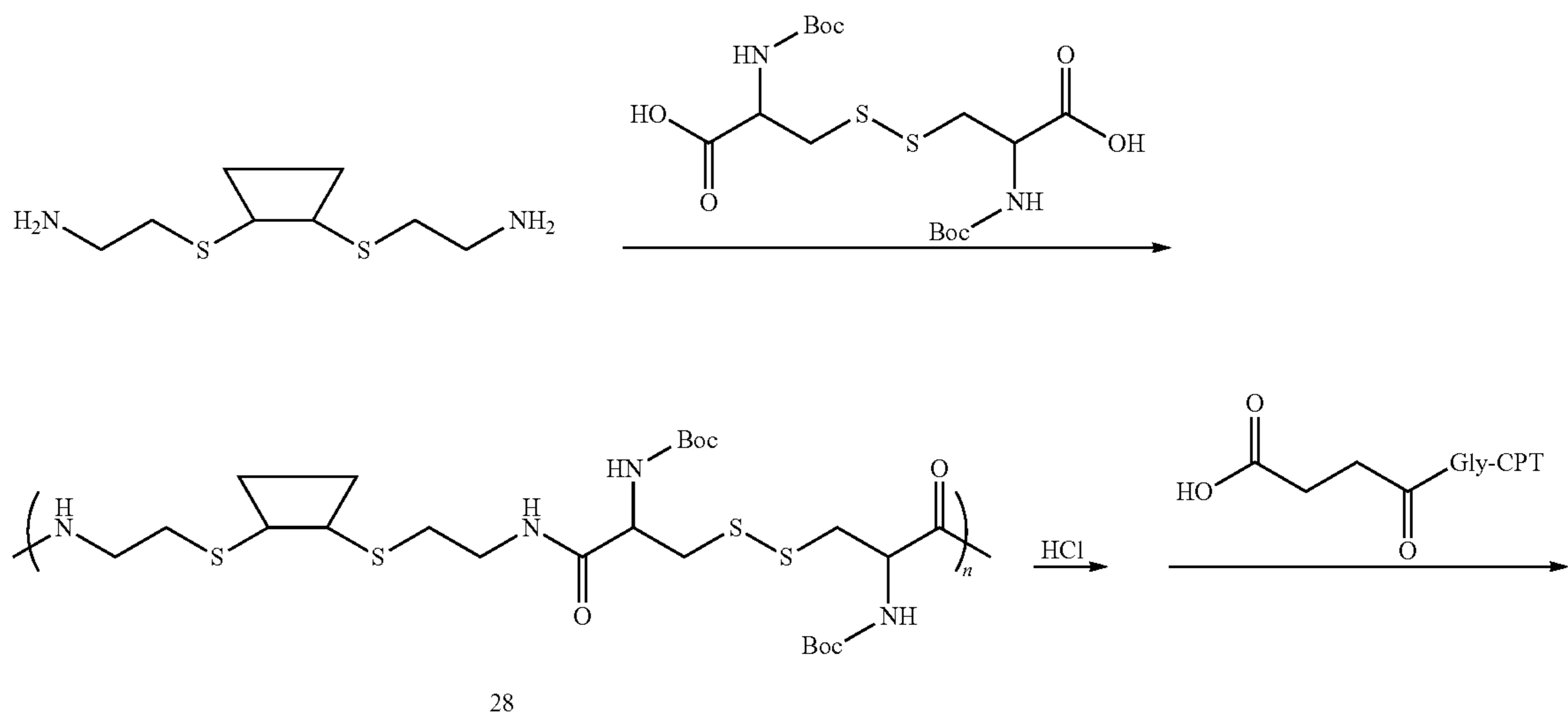
Scheme XXXIII
