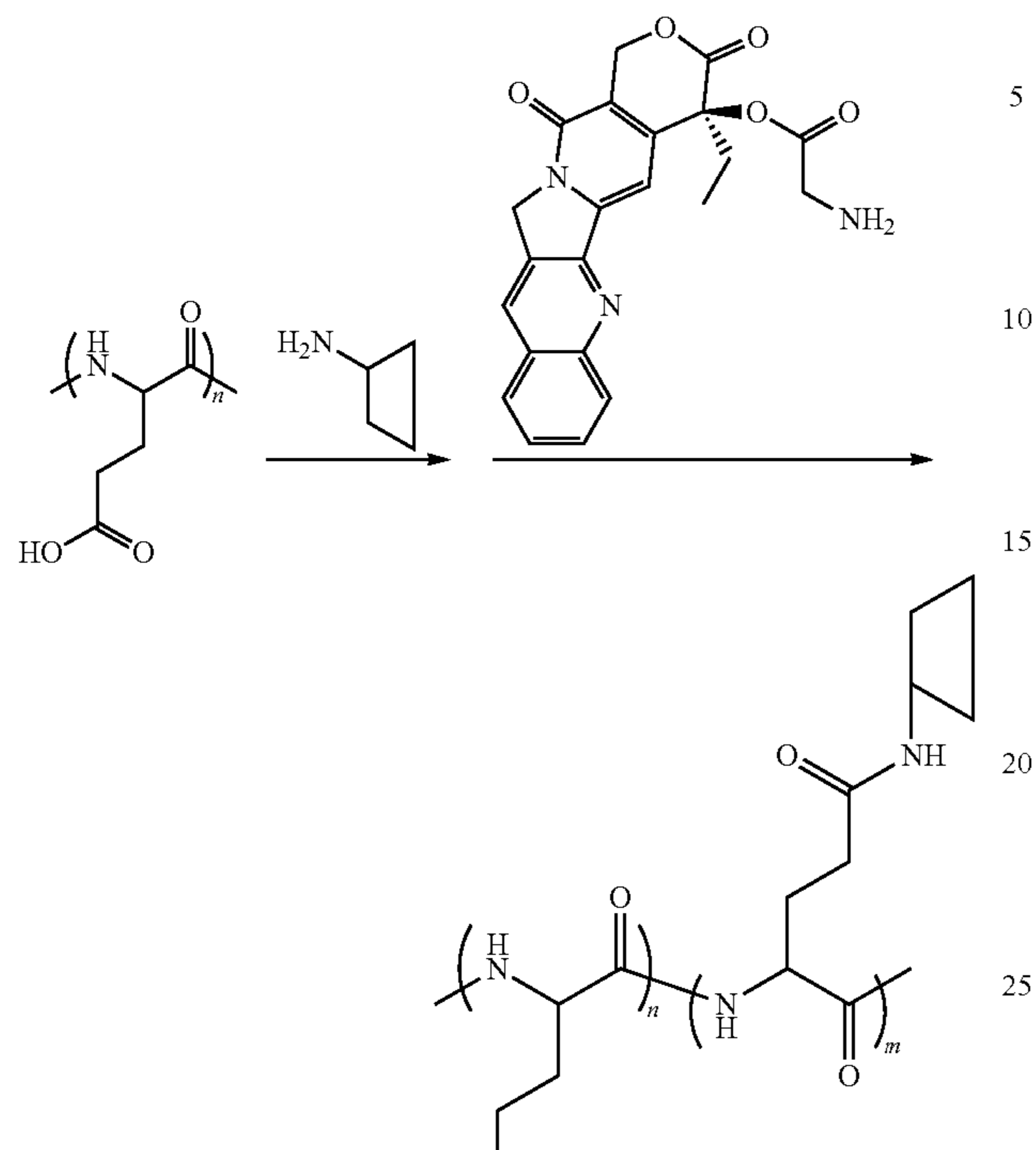
Scheme XII
