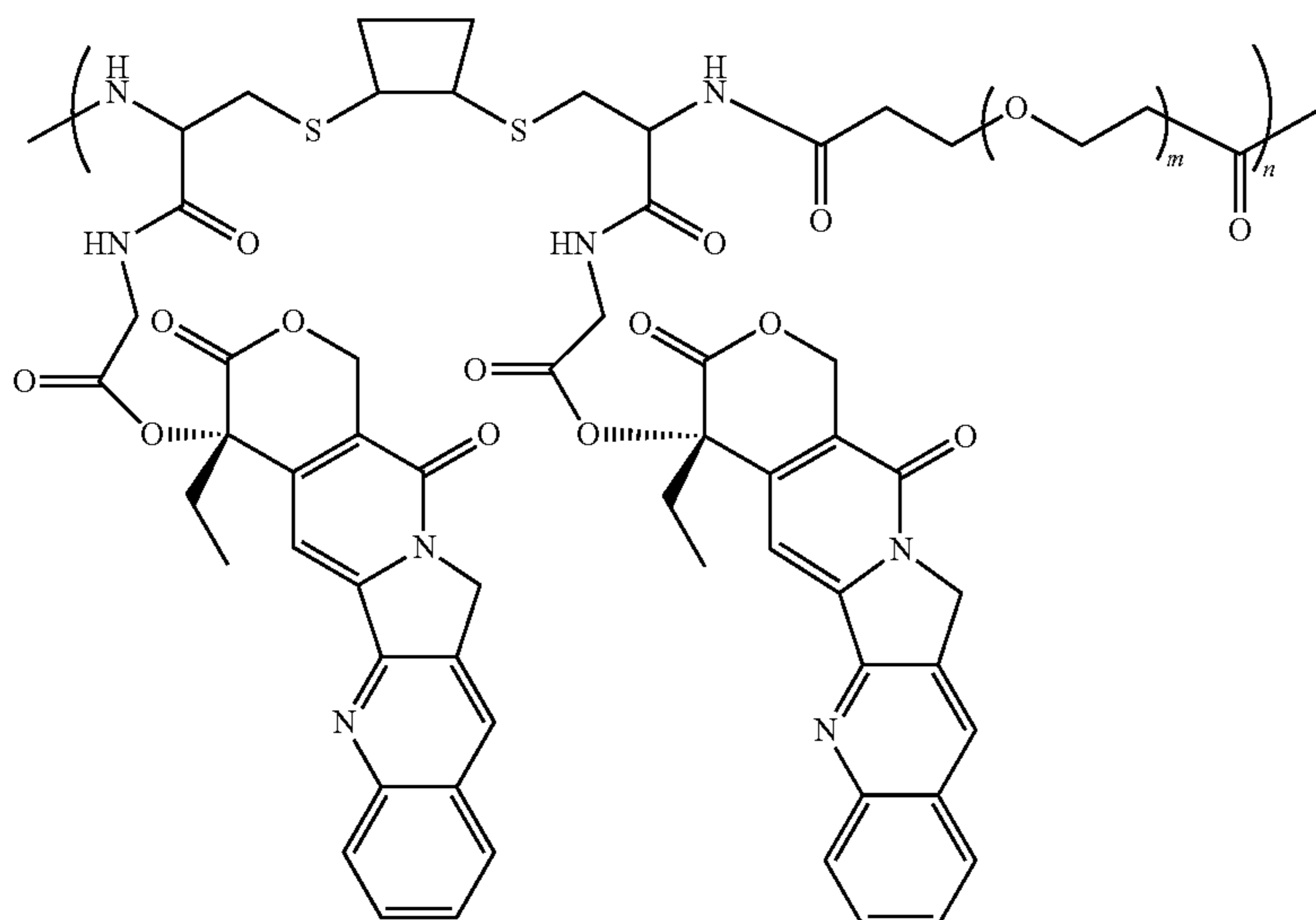
Scheme XXXXIII
