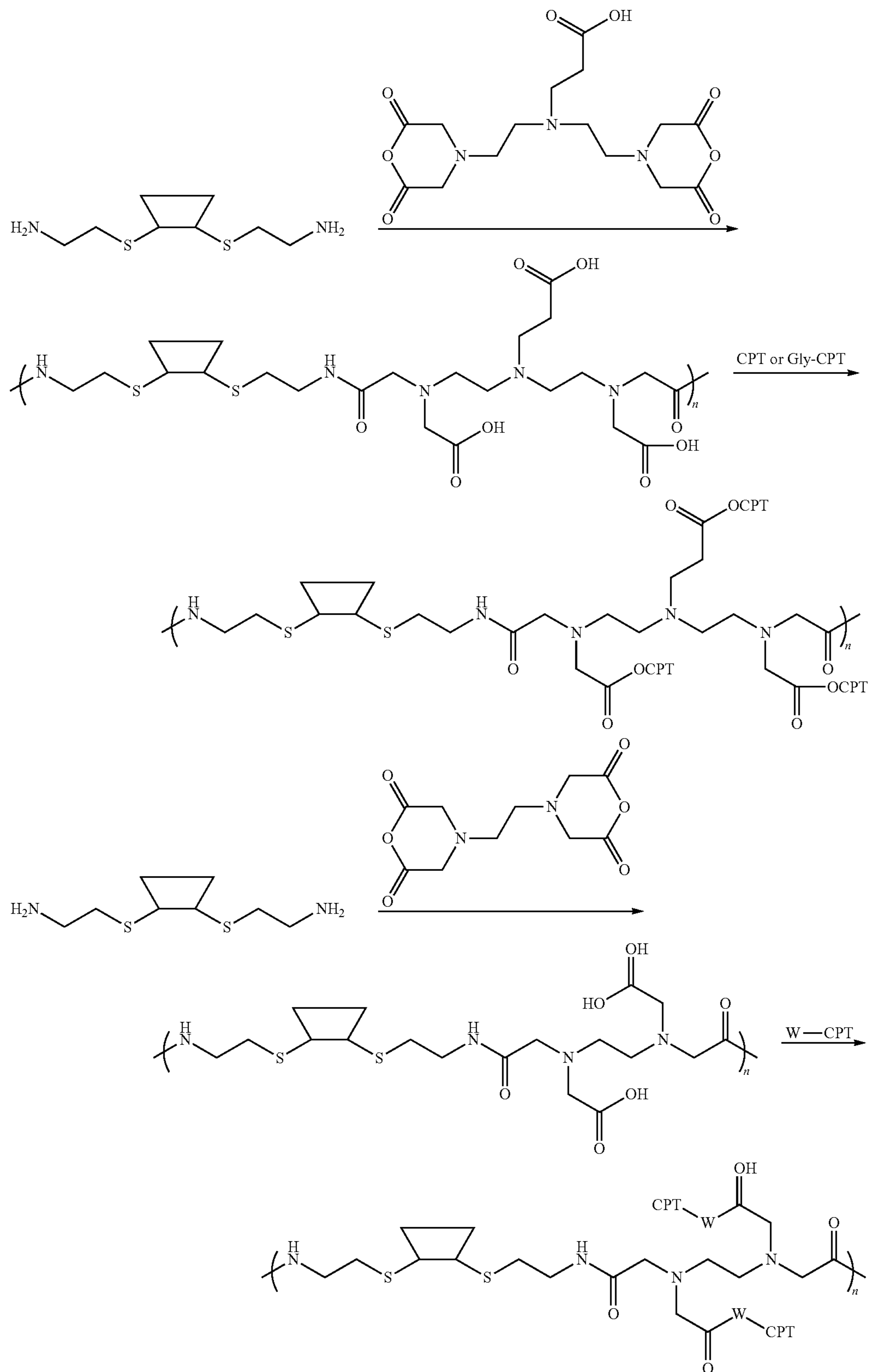
Scheme V
