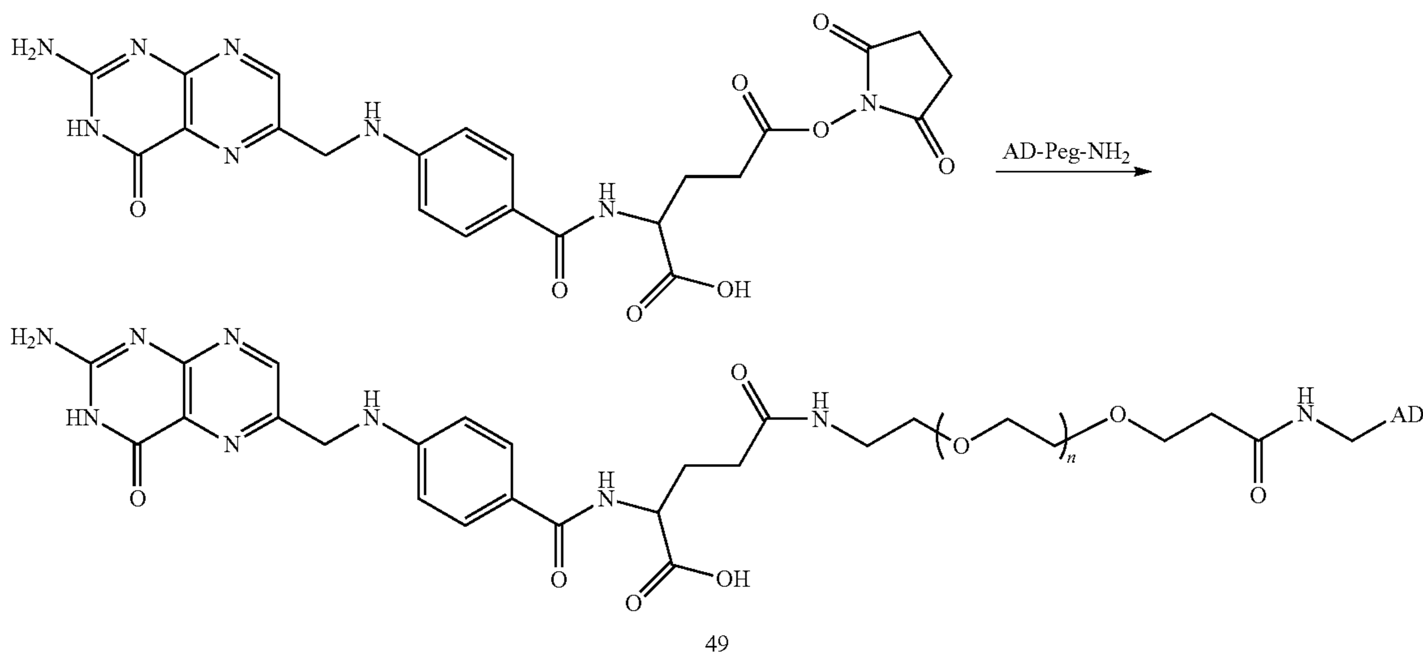
Scheme L
