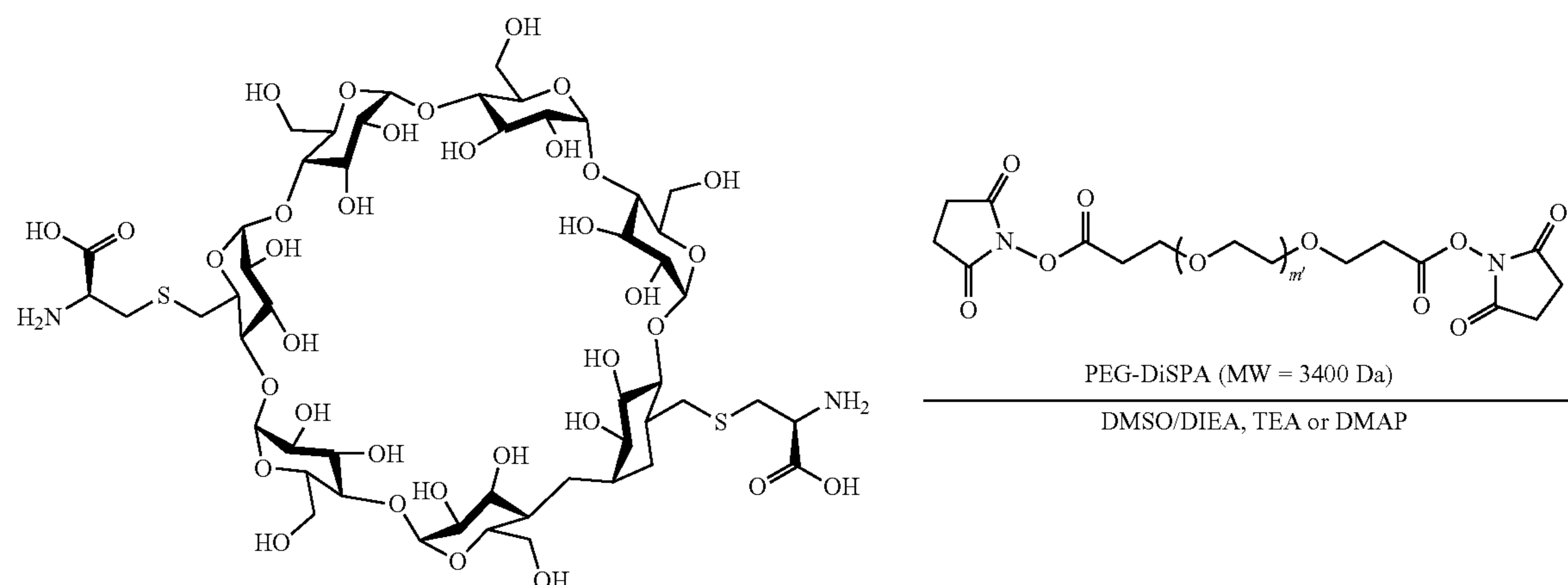
Scheme XXXVIIIa
