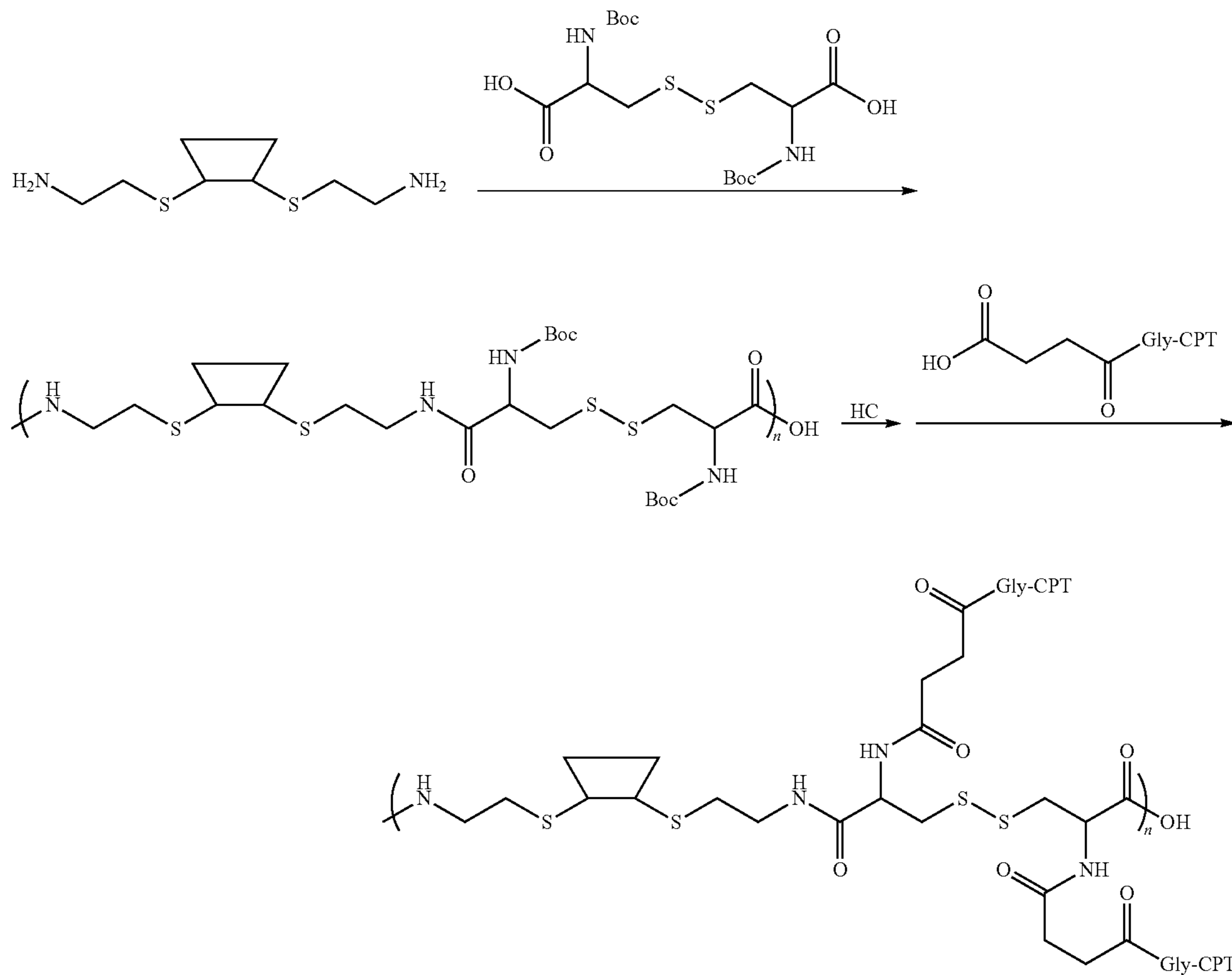
Scheme VII
