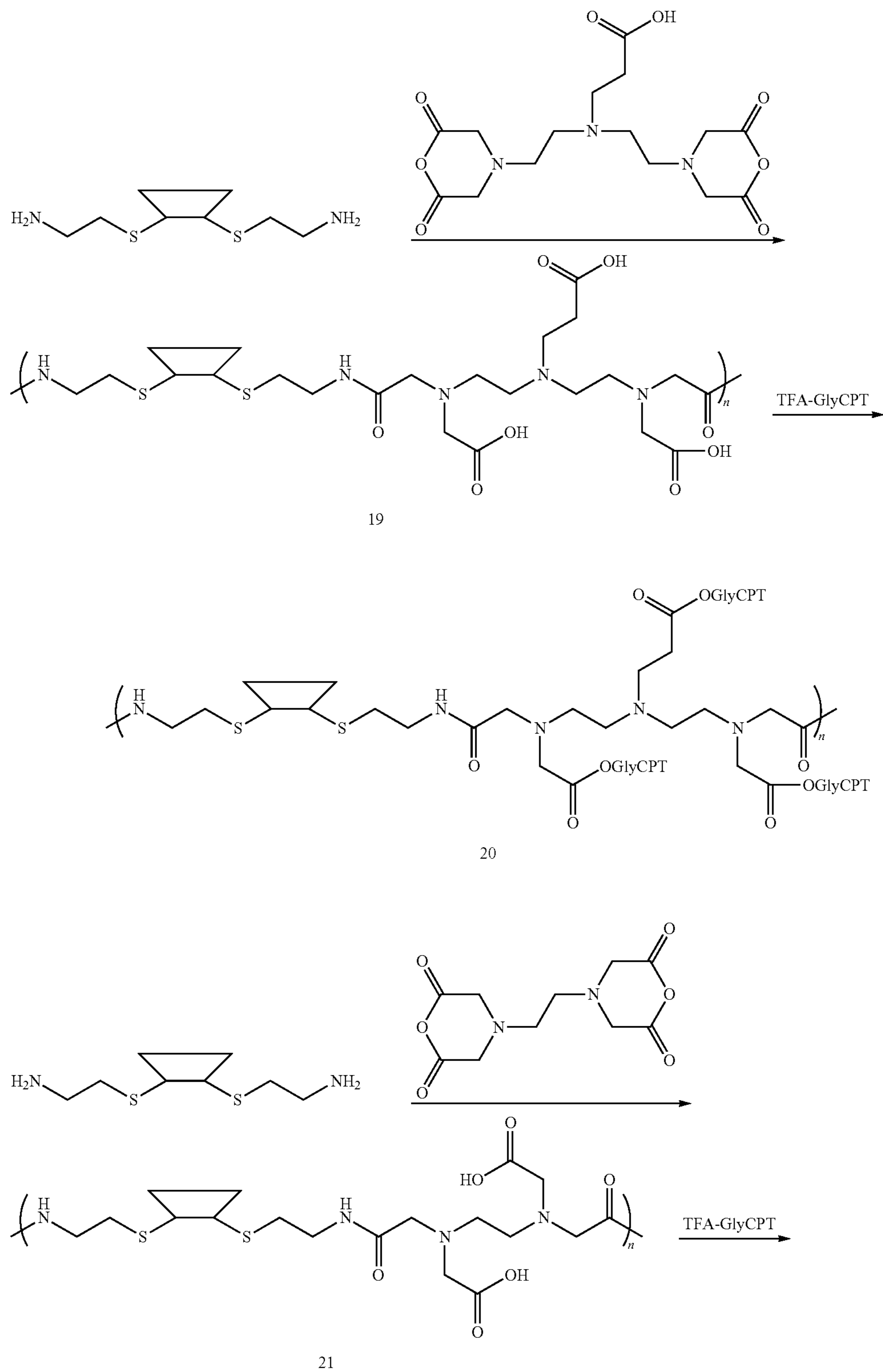
Scheme XXIX
