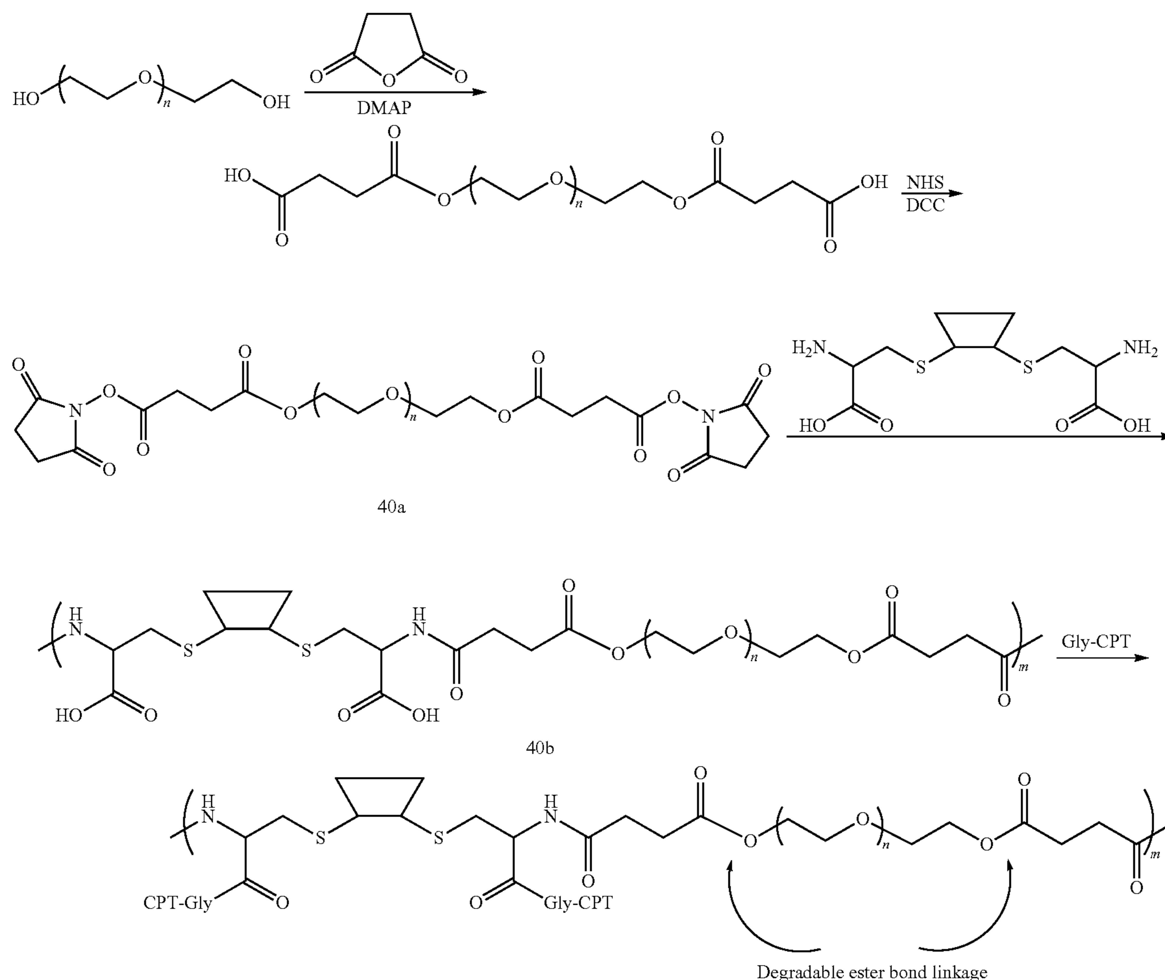
Scheme XXXXI
