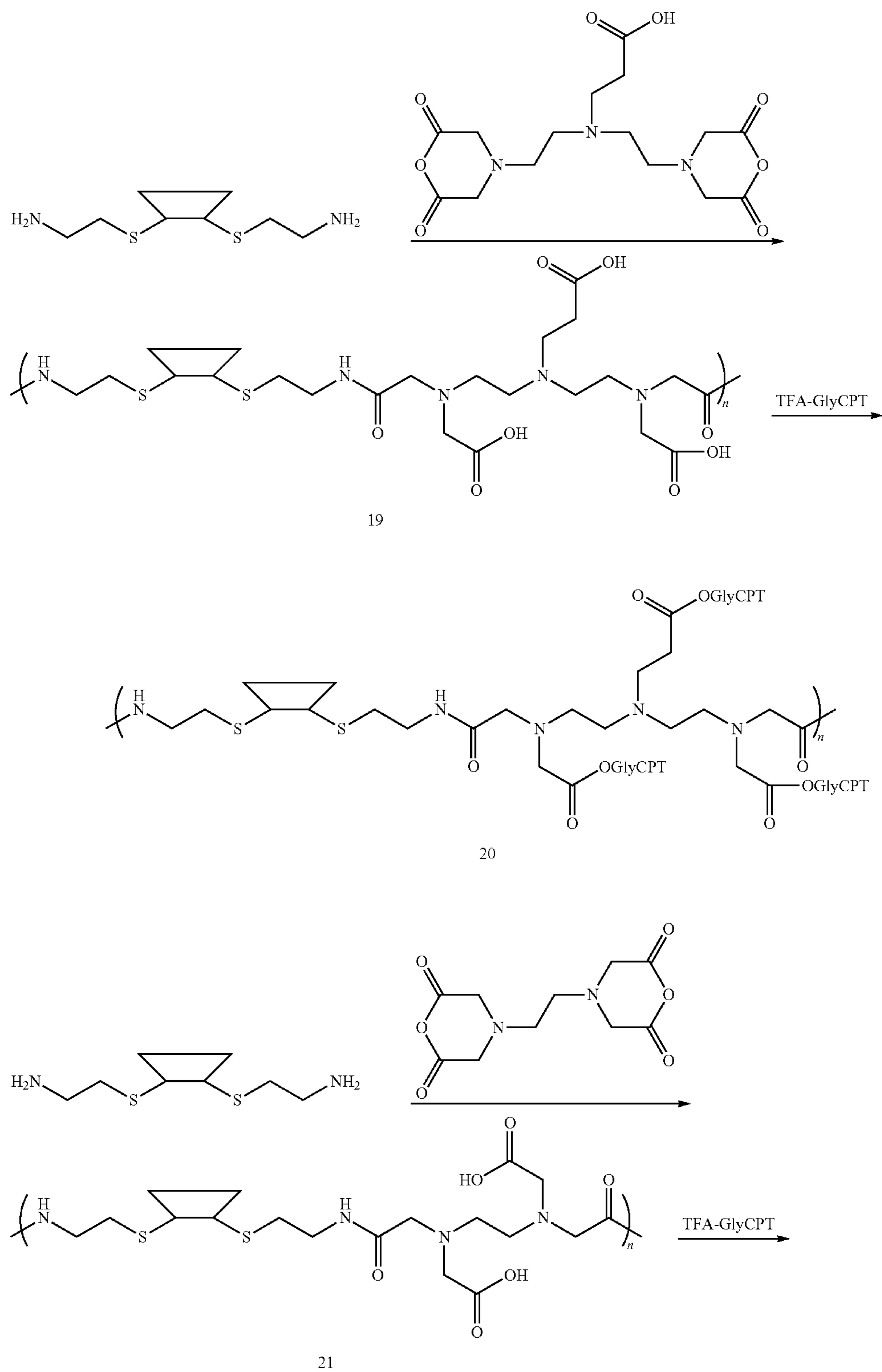
Scheme XXIX
