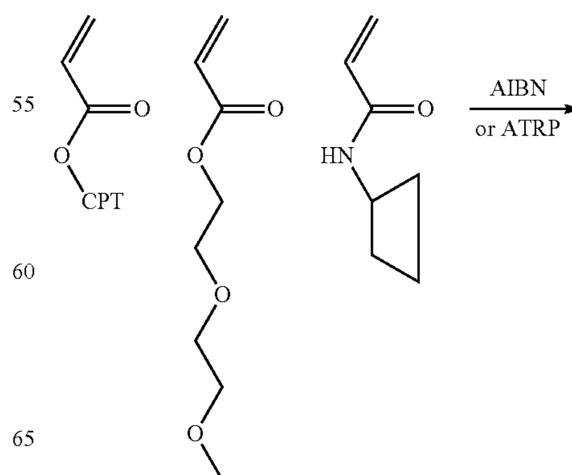
Scheme XXXV
