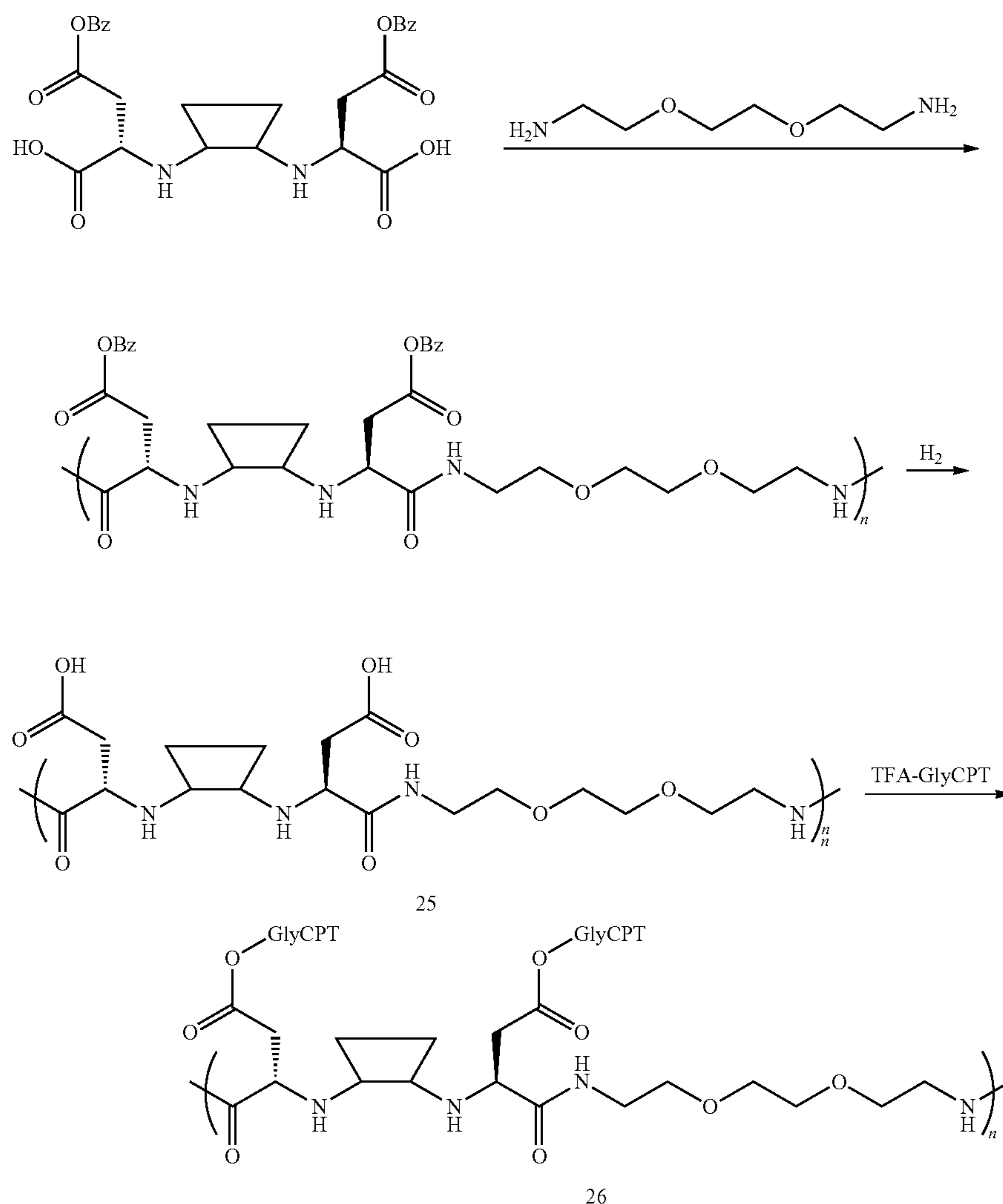
Scheme XXXI
