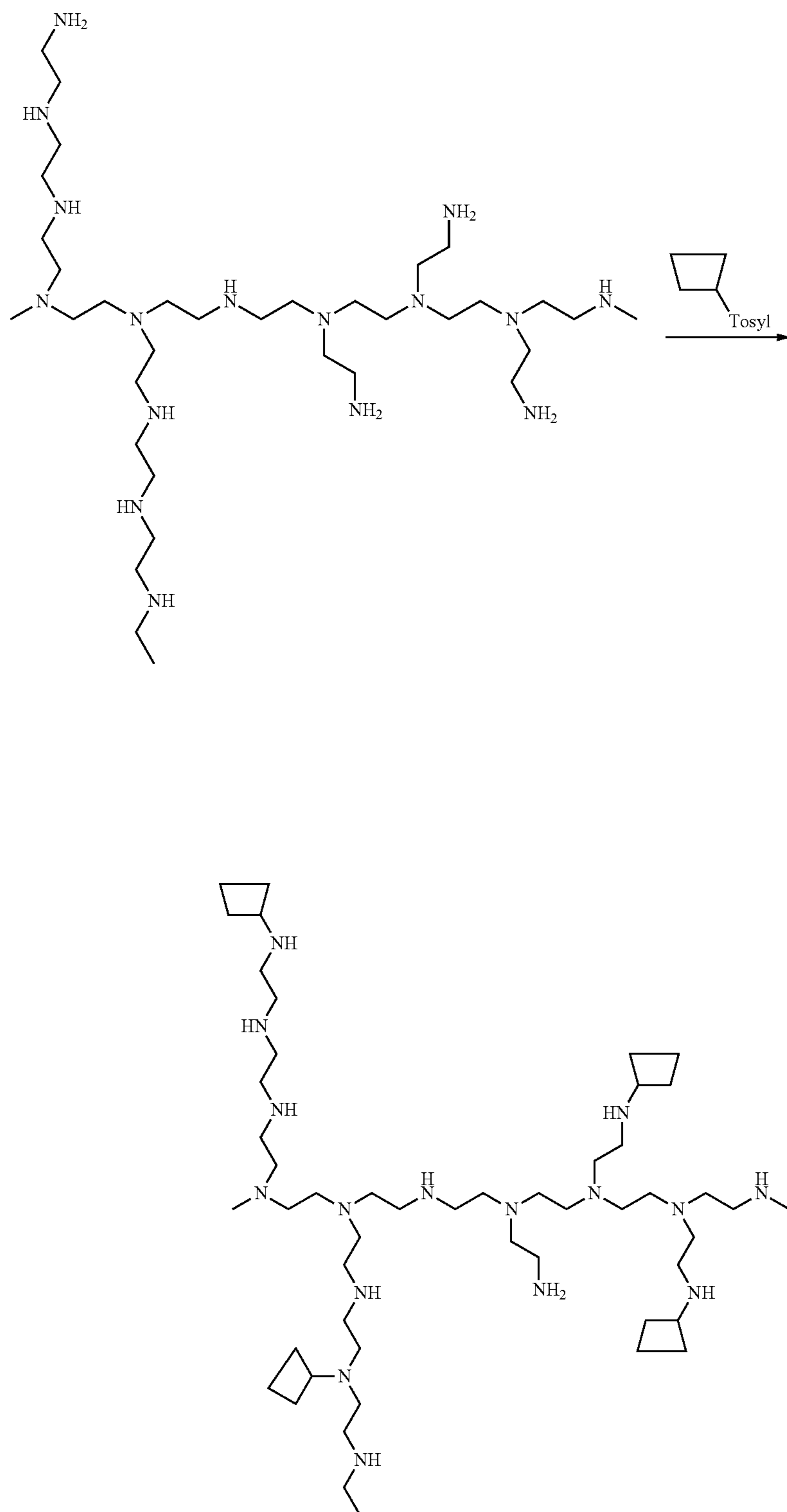
Scheme XXXXIV
