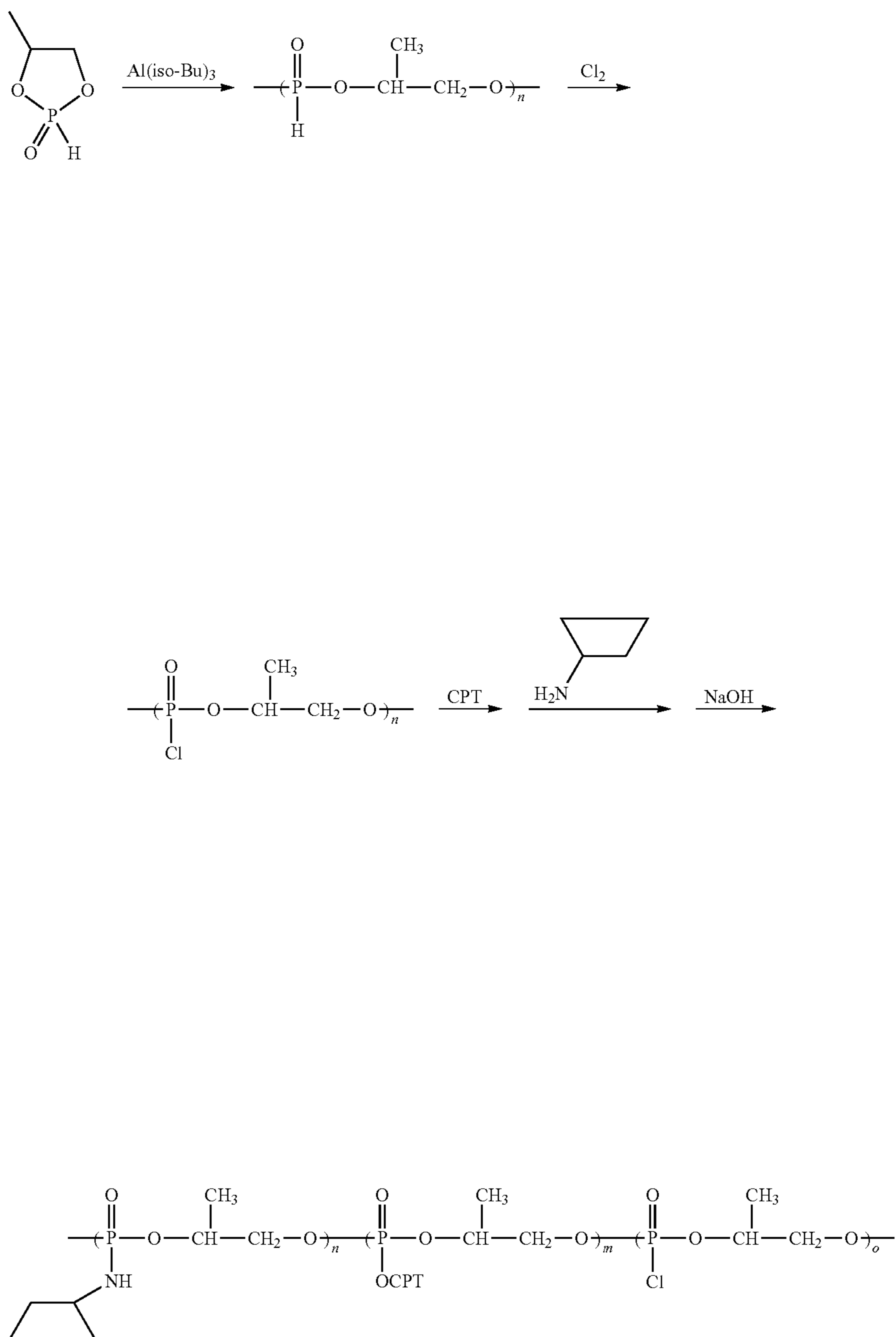
Scheme IX
