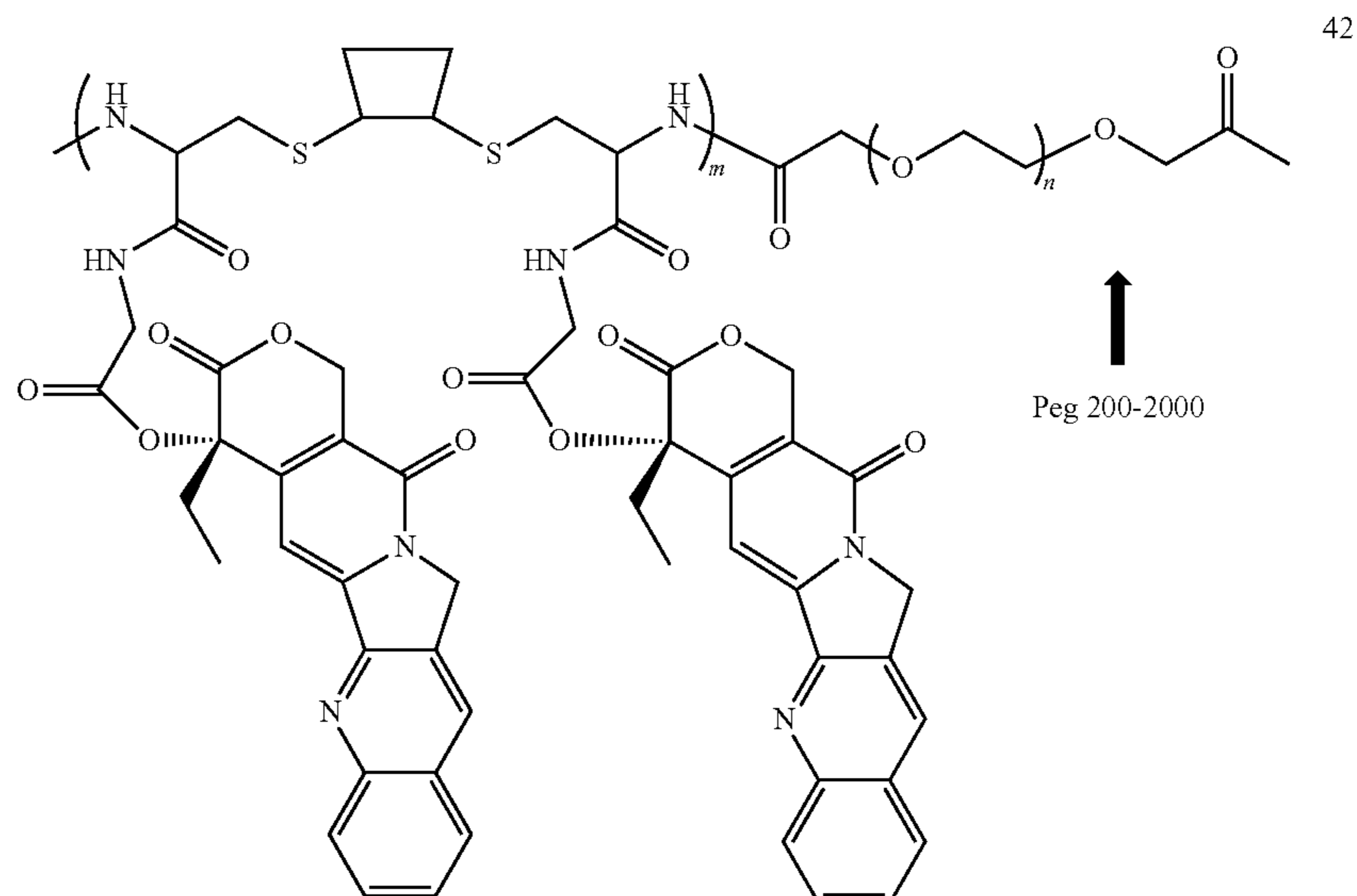
Scheme XXXXII
