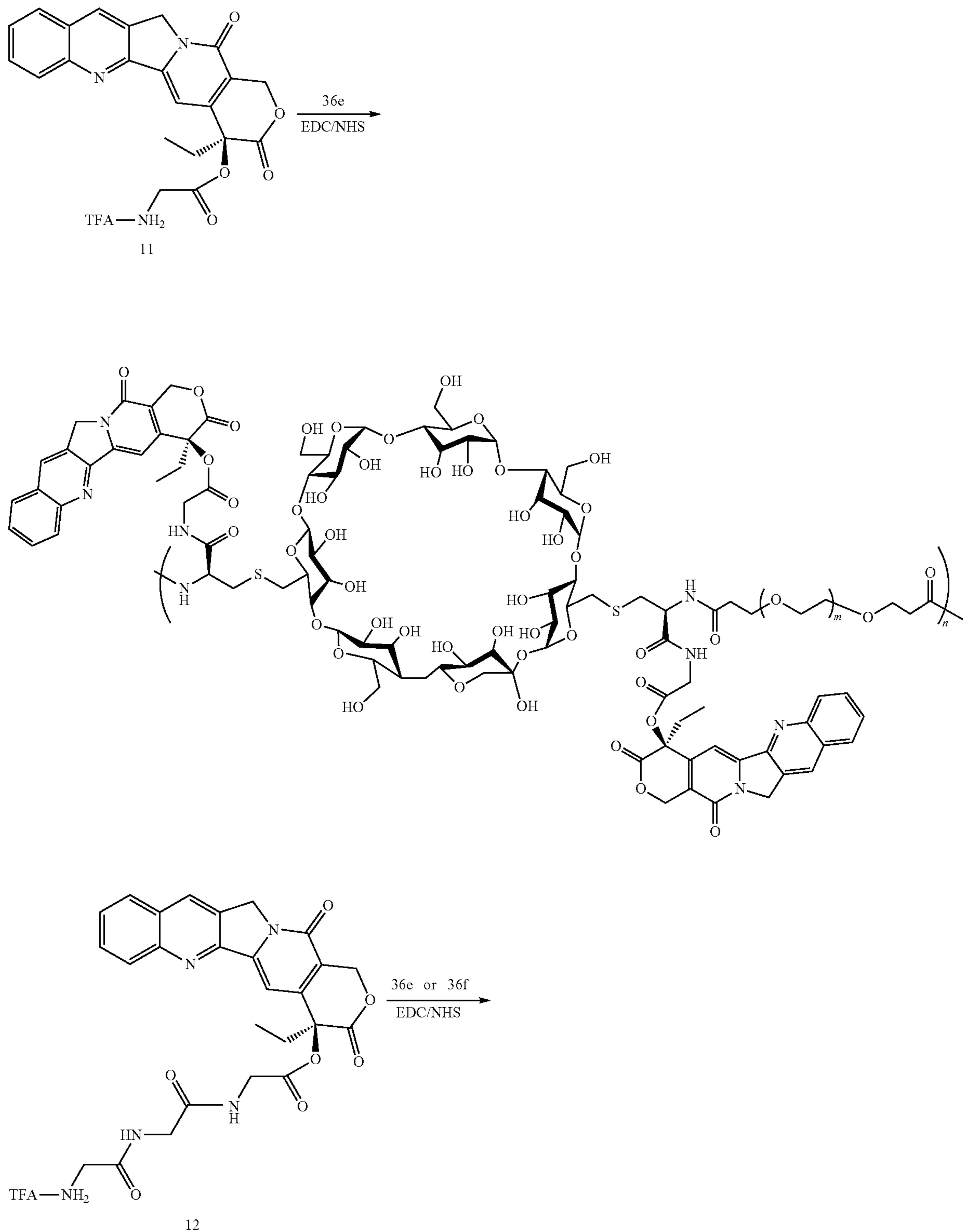
Scheme XXXIX
