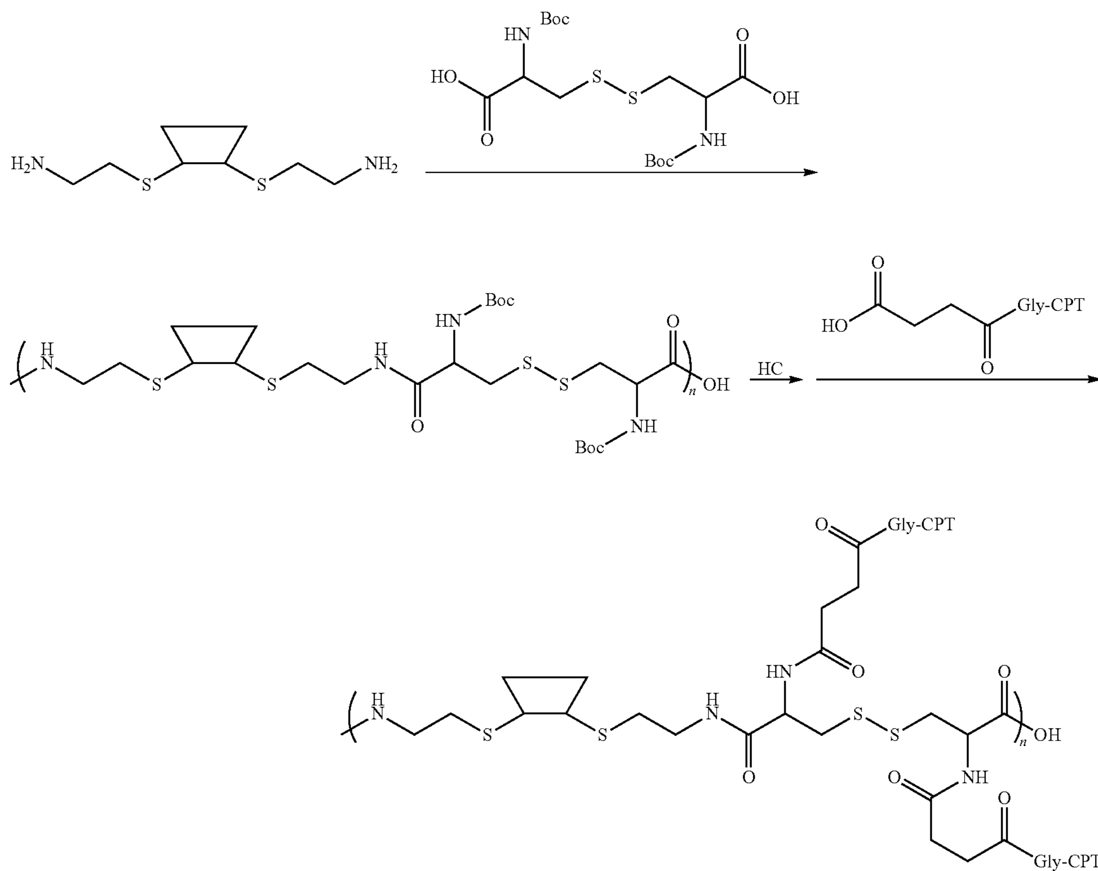
Scheme VII
