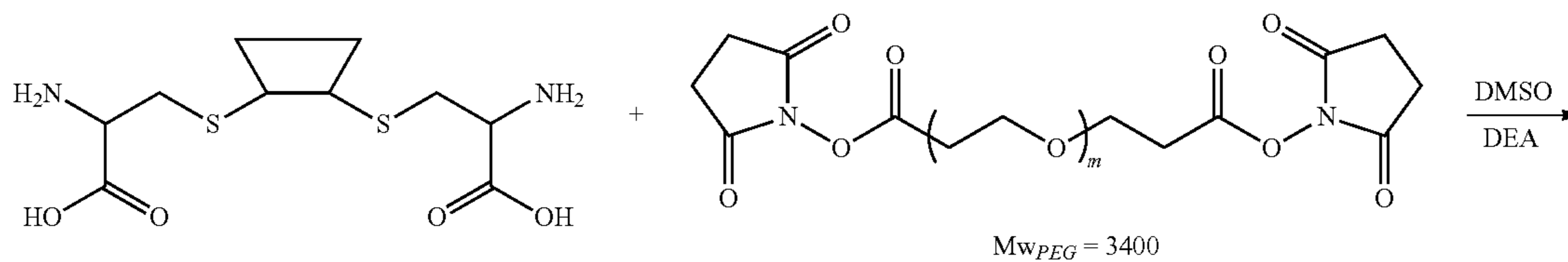
Scheme XIII
