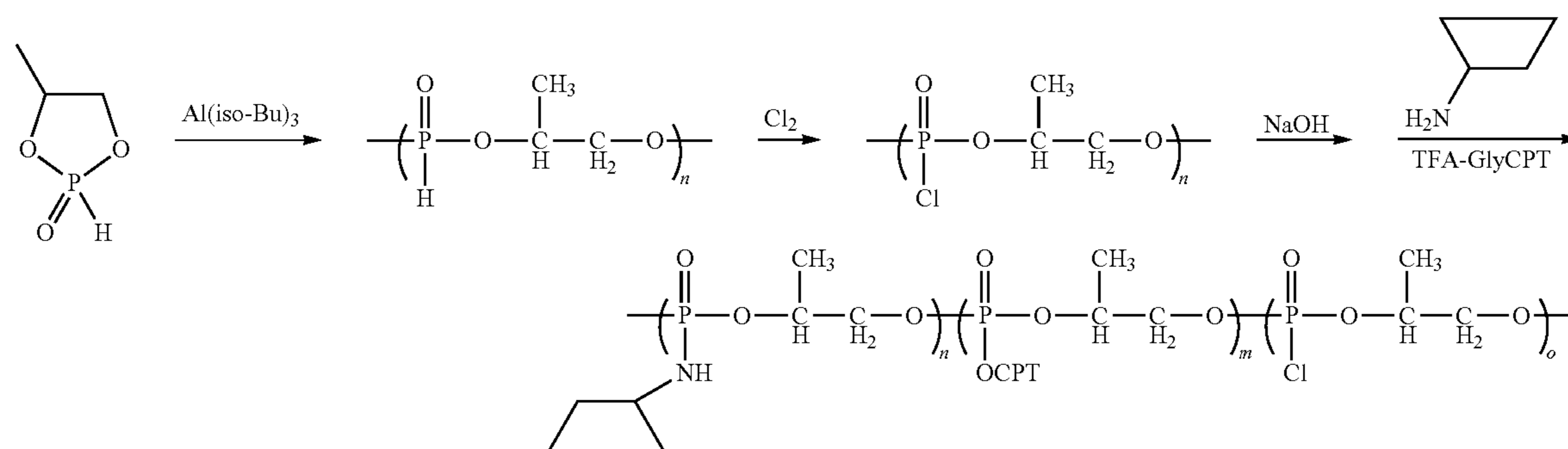
Scheme XXXIV
