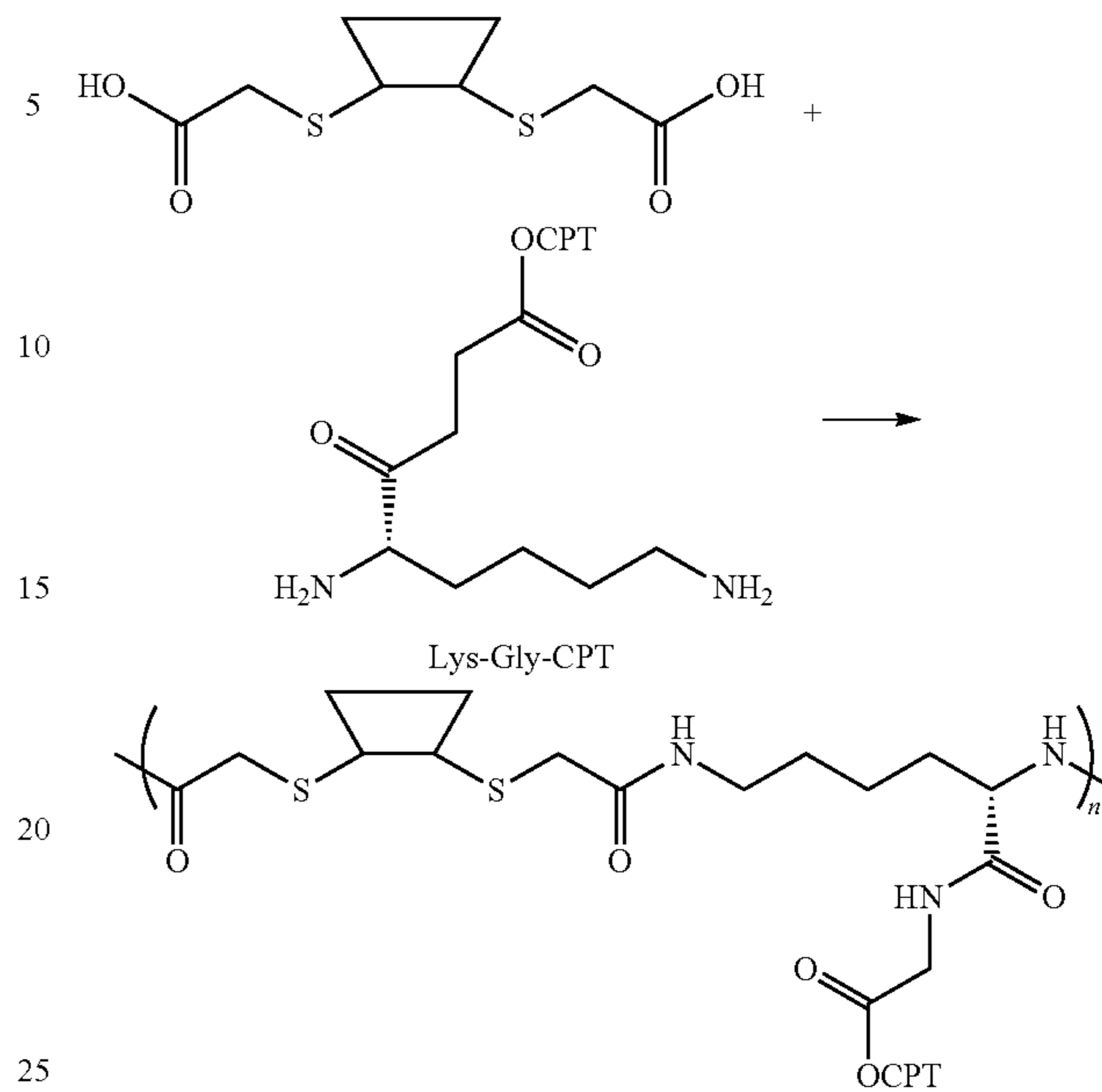
Scheme VIII
