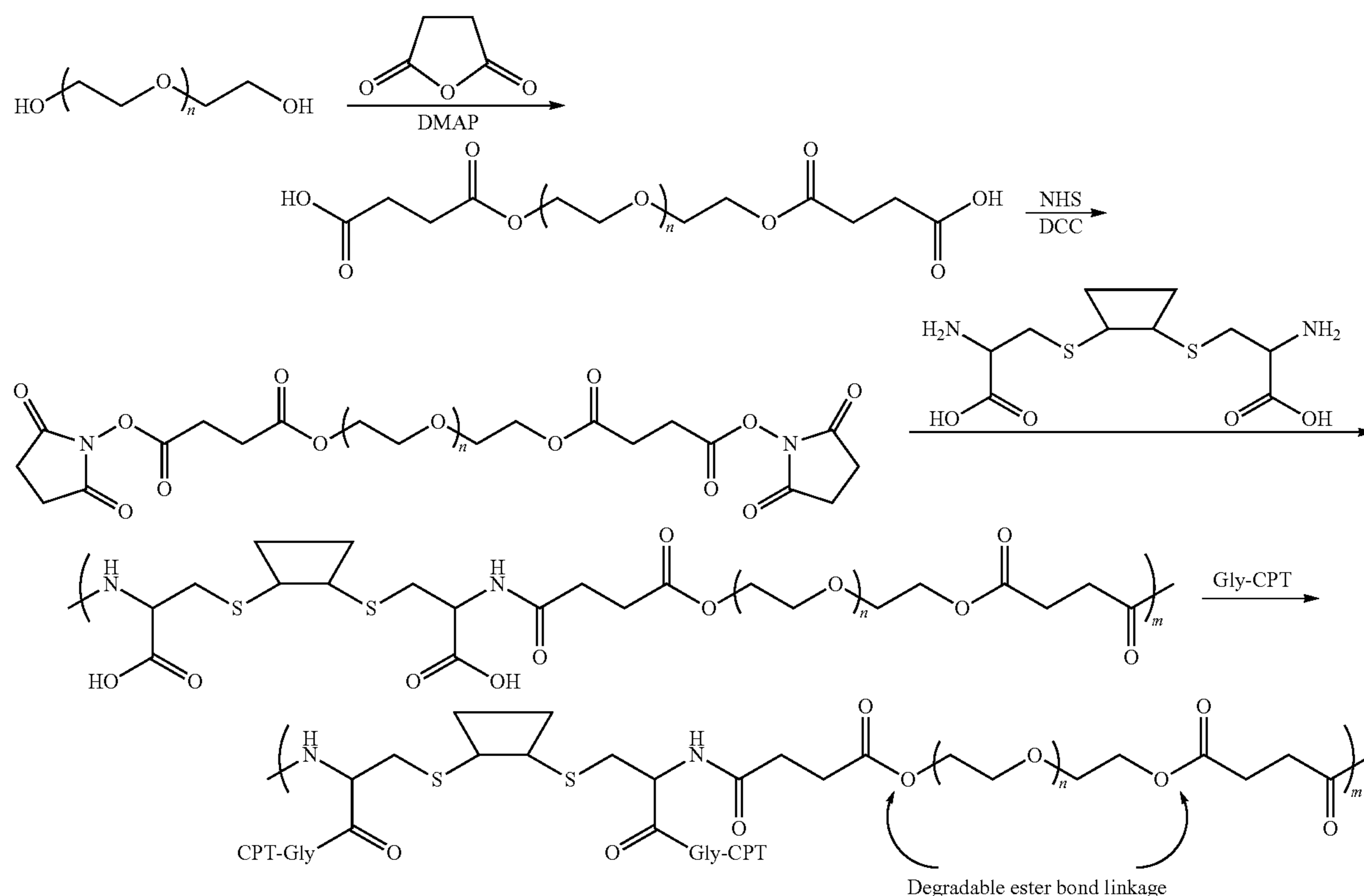
Scheme XIV
