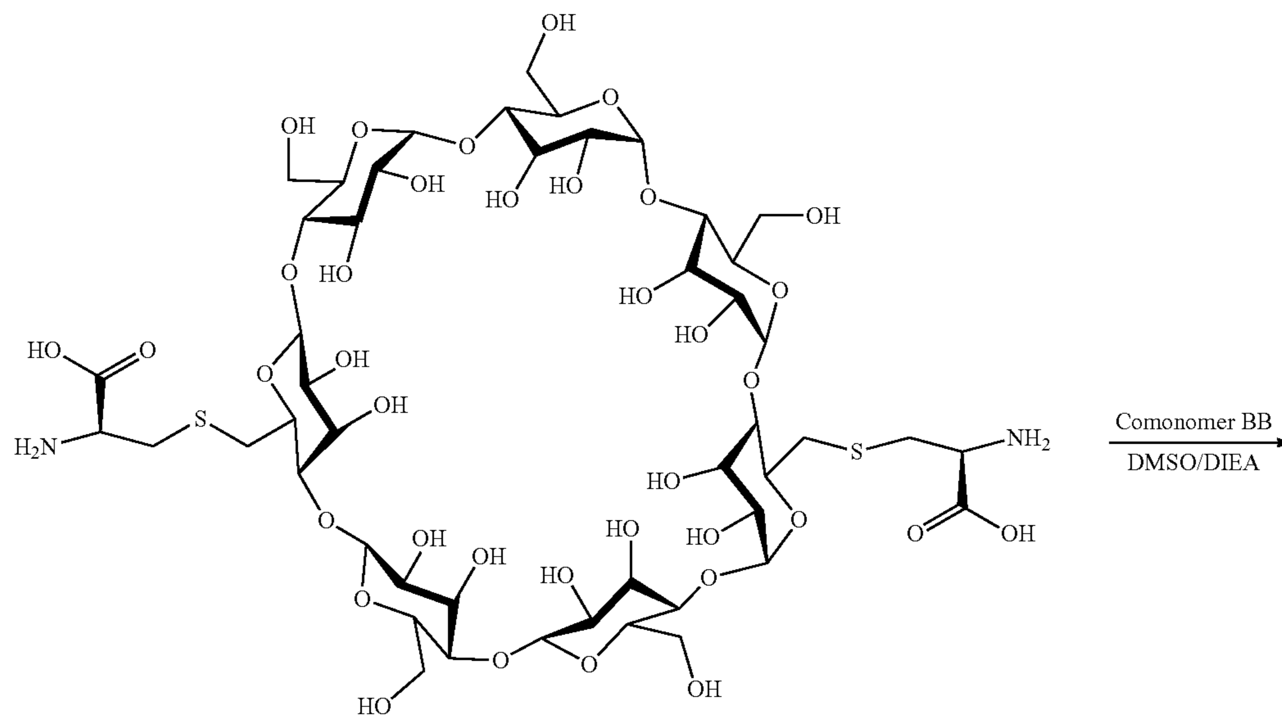
Scheme XXXVIIIb
