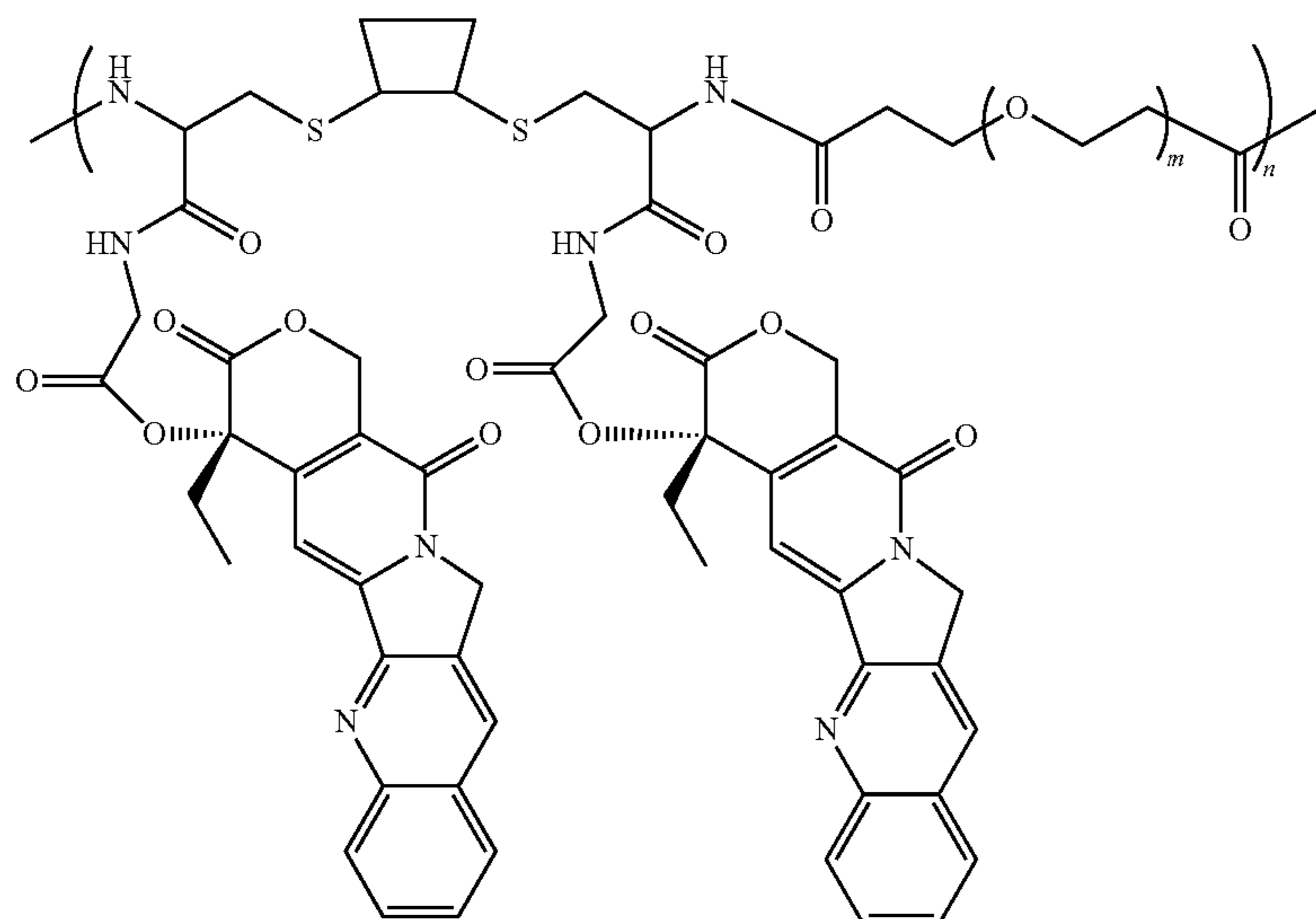
Scheme XXXXIII
