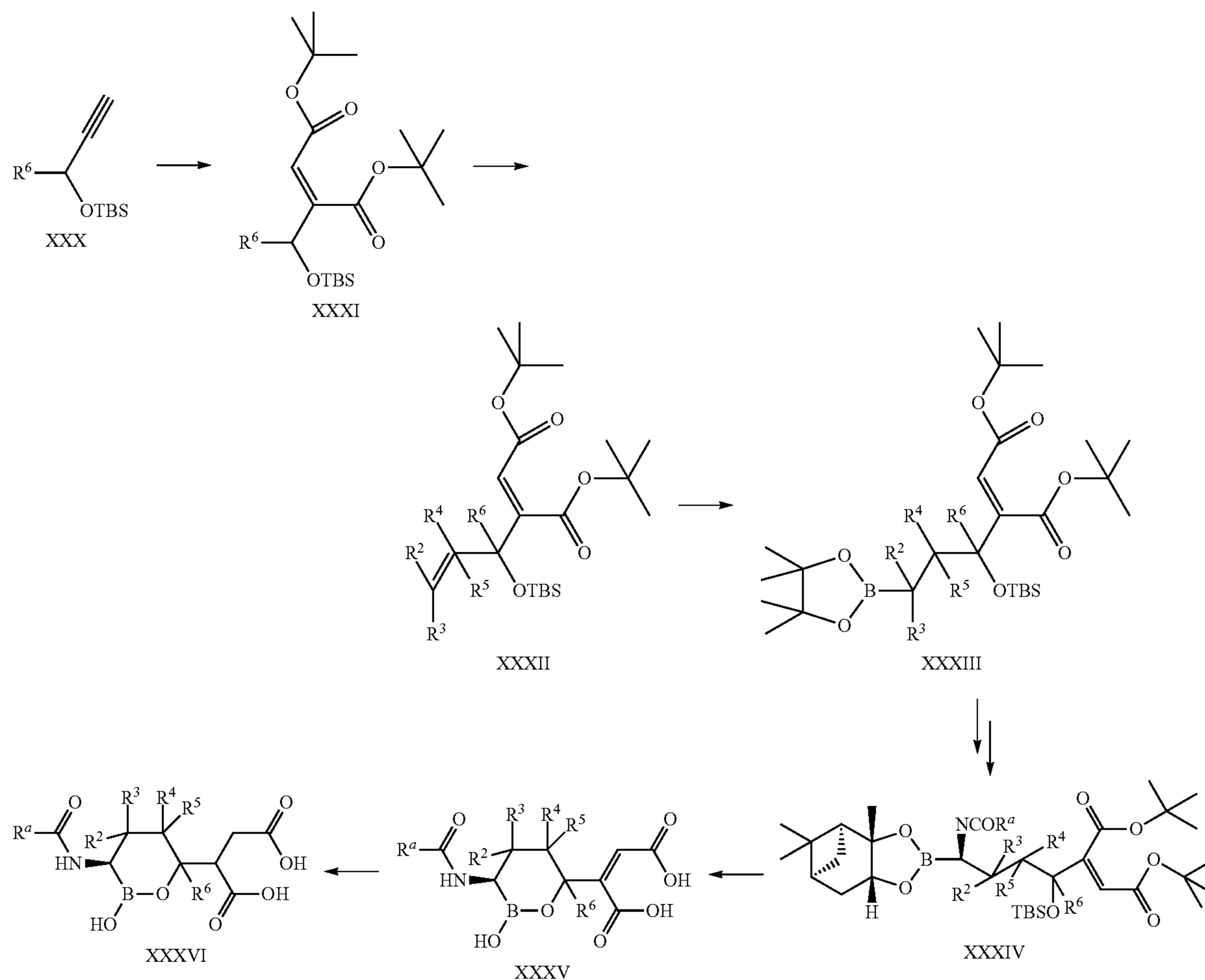
Scheme 7
