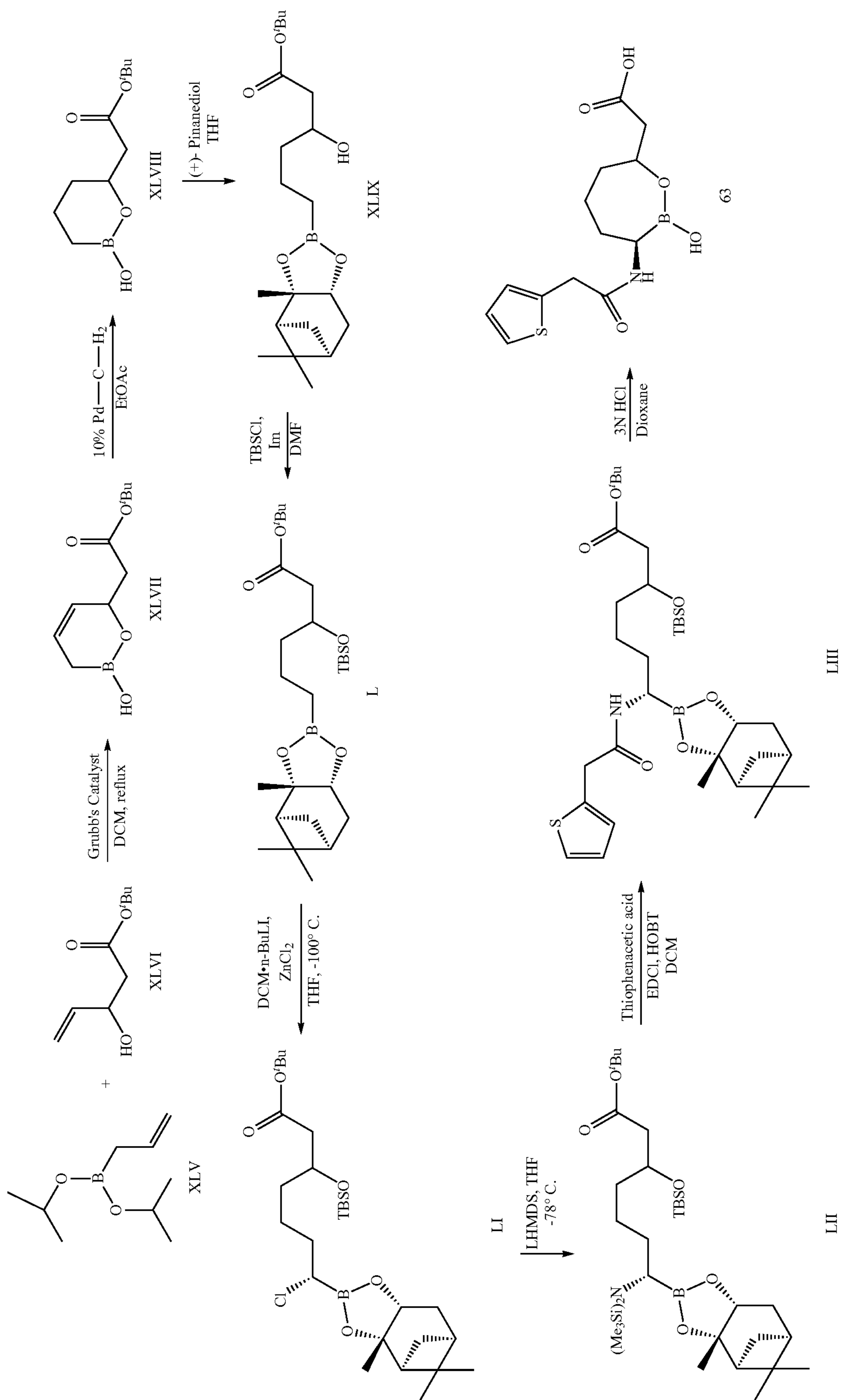
Scheme 11
