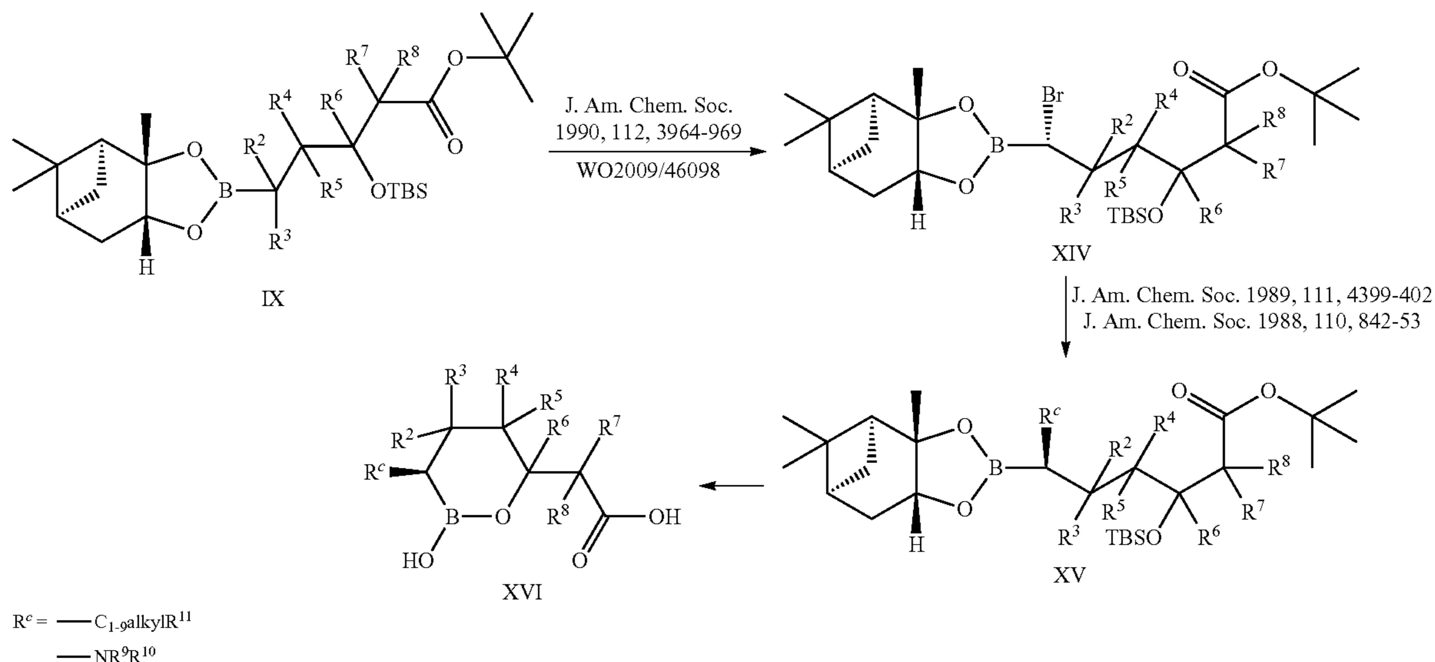
Scheme 2
