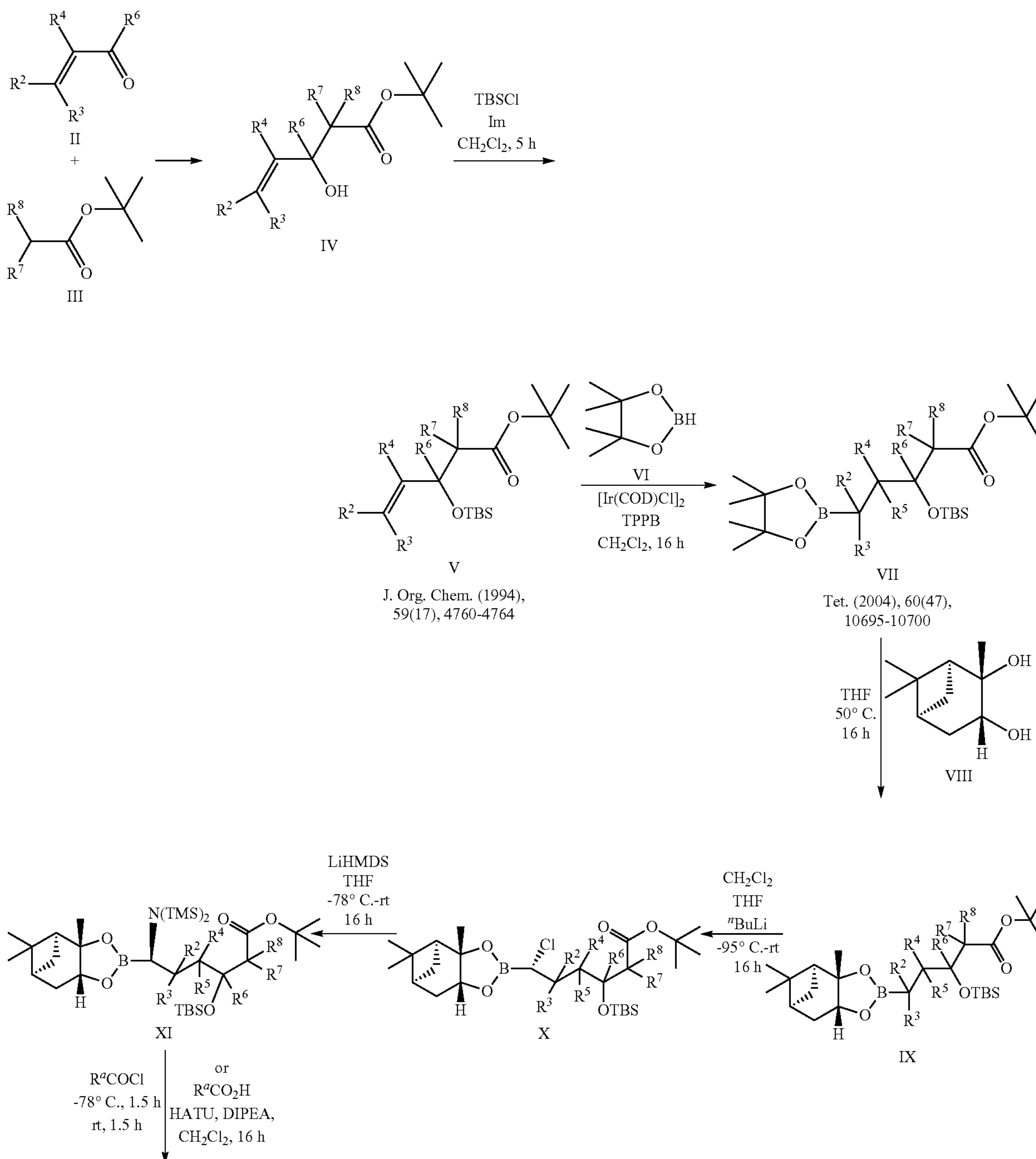
Scheme 1
