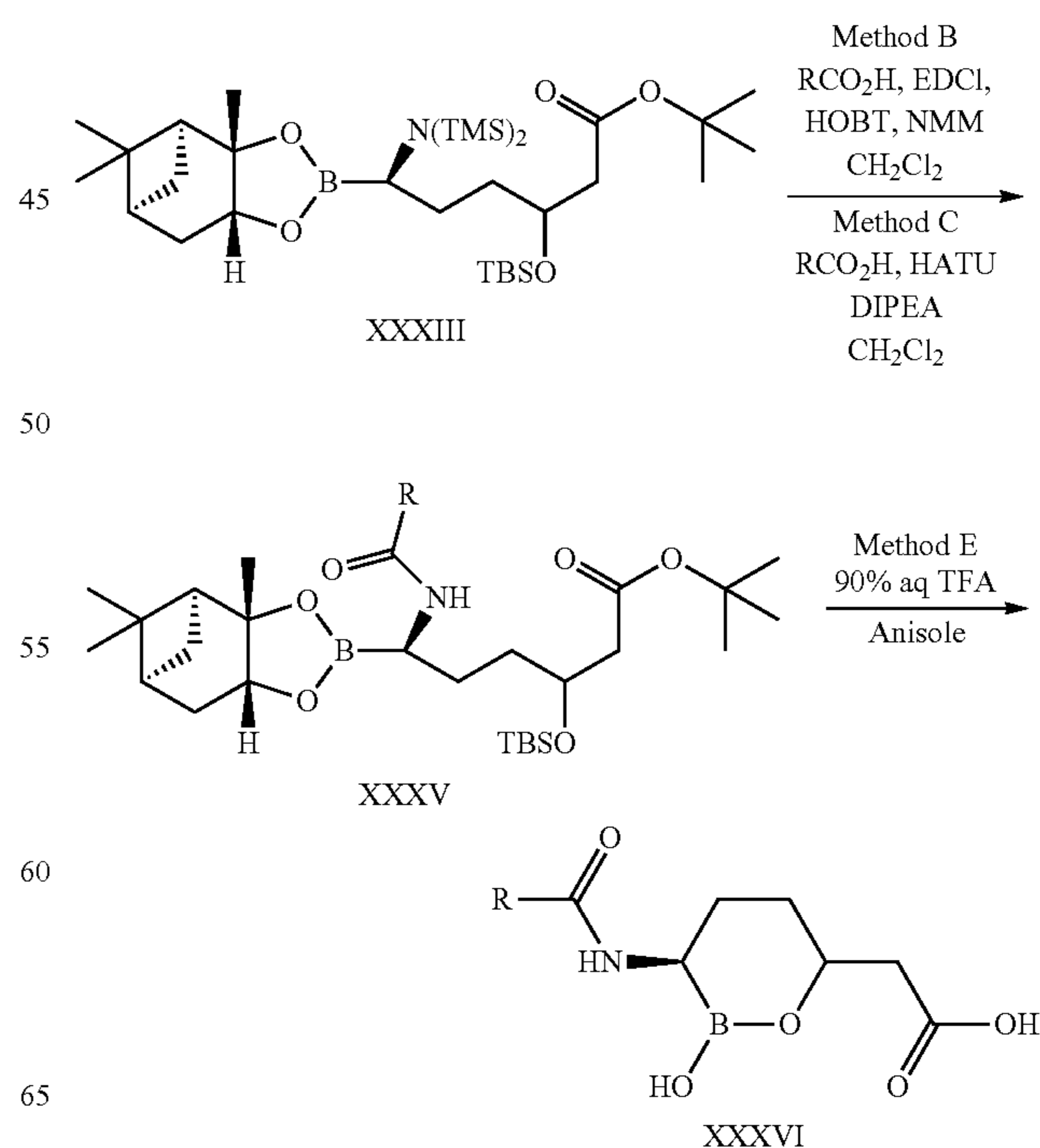
Scheme 9
