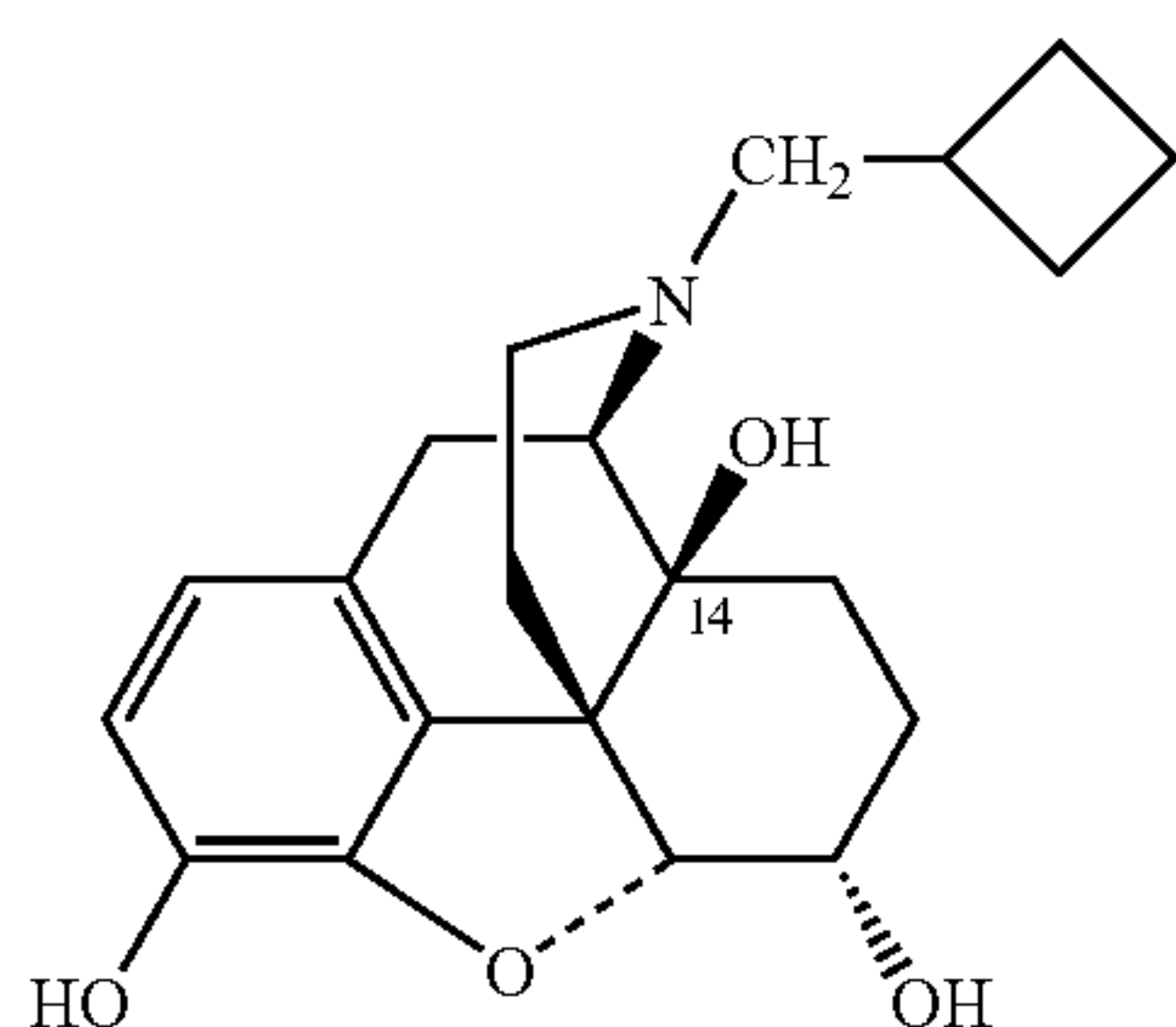
Nalbuphine
