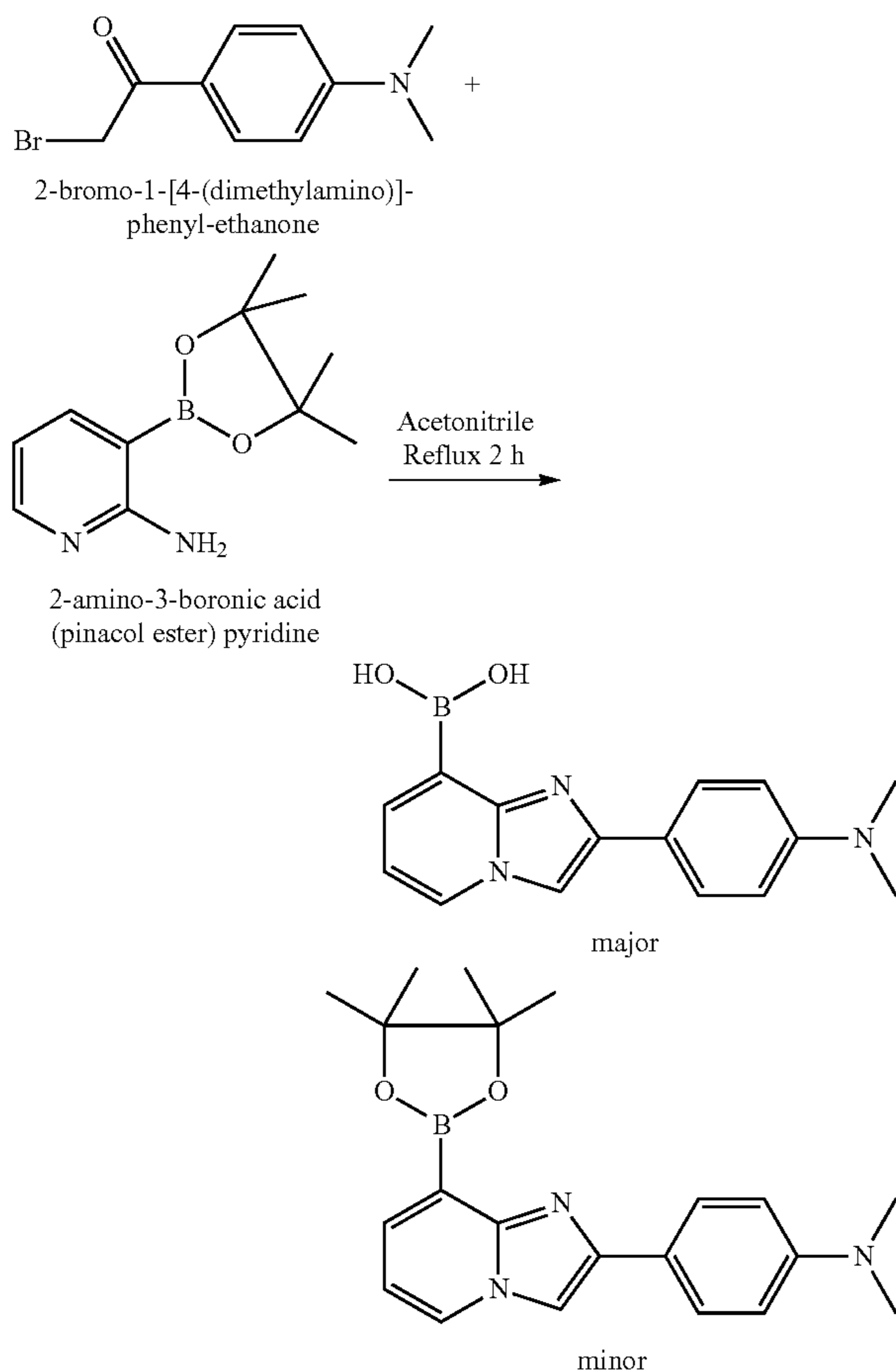
Scheme 2. Synthesis of B-DIP
