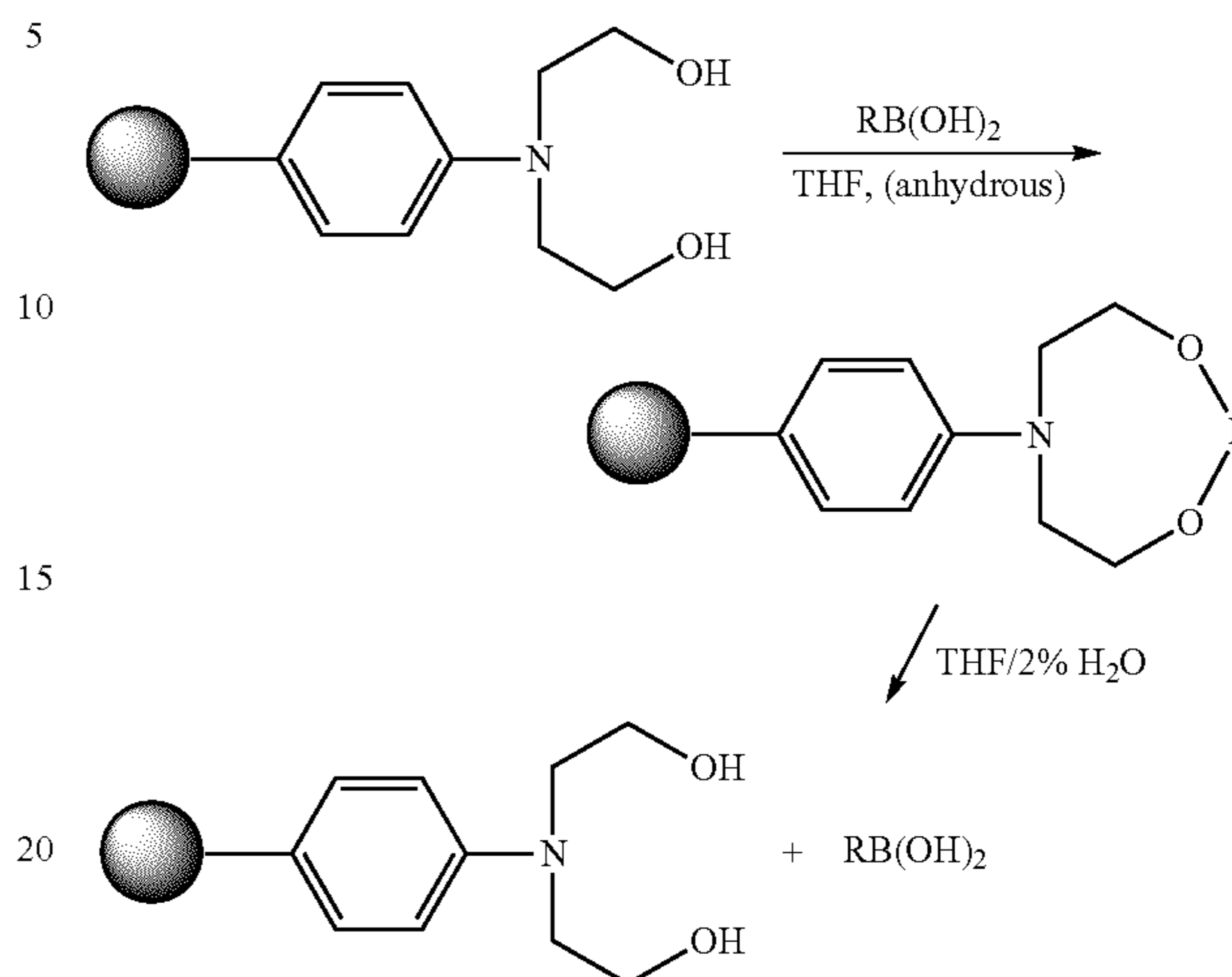
Scheme 3. Purification of boronic acid derivatives by affinity chromatography on solid support N, N, Diethanolaminomethyl polystyrene (DEAM-PS).
