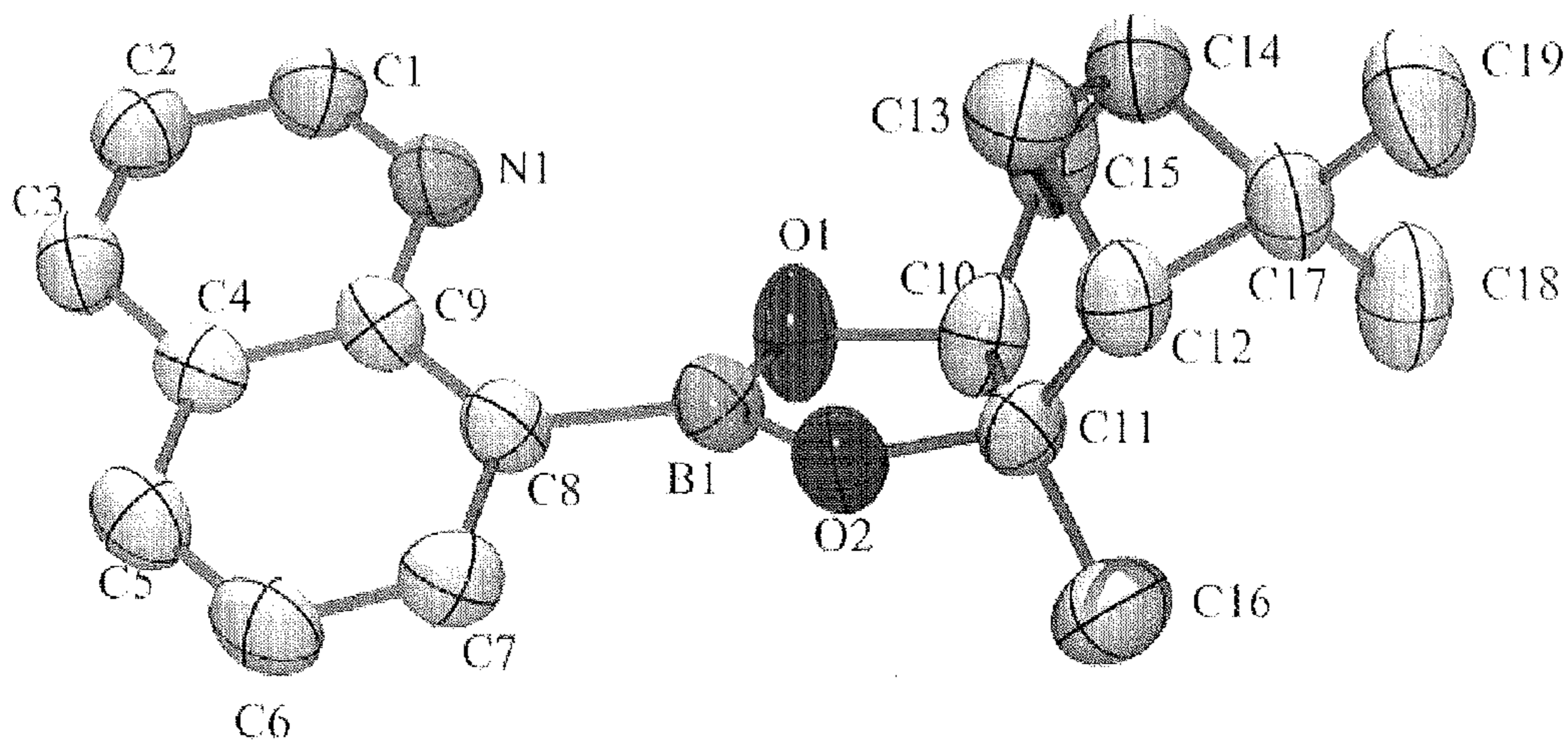
Figure 1. X-ray crystal structure of QBP.
