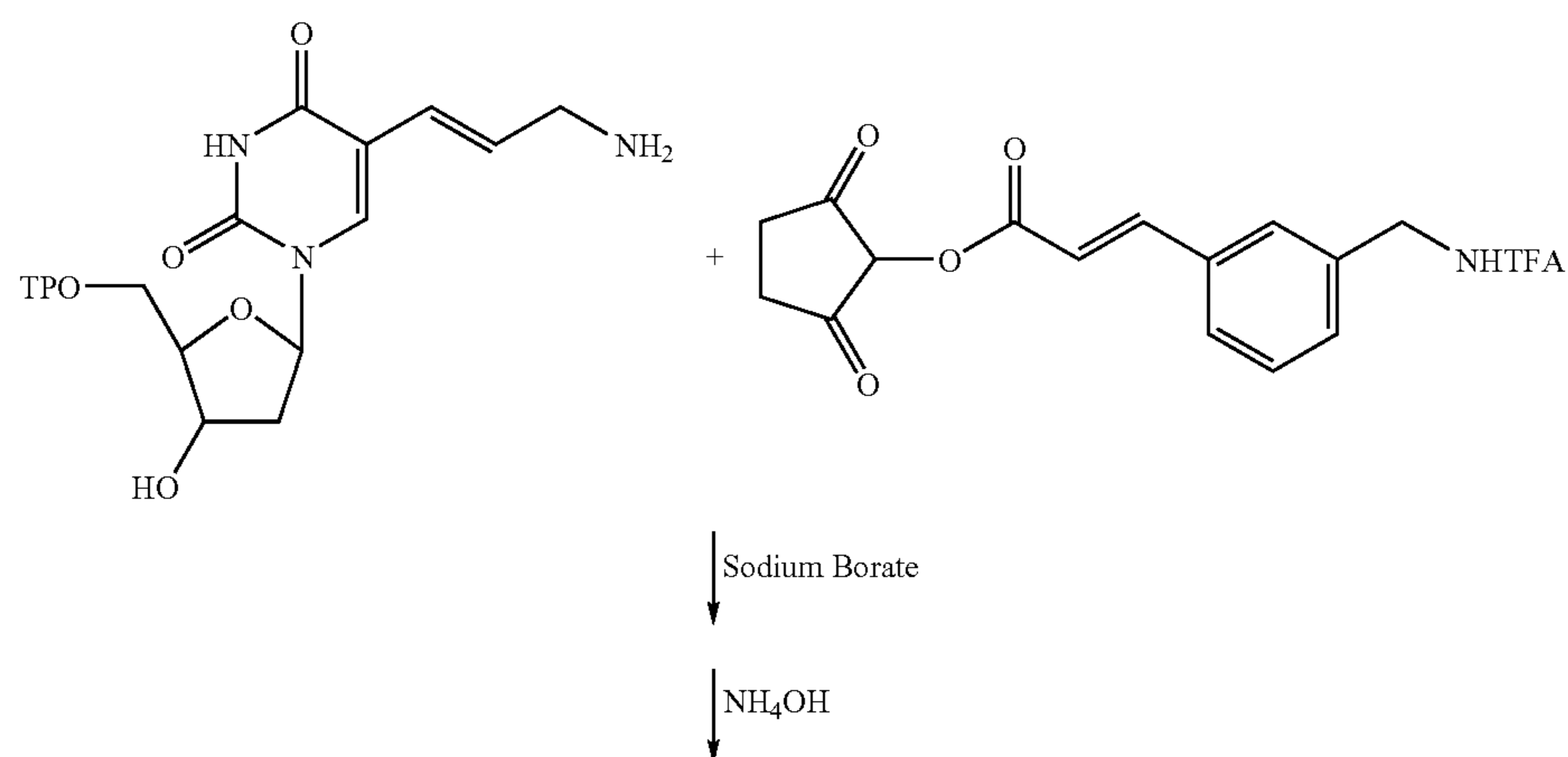
Scheme 14
