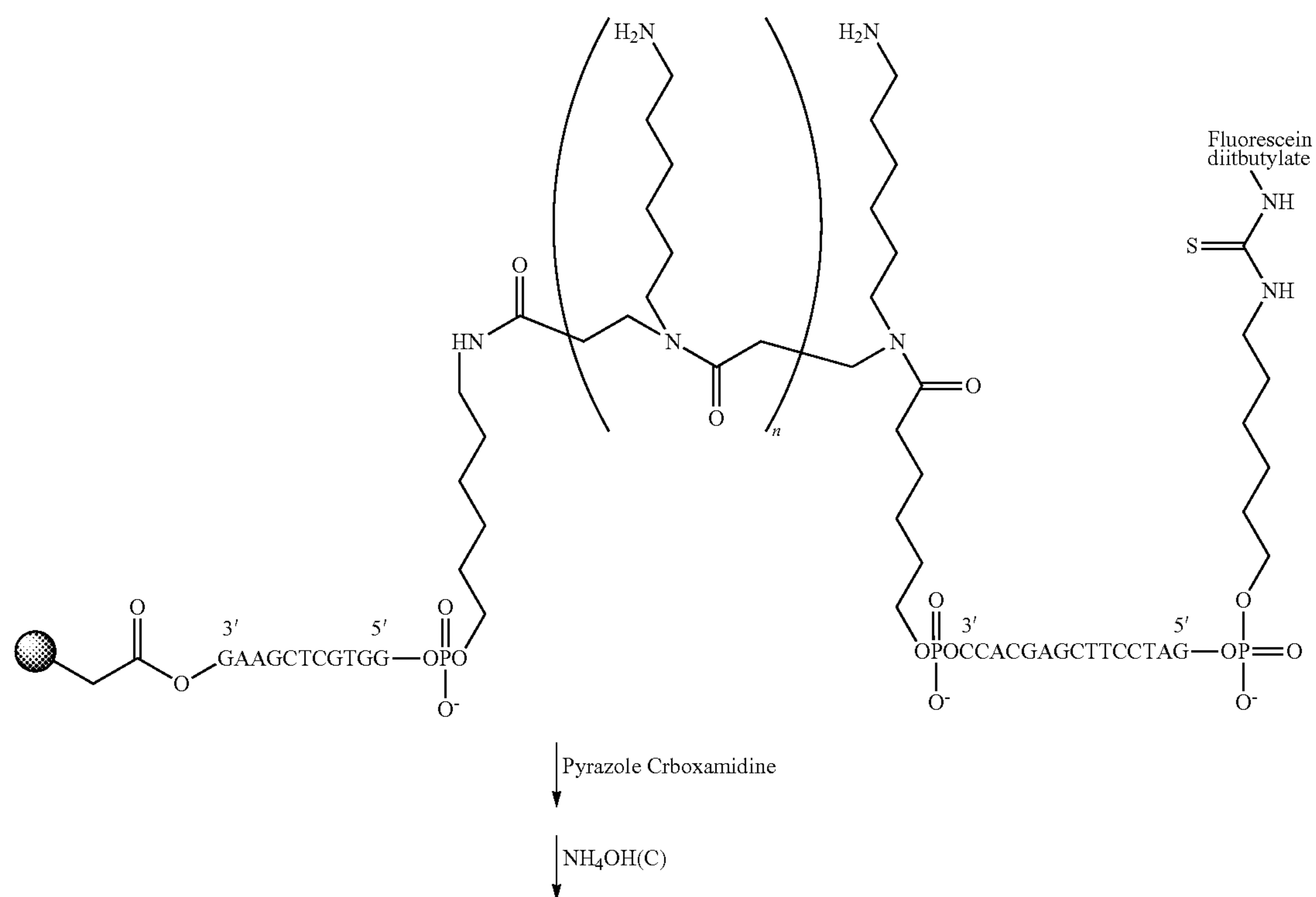
Scheme 29
