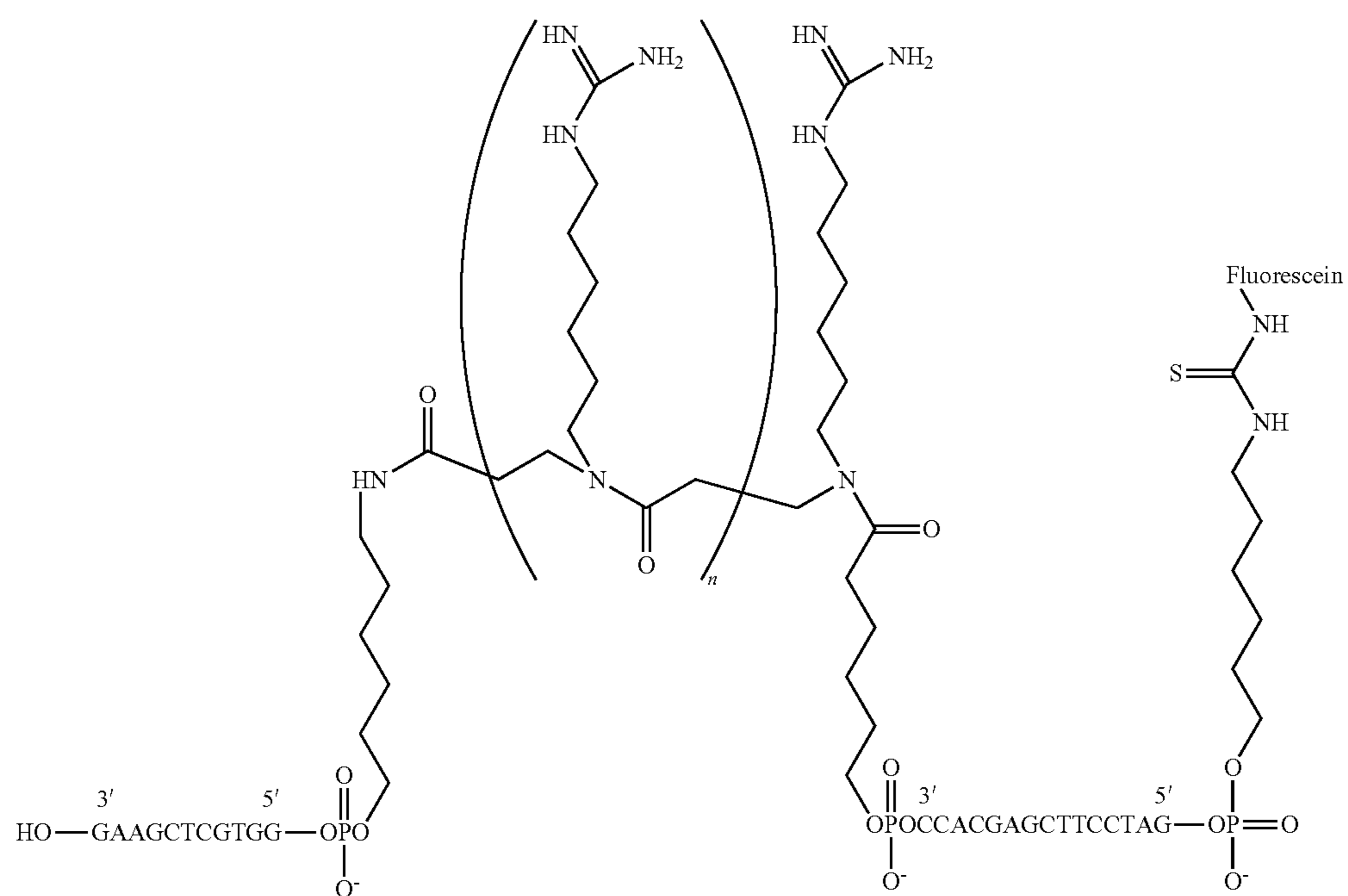
Compound 52
