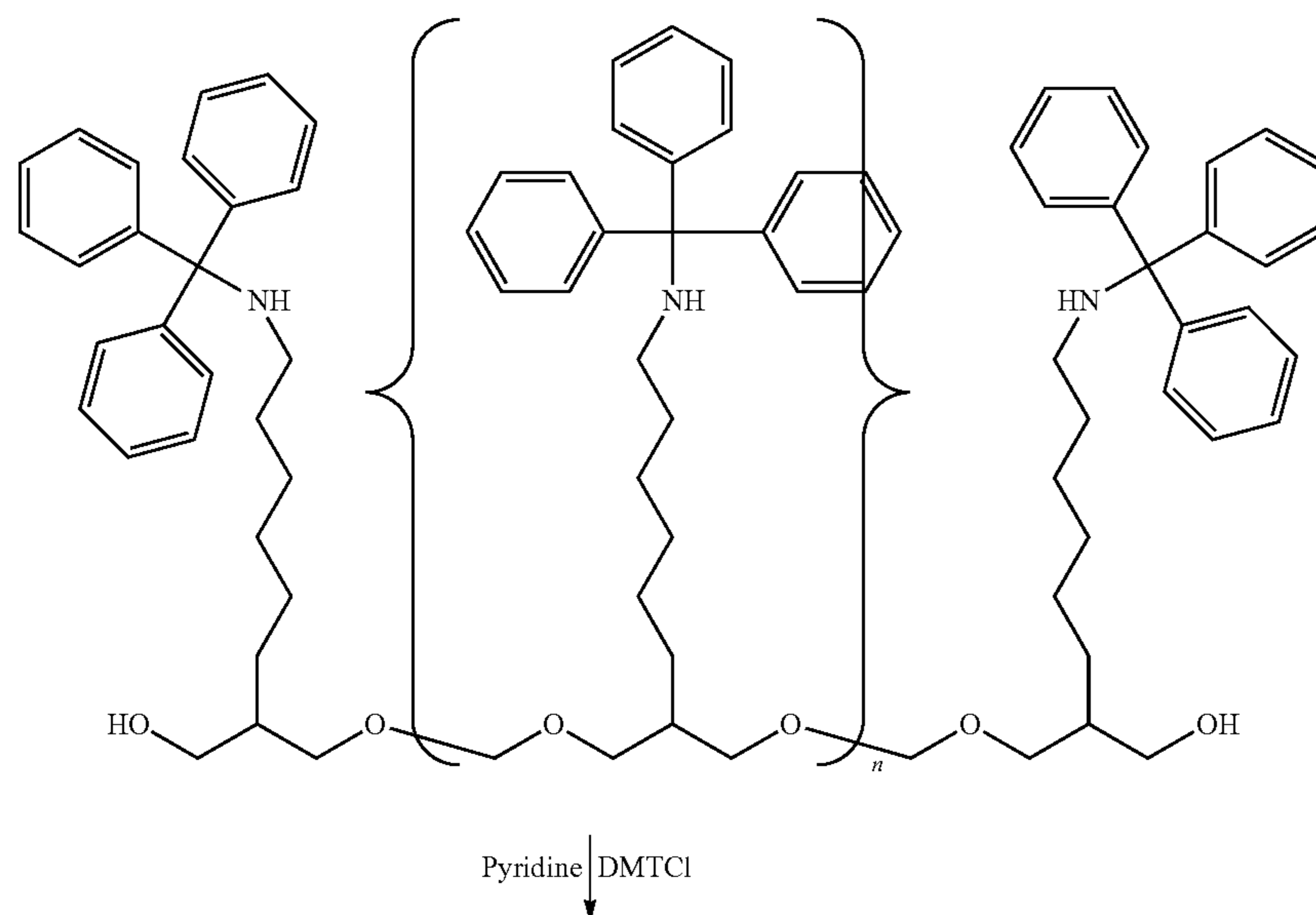
Scheme 62
