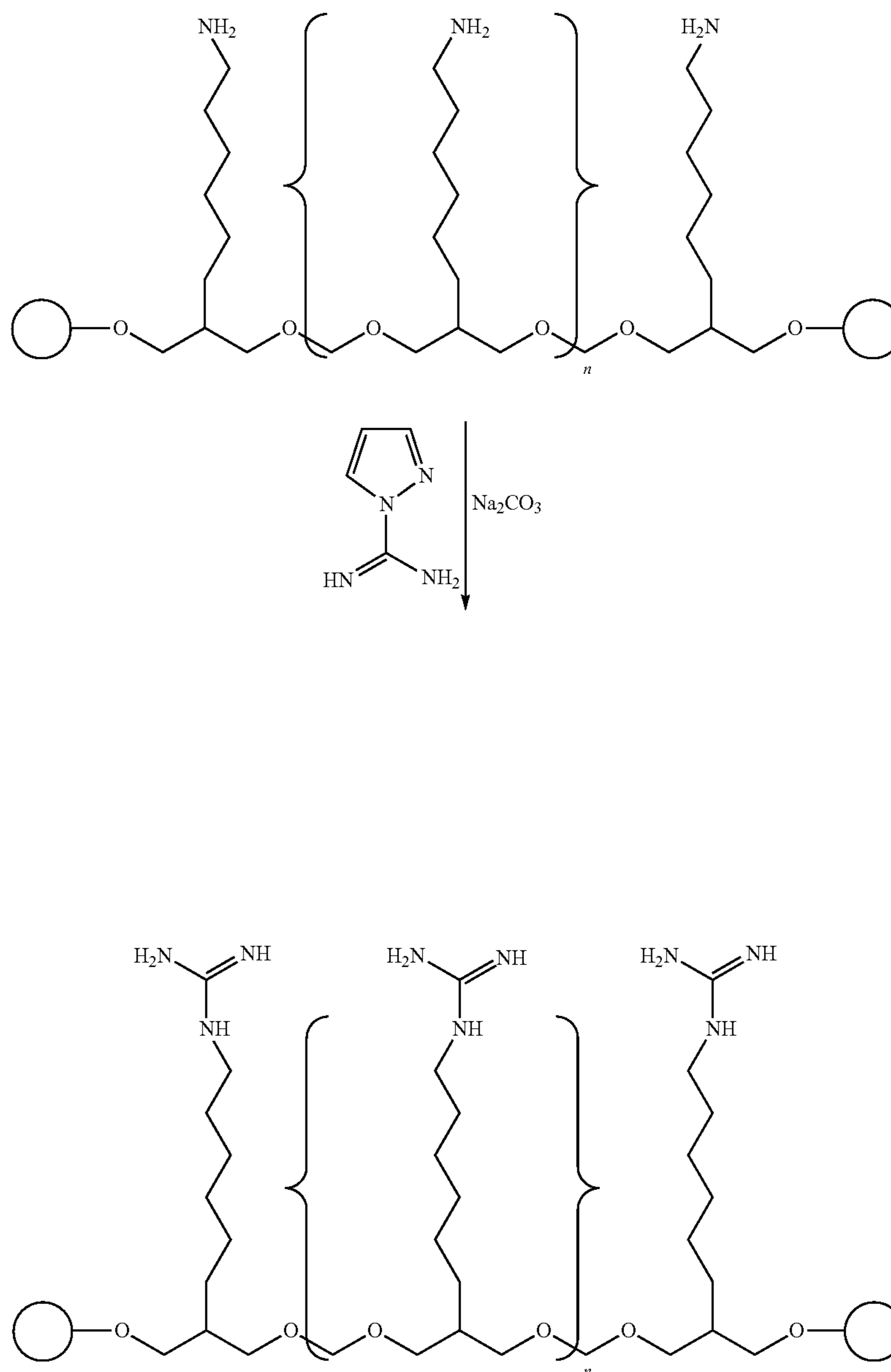
Scheme 53
