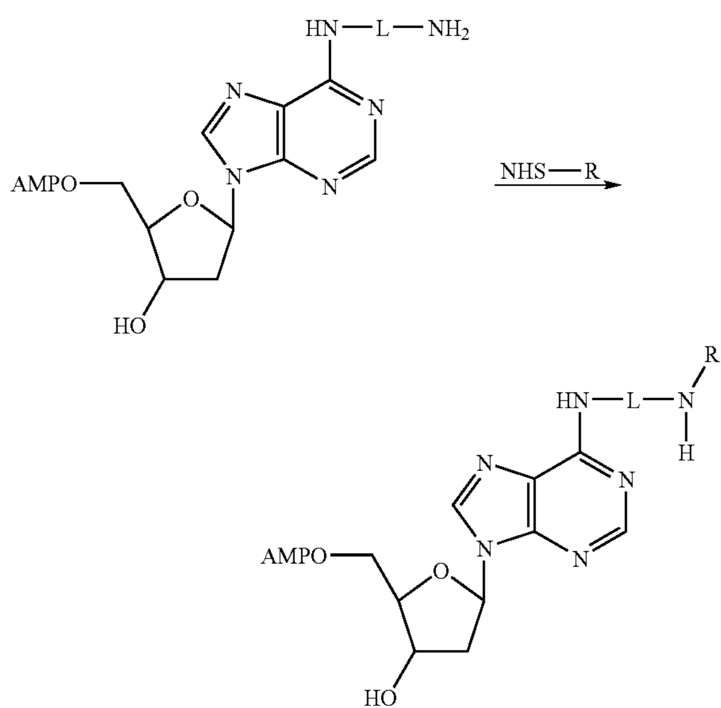
Scheme 13
