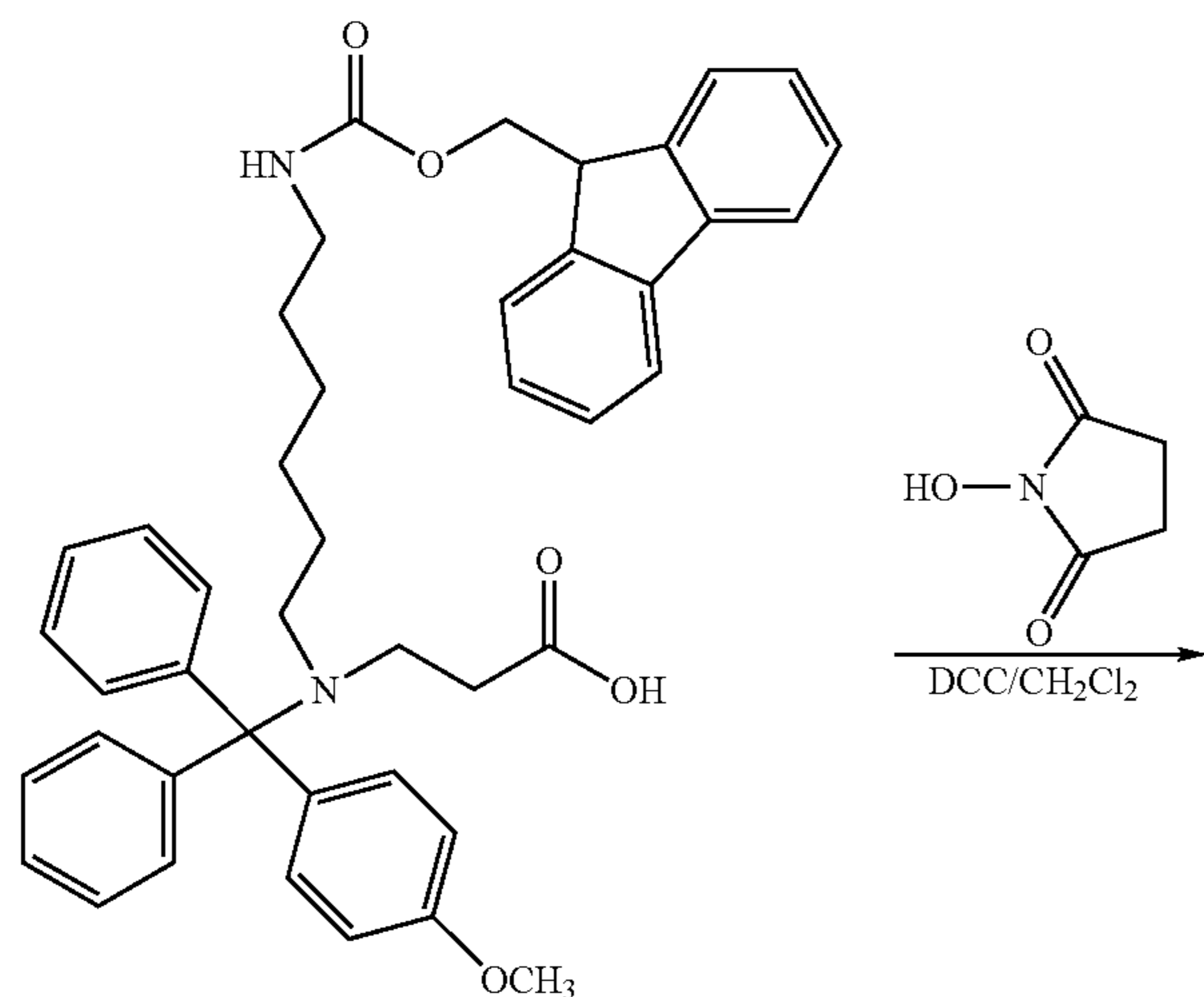
Scheme 22
