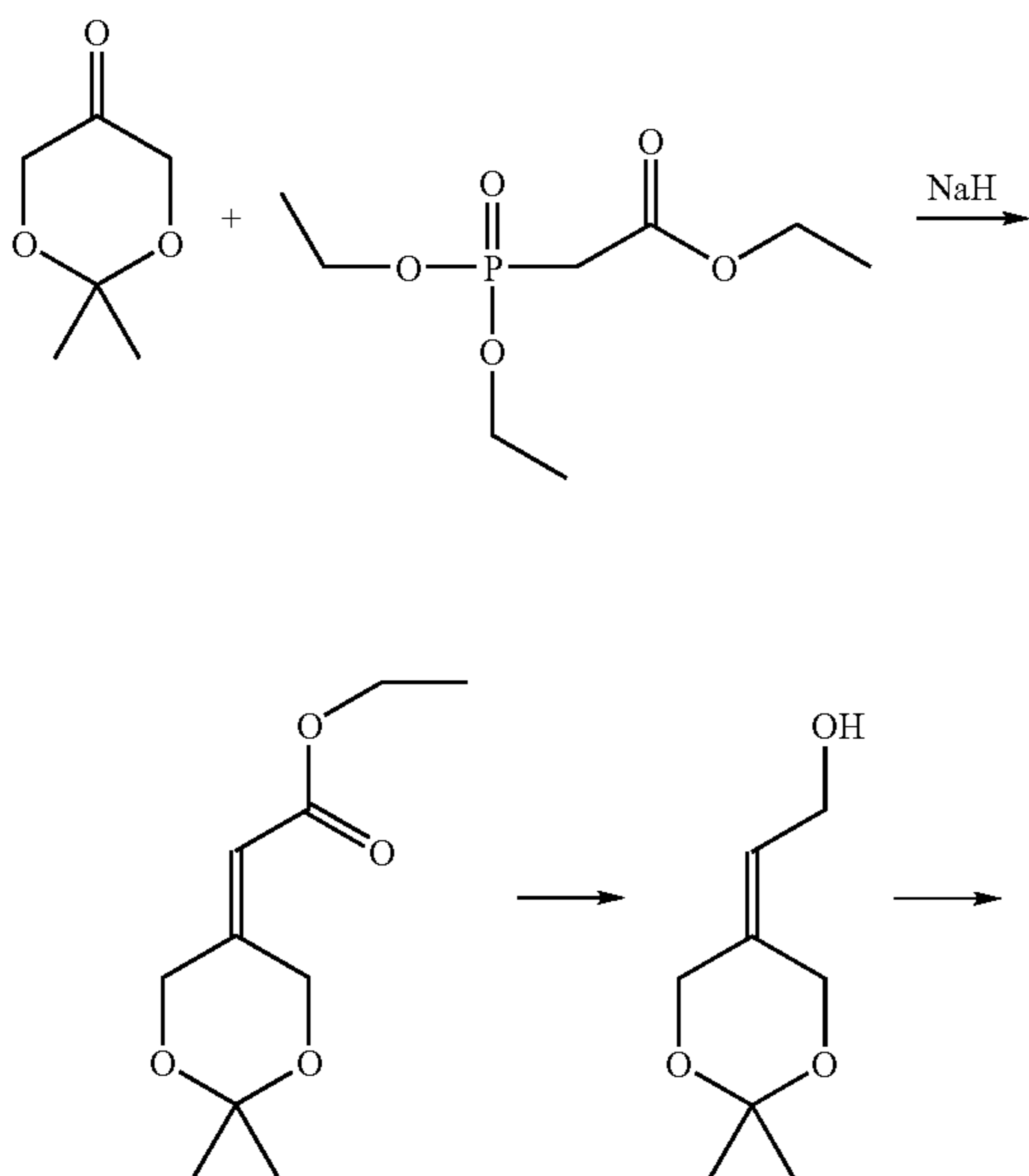
Scheme 54
