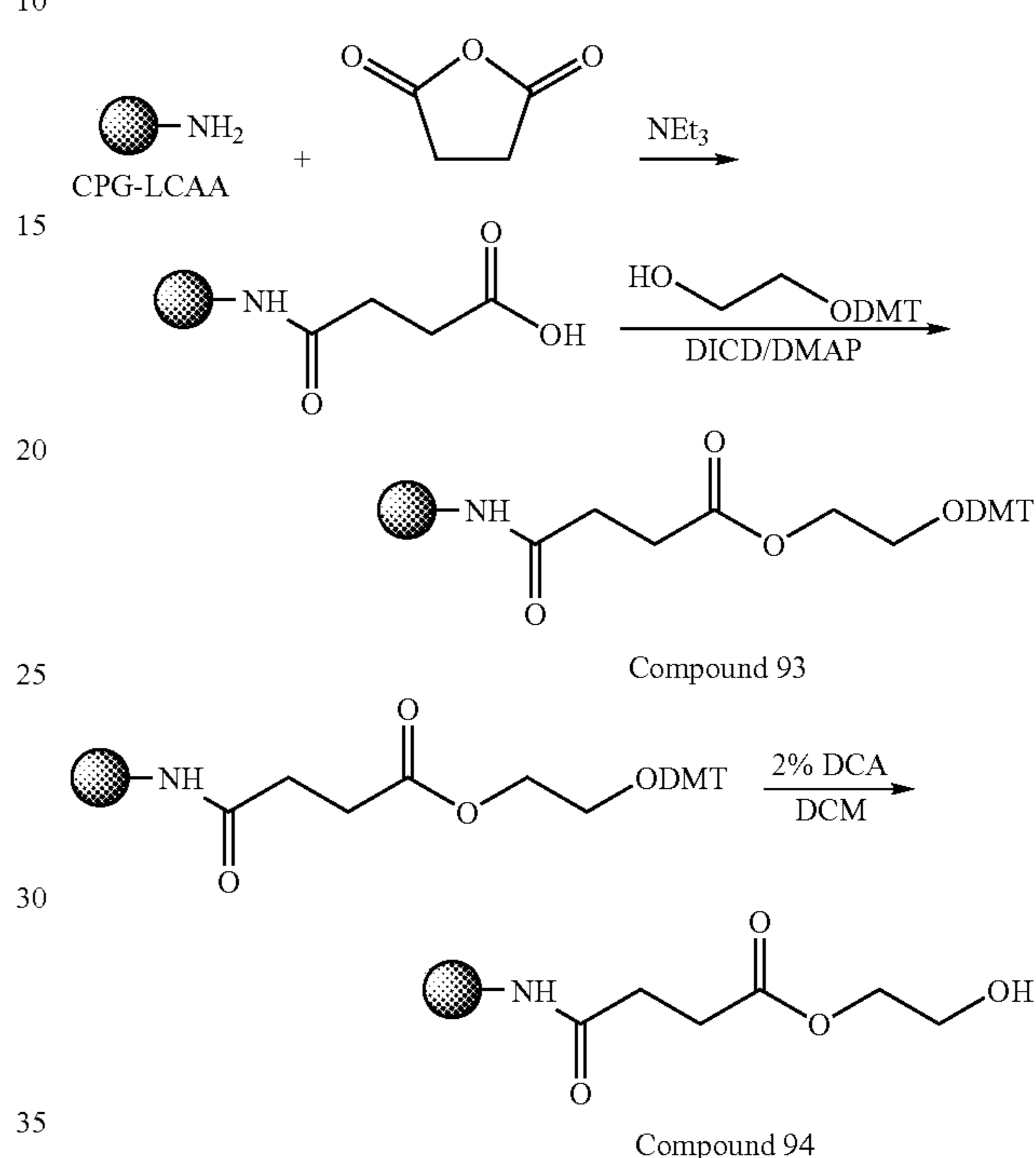
Scheme 58
