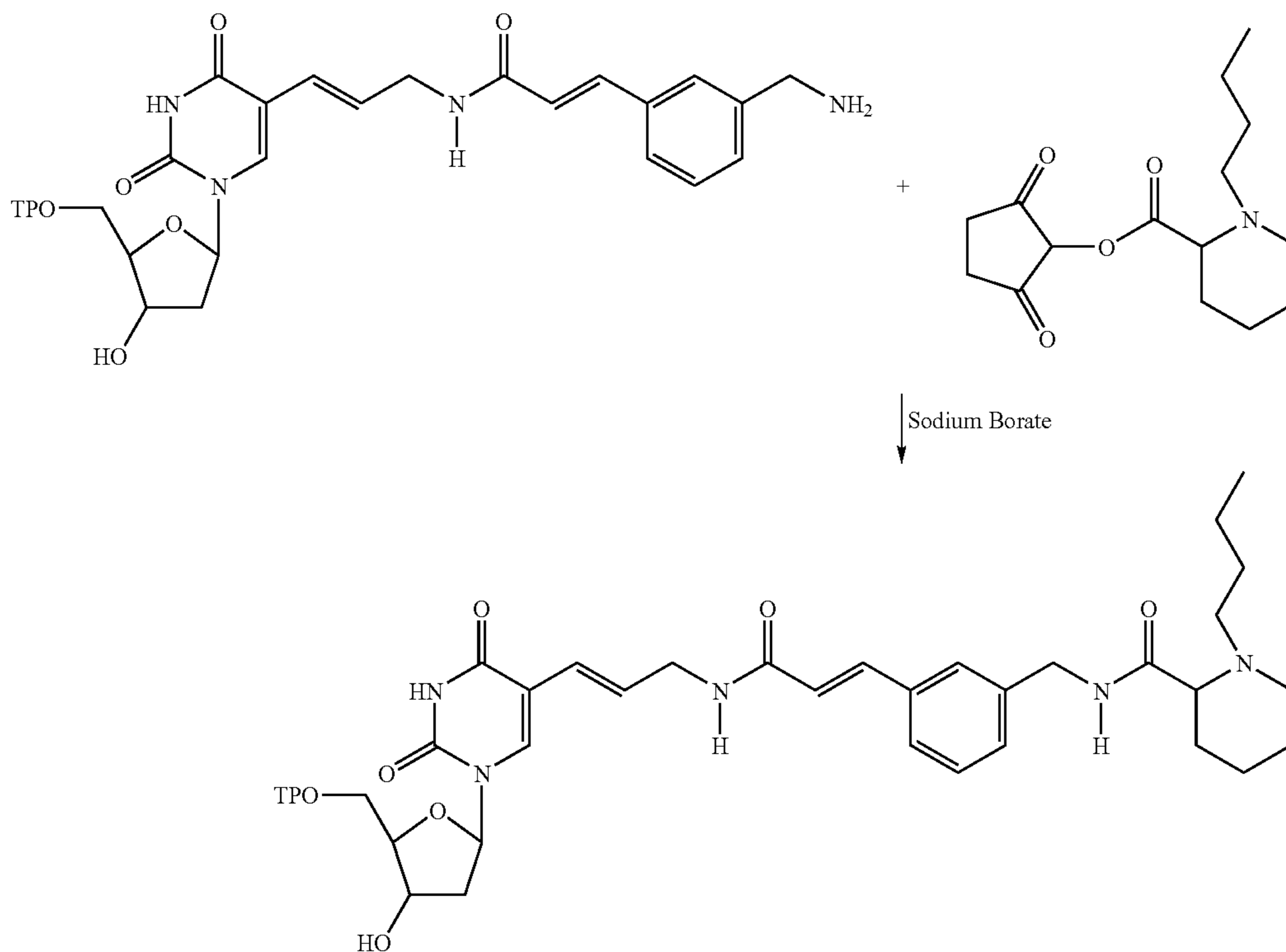
Compound 37
