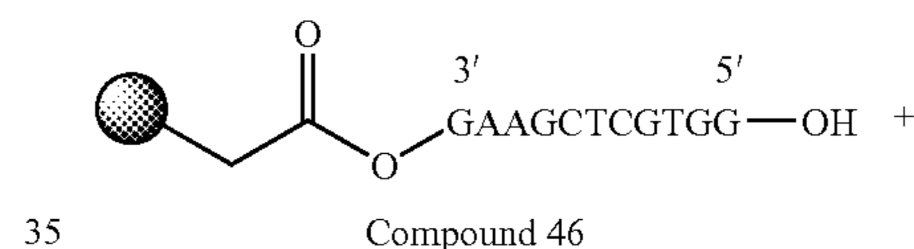
Scheme 24
