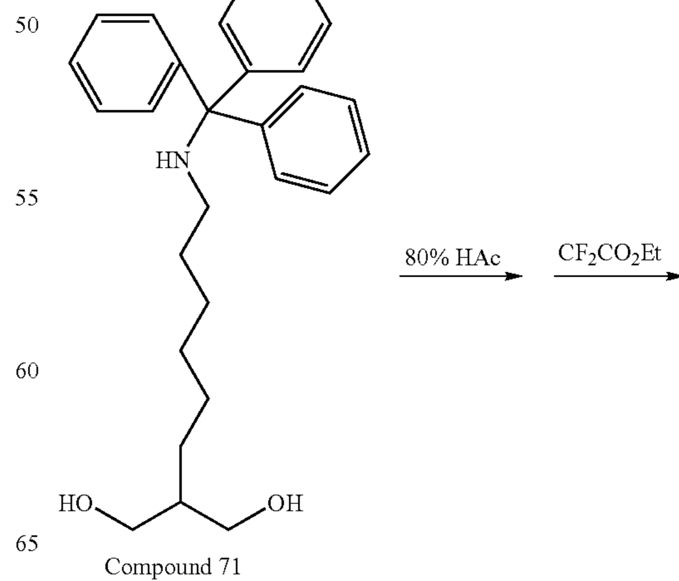
Scheme 55
