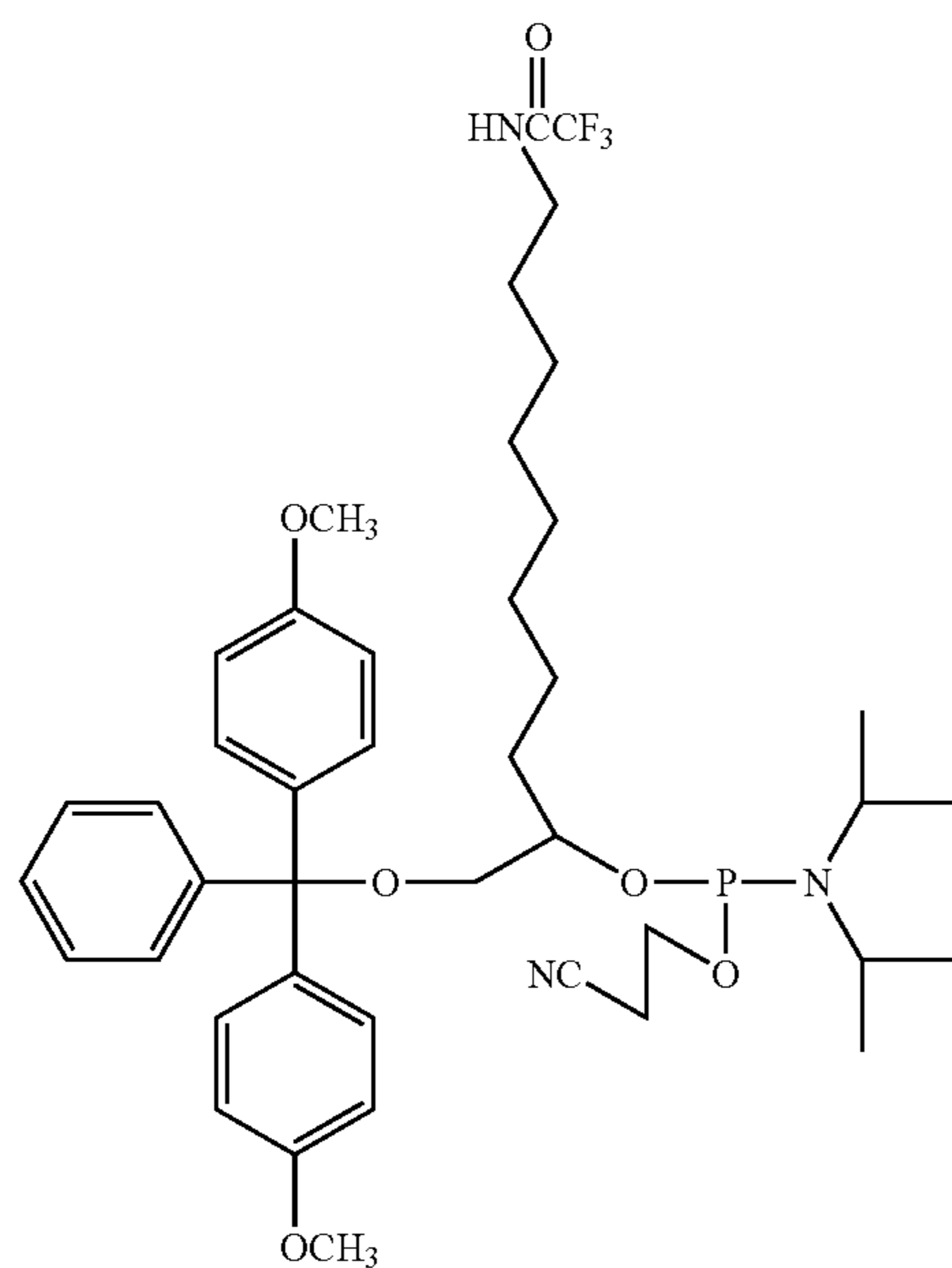
Compound 61
