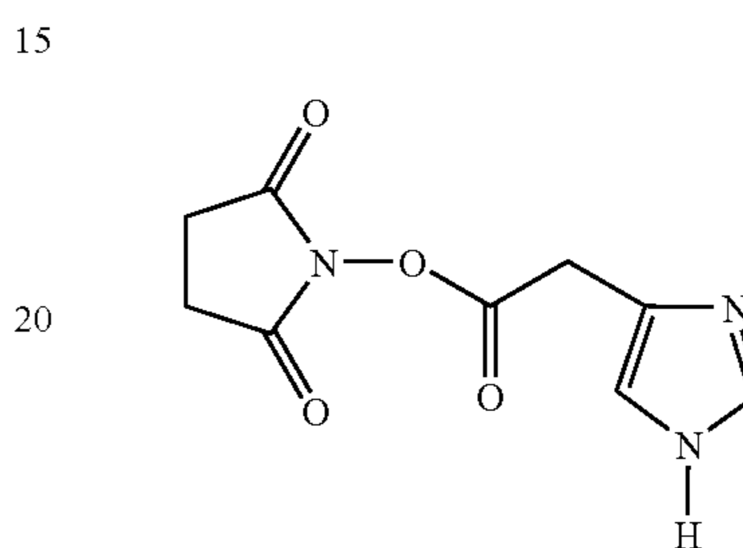
NHS-Imidazole
