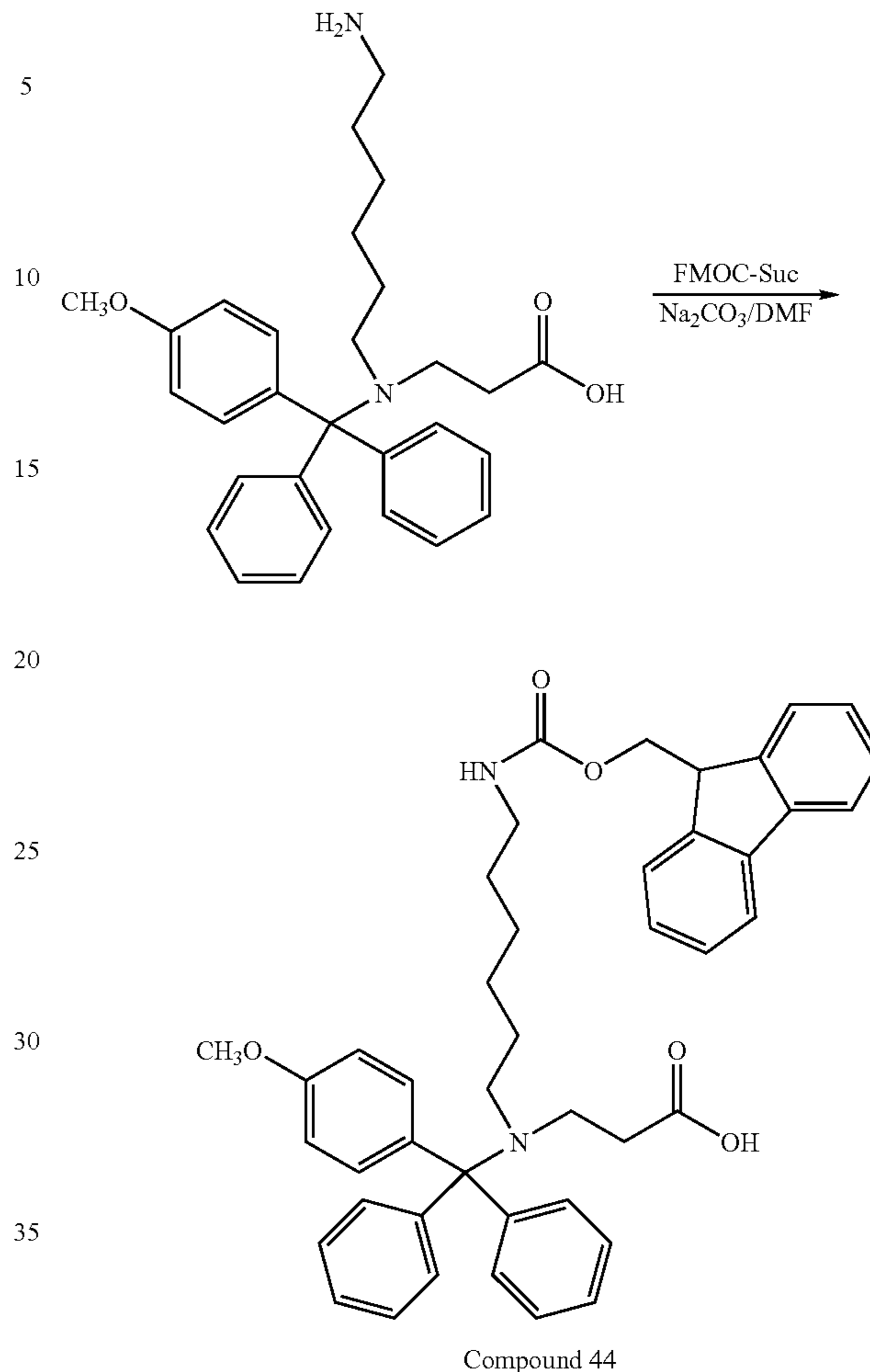
Scheme 21
