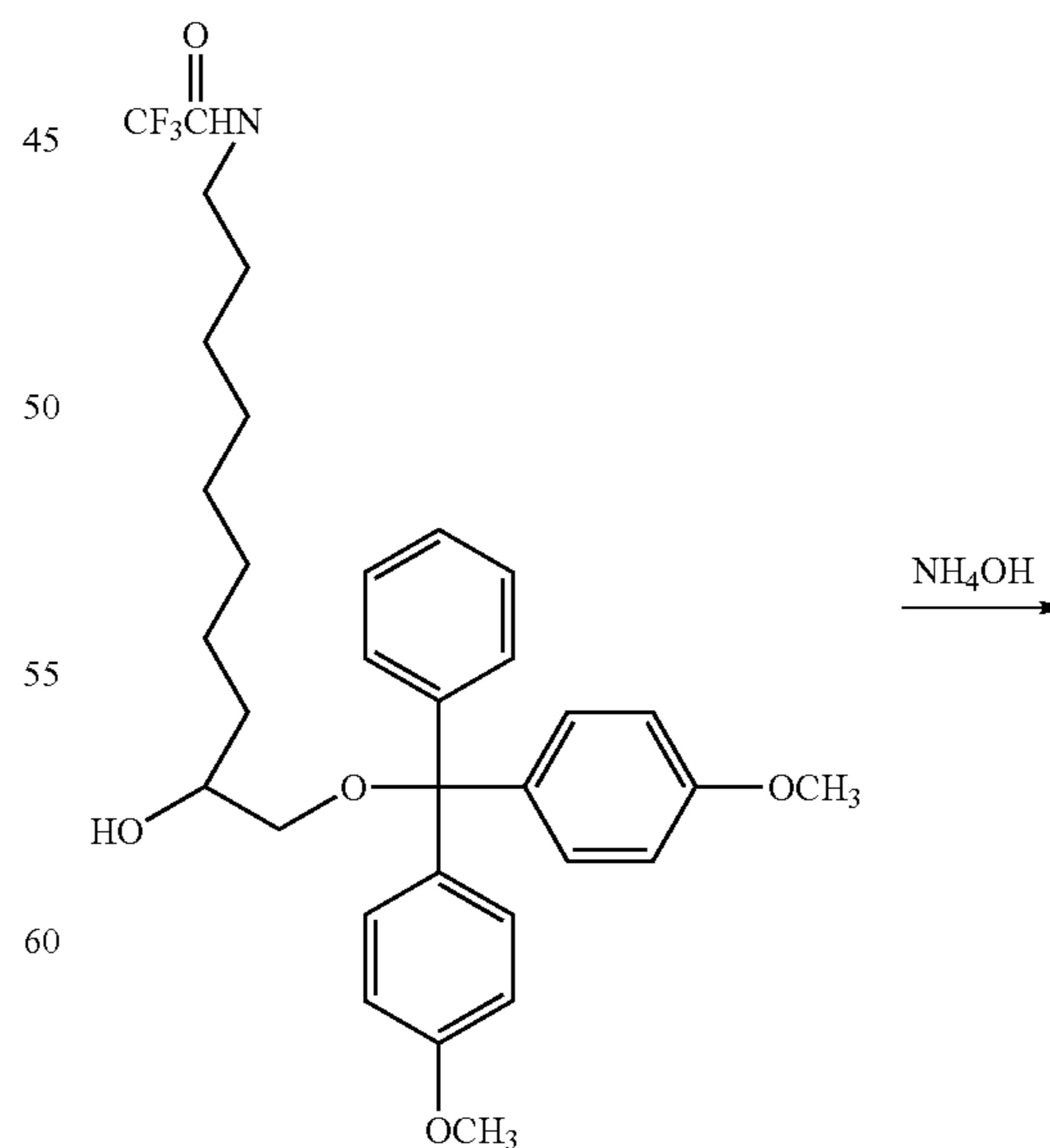
Scheme 37
