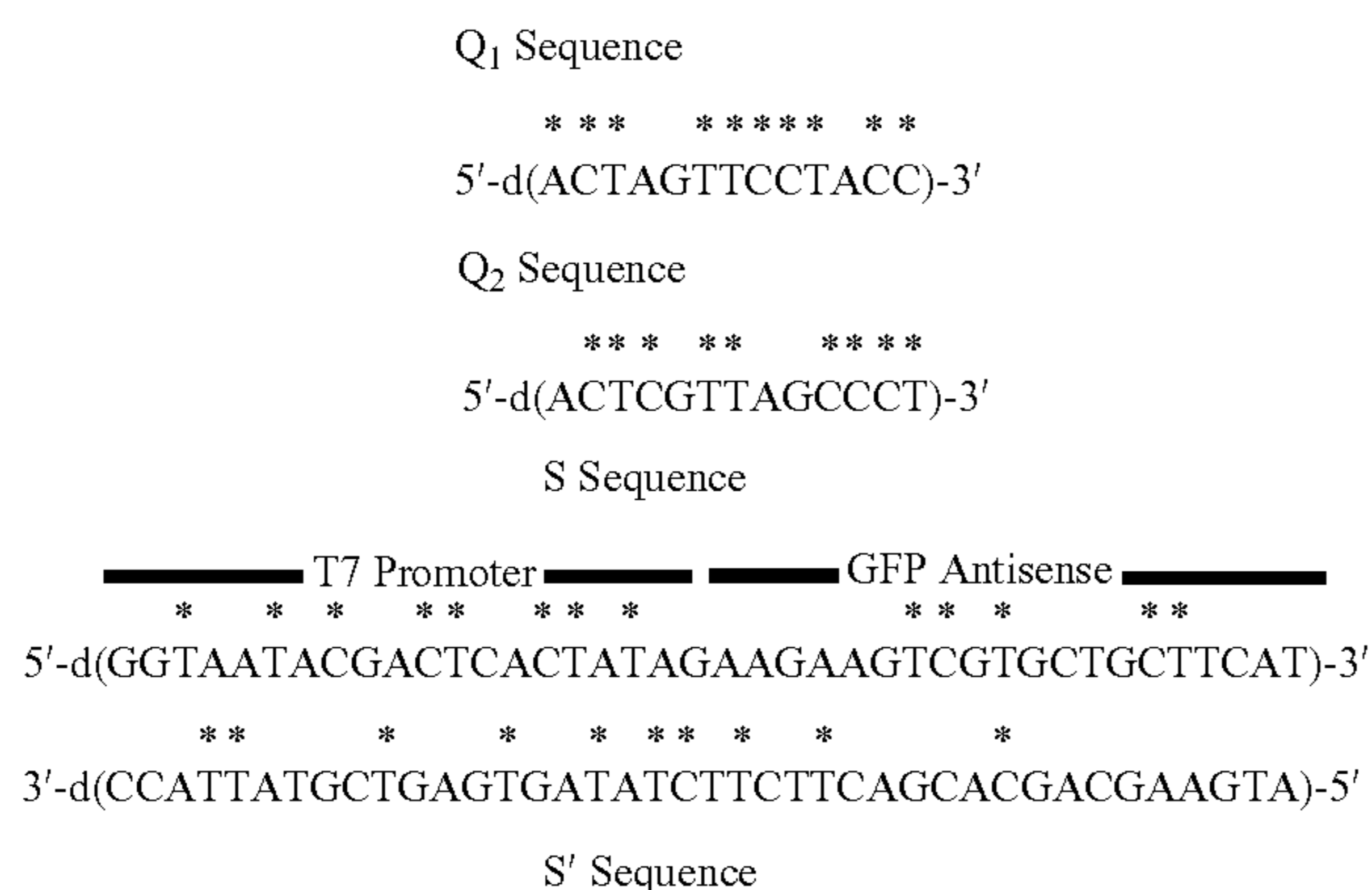
Scheme 73
