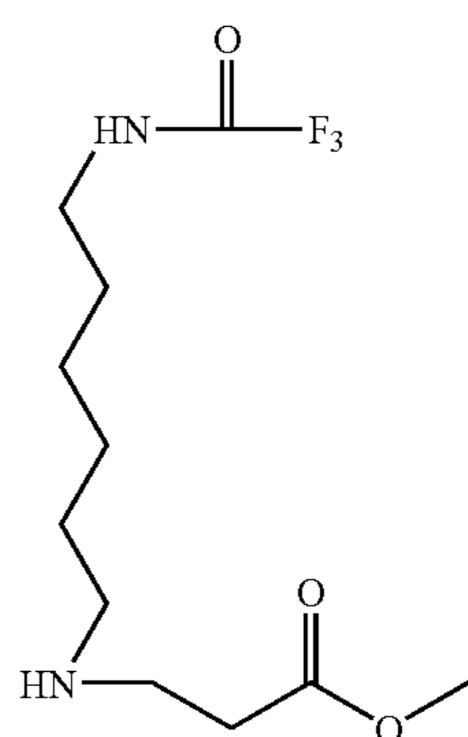
Compound 41
