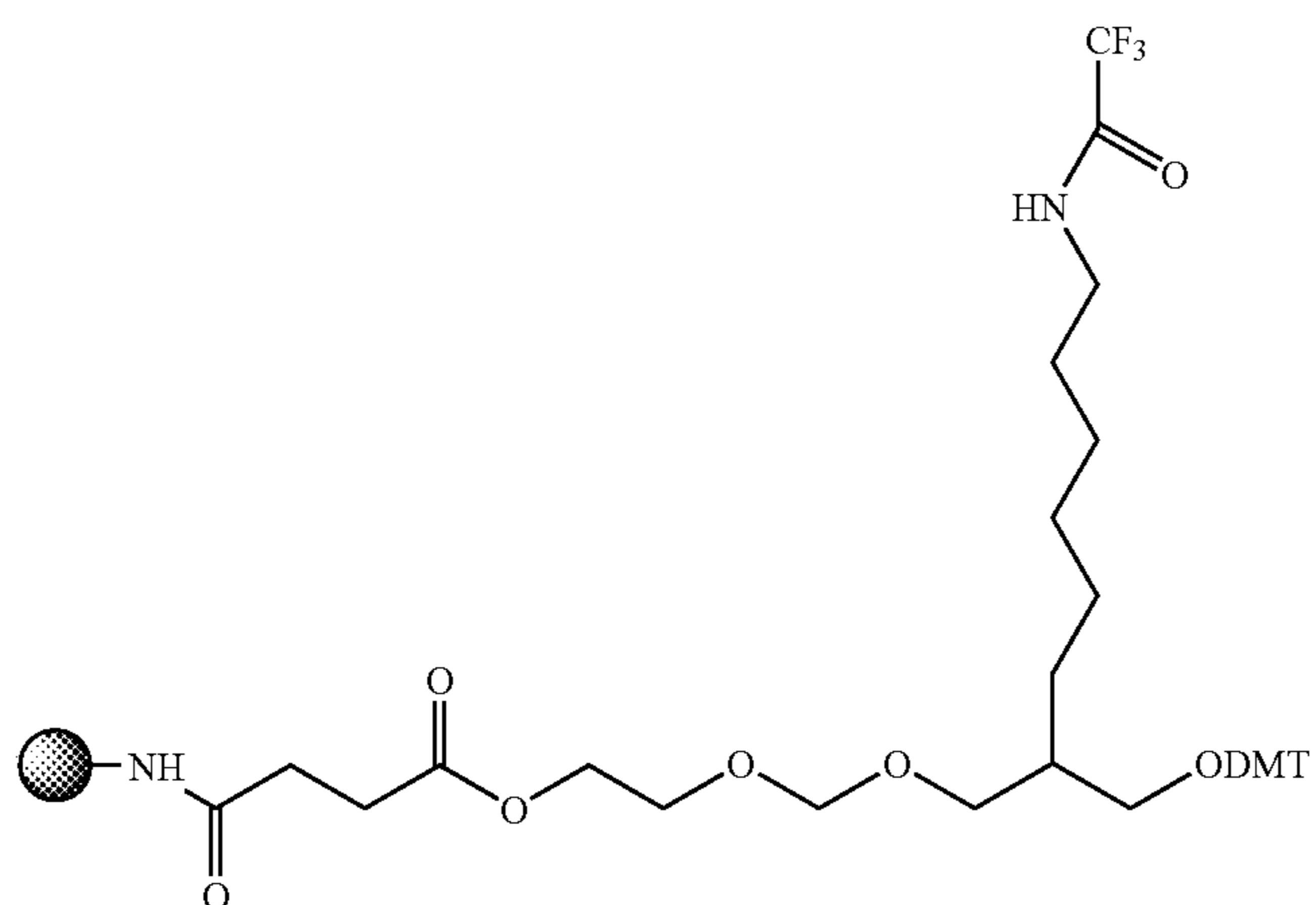
Compound 95
