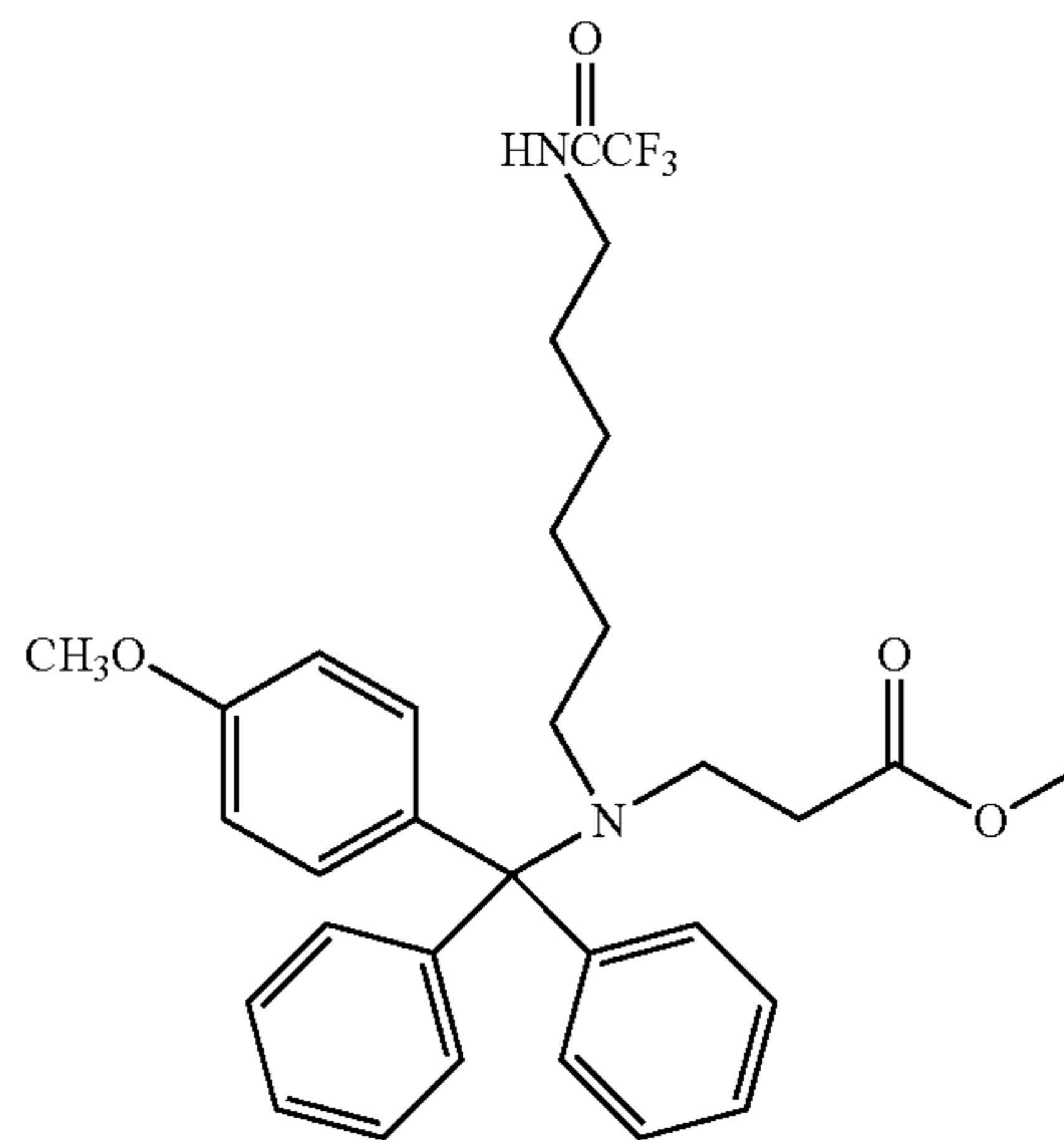
Compound 42
