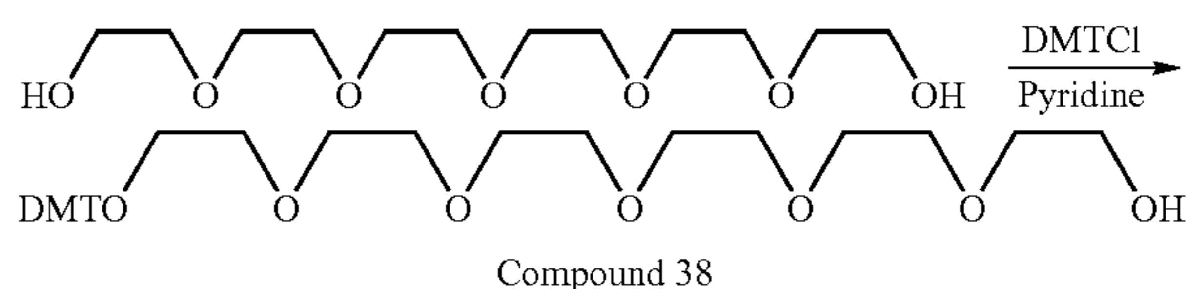
Scheme 15
