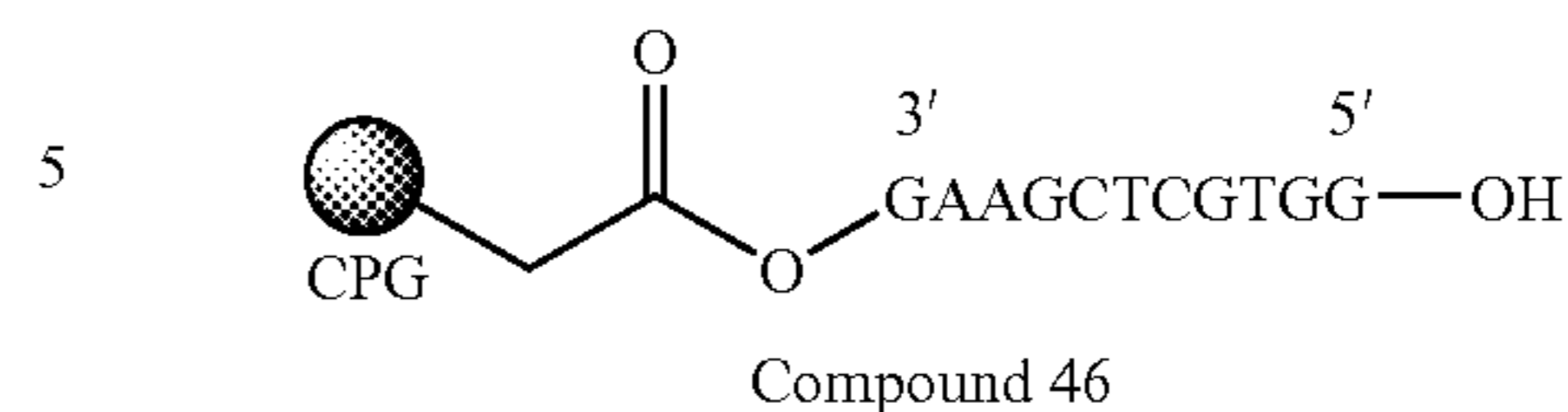
Scheme 23
