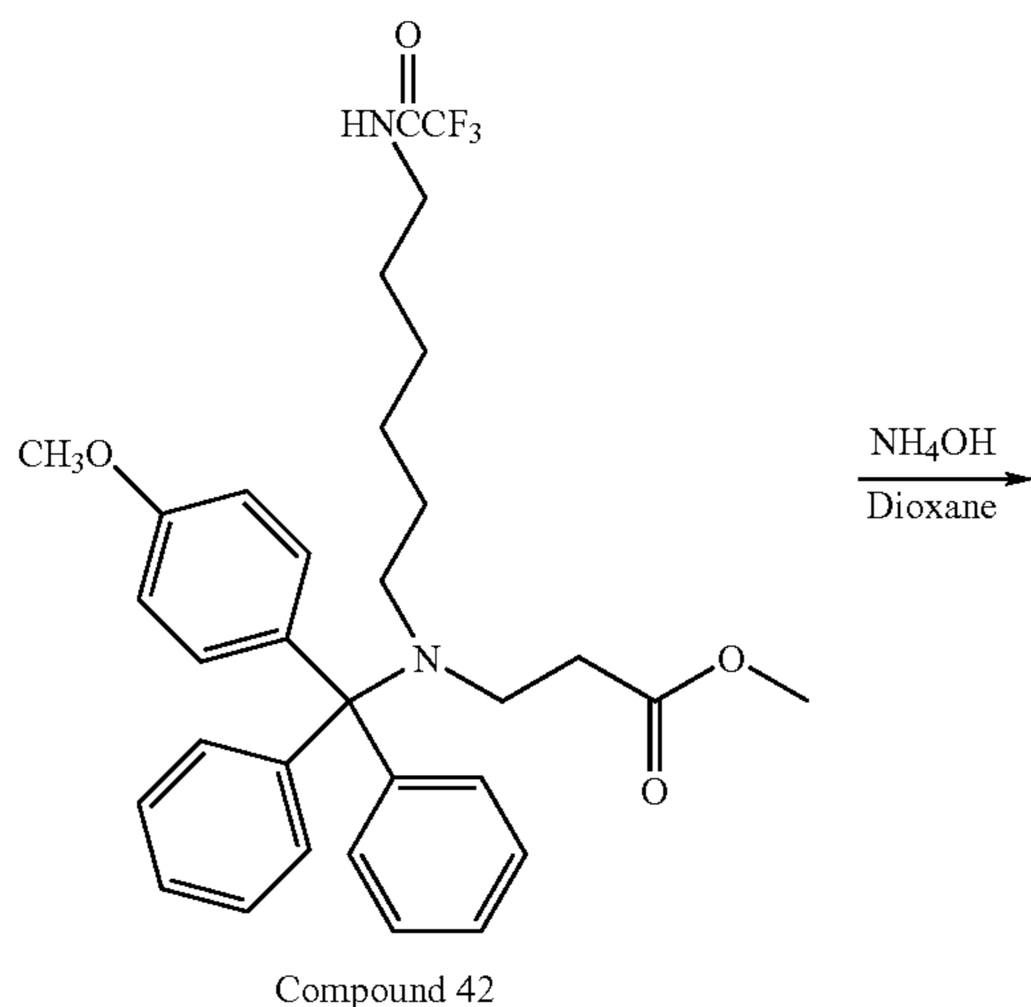
Scheme 20
