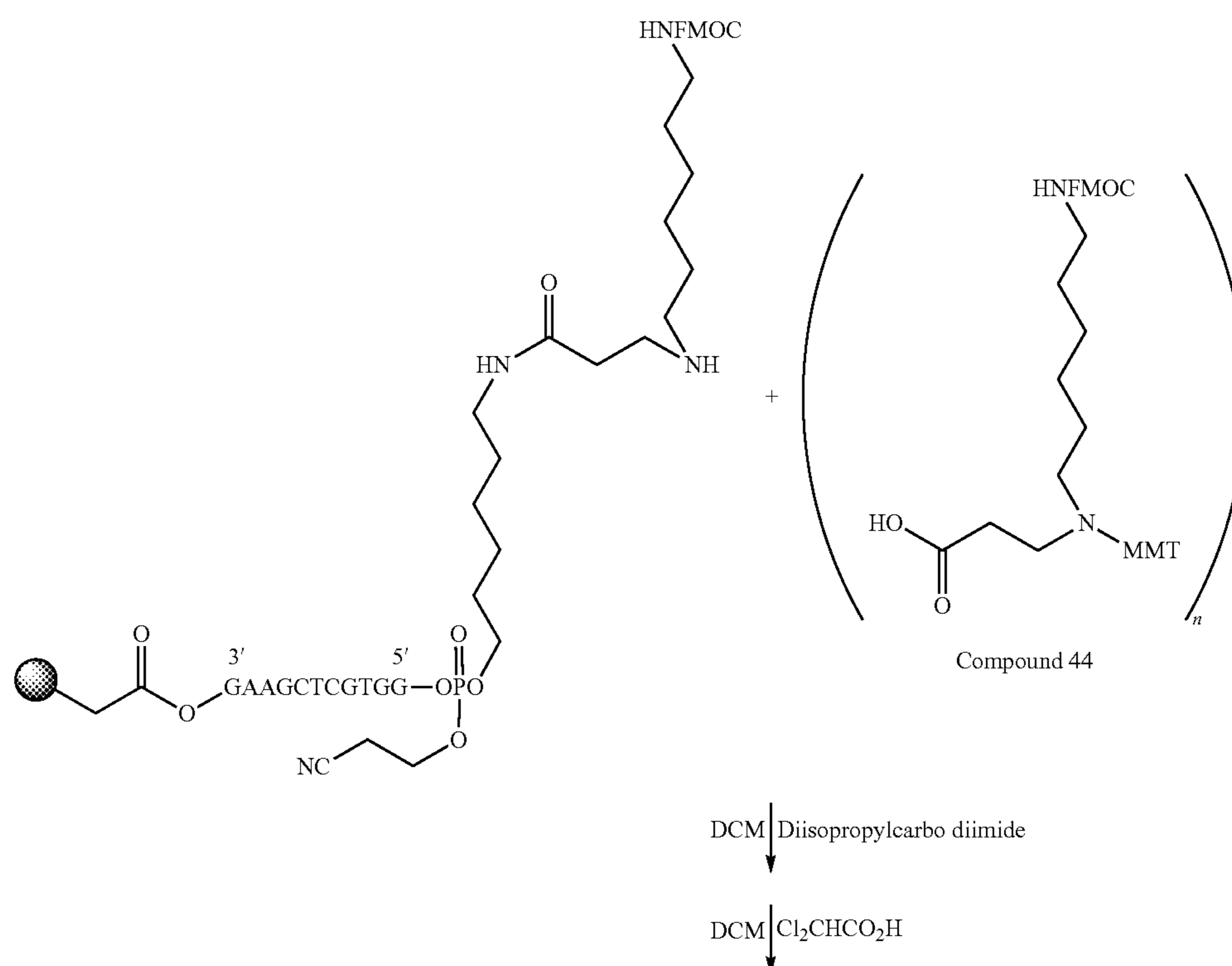
Scheme 25
