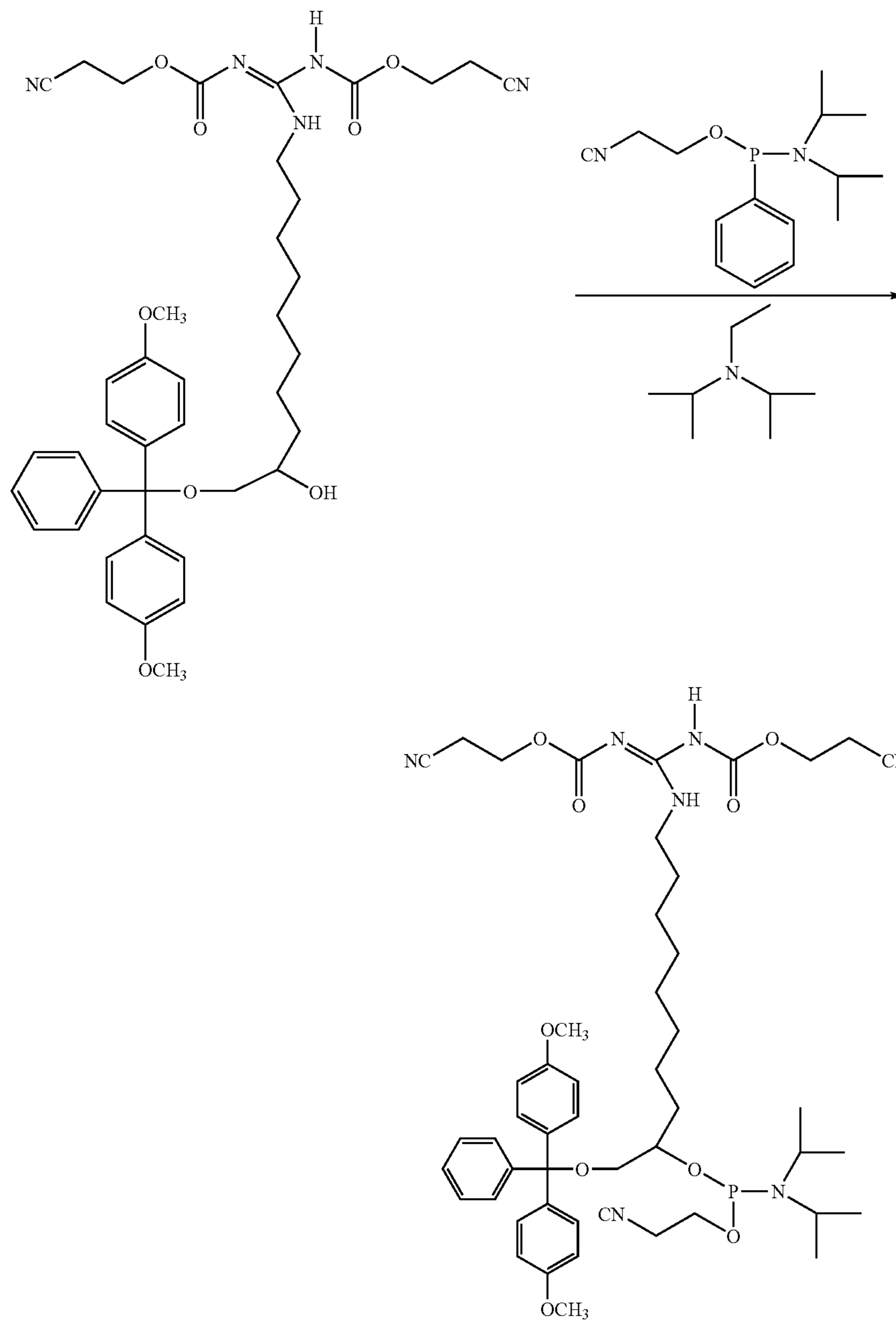
Compound 67
