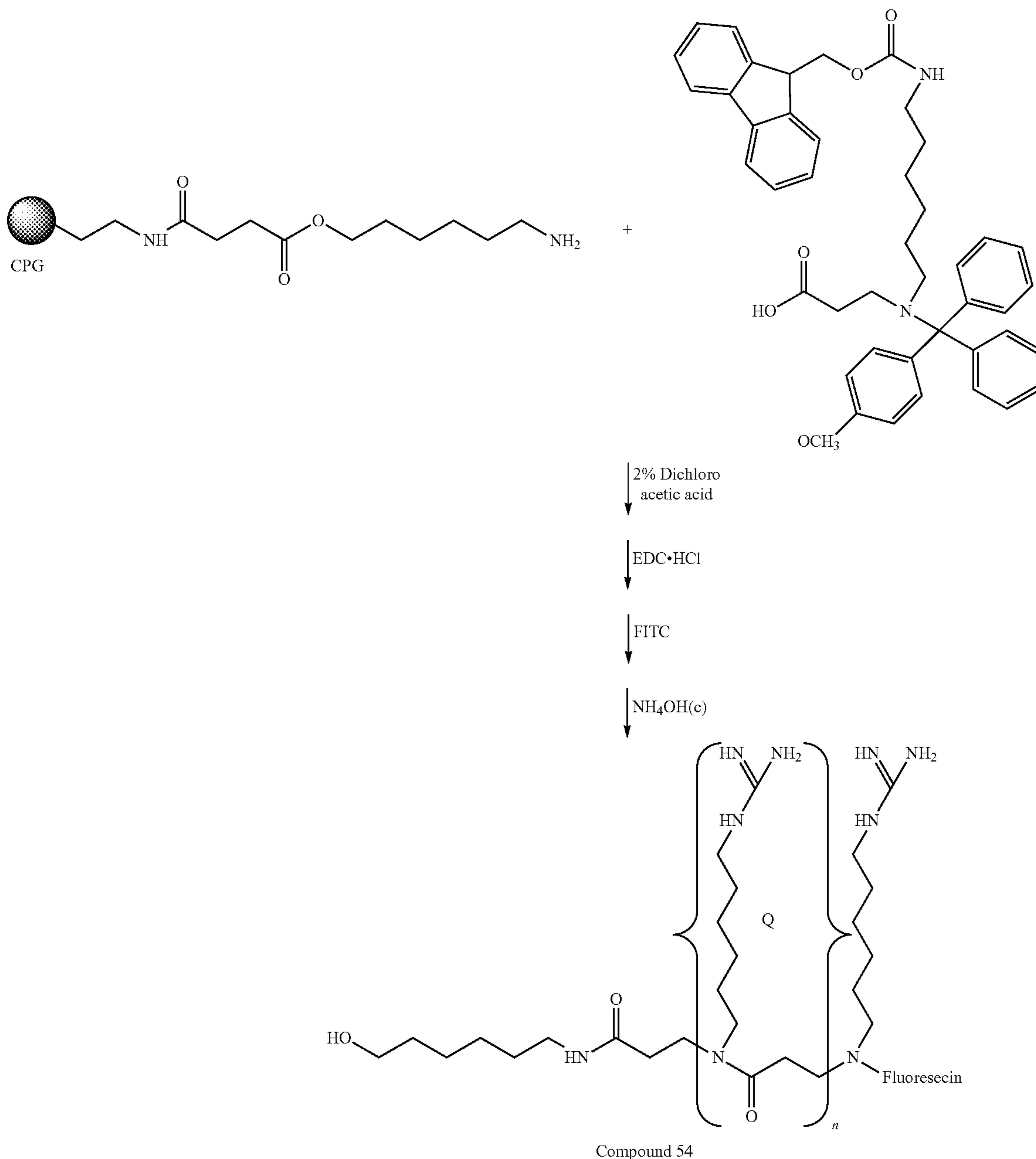
Scheme 79
