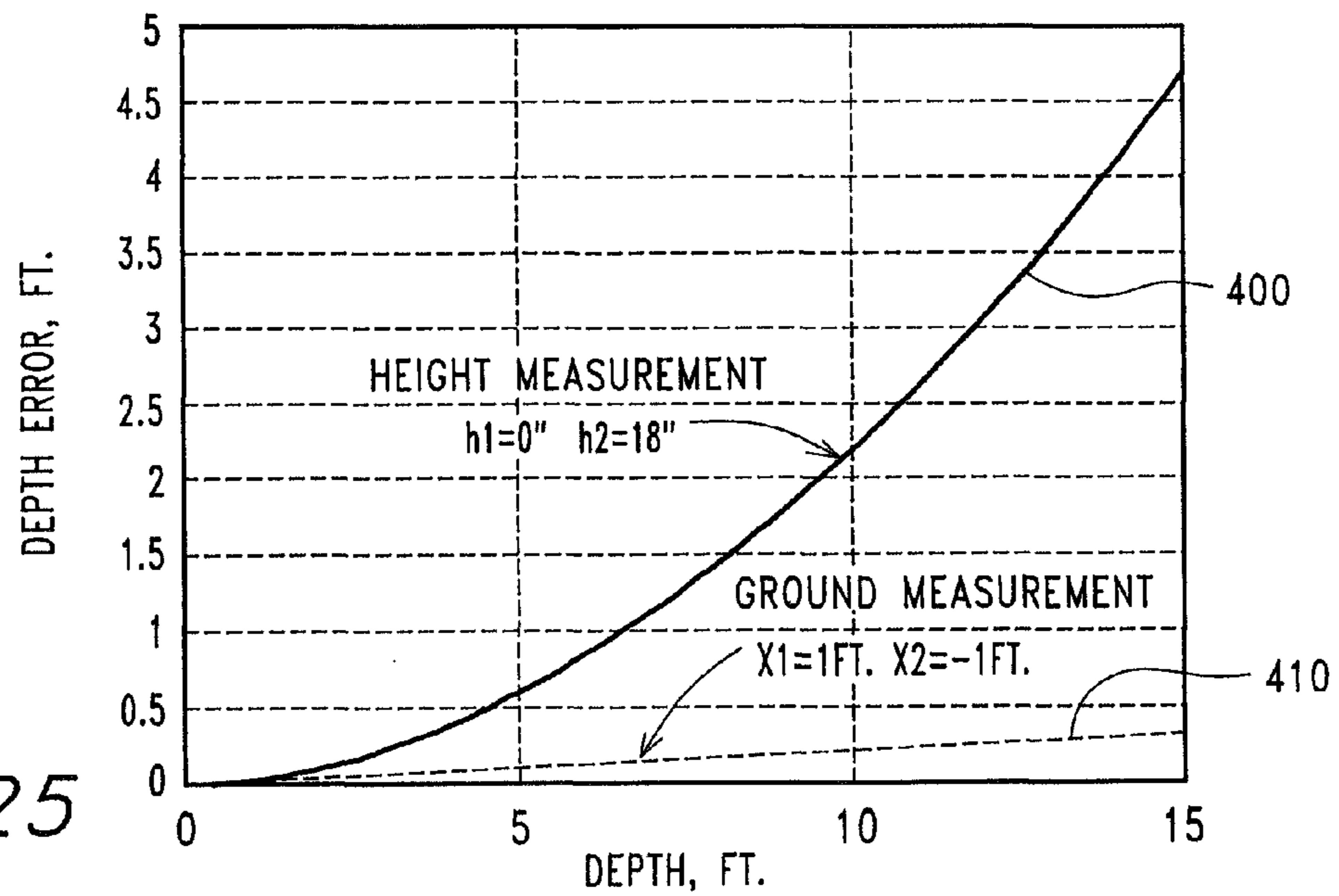
DEPTH ERROR DUE TO A FLUX MEASUREMENT ERROR OF 2%
