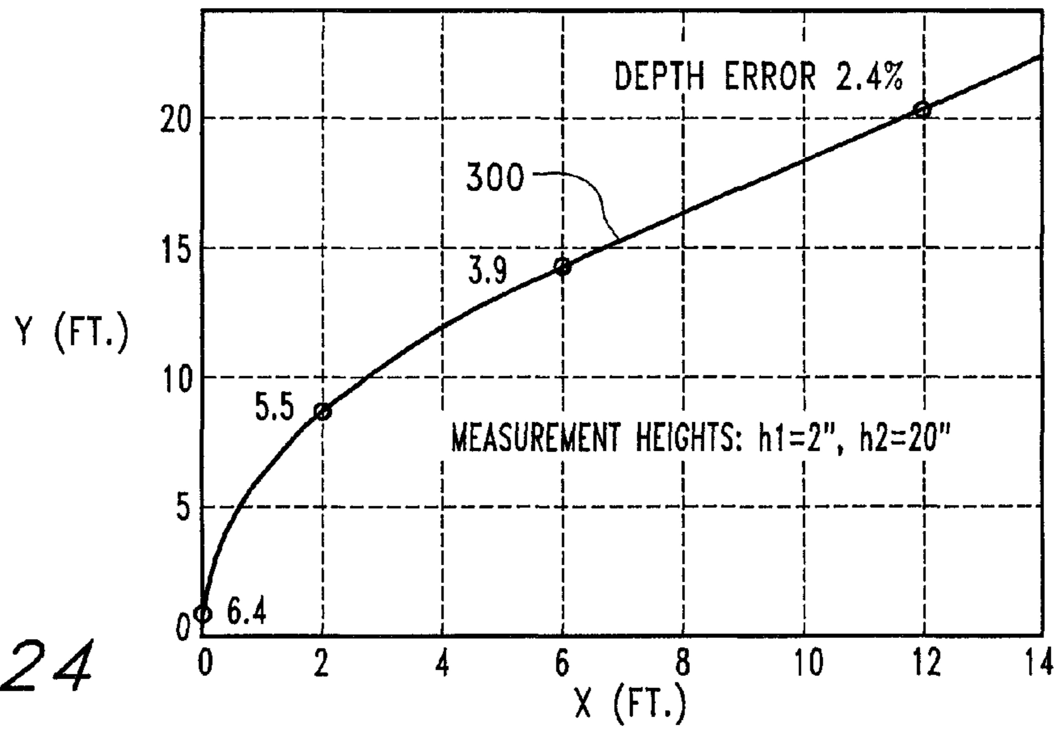
CABLE DEPTH FROM 2-POINT HEIGHT MEASUREMENTS, 5 FT. DEPTH
