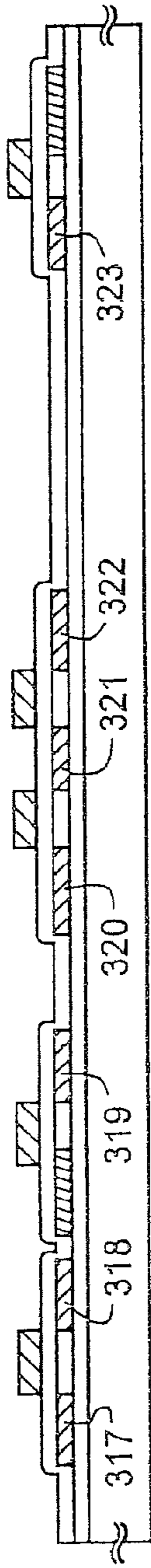
FIG. 4A STEP OF ADDING N-TYPE IMPURITY ELEMENT
