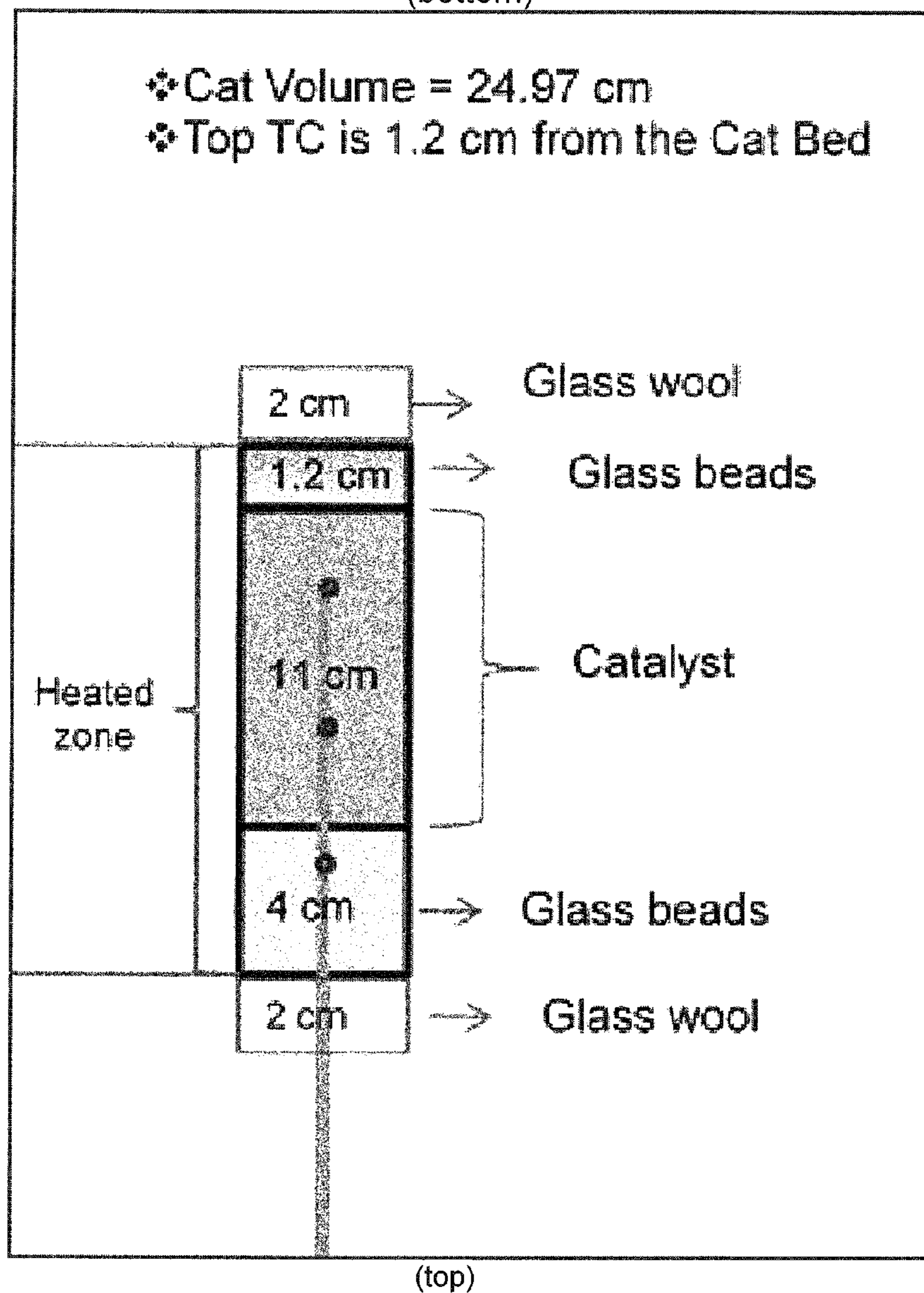
FIG 4 Laboratory Reactor Configuration (shown inverted) (bottom)
