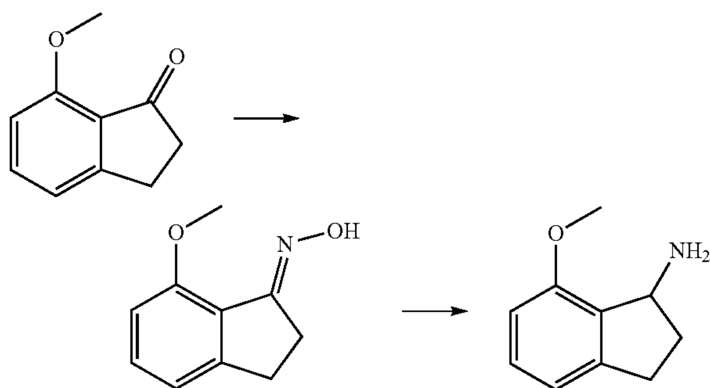
Step 1: Synthesis of 7-methoxyindan-1-one oxime
