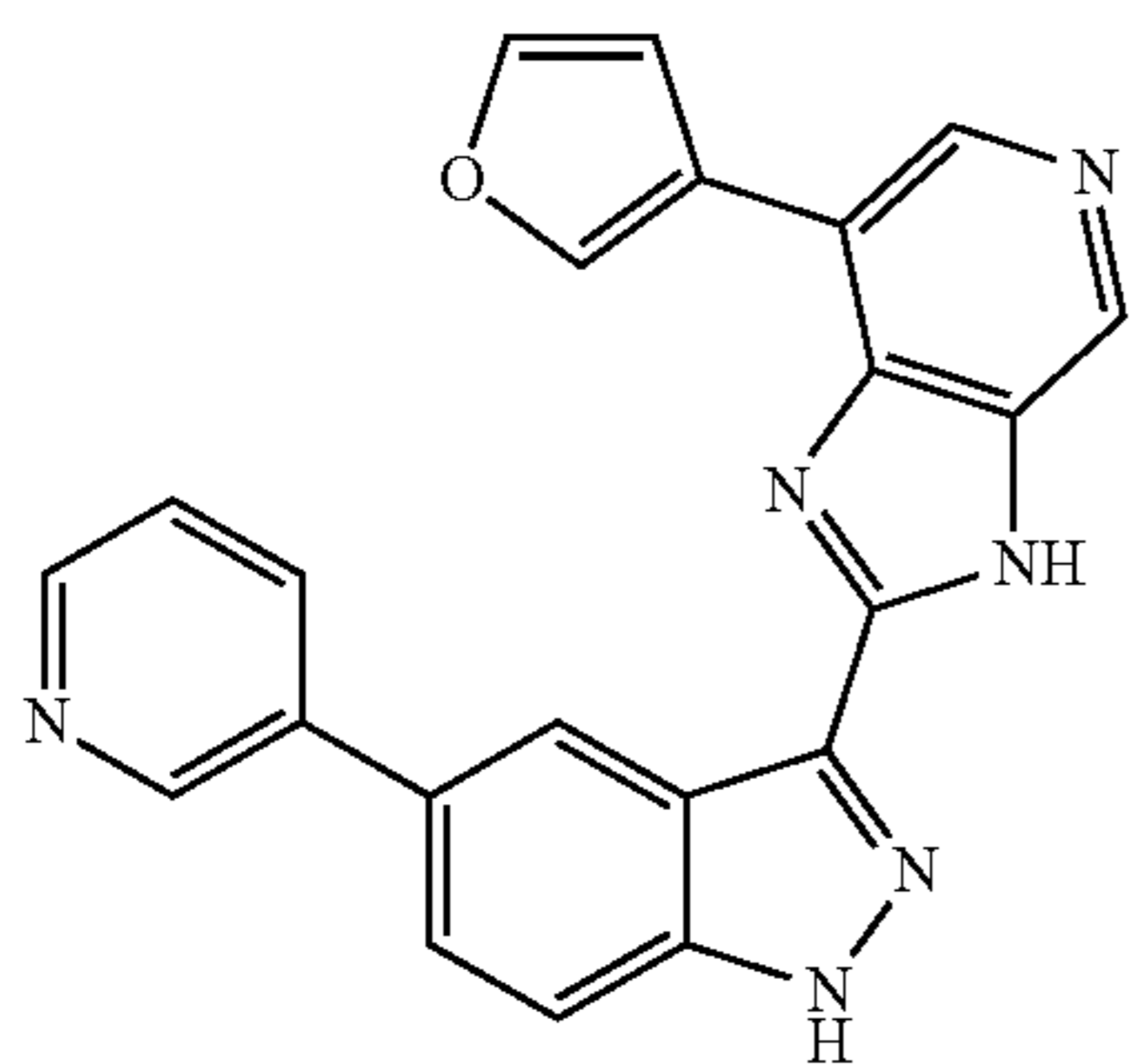
7-(Furan-3-yl)-2-(5-(pyridin-3-yl)-1H-indazol-3-yl)-3H-imidazo[4,5-c]pyridine 315
