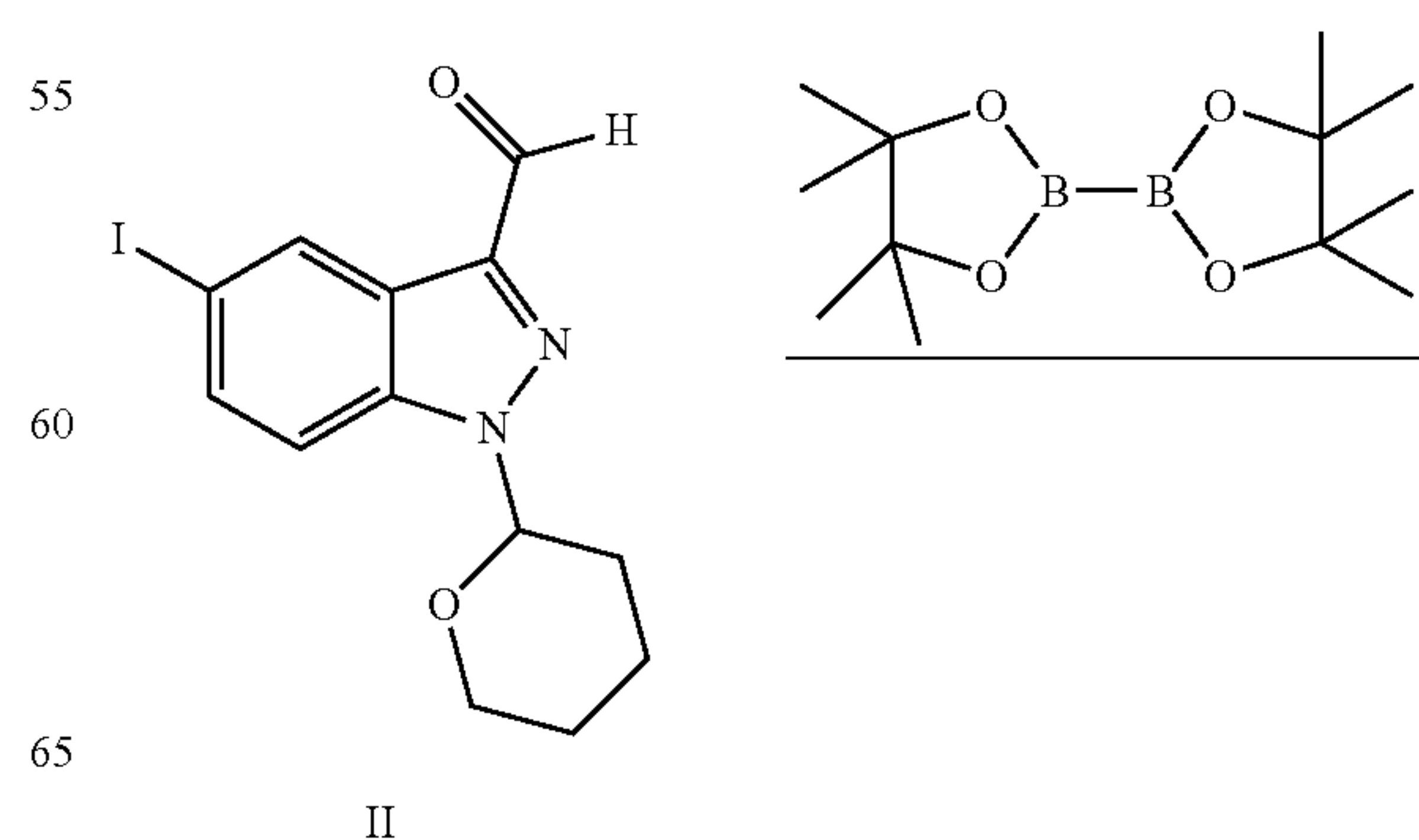
Scheme 1
