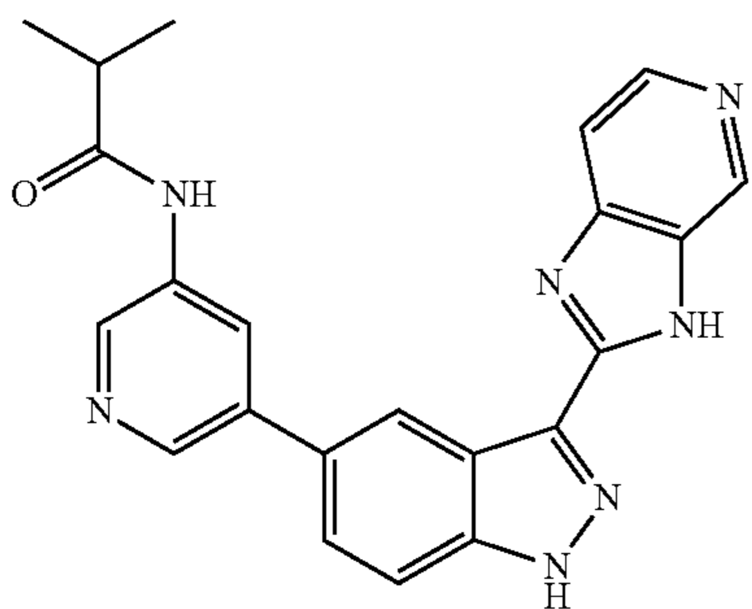
N-(5-(3-(3H-imidazo[4,5-c]pyridin-2-yl)-1H-indazol-5-yl)pyridin-3-yl)isobutyramide 9
