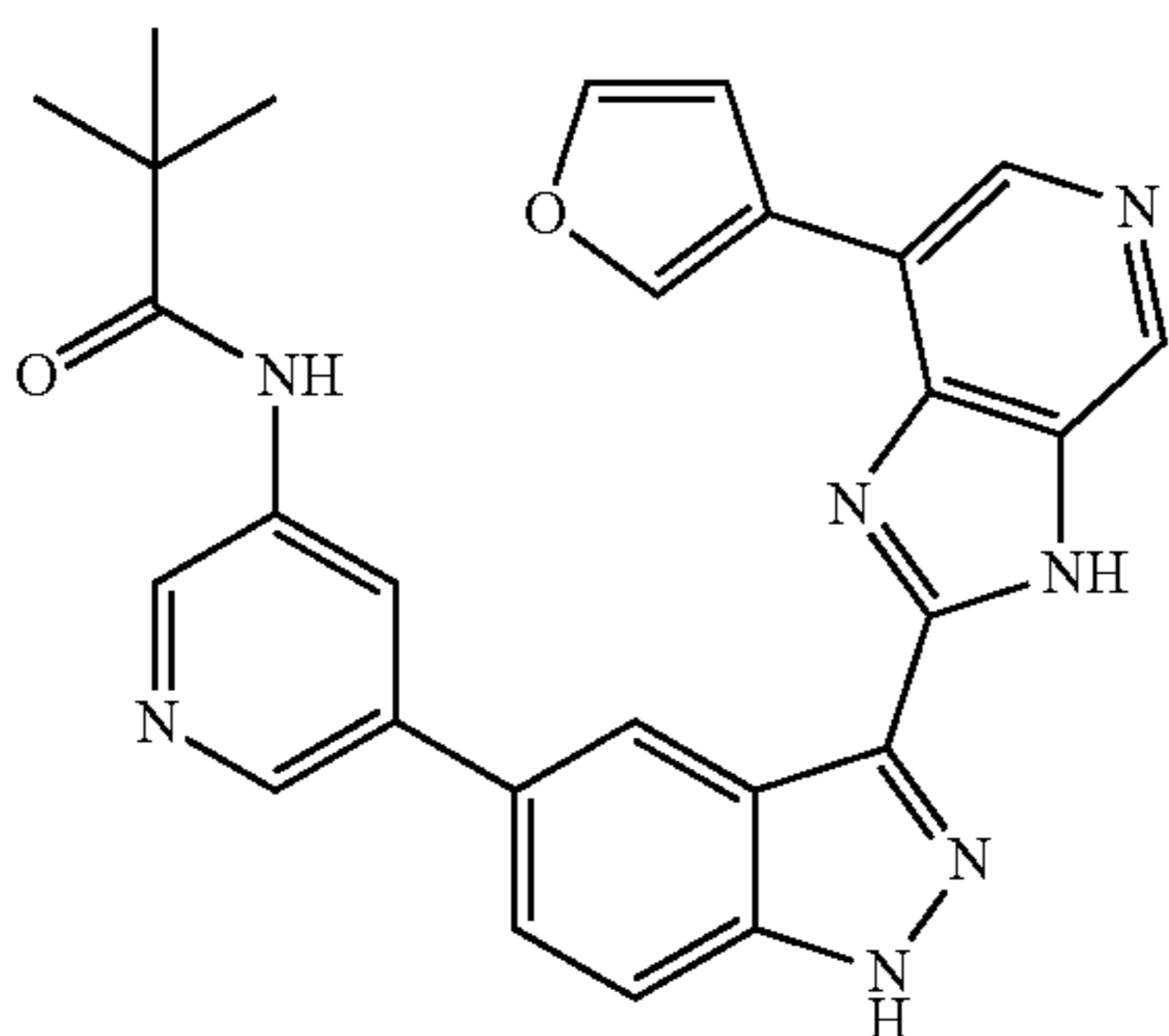
N-(5-(3-(7-(Furan-3-yl)-3H-imidazo[4,5-c]pyridin-2-yl)-1H-indazol-5-yl)pyridin-3-yl)pivalamide 319
