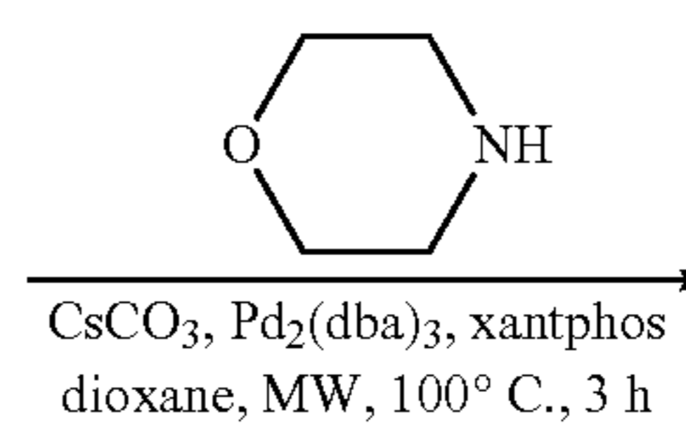
Scheme 7
