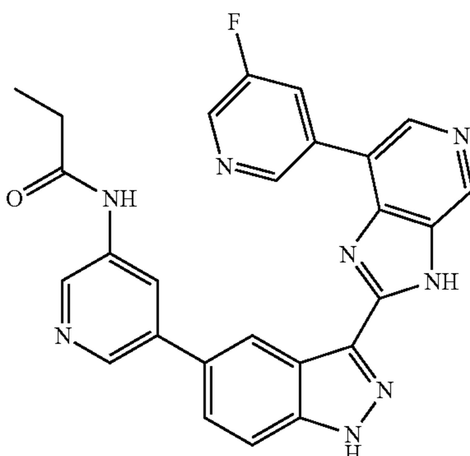
N-(5-(3-(7-(5-fluoropyridin-3-yl)-3H-imidazo[4,5-c]pyridin-2-yl)-1H-indazol-5-yl)pyridin-3-yl)propionamide 20
