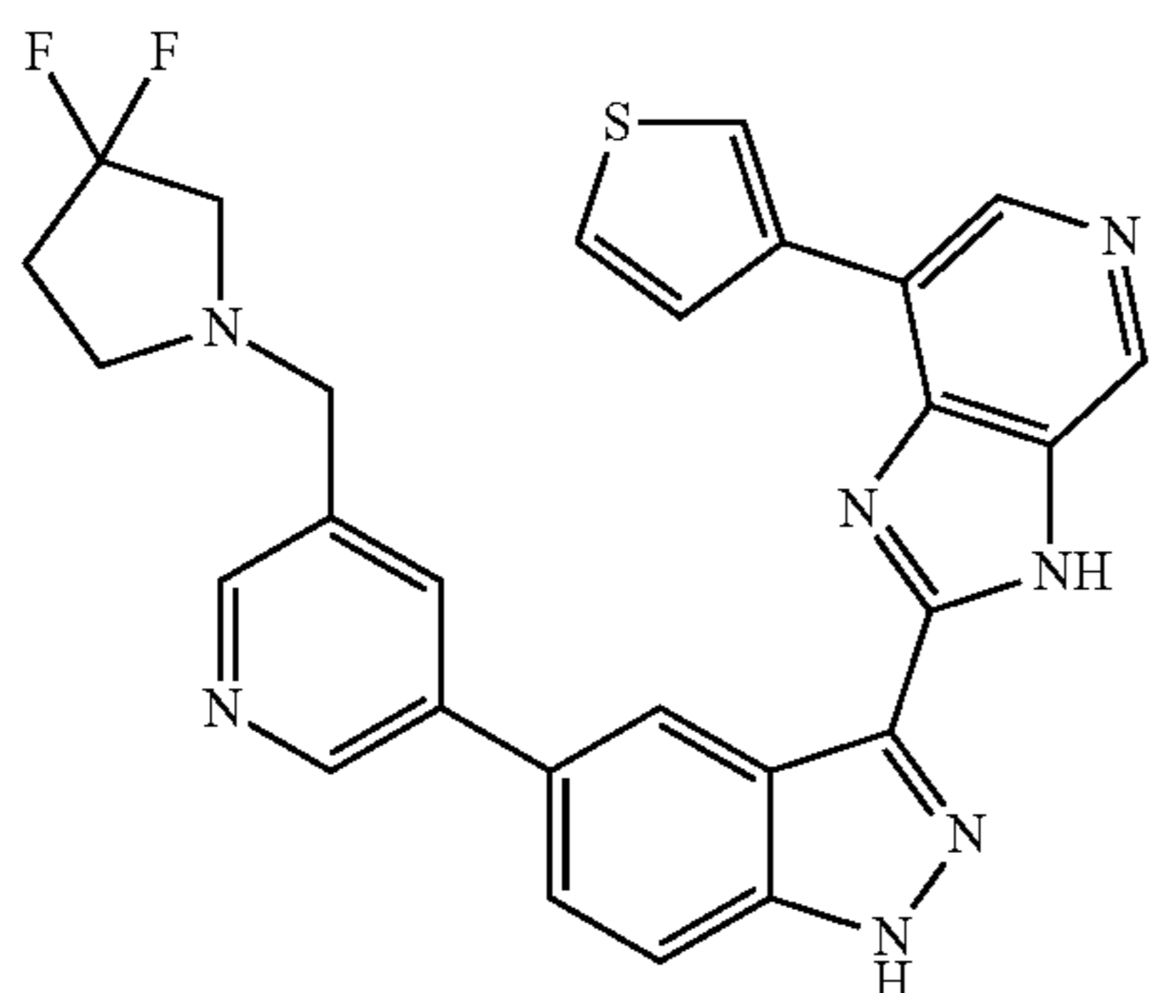
2-(5-(5-((3,3-Difluoropyrrolidin-1-yl)methyl)pyridin-3-yl)-1H-indazol-3-yl)-7-(thiophen-3-yl)-3H-imidazo[4,5-c]pyridine 346
