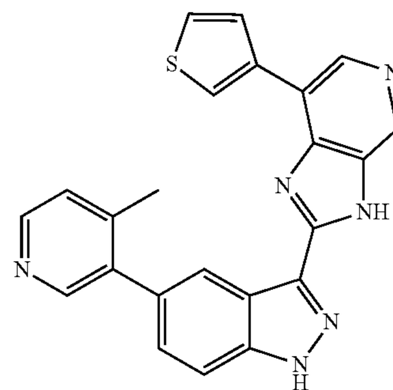
2-(5-(4-Methylpyridin-3-yl)-1H-indazol-3-yl)-7-(thiophen-3-yl)-3H-imidazo[4,5-c]pyridine 293
