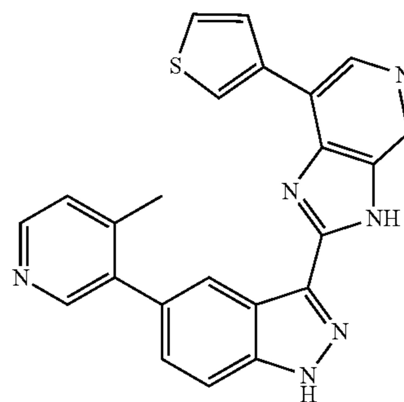
2-(5-(4-Methylpyridin-3-yl)-1H-indazol-3-yl)-7-(thiophen-3-yl)-3H-imidazo[4,5-c]pyridine 293
