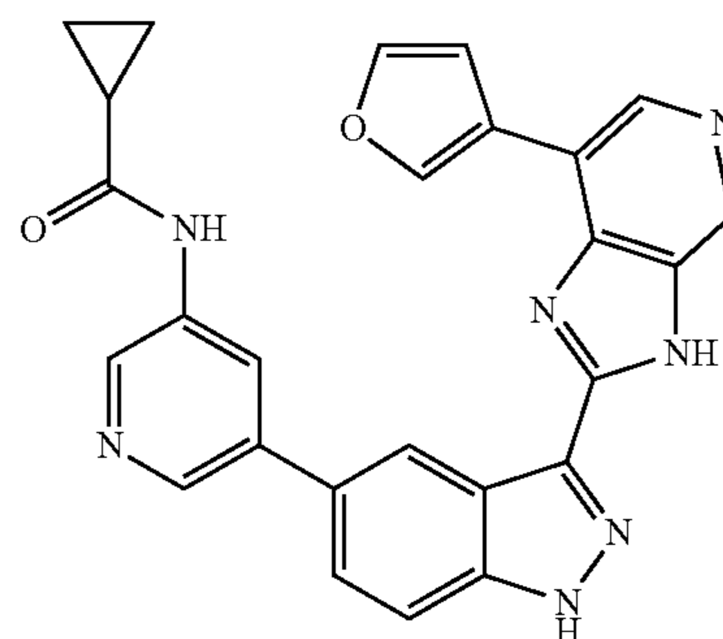
N-(5-(3-(7-(Furan-3-yl)-3H-imidazo[4,5-c]pyridin-2-yl)-1H-indazol-5-yl)pyridin-3-yl)cyclopropanecarboxamide 330
