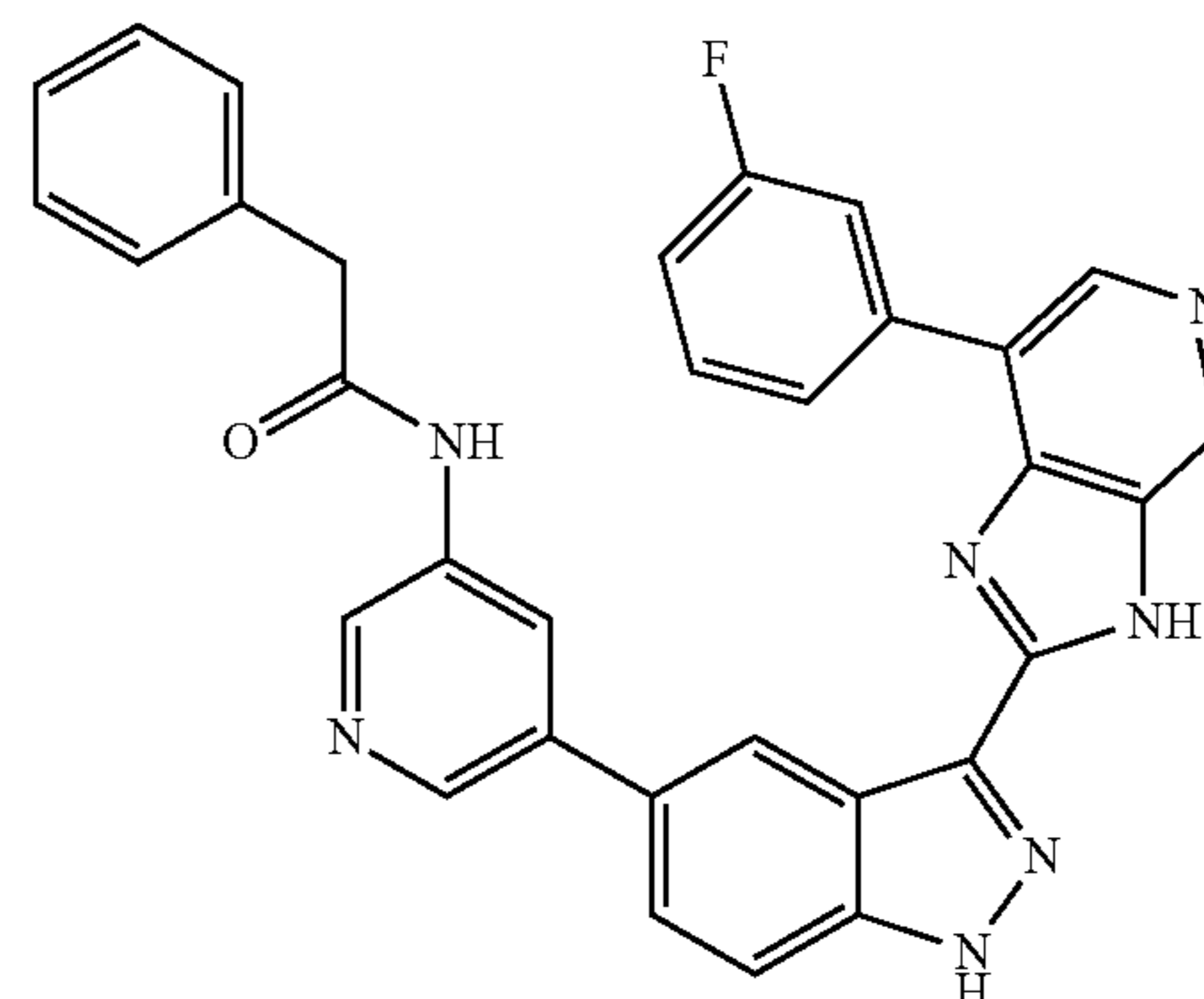
N-(5-(3-(7-(3-Fluorophenyl)-3H-imidazo[4,5-c]pyridin-2-yl)-1H-indazol-5-yl)pyridin-3-yl)-2-phenylacetamide 86
