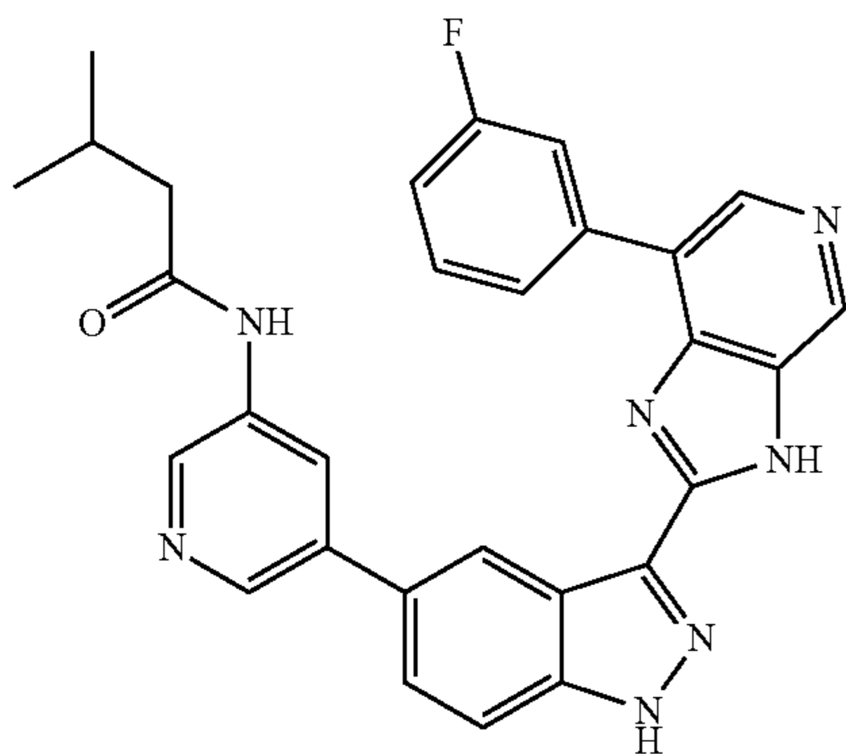
N-(5-(3-(7-(3-fluorophenyl)-3H-imidazo[4,5-c]pyridin-2-yl)-1H-indazol-5-yl)pyridin-3-yl)-3-methylbutanamide 10
