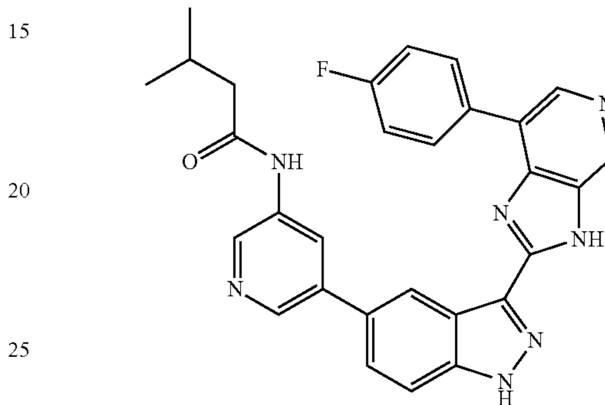
N-(5-(3-(3H-imidazo[4,5-c]pyridin-2-yl)-1H-indazol-5-yl)pyridin-3-yl)isobutyramide 9
