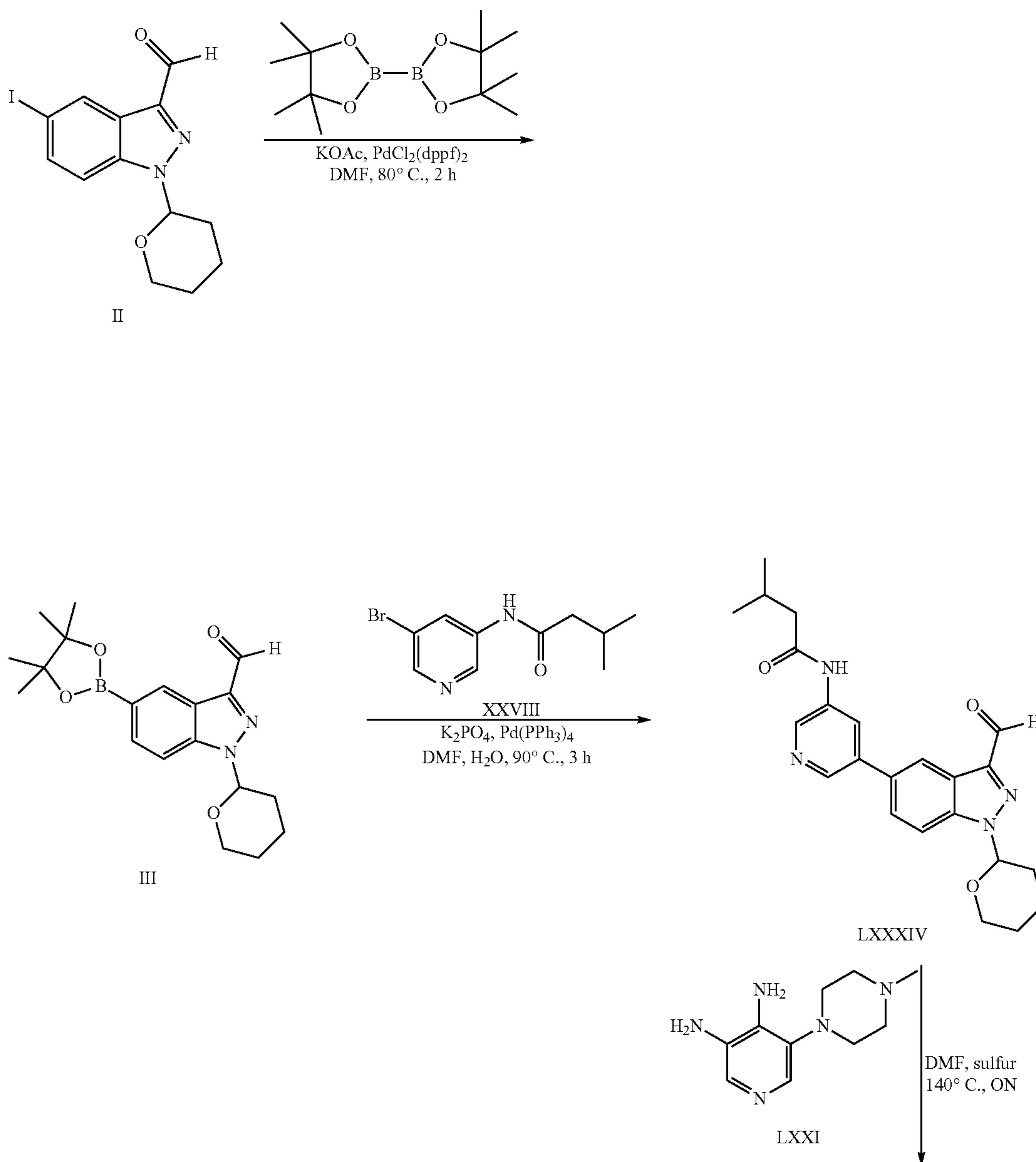
Scheme 16
