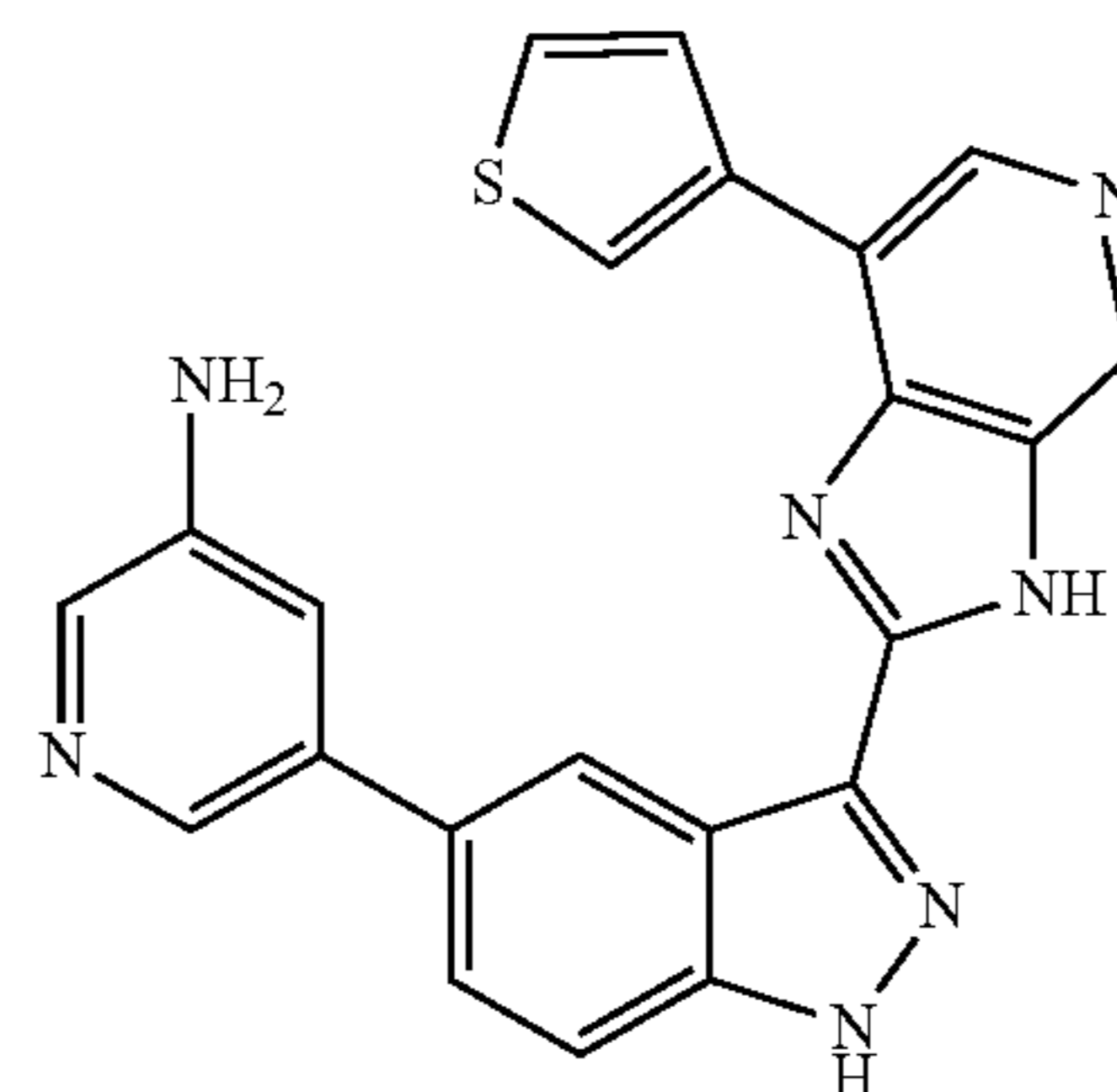
5-(3-(7-(Thiophen-3-yl)-3H-imidazo[4,5-c]pyridin-2-yl)-1H-indazol-5-yl)pyridin-3-amine 291
