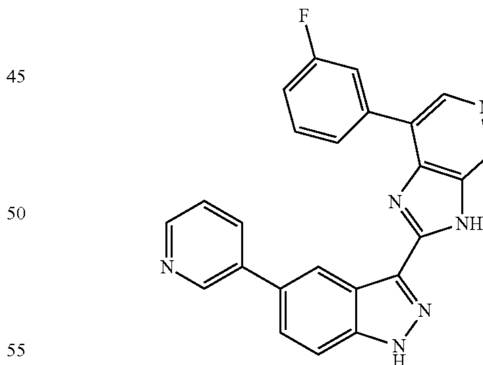
N-(5-(3-(7-(3-fluorophenyl)-3H-imidazo[4,5-c]pyridin-2-yl)-1H-indazol-5-yl)pyridin-3-yl)-3-methylbutanamide 10
