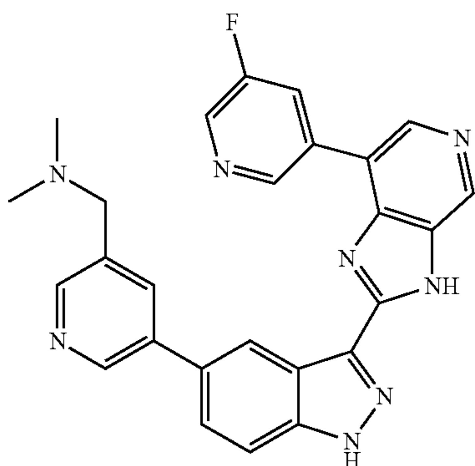
1-(5-(3-(7-(5-fluoropyridin-3-yl)-3H-imidazo[4,5-c]pyridin-2-yl)-1H-indazol-5-yl)pyridin-3-yl)-N,N-dimethylmethanamine 16
