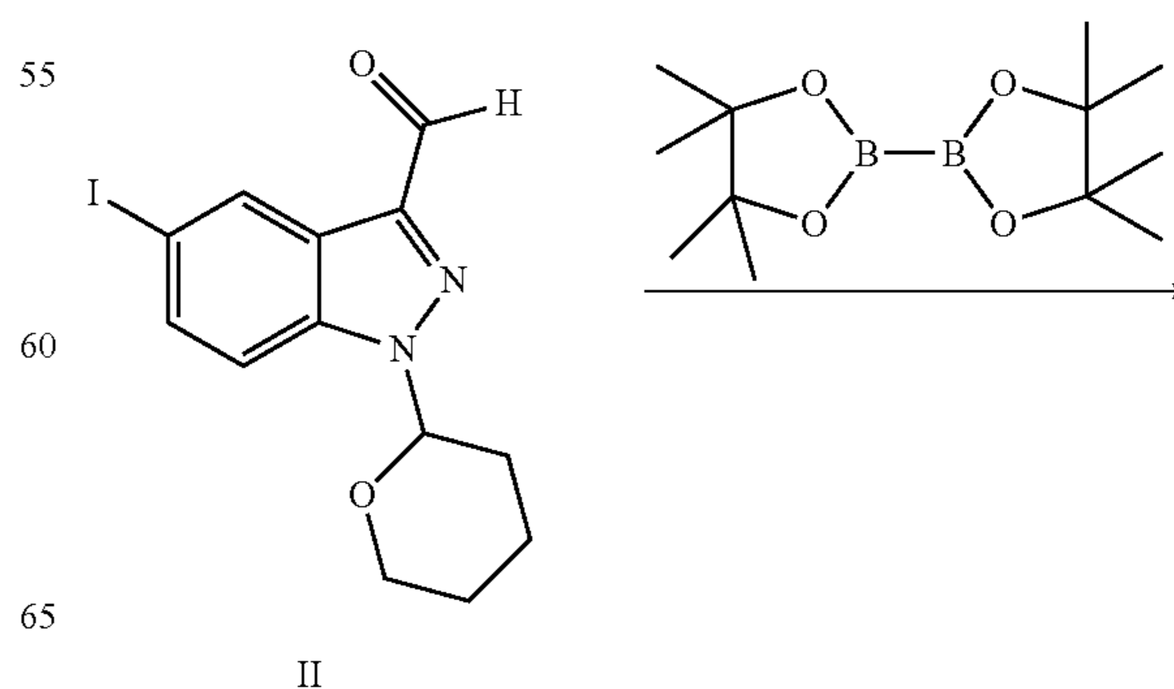
Scheme 1
