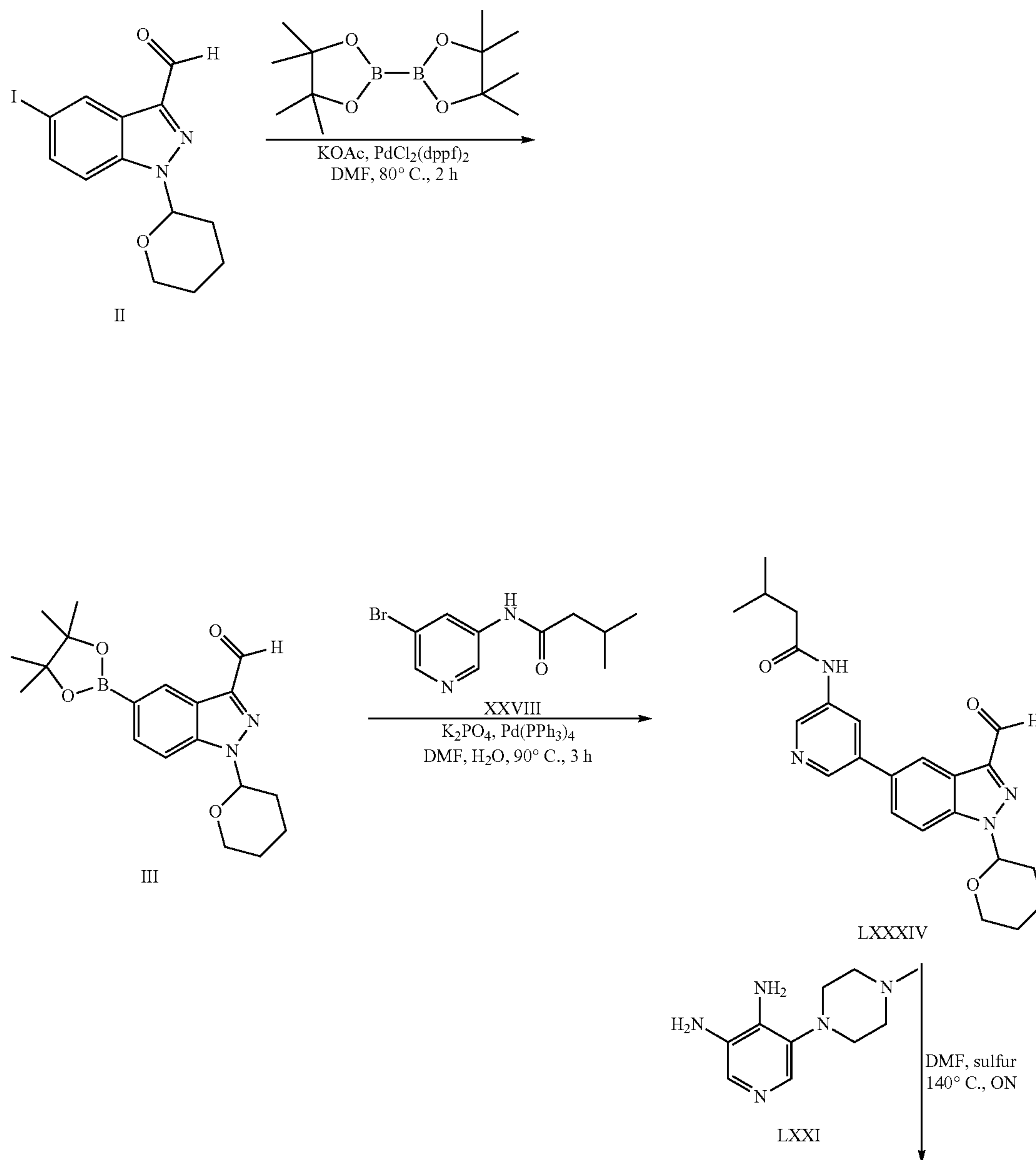
Scheme 16
