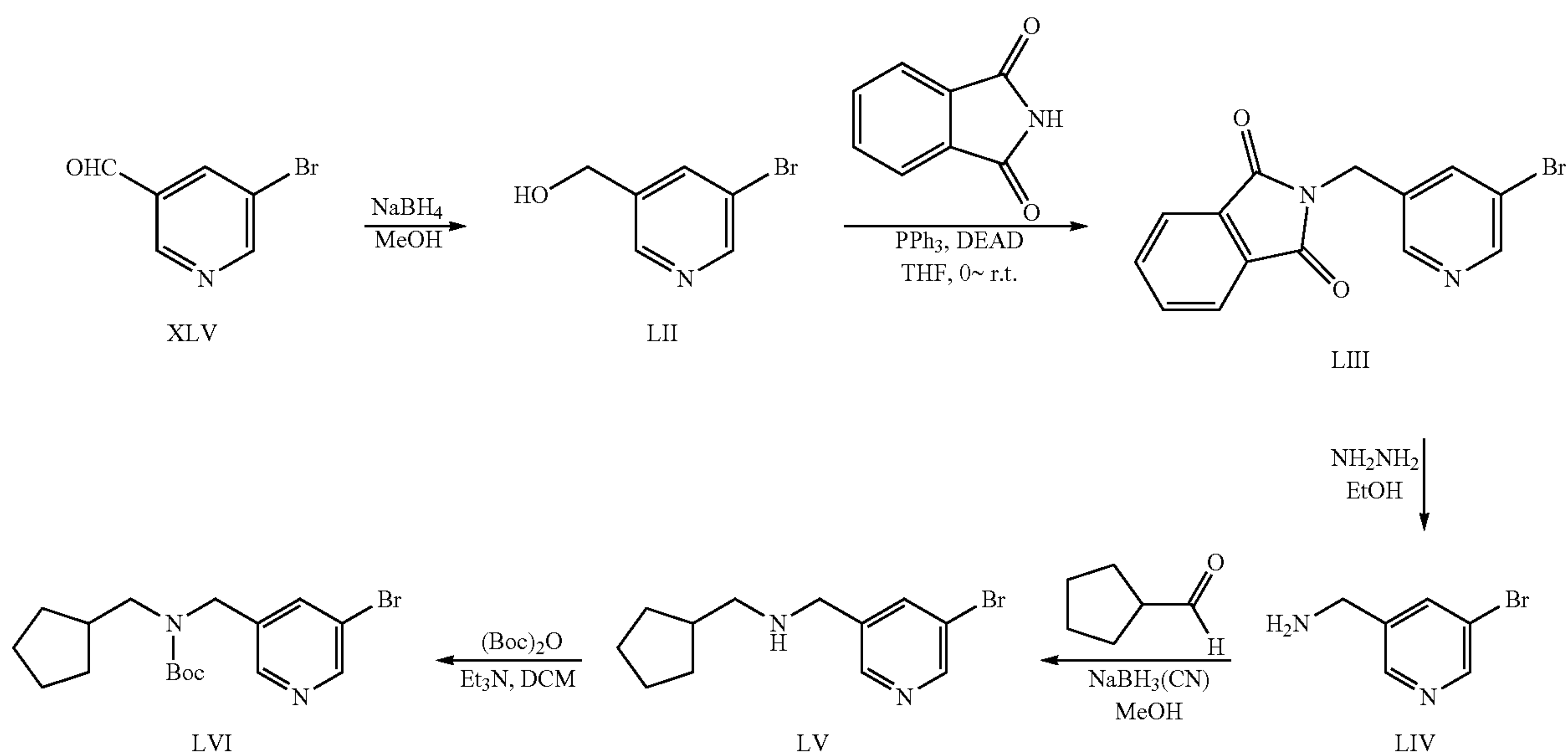
Scheme 11
