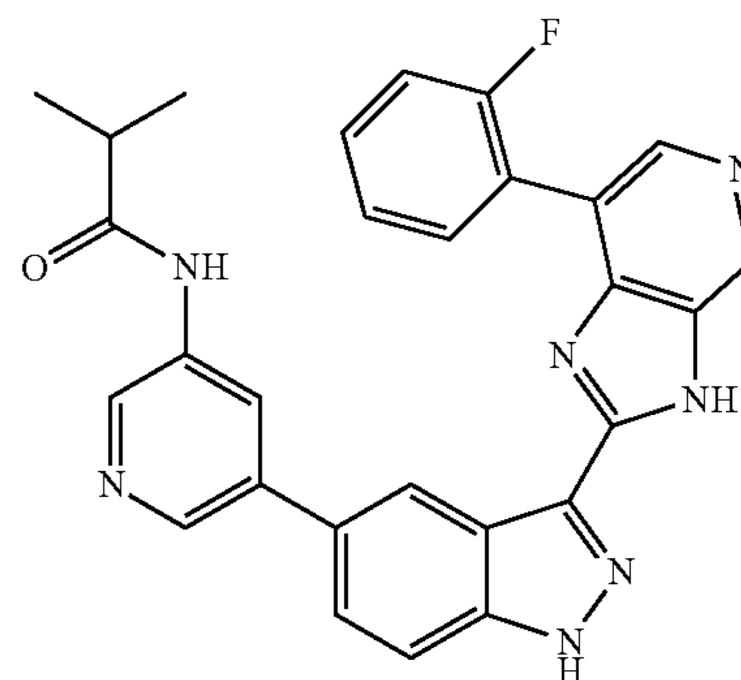
N-(5-(3-(7-(2-Fluorophenyl)-3H-imidazo[4,5-c]pyridin-2-yl)-1H-indazol-5-yl)pyridin-3-yl)isobutyramide 31
