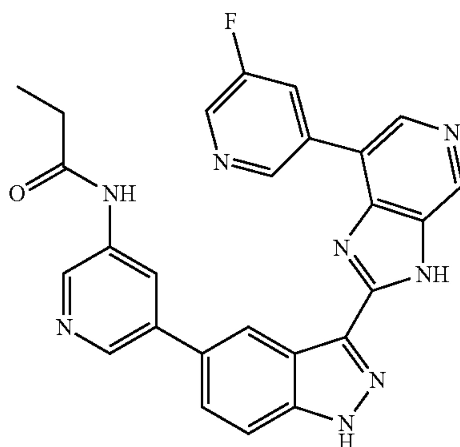
N-(5-(3-(7-(5-fluoropyridin-3-yl)-3H-imidazo[4,5-c]pyridin-2-yl)-1H-indazol-5-yl)pyridin-3-yl)propionamide 20
