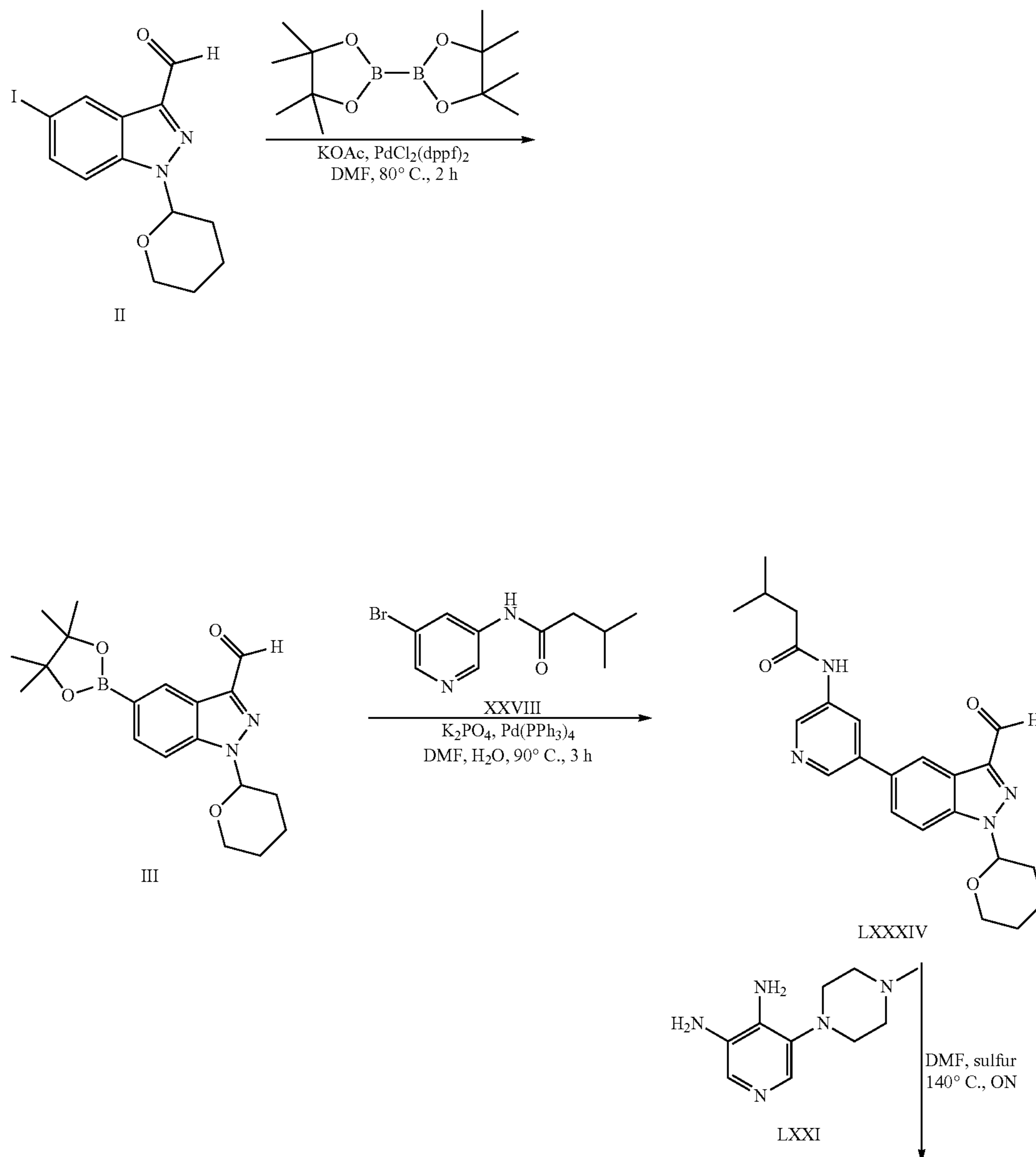
Scheme 16
