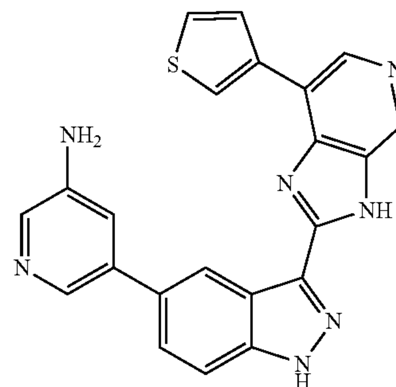
5-(3-(7-(Thiophen-3-yl)-3H-imidazo[4,5-c]pyridin-2-yl)-1H-indazol-5-yl)pyridin-3-amine 291
