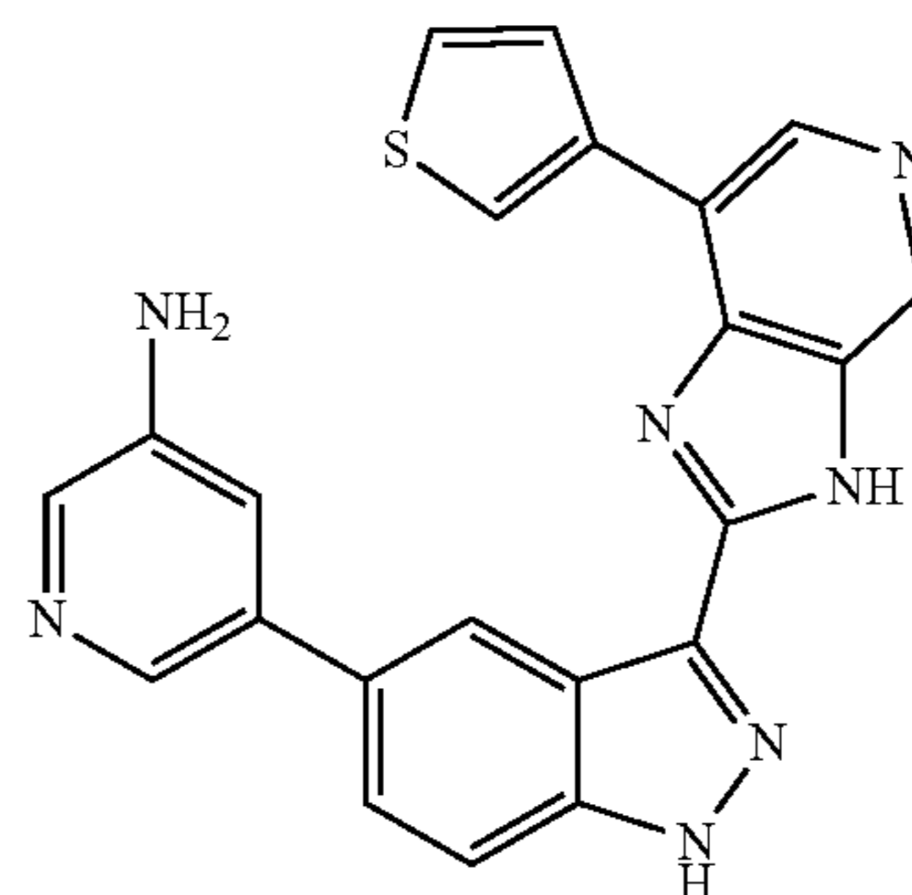
5-(3-(7-(Thiophen-3-yl)-3H-imidazo[4,5-c]pyridin-2-yl)-1H-indazol-5-yl)pyridin-3-amine 291
