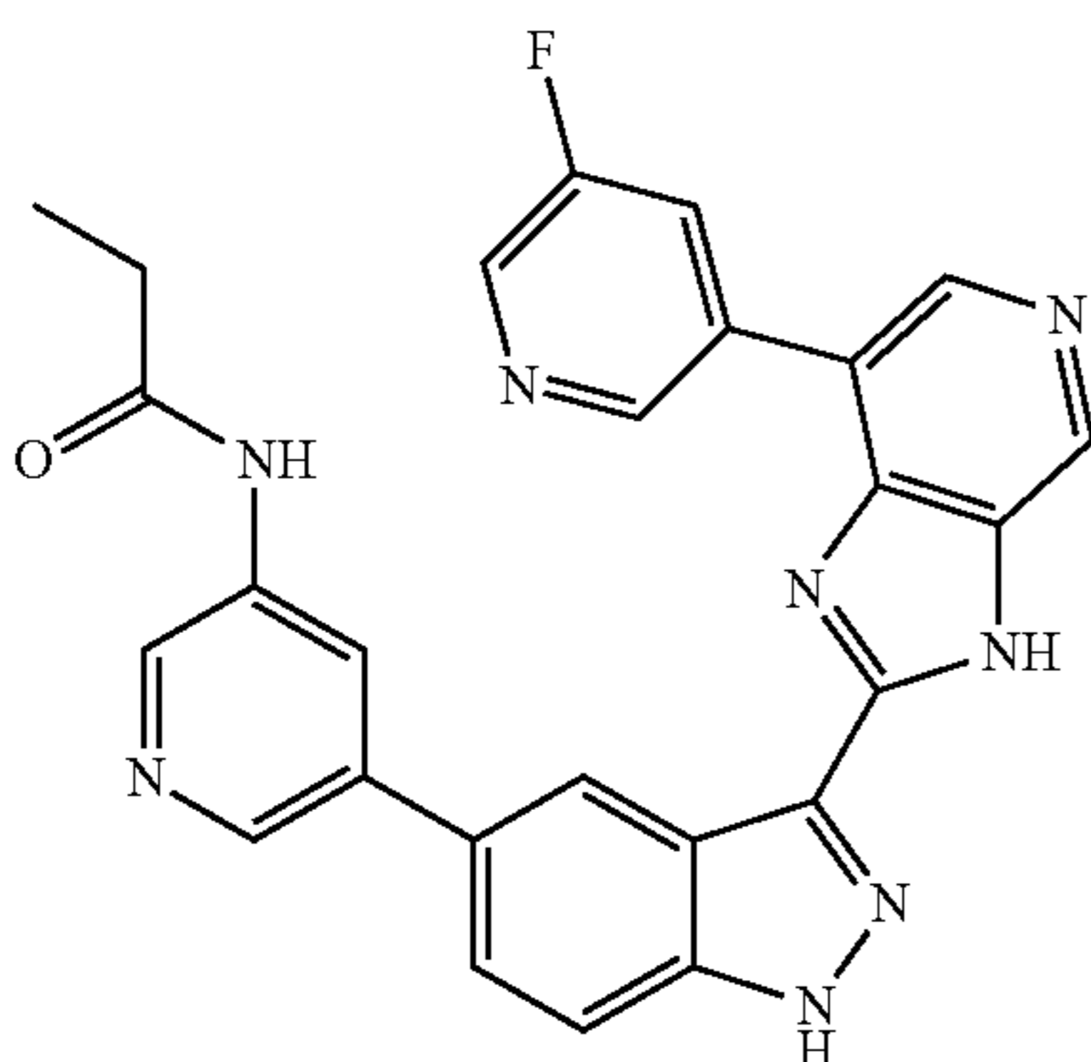
N-(5-(3-(7-(5-fluoropyridin-3-yl)-3H-imidazo[4,5-c]pyridin-2-yl)-1H-indazol-5-yl)pyridin-3-yl)propionamide 20
