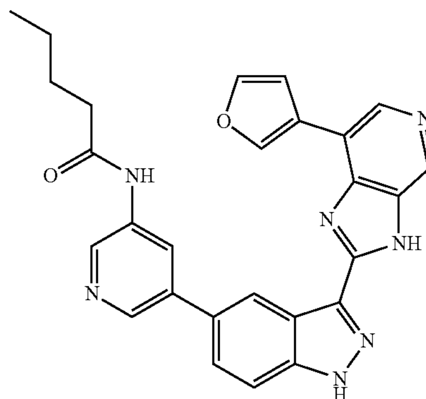
N-(5-(3-(7-(Furan-3-yl)-3H-imidazo[4,5-c]pyridin-2-yl)-1H-indazol-5-yl)pyridin-3-yl)pentanamide 329
