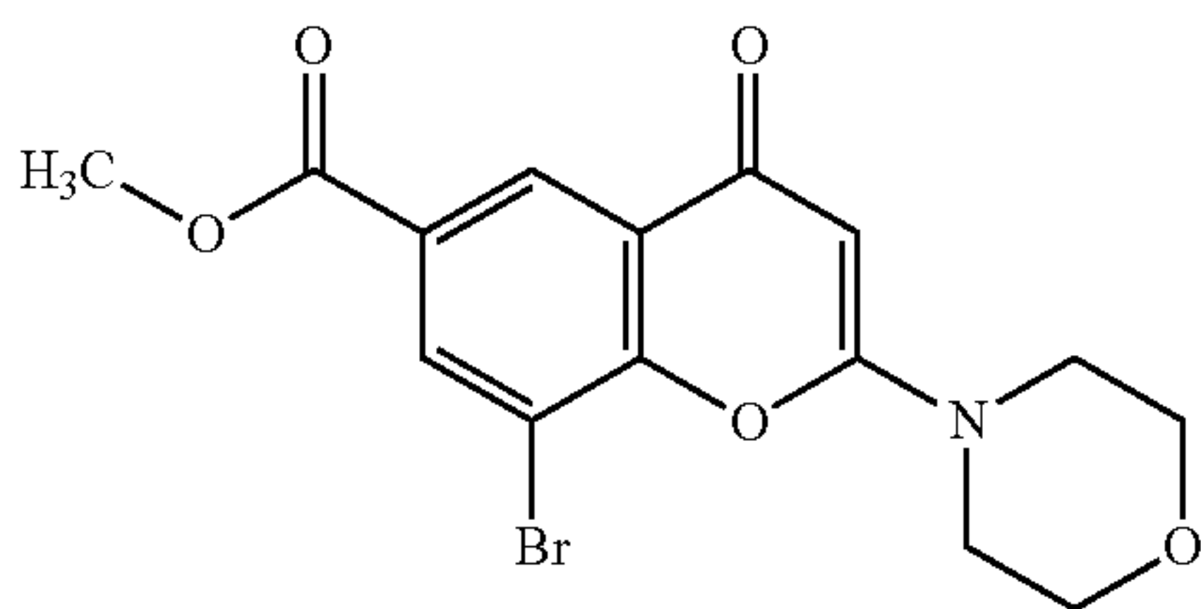
methyl 8-bromo-2-morpholin-4-yl-4-oxo-4H-chromene-6-carboxylate
