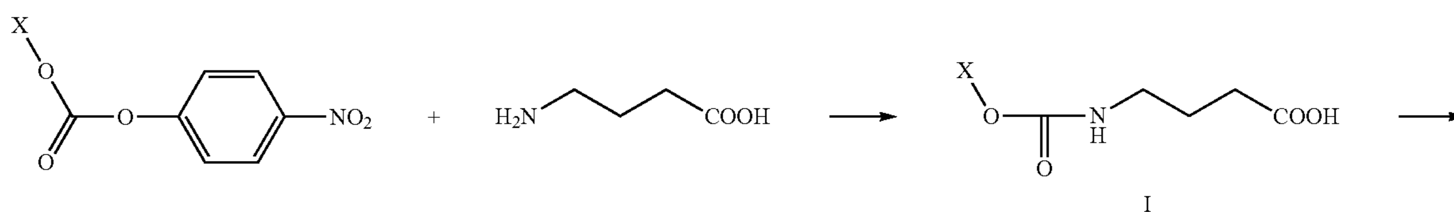
Reaction scheme 1
