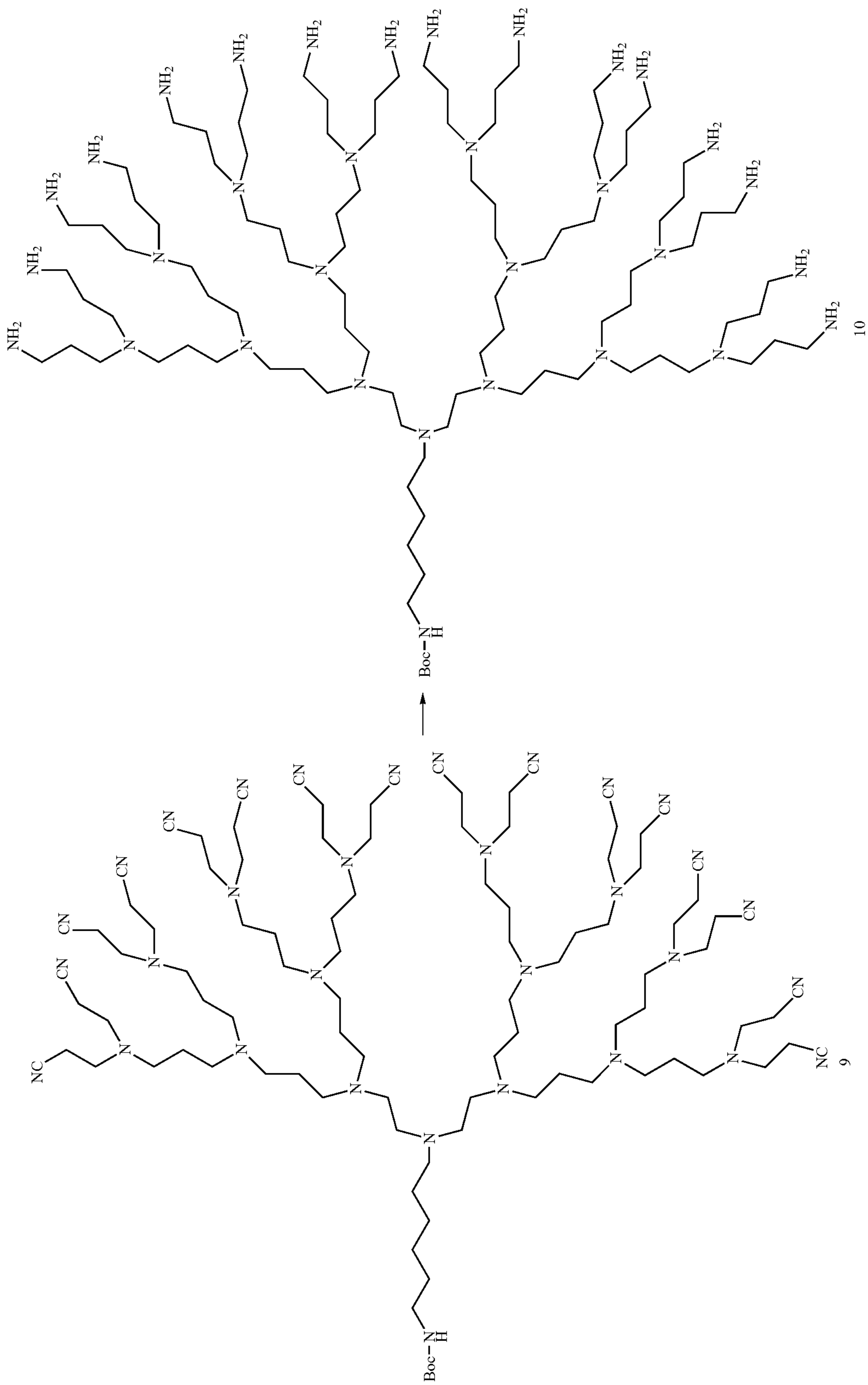
7. Boc-[16]-NH 2 (10)
