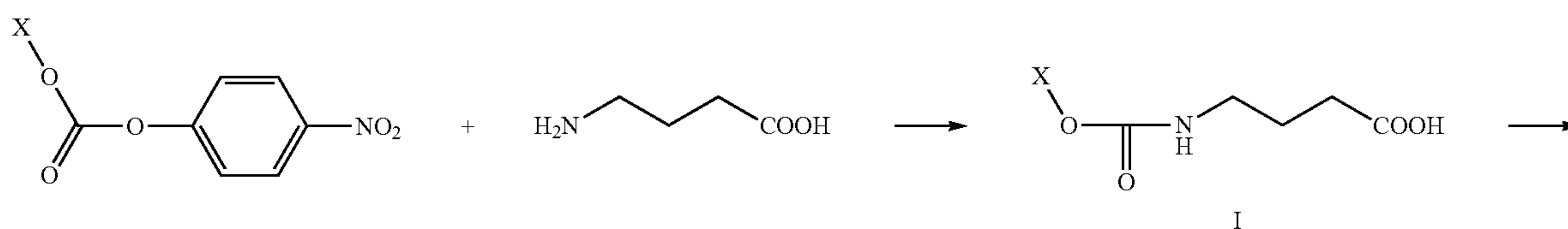
Reaction scheme 1
