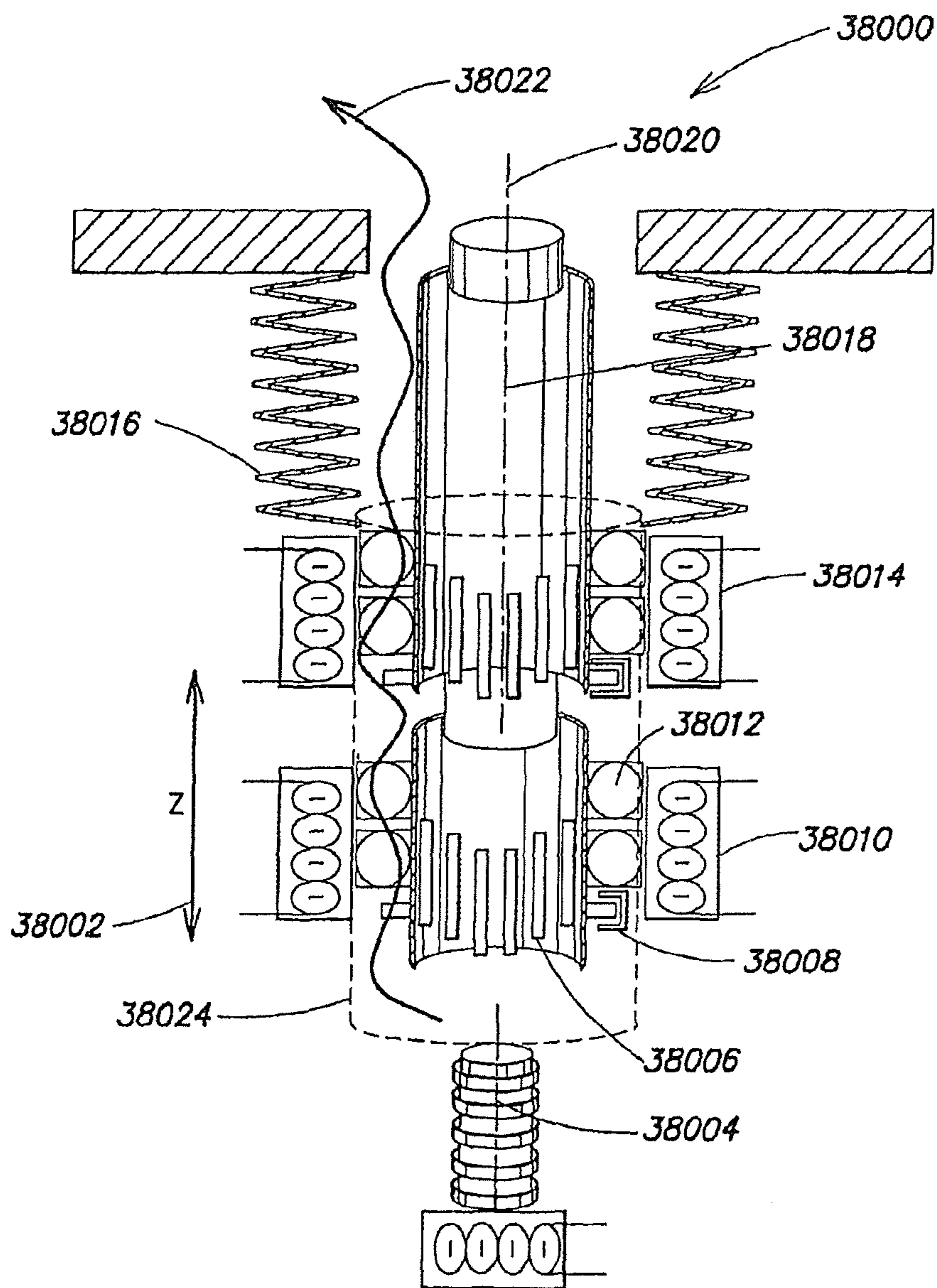
FIG. 38 (PRIOR ART)
