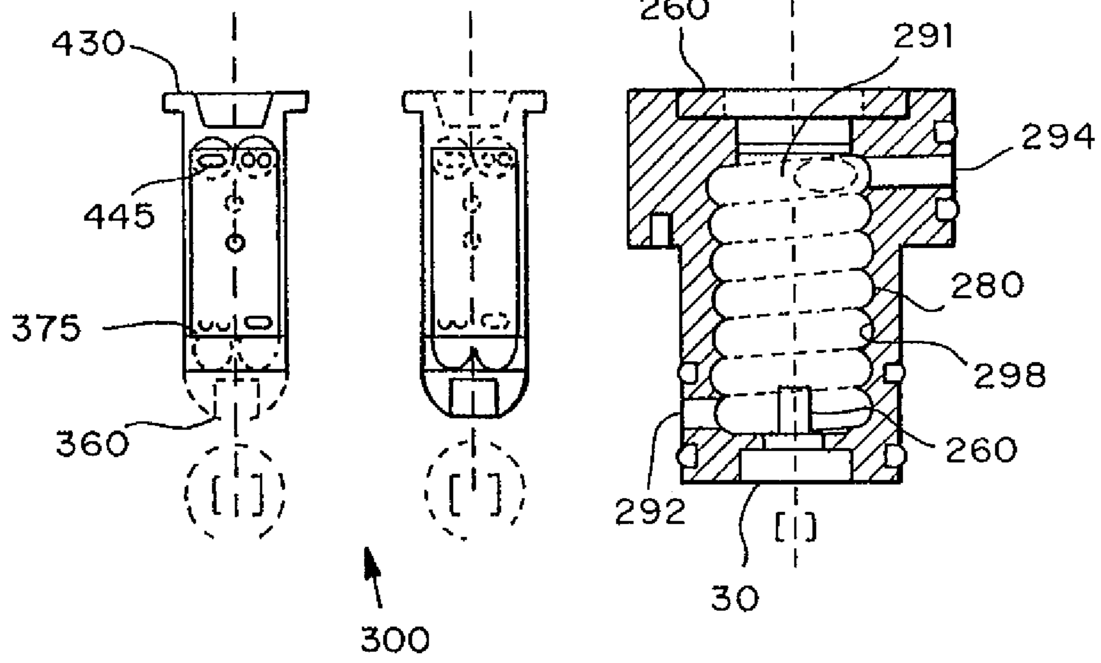
FIG. 18 PARTICLE ENTRAINMENT TURBOCELL MODULE
