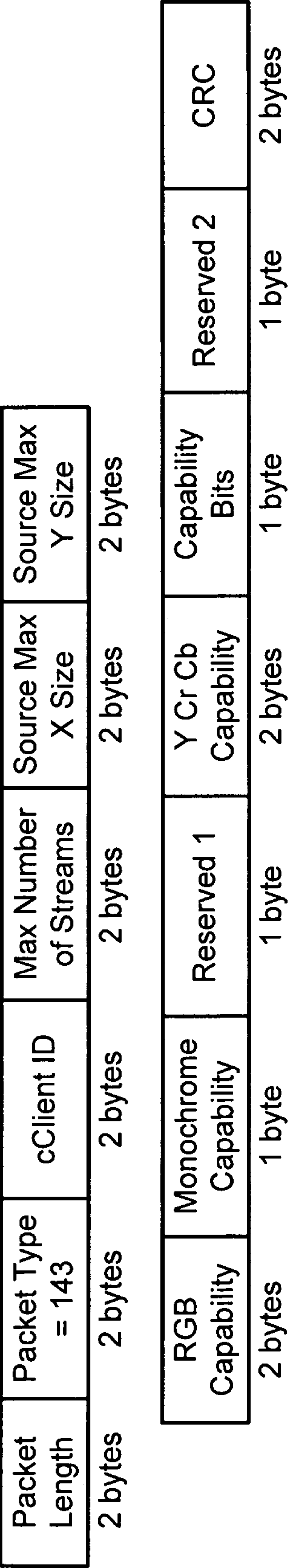
Scaled Video Stream Capability Packet
