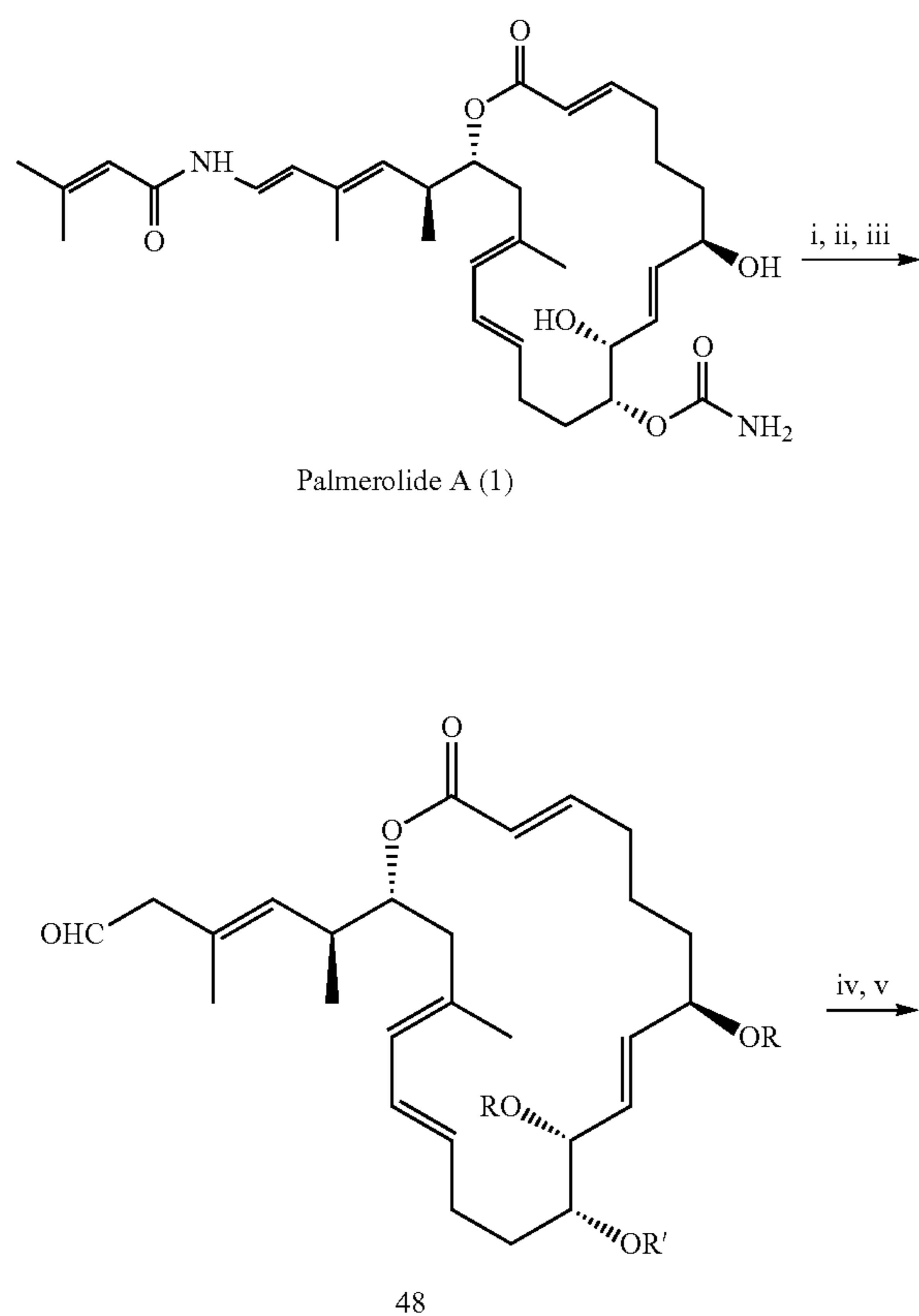
Scheme 10.
