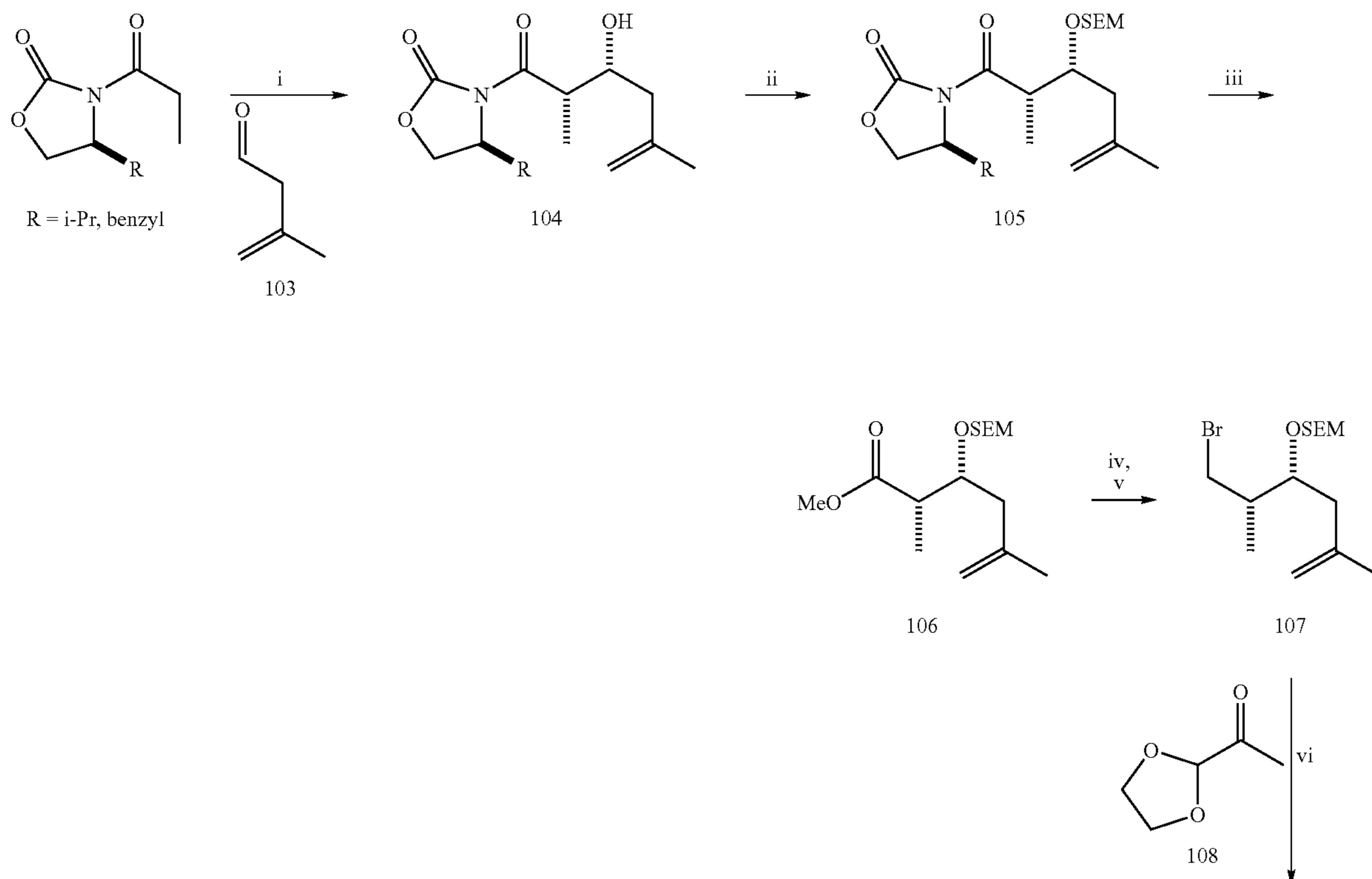
Scheme 15.
