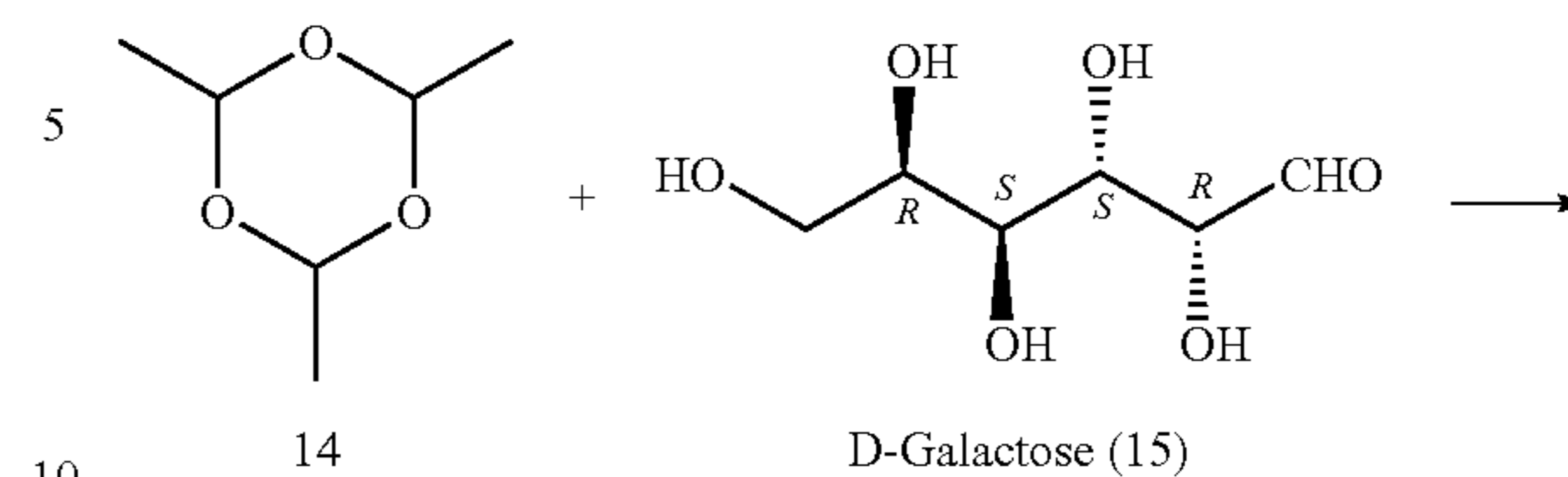
Scheme 2: Synthetic procedures for preparation of (2R,3R)-1,2,3,6-tetrahydroxyhexane (12)
