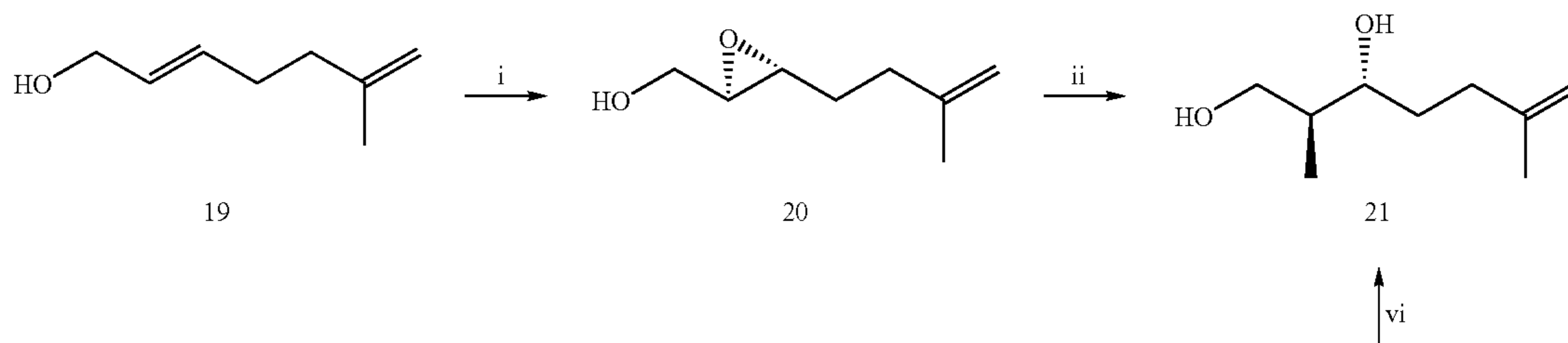
Scheme 3.
