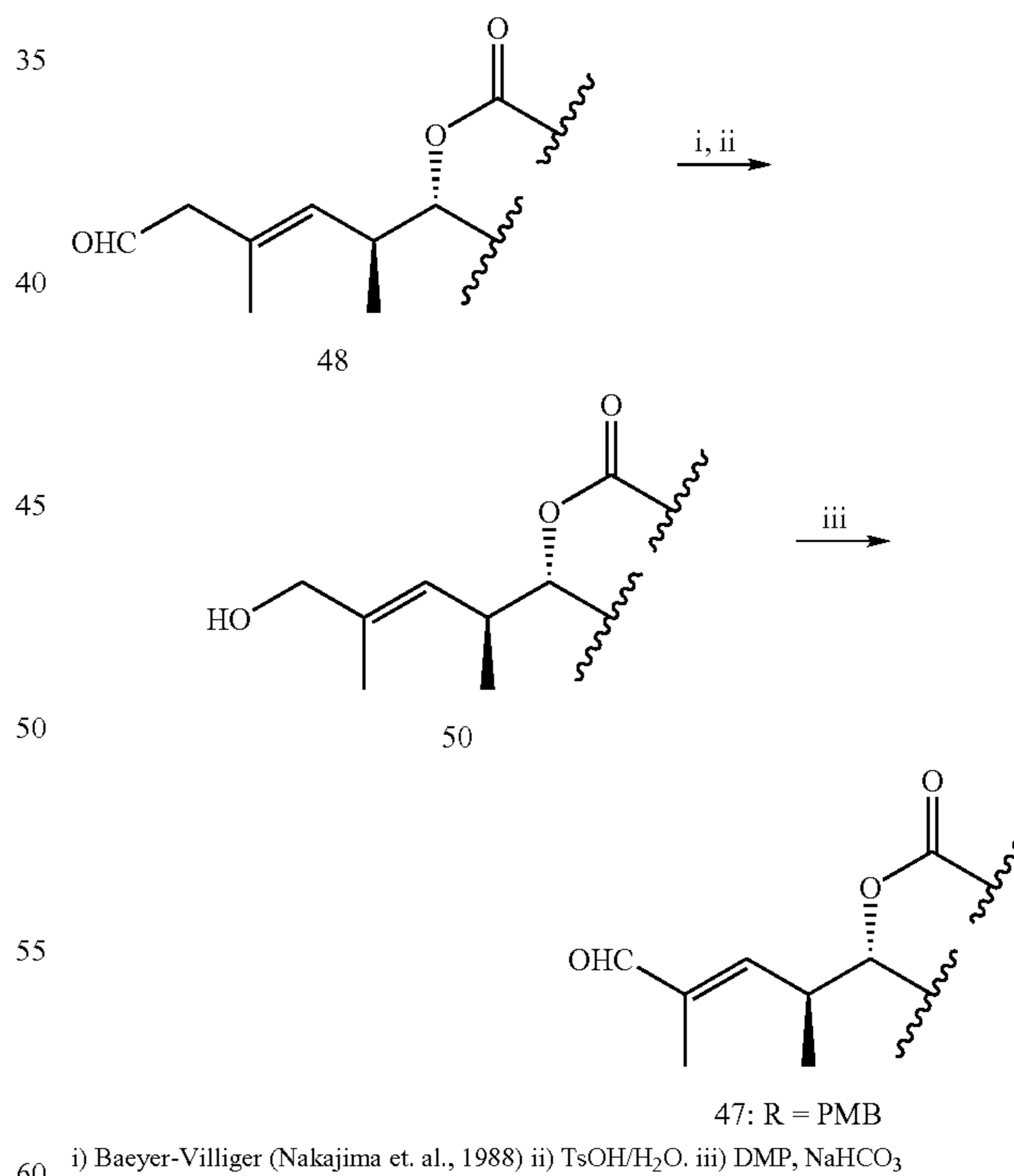
Scheme 11.
