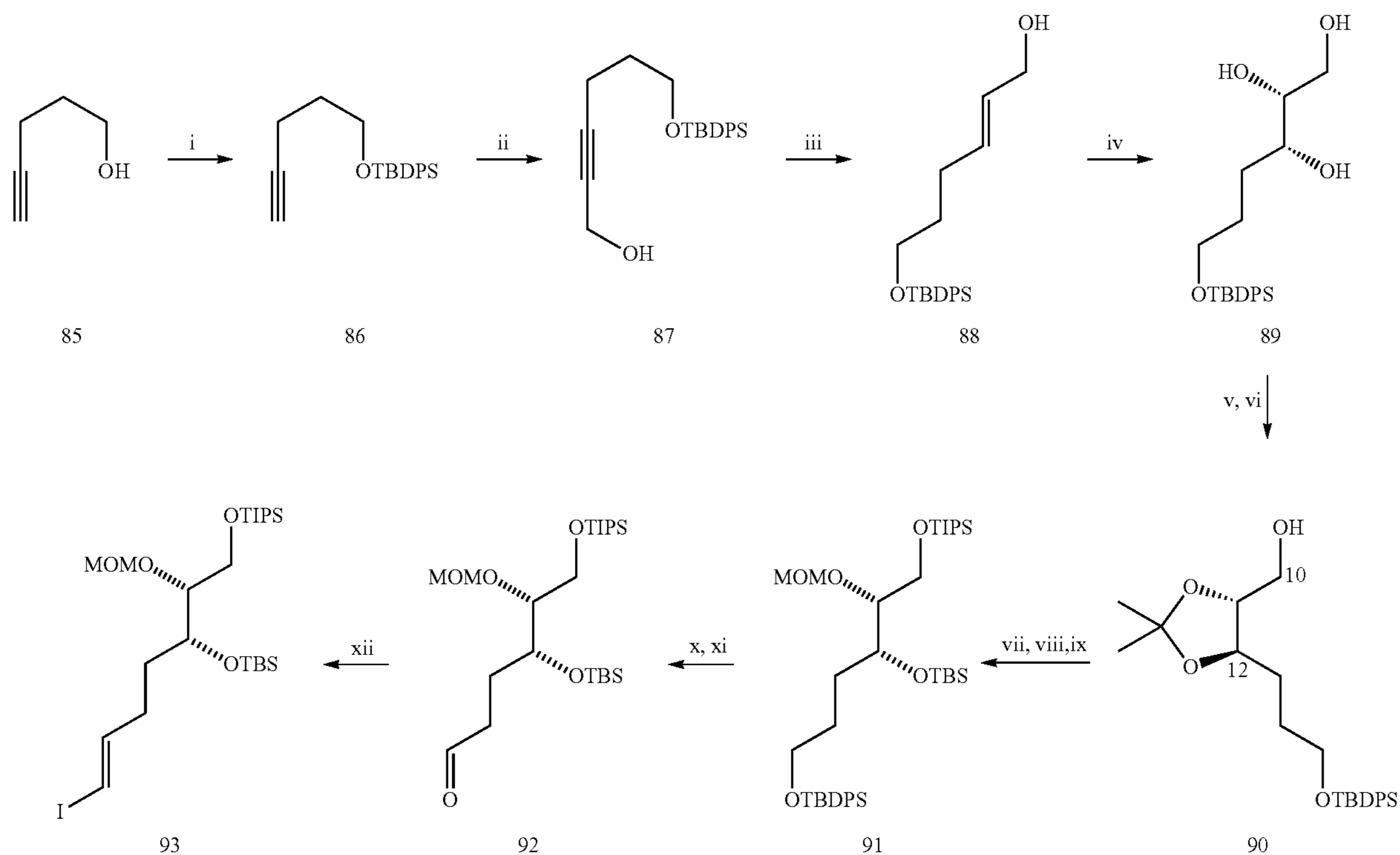
Scheme 13.
