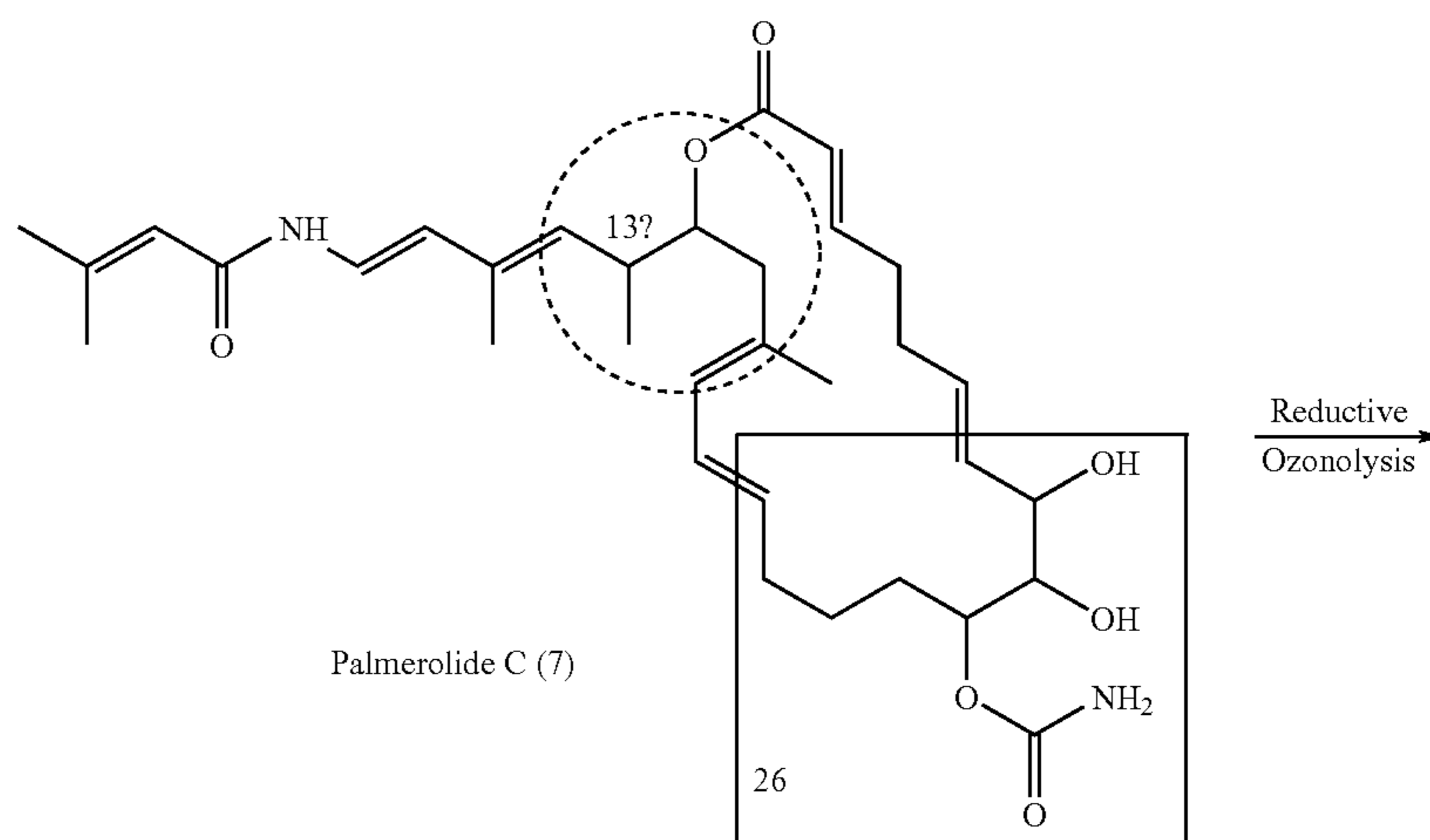
Scheme 5. Ozonolysis of palmerolide C (7).
