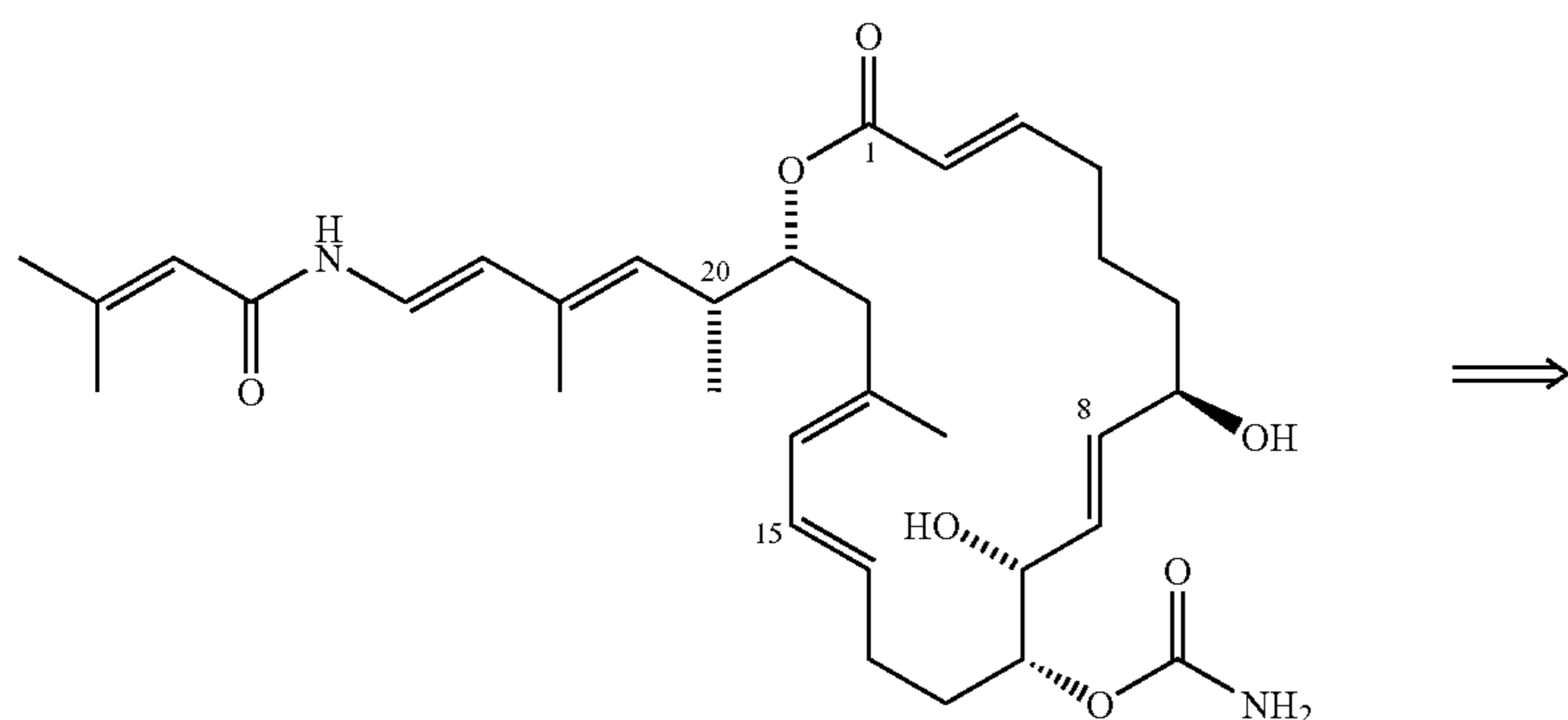
Scheme 12. Retrosynthetic analysis of palmerolide A (1)
