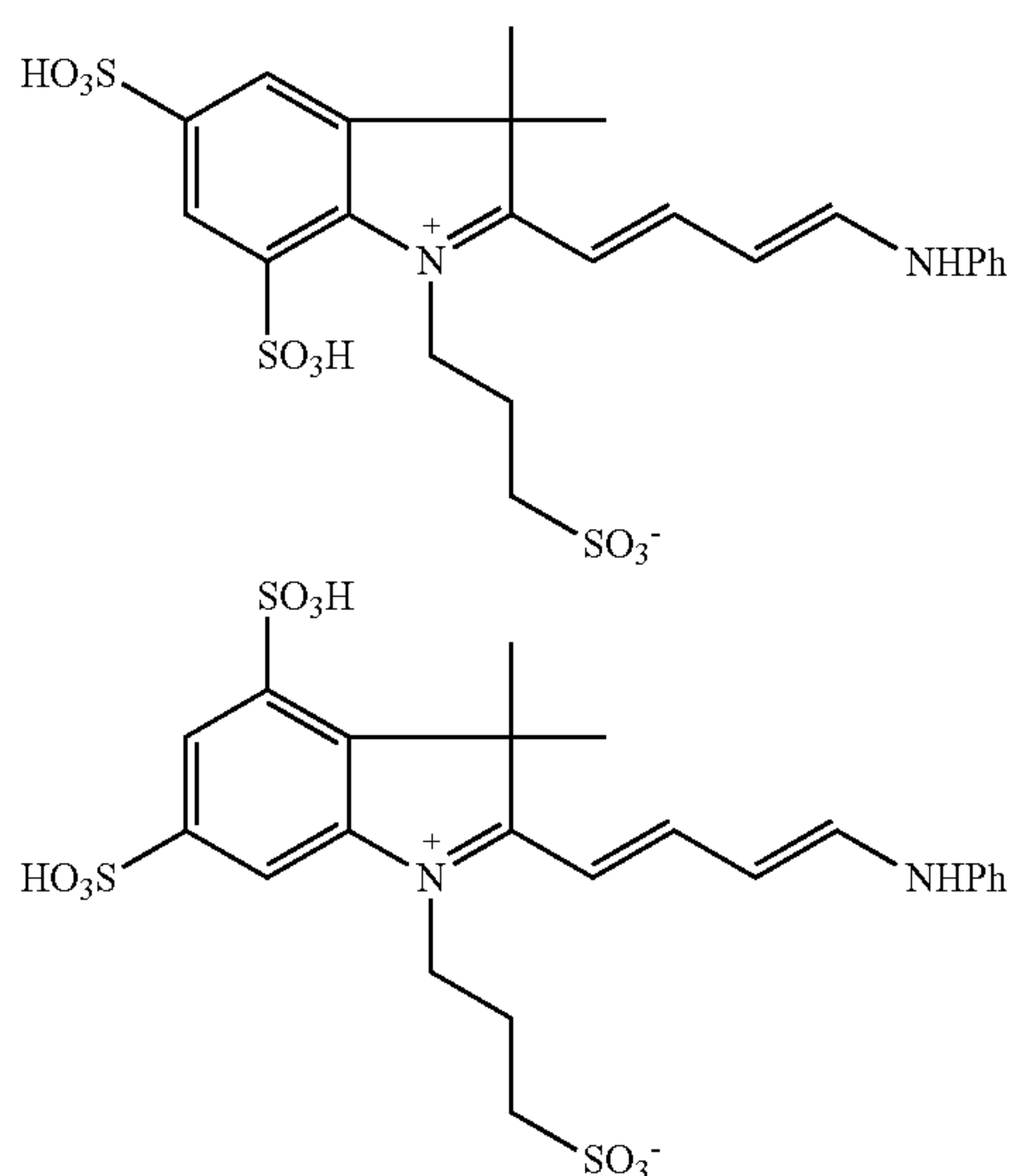
1.21 2-[(1E,3E)-4-Anilinobuta-1,3-dienyl]-3,3-dimethyl-1-(3-sulfonatopropyl)-3H-indoleninium-5,7-disulfonate and 2-[(1E,3E)-4-Anilinobuta-1,3-dienyl]-3,3-dimethyl-1-(3-sulfonatopropyl)-3H-indoleninium-4,6-disulfonate
