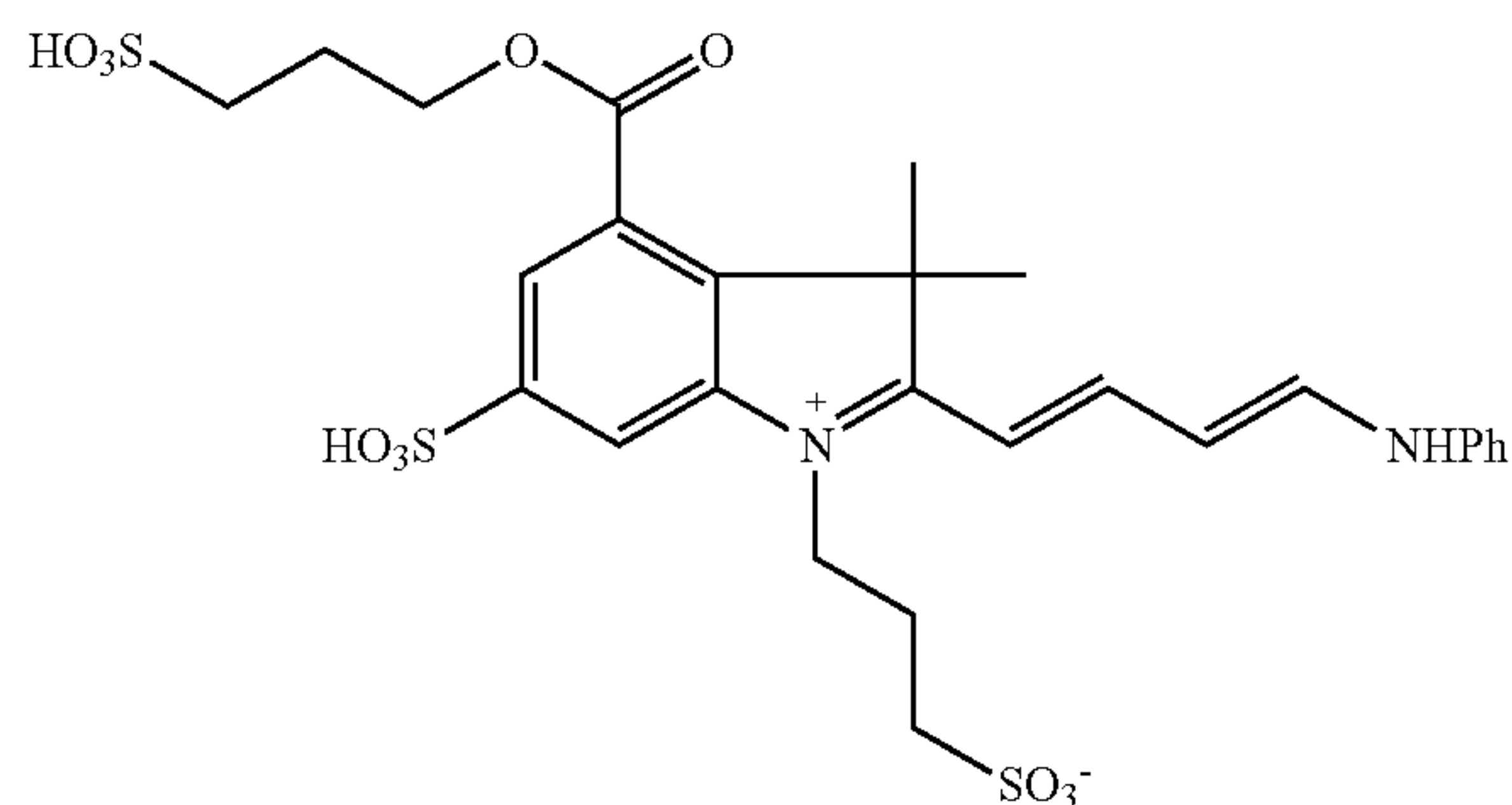
1.19 2-[(1E,3E)-4-Anilinobuta-1,3-dienyl]-3,3-dimethyl-1-(3-sulfonatopropyl)-3H-indoleninium-4-(sulfonatopropylcarboxylate)-6-sulfonate
