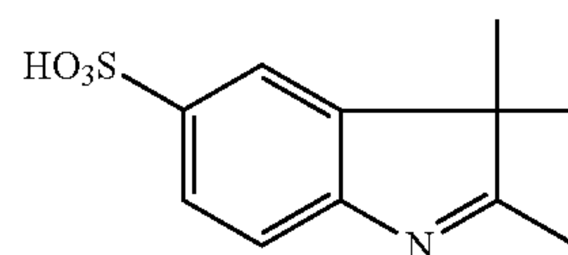
1.3 2,3,3-Trimethylindoleninium-5-sulfonate
