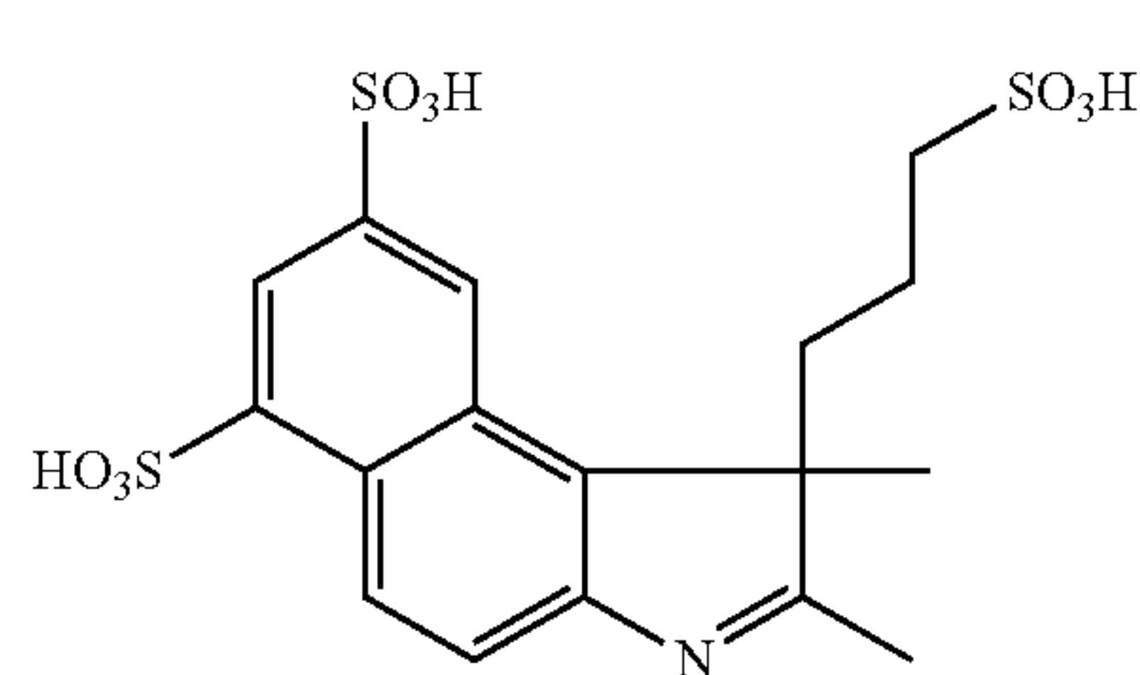
1,2-Dimethyl-1-(3-sulfopropyl)benz[e]indole-6,8-disulfonate
