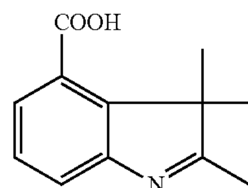
1.2 2,3,3-Trimethyl-4-carboxy-3H-indole
