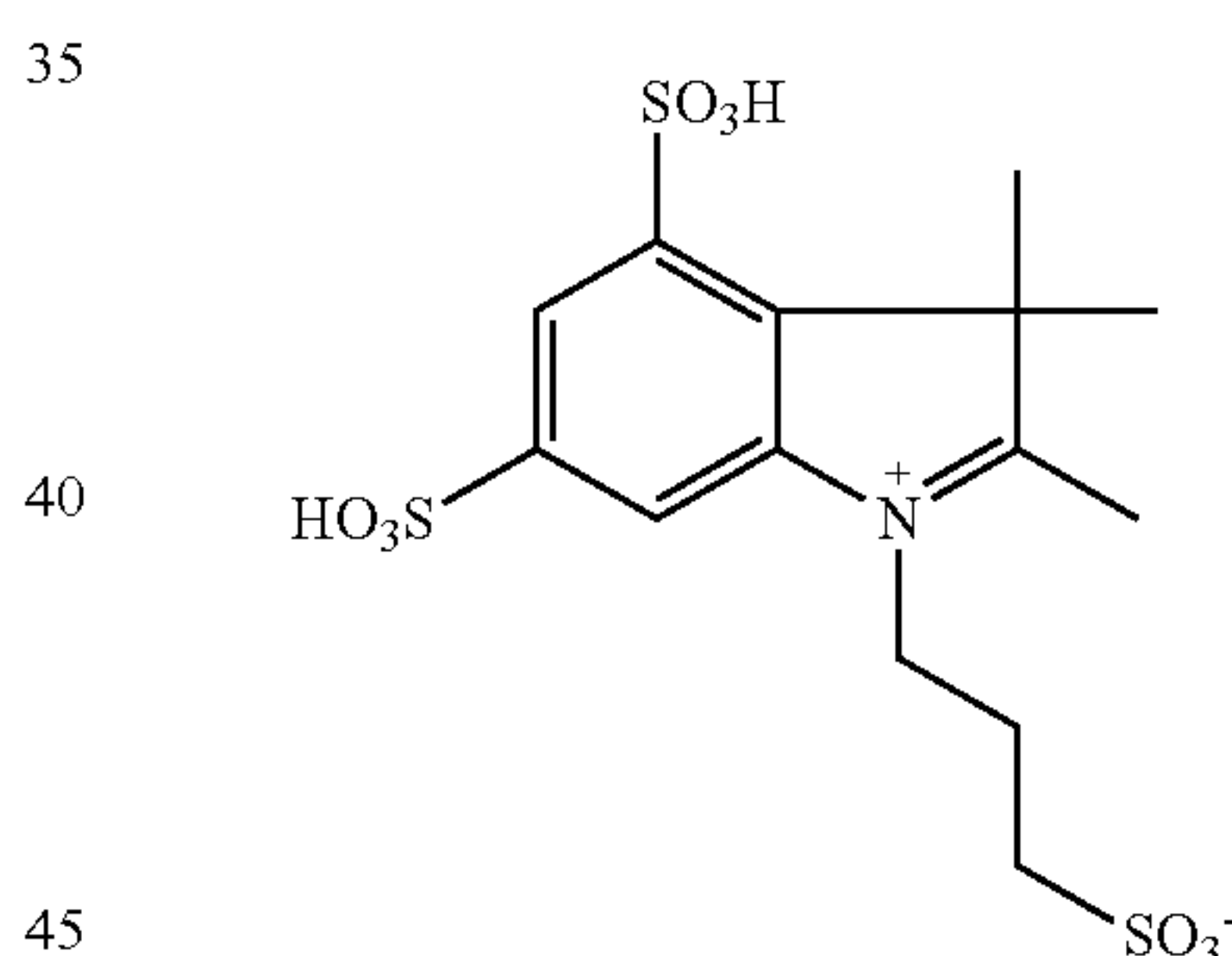
1-(3-Sulfonatopropyl)-2,3,3-trimethylindoleninium
