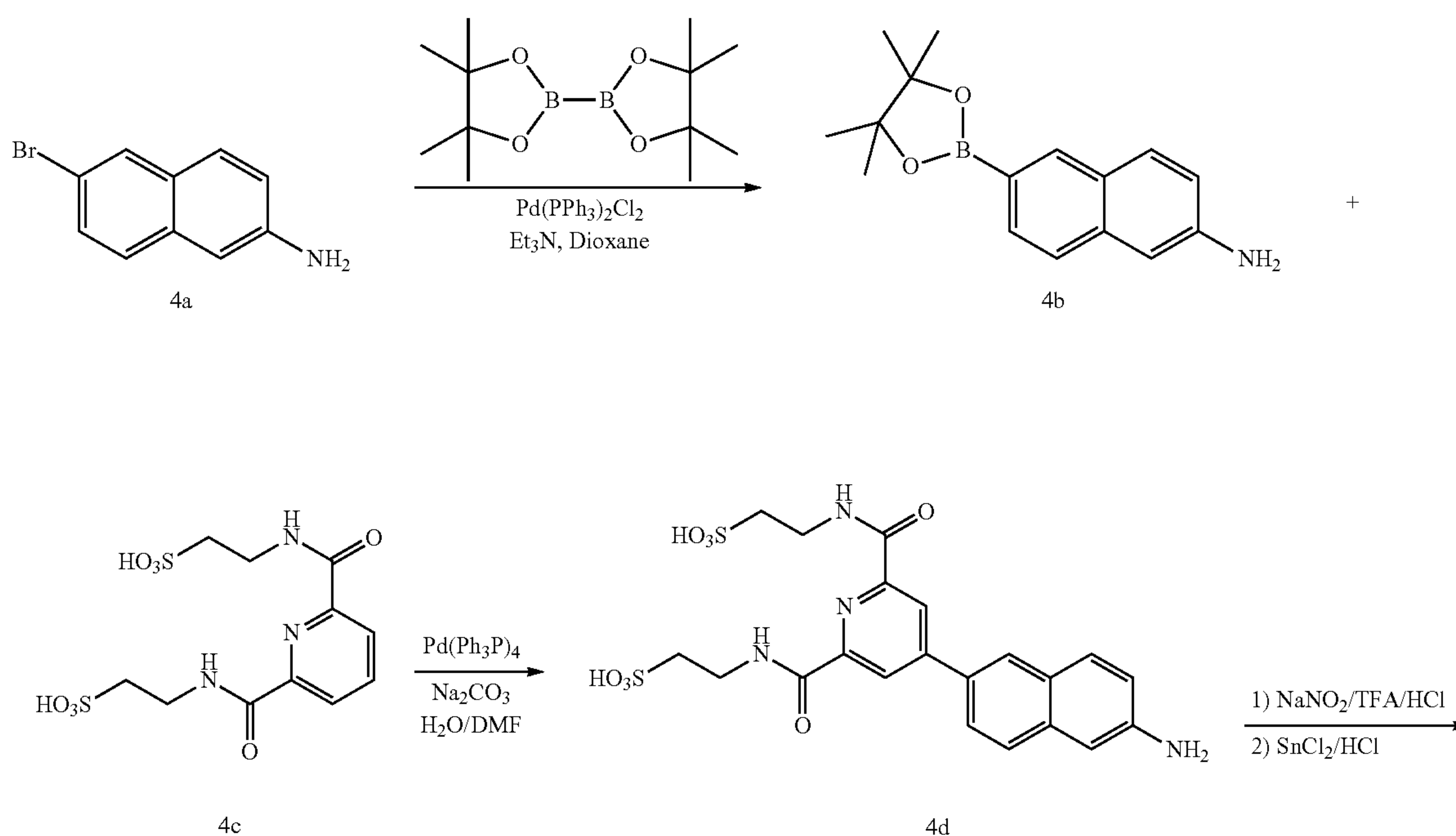
Scheme 6: Synthesis of pyridyl benzimidazole cyanine dyes
