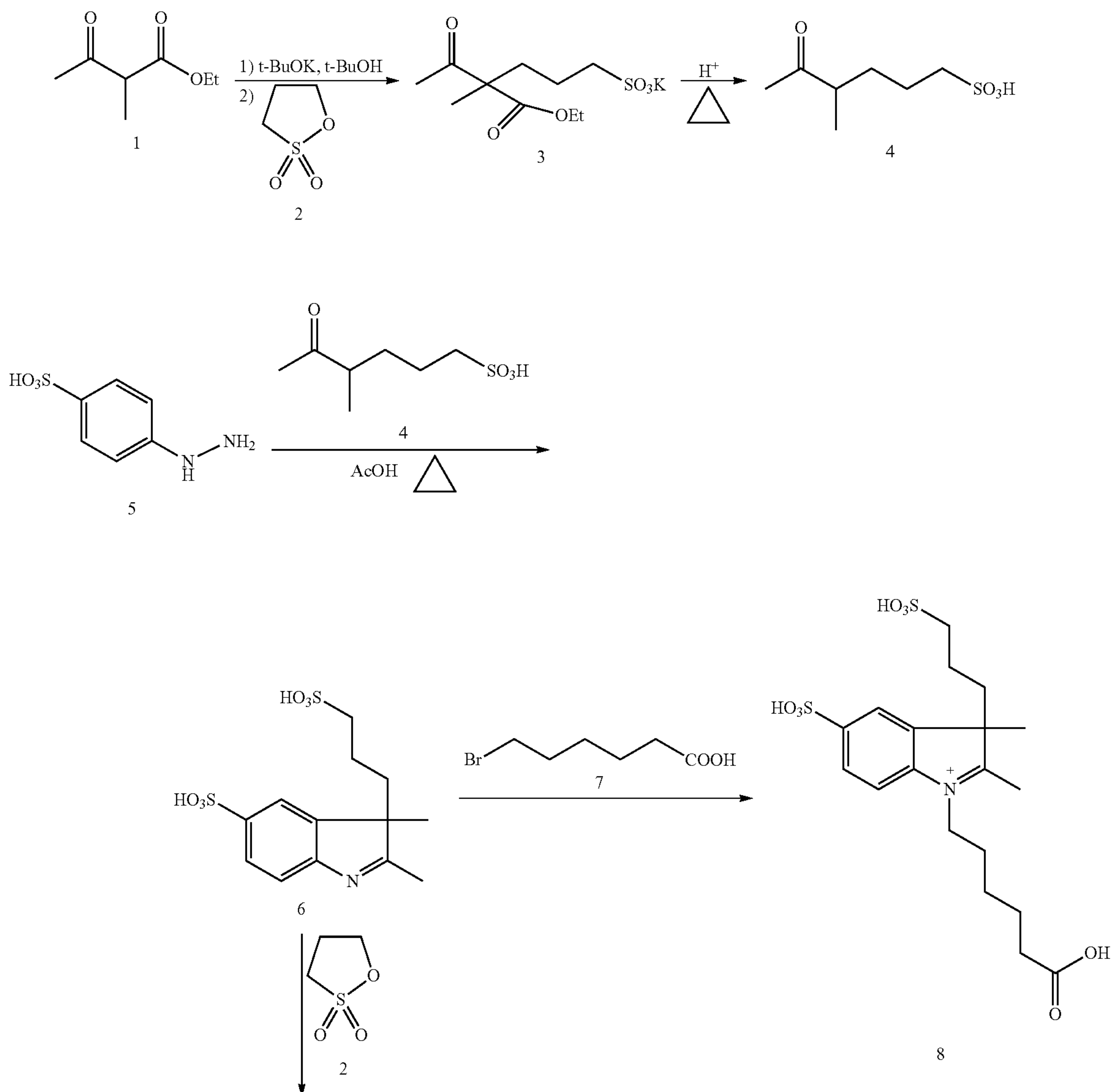
Scheme 1. Synthesis of Pentasulfonated Cyanine Dyes
