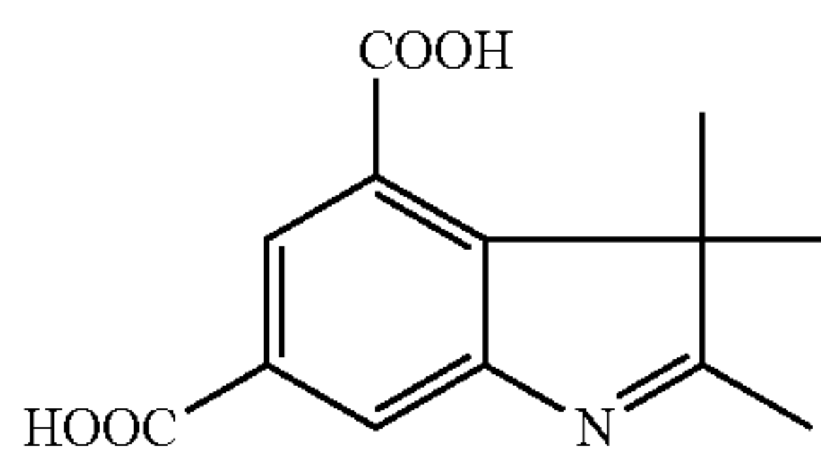
2,3,3-trimethyl-4,6-dicarboxy-3H-indole
