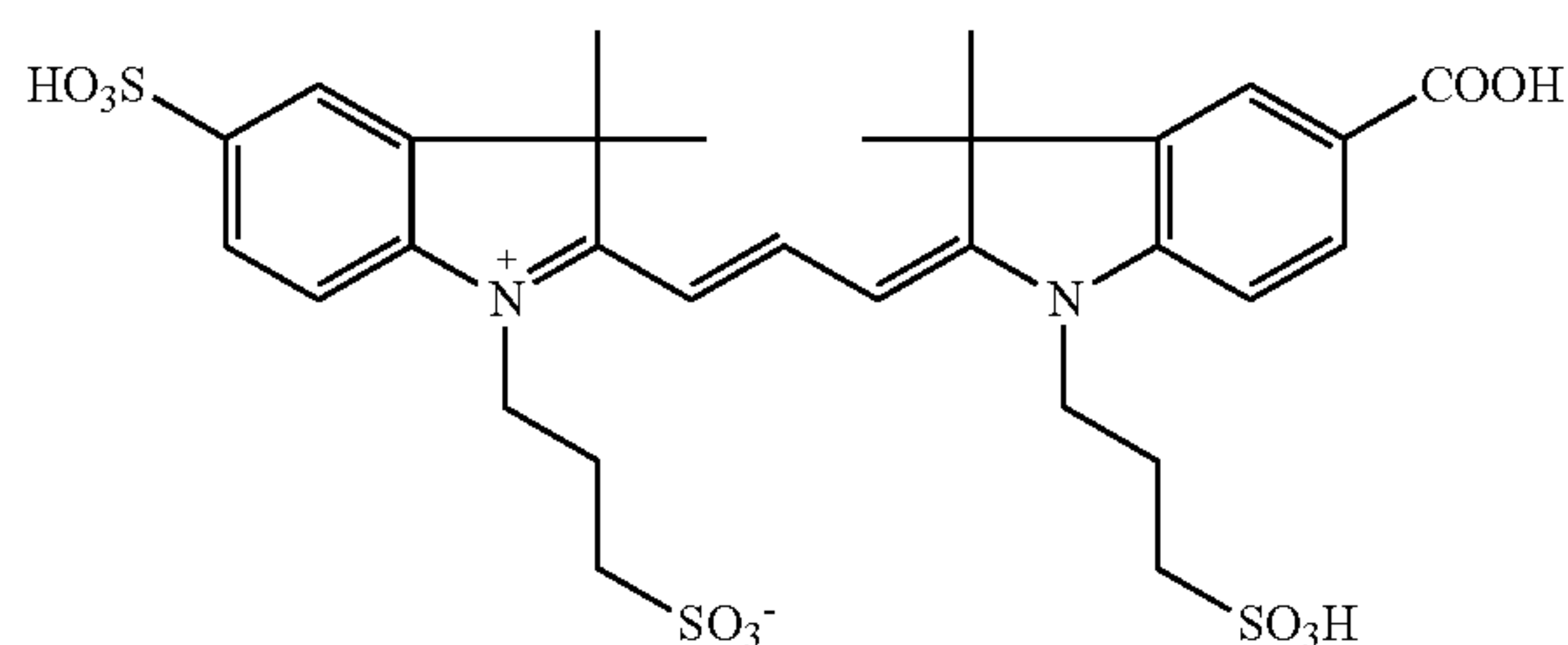
1.22 Preparation of 1.22
