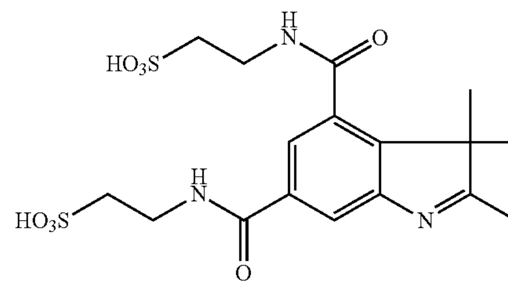
2,3,3-trimethyl-4,6-di(sulfoethylcarboxamide)-3H-indole
